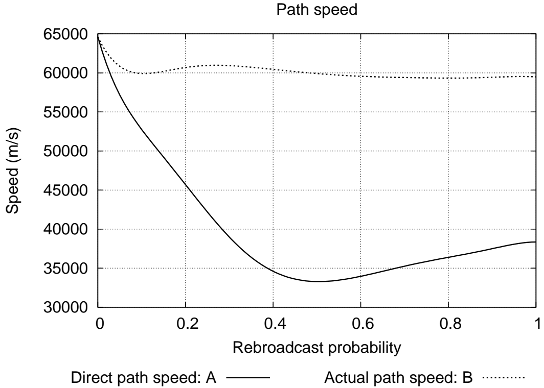
Figure 3.6: Path speed
