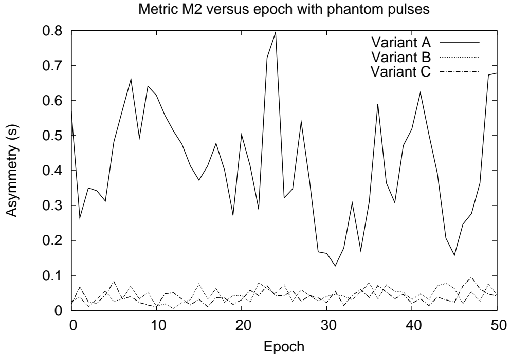
Figure 7.9: Phantom pulses
