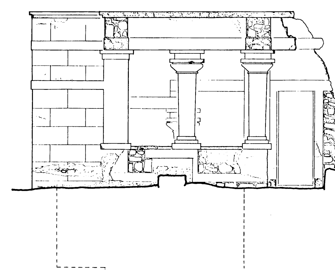
South Elevation
