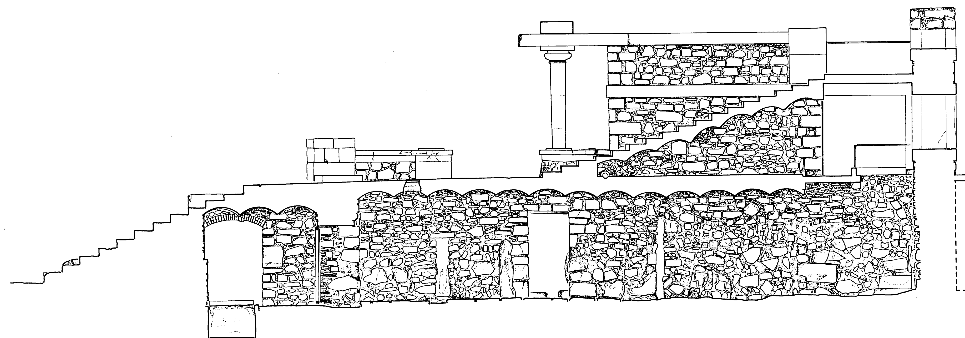
Section B-B
