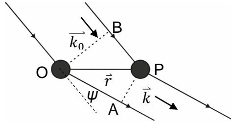
Figure 2.2 The incident and scattered beam directions and the path difference
