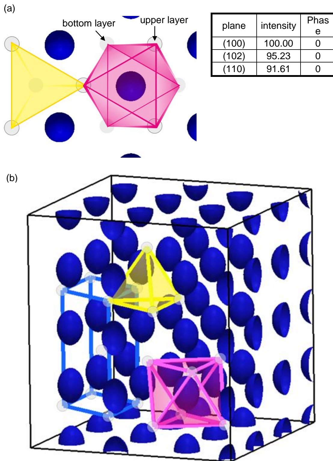
Figure 5.9. Neutron scattering length density contour map of 12-12-12Rb + 17.5wt% C 19 D 40 in the HCP phase: (a) top view and (b) side view. (Blue: high NSLD density; gray sphere: supramolecule; yellow: tetrahedron; pink: octahedron)
