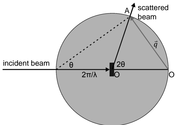
Figure 2.5 Ewald Sphere
