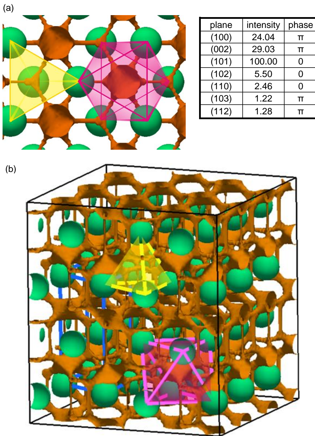
Figure 5.7. The contour maps of electron density of 12-12-12Rb + 17.5wt% C 19 D 40 in the HCP phase: (a) top view and (b) side view. (Green: high ED; Orange: low ED; yellow: tetrahedron; pink: octahedron)
