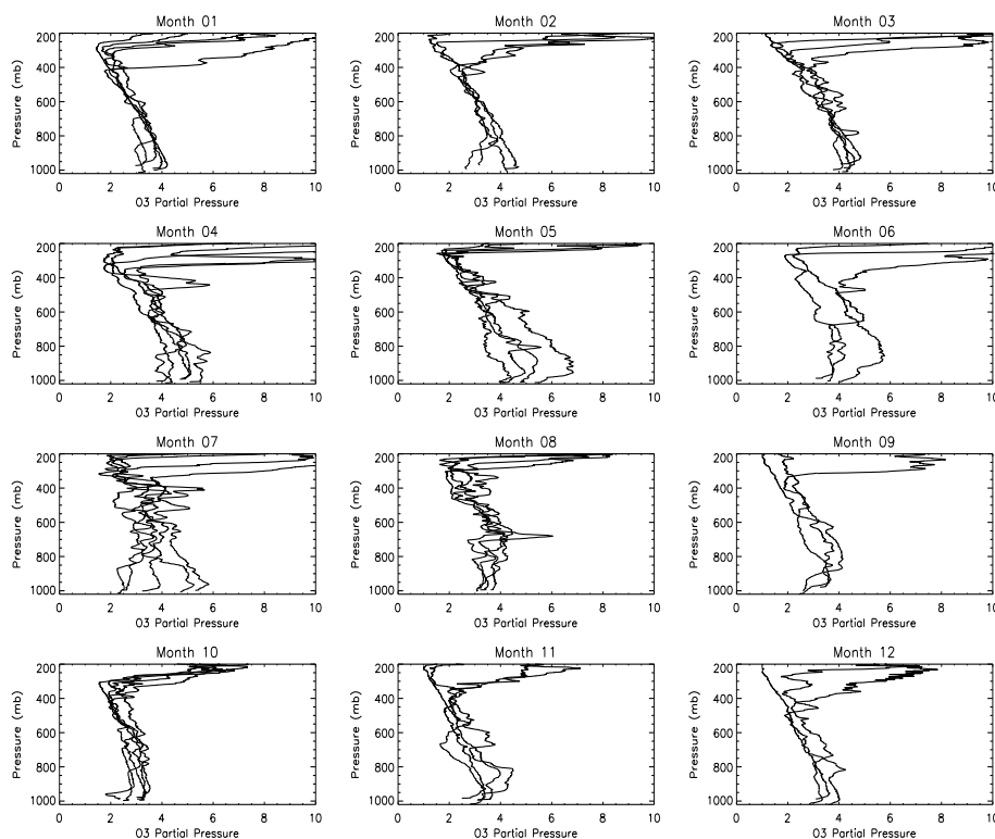
Figure 3.18: Ozonesonde profiles (partial pressure - Pa) for 2008 from Lerwick, Shetland.
