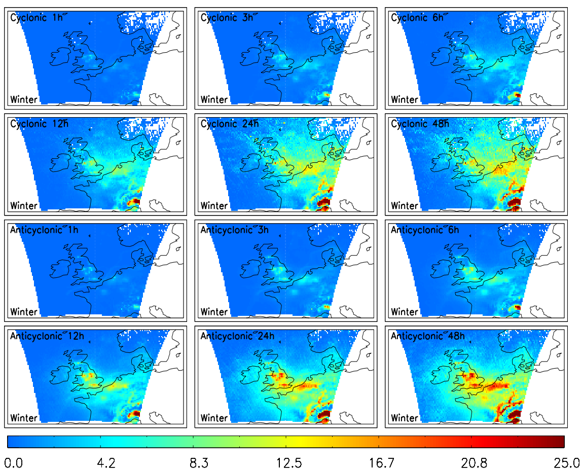
Figure 6.10: Winter AQUM column abundances of tracers with different lifetimes for cyclonic and anticyclonic conditions.
