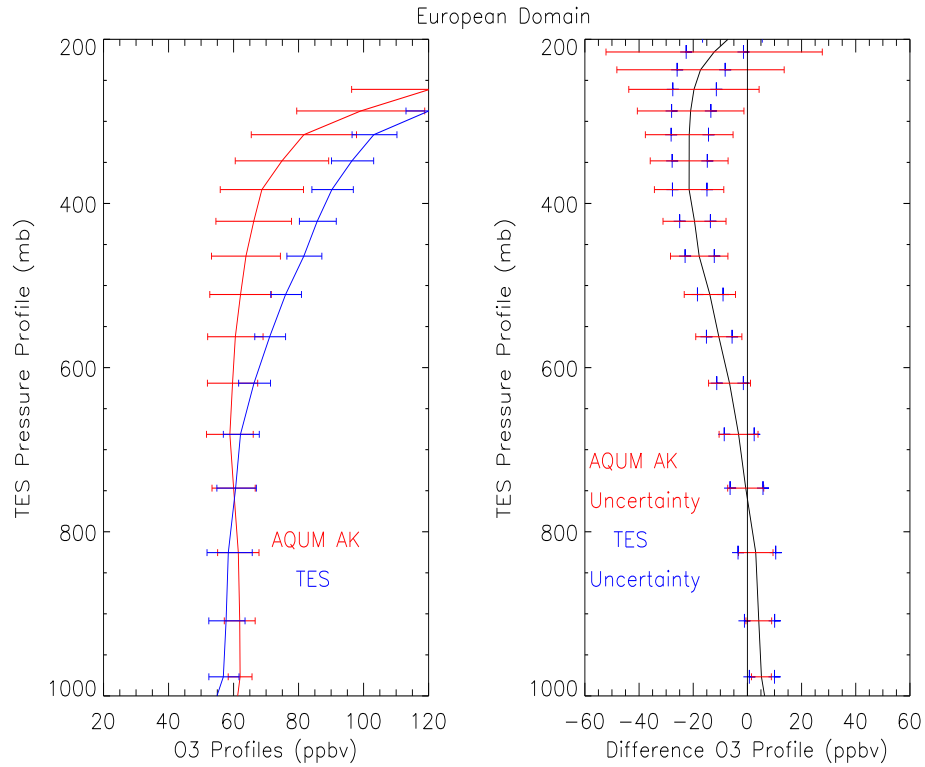
Figure 3.10: European domain July 2006 averaged vertical profiles (ppbv) of AQUM (red), TES (blue) O 3 and the difference.
