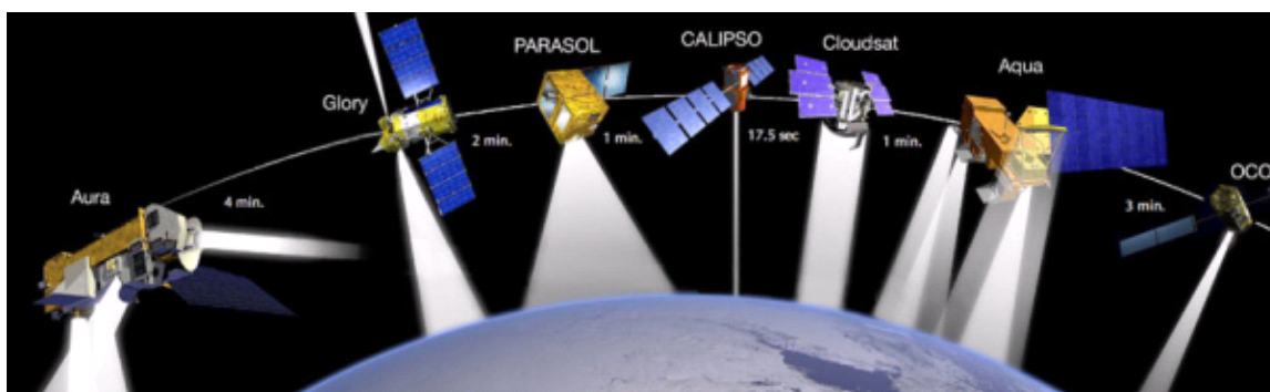
Figure 3.3: The NASA A-Train consists of satellites with various scientific missions. In the figure, AURA is on the left in the train, while AQUA is approximately 10 minutes ahead (NASA, 2012).
