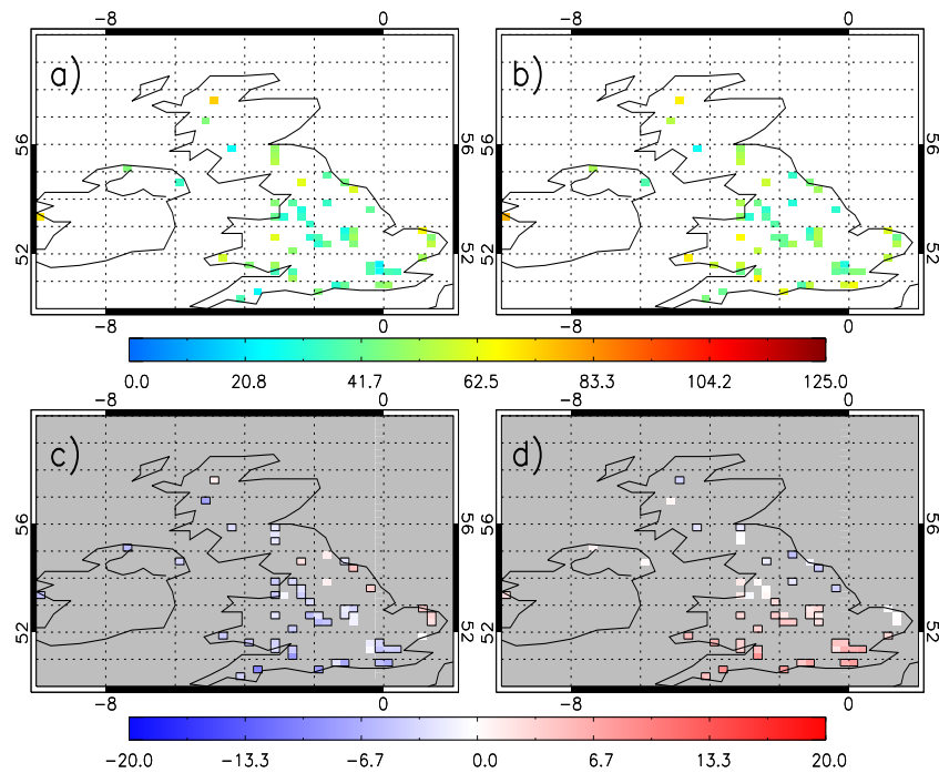
Figure 5.15: Composites of winter AURN surface \text{O}_3 ( \mu\text{g}/\text{m}^3 ), 2000-2010, for (a) anti-cyclonic conditions, (b) cyclonic conditions, (c) anticyclonic anomalies and (d) cyclonic anomalies.
