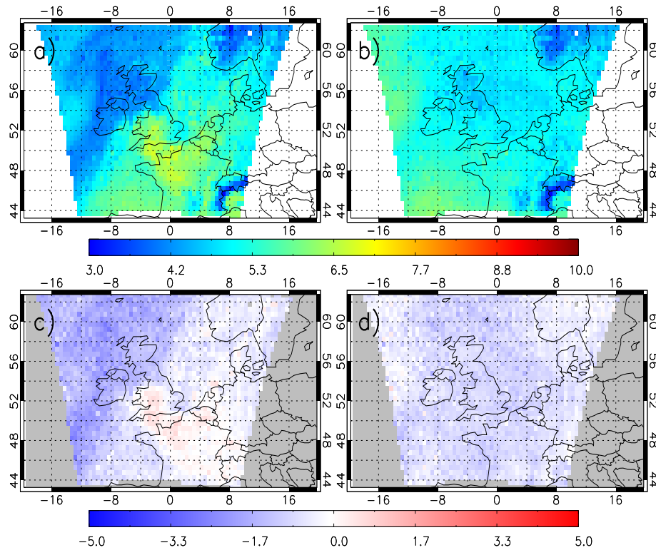
Figure 3.12: July 2006 subcolumn O_3 ( 10^{17} molecules/ cm^2 ), surface-500 hPa, for a) AQUM, b) AQUM (AKs applied), c) AQUM - OMI mean bias and d) AQUM (AKs applied) - OMI mean bias.
