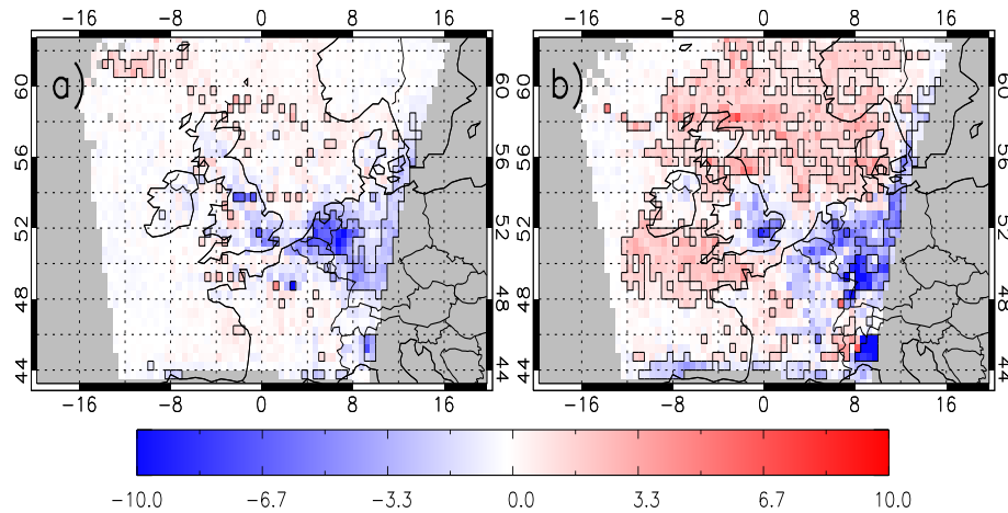
Figure 4.7: Mean bias in tropospheric NO 2 column ( \times 10^{15} molecules/cm 2 ) for 2006 between AQUM Run C (with AKs applied) and SCIAMACHY for (a) summer (RMSE= 4.55 \times 10^{15} molecules/cm 2 and FGE=0.63) and (b) winter ( 6.77 \times 10^{15} molecules/cm 2 and FGE=0.70).
