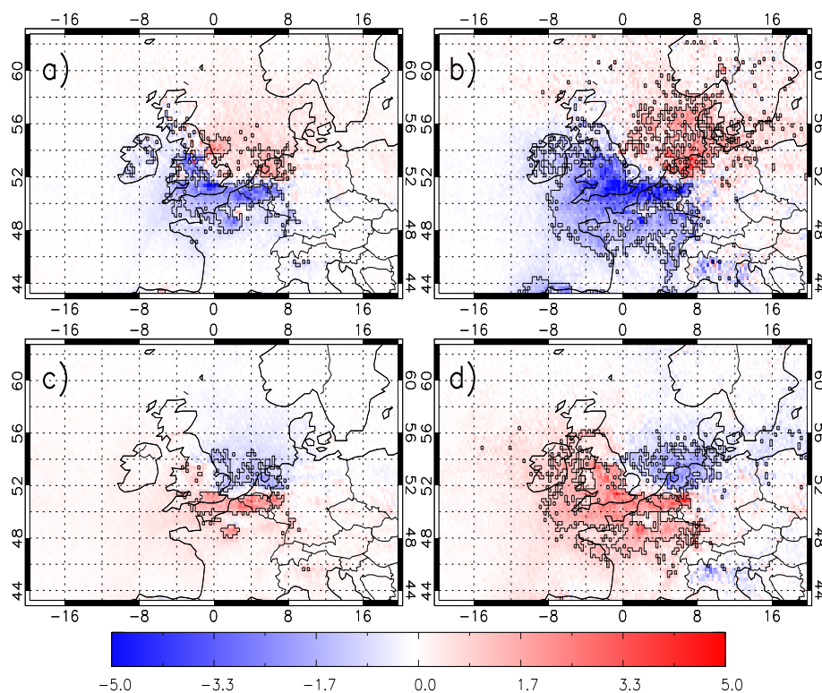
Figure 5.3: Anomalies of OMI column NO 2 composites compared to seasonal 7-year average ( \times 10^{15} molecules/cm 2 ) for (a) summer cyclonic, (b) winter cyclonic, (c) summer anticyclonic and (d) winter anticyclonic conditions. Black boxes indicate where the anomalies are statistically significant at the 95% level.
