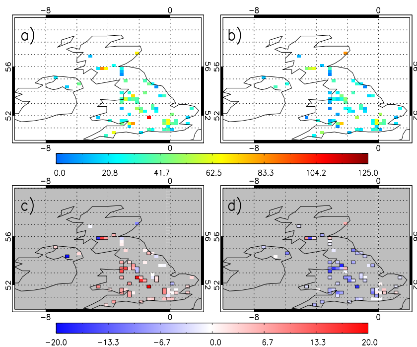
Figure 5.13: Composites of winter AURN surface \text{NO}_2 ( \mu\text{g}/\text{m}^3 ), 2000-2010, for (a) south-easterly flow, (b) north-westerly flow, (c) south-easterly anomalies and (d) north-westerly anomalies.
