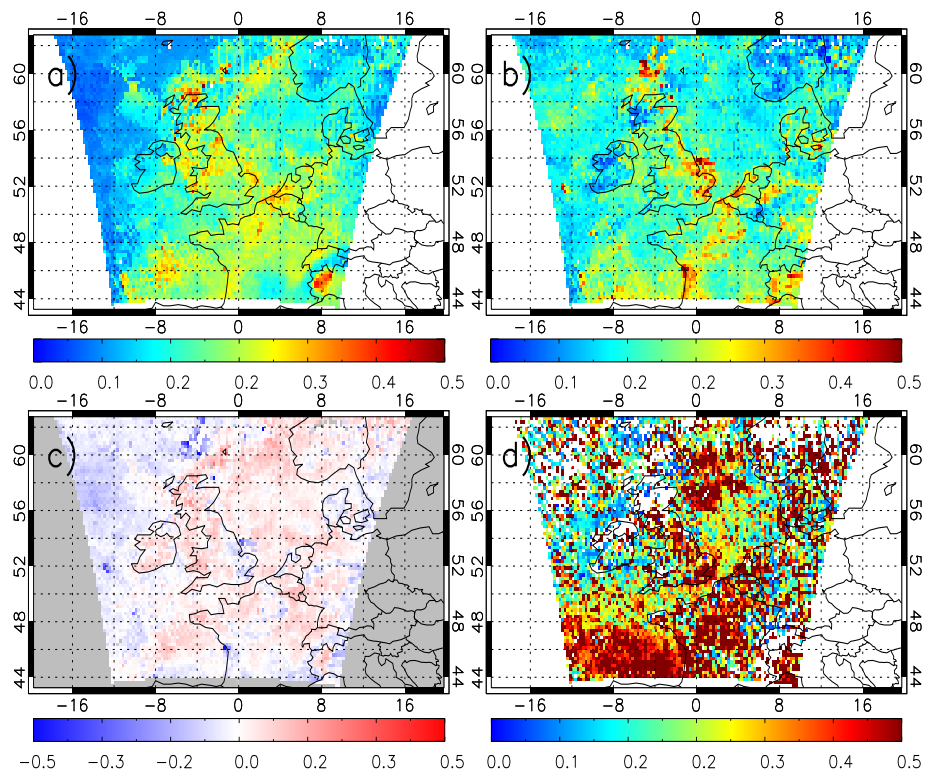
Figure 3.7: July 2006 column aerosol optical depth (AOD): a) AQUM (0.55 \mu\text{m} ), b) MODIS (0.55 \mu\text{m} ), c) AQUM - MODIS mean bias and d) OMI (0.44 \mu\text{m} ).
