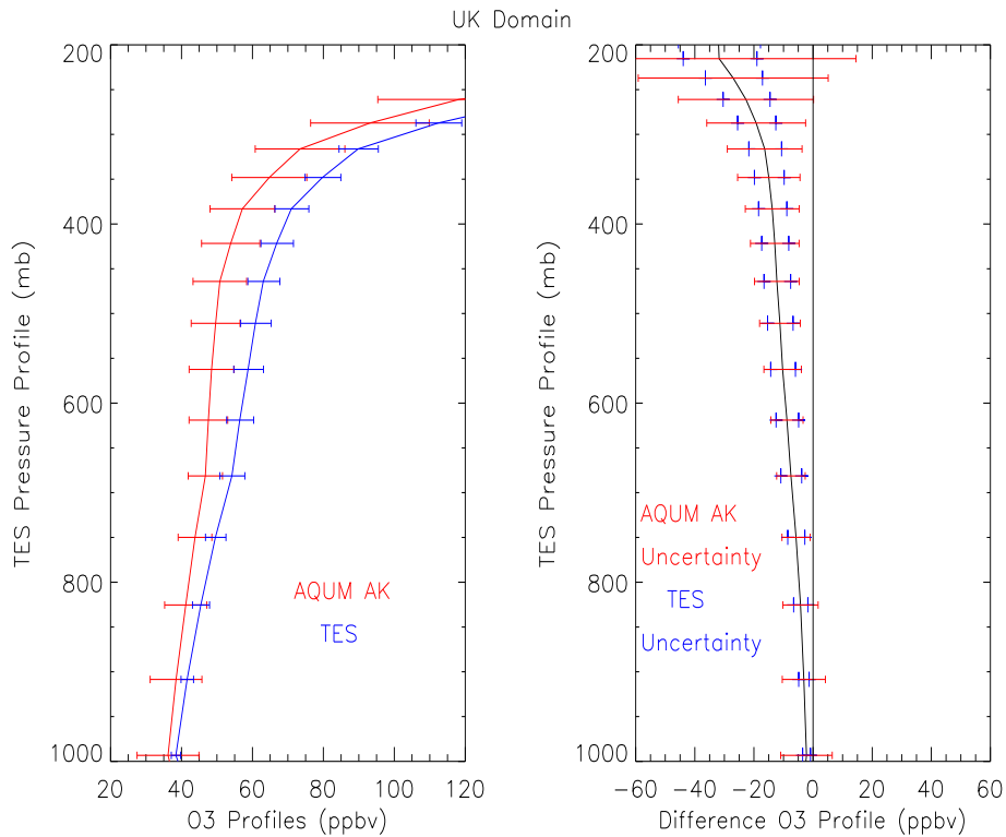
Figure 3.9: UK domain July 2006 averaged vertical profiles (ppbv) of AQUM (red), TES (blue) O_3 and the difference.
