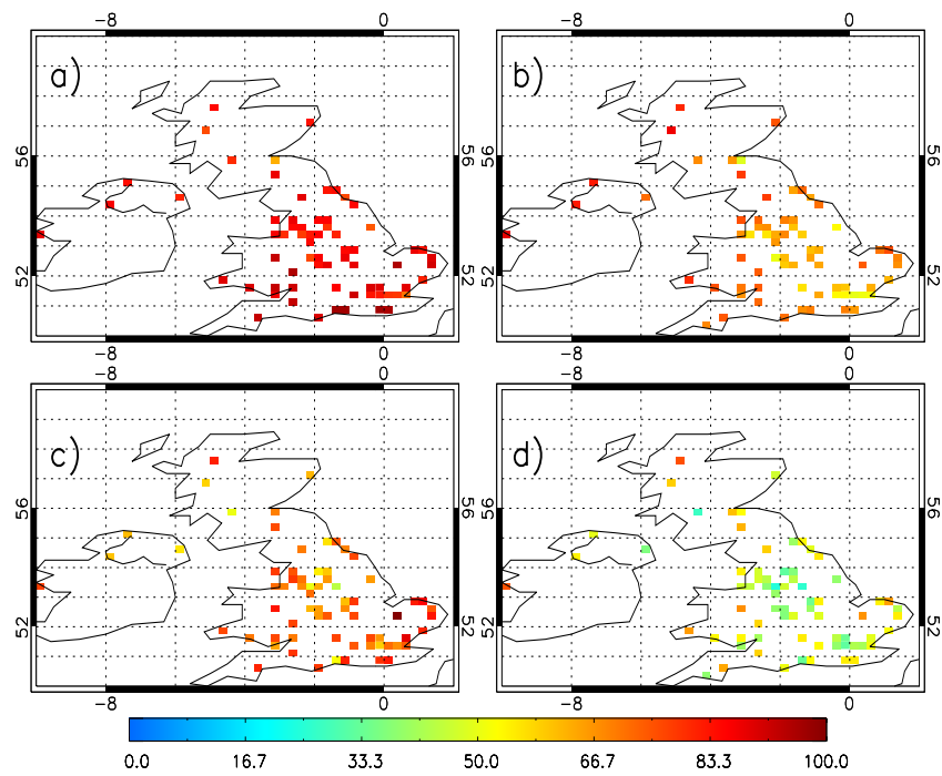
Figure 4.16: Surface O_3 ( \mu\text{g}/\text{m}^3 ) for 2006 of (a) AQUM Run MACC summer, (b) AQUM Run MACC winter, (c) AURN summer and (d) AURN winter.
