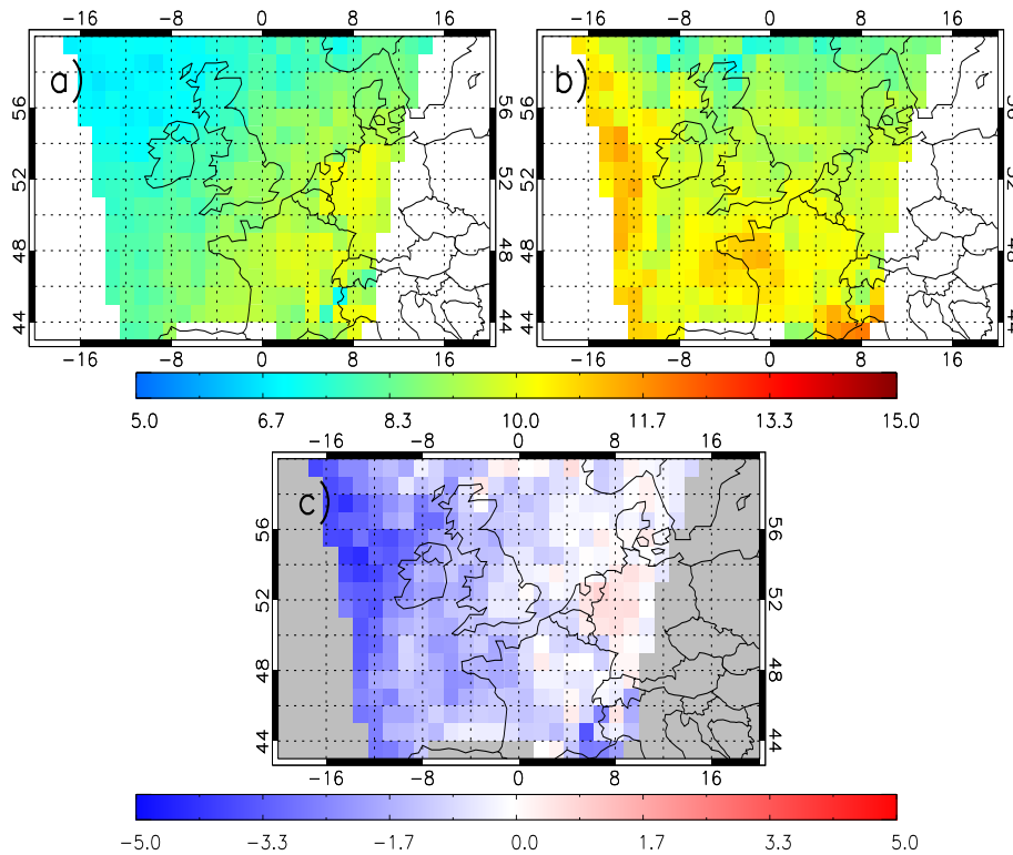
Figure 3.13: Tropospheric column O_3 ( 10^{17} molecules/cm ^2 ) for a) AQUM, b) OMI/MLS and c) AQUM - OMI/MLS biases.
