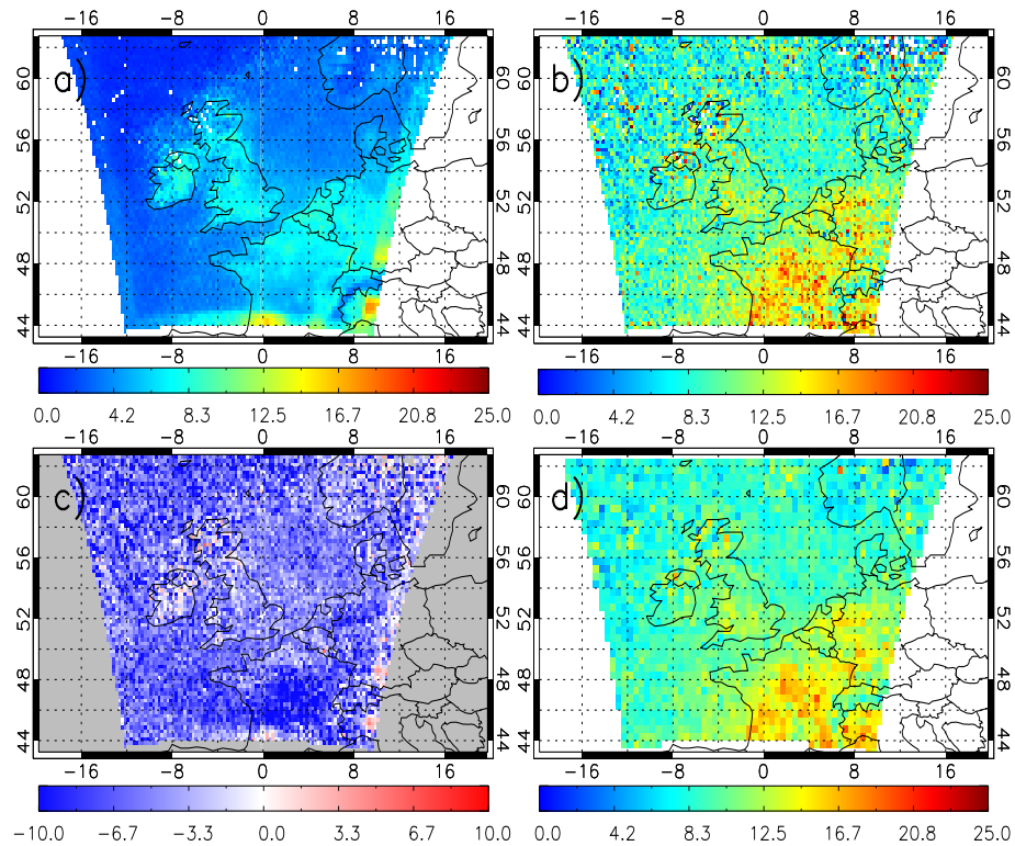
Figure 3.5: July 2006 tropospheric column HCHO ( 10^{15} molecules/cm 2 ): a) AQUM, b) OMI and c) mean bias. d) OMI column HCHO on a coarser 0.5^\circ \times 0.5^\circ grid.
