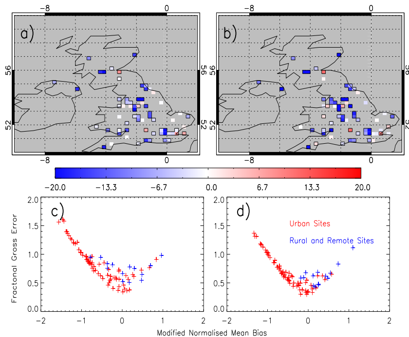
Figure 4.15: Surface NO 2 ( \mu\text{g}/\text{m}^3 ) AQUM Run MACC - AURN mean bias for 2006 of (a) summer and (b) winter. AQUM - AURN MNMB and FGE for (c) summer and (d) winter.
