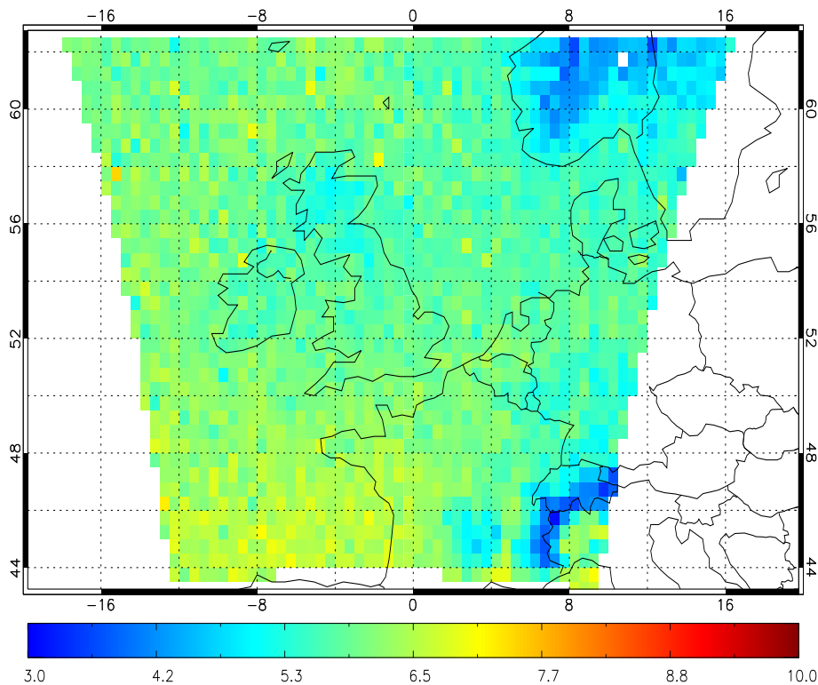
Figure 3.11: OMI subcolumn O_3 ( 10^{17} molecules/ cm^2 ), surface-500 hPa, for July 2006.
