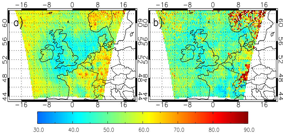
Figure 4.2: New seasonal satellite mean error, obtained by reduction of random error using the methodology described in Section 4.2.2, as a percentage of the simple seasonal mean of satellite total error for 2006. Smoothing errors have been removed. (a) Summer and (b) winter.
