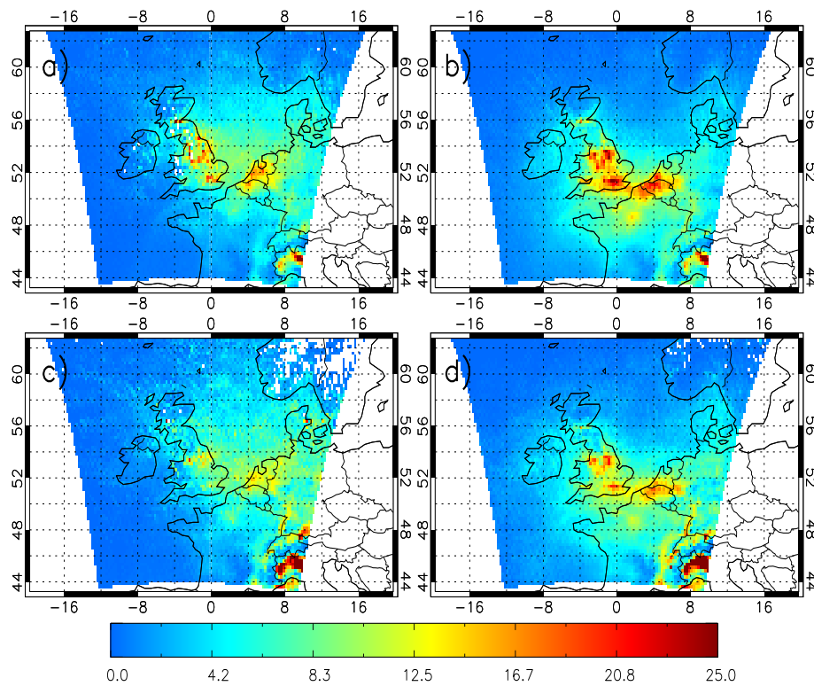
Figure 6.8: Composites of AQUM (AKs applied) column tracer 24 (i.e. tracer with a lifetime of 24 hours) ( \times 10^{15} molecules/cm 2 ) for 2006-2010 for (a) summer cyclonic, (b) summer anticyclonic, (c) winter cyclonic and (d) winter anticyclonic conditions.
