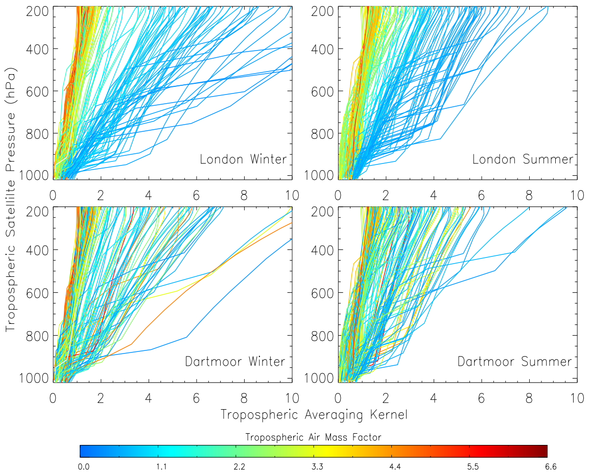
Figure 4.1: Example OMI averaging kernels for London (top) and Dartmoor (bottom) for summer (right) and winter (left) 2006. Averaging kernels have been coloured according to their respective tropospheric air mass factor values.
