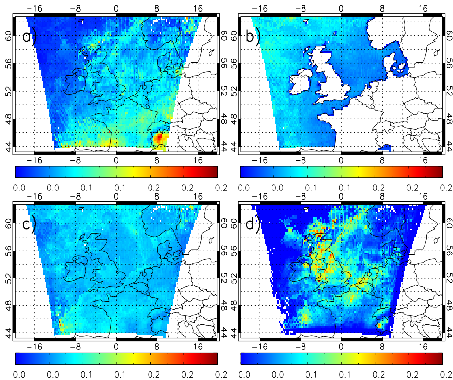
Figure 3.8: AQUM July 2006 column OD ( 0.55 \mu\text{m} ): a) ammonium sulphate b) Sea Salt, c) fossil fuel burning and d) ammonium nitrate.
