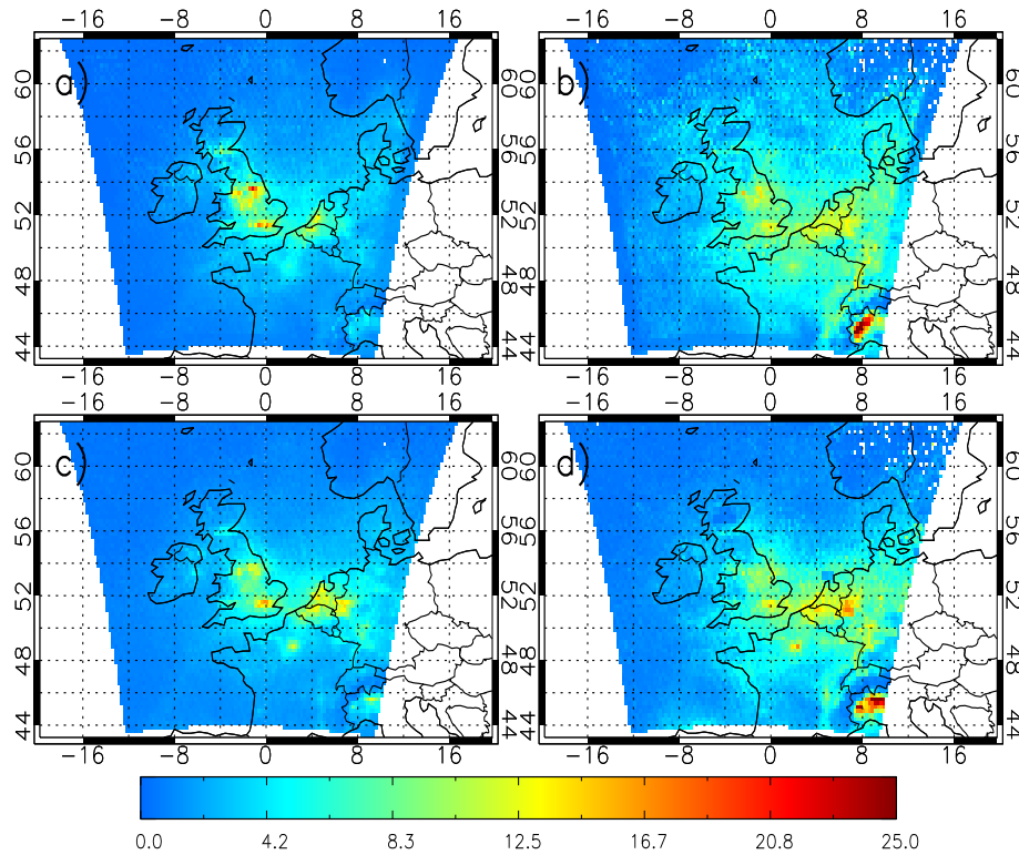
Figure 4.4: Tropospheric \text{NO}_2 column ( \times 10^{15} molecules/ \text{cm}^2 ) for 2006 of (a) AQUM Run C (with averaging kernels (AK) applied) summer, (b) AQUM Run C (with AKs applied) winter, (c) OMI summer and (d) OMI winter.
