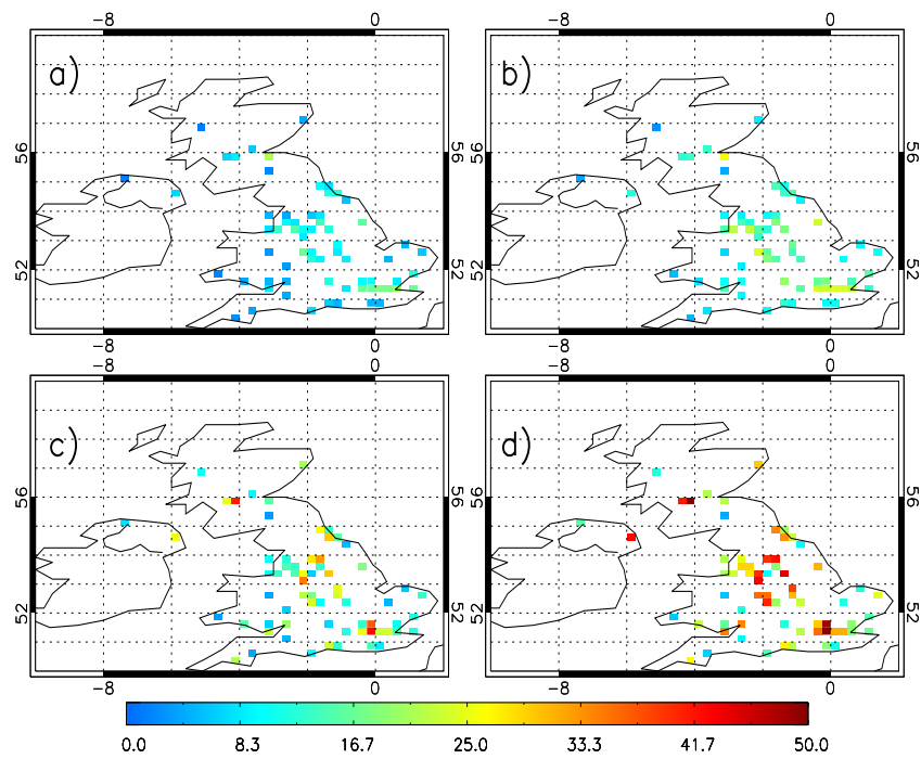
Figure 4.8: Surface NO 2 ( \mu\text{g}/\text{m}^3 ) for 2006 of (a) AQUM Run C summer, (b) AQUM Run C winter, (c) AURN summer and (d) AURN winter.
