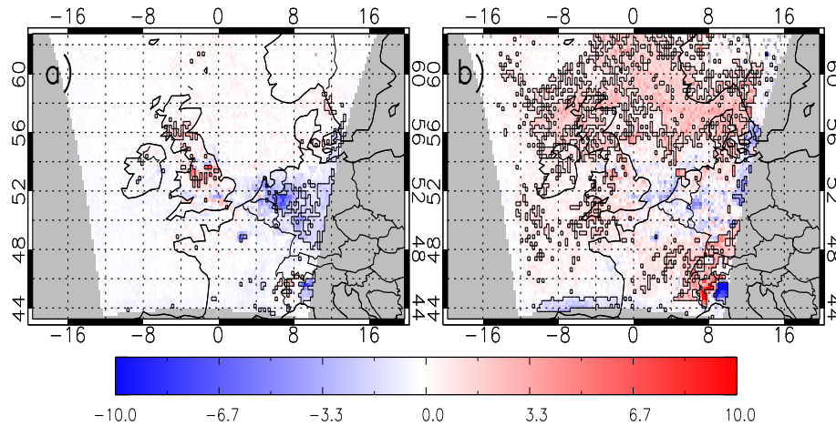
Figure 4.5: Mean bias in tropospheric NO 2 column ( \times 10^{15} molecules/cm 2 ) for 2006 between AQUM Run C (with AKs applied) and OMI for (a) summer (RMSE= 3.68 \times 10^{15} molecules/cm 2 and FGE=0.65) and (b) winter ( 5.12 \times 10^{15} molecules/cm 2 and FGE=0.63). The RMSE and FGE are over the UK between 8°W-2°E and 50-60°N and black polygoned regions show significant differences. Also the same for other mean bias plots below in this chapter.
