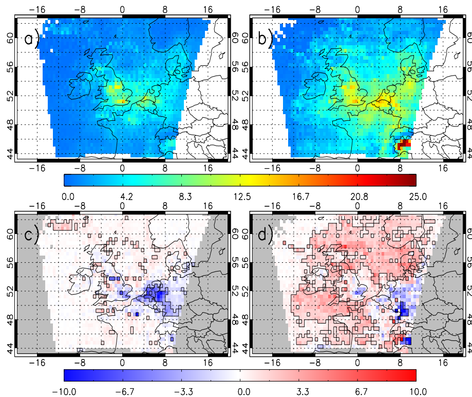
Figure 4.13: Tropospheric column \text{NO}_2 ( \times 10^{15} molecules/ \text{cm}^2 ) for 2006 from AQUM Run MACC (AKs applied) for (a) summer and (b) winter. AQUM Run MACC (AKs applied) and SCIAMACHY mean bias for (c) summer (RMSE= 4.51 \times 10^{15} molecules/ \text{cm}^2 and FGE=0.60) and (d) winter (RMSE= 6.83 \times 10^{15} molecules/ \text{cm}^2 and FGE=0.70).
