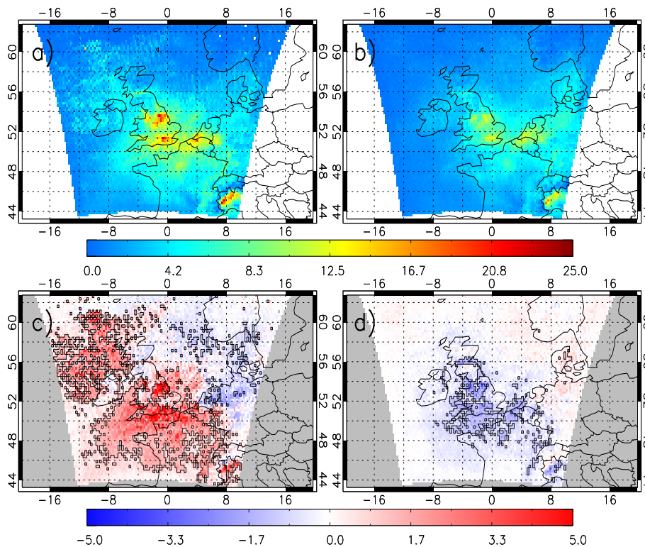
Figure 5.19: Composites of AQUM column \text{NO}_2 ( \times 10^{15} molecules/cm 2 ) between 2006-2010 for (a) PWC 5 (Drizzle) conditions, (b) PWC 8 (Showers) conditions, (c) PWC 5 (Drizzle) anomalies and (d) PWC 8 (Showers) anomalies.
