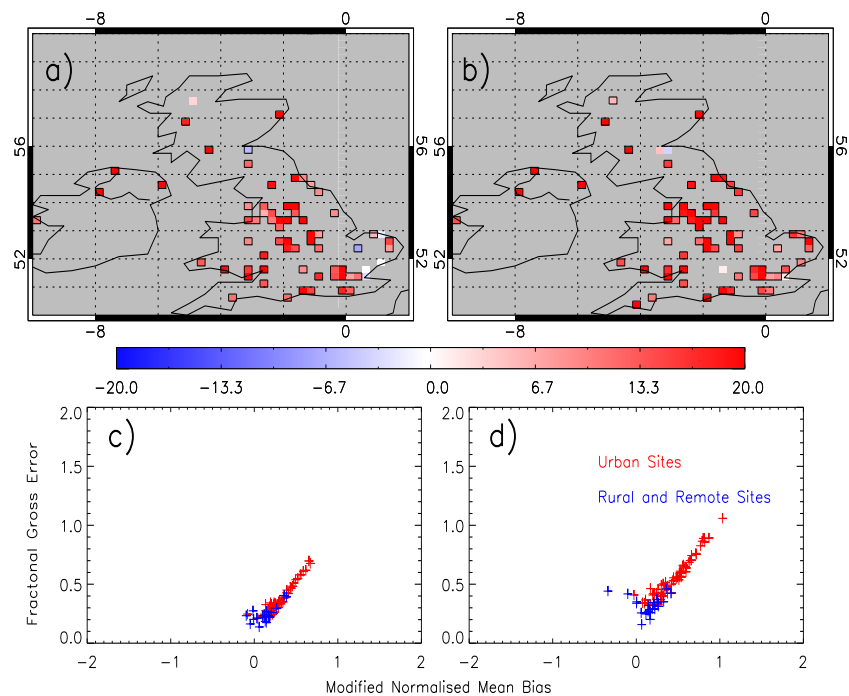
Figure 4.17: Surface O_3 ( \mu\text{g}/\text{m}^3 ) AQUM Run MACC - AURN mean bias for 2006 of (a) summer and (b) winter. AQUM - AURN MNMB and FGE for (c) summer and (d) winter.
