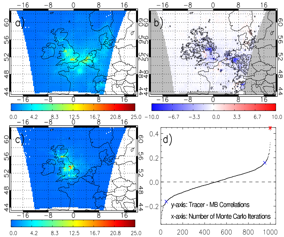
Figure 4.19: Tropospheric column ( \times 10^{15} molecules/cm 2 ) for JJA 2006 of (a) AQUM Run E1 NO 2 (AKs applied), (b) AQUM Run E1 NO 2 (AKs applied) - OMI (RMSE= 3.02 \times 10^{15} molecules/cm 2 and FGE=0.68) and (c) AQUM Run E2 Tracer (AKs applied). (d) Peak Run E2 and co-located Run C-OMI MB correlation (red star) significance distribution. Black dots are Run E2 and random Run C-OMI MB correlations. Blue X=5 th and 95 th percentiles of the 1000 size sample.
