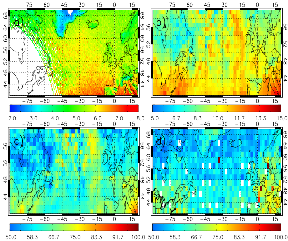
Figure 3.15: Atlantic O_3 for July 2006 for a) OMI subcolumns ( \times 10^{17} molecules/cm 2 ), surface - 500 hPa, b) OMI/MLS tropospheric columns ( \times 10^{17} molecules/cm 2 ), c) OMI/MLS tropospheric mean profiles (ppbv) and d) TES tropospheric mean profiles (ppbv) (JJA 2006).
