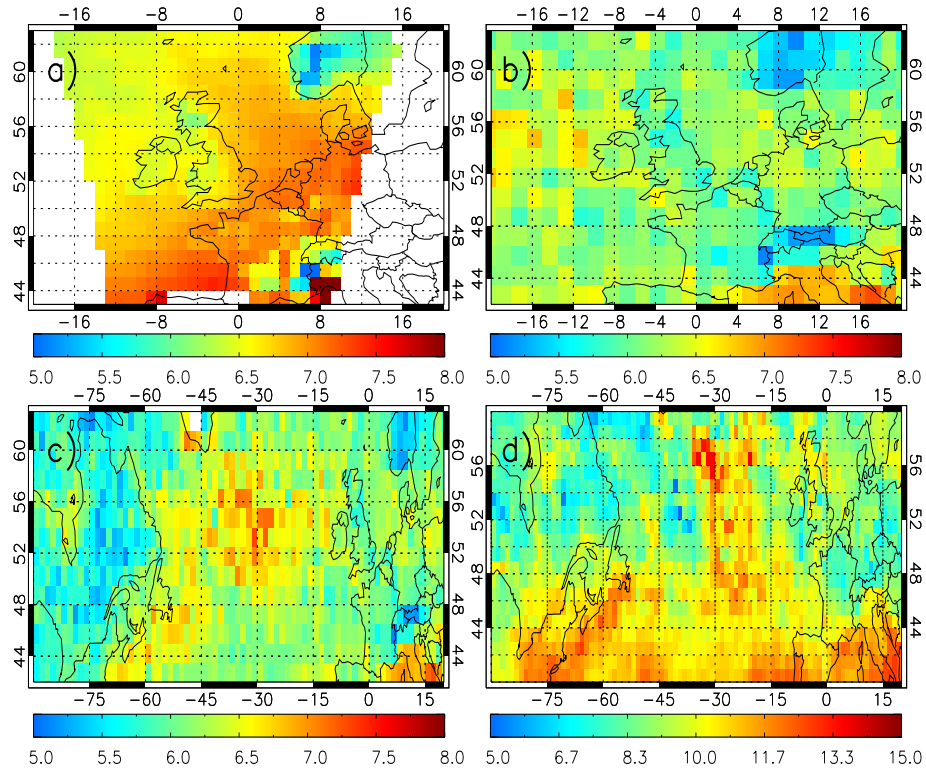
Figure 3.16: JJA 2008 subcolumn, surface - 450 hPa, O 3 ( 10^{17} molecules/cm 2 ) for a) AQUM, b) GOME-2 and c) GOME-2 Atlantic coverage. d) OML/MLS tropospheric column O 3 ( 10^{17} molecules/cm 2 ) for JJA 2008.
