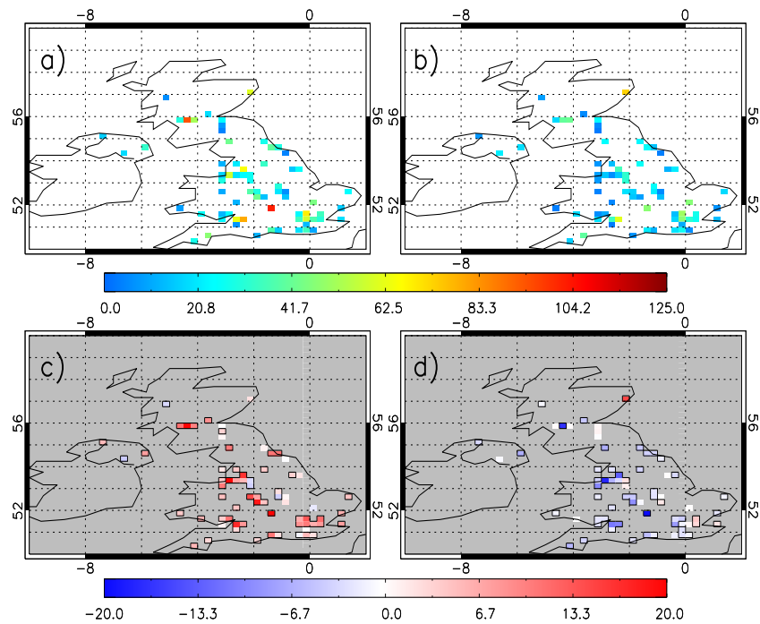
Figure 5.12: Composites of summer AURN surface NO 2 ( \mu\text{g}/\text{m}^3 ), 2000-2010, for (a) south-easterly flow, (b) north-westerly flow, (c) south-easterly anomalies and (d) north-westerly anomalies.
