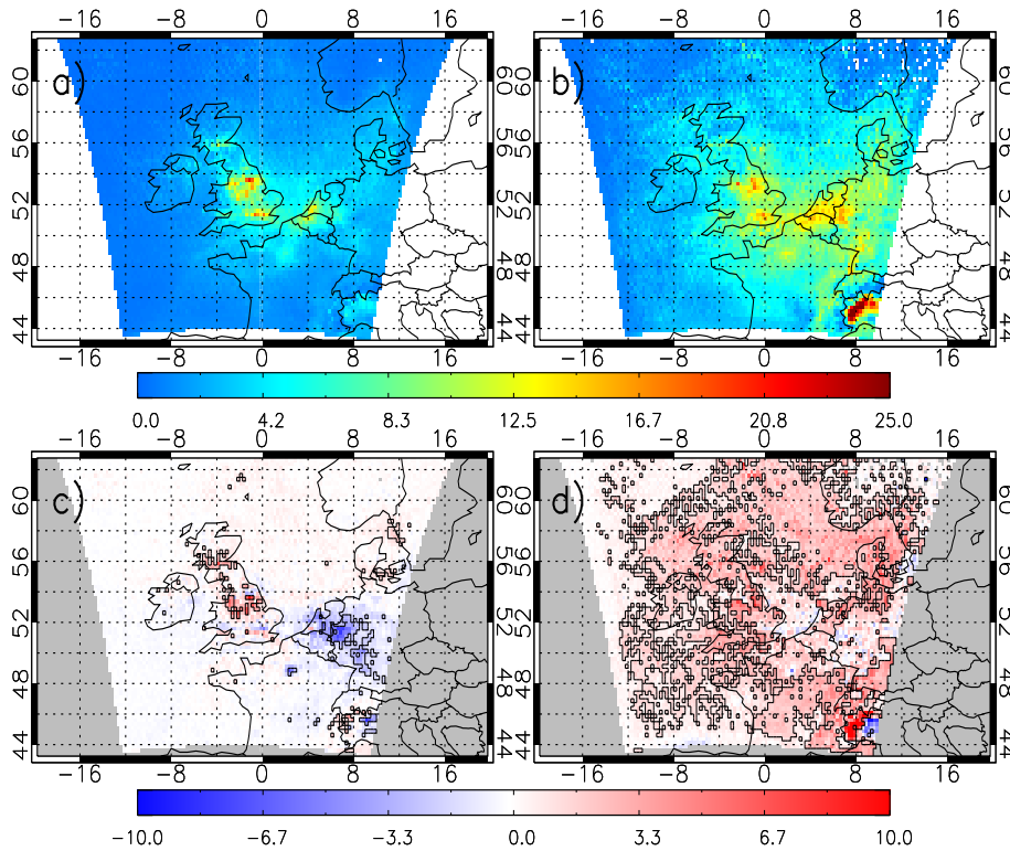
Figure 4.12: Tropospheric column NO 2 ( \times 10^{15} molecules/cm 2 ) for 2006 from AQUM Run MACC (AKs applied) for (a) summer and (b) winter. AQUM Run MACC (AKs applied) and OMI mean bias for (c) summer (RMSE= 3.74 \times 10^{15} molecules/cm 2 and FGE=0.63) and (d) winter (RMSE= 6.00 \times 10^{15} molecules/cm 2 and FGE=0.65).
