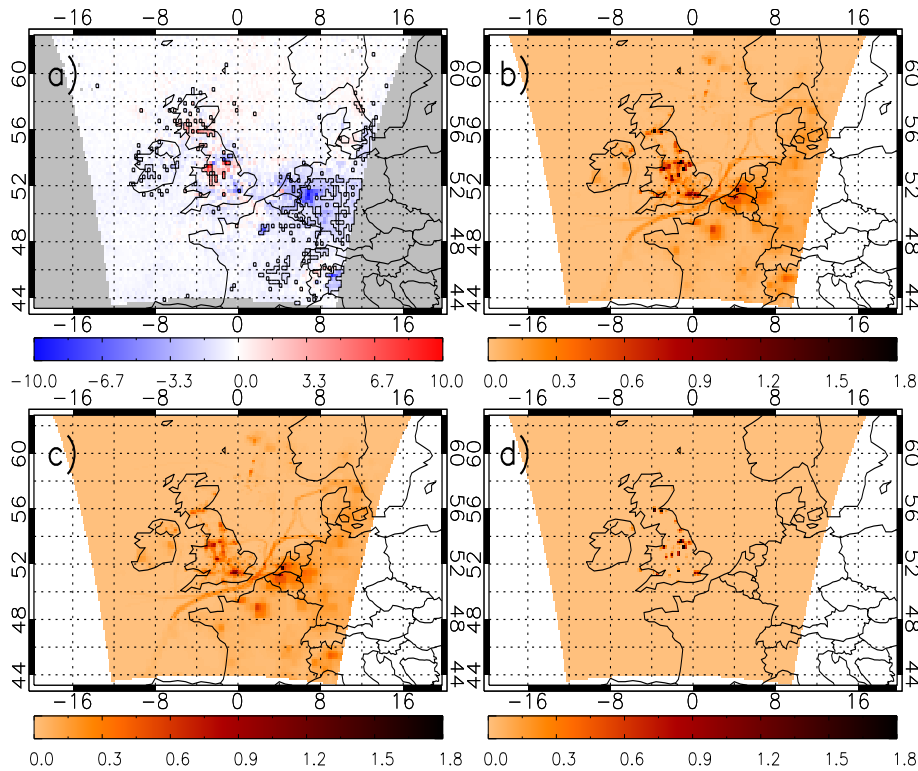
Figure 4.18: a) AQUM Run C (AKs applied) - OMI tropospheric NO 2 column ( \times 10^{15} molecules/cm 2 ) JJA 2006 mean bias. These are the control MBs to compare to the point source sensitivity experiments (RMSE = 3.64 \times 10^{15} molecules/cm 2 and FGE = 0.66). NO x emissions ( \times 10^{-9} kg/m 2 /s), JJA 2006, used in AQUM for (b) Run C and (c) Run E1. Panel (d) shows the difference between panels (b) and (c).
