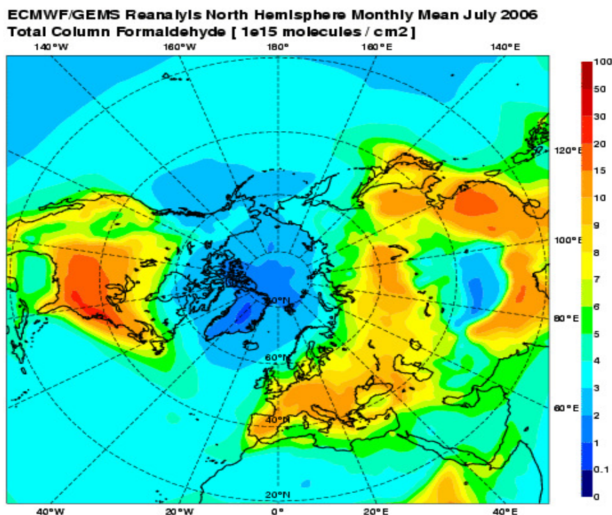
Figure 3.6: GEMS July 2006 northern hemispheric total column HCHO ( 10^{15} molecules/cm 2 ).
