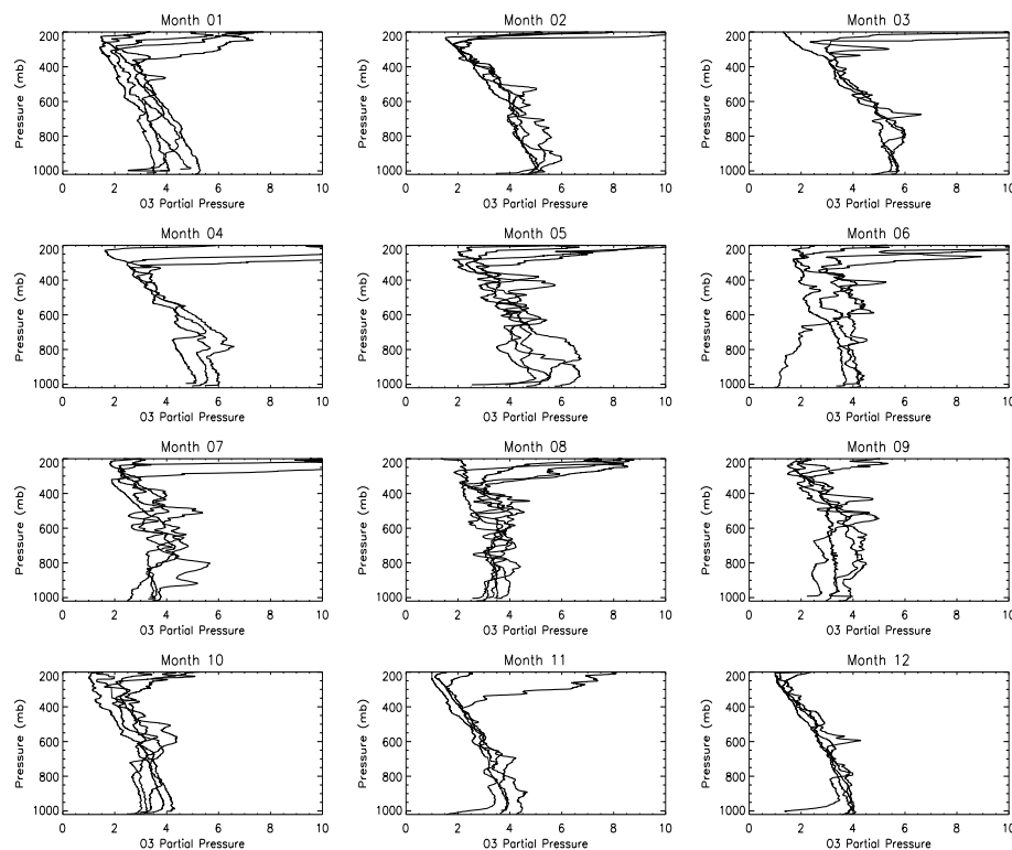
Figure 3.19: Ozonesonde profiles (partial pressure - Pa) for 2008 from the Valentia Observatory, Ireland.
