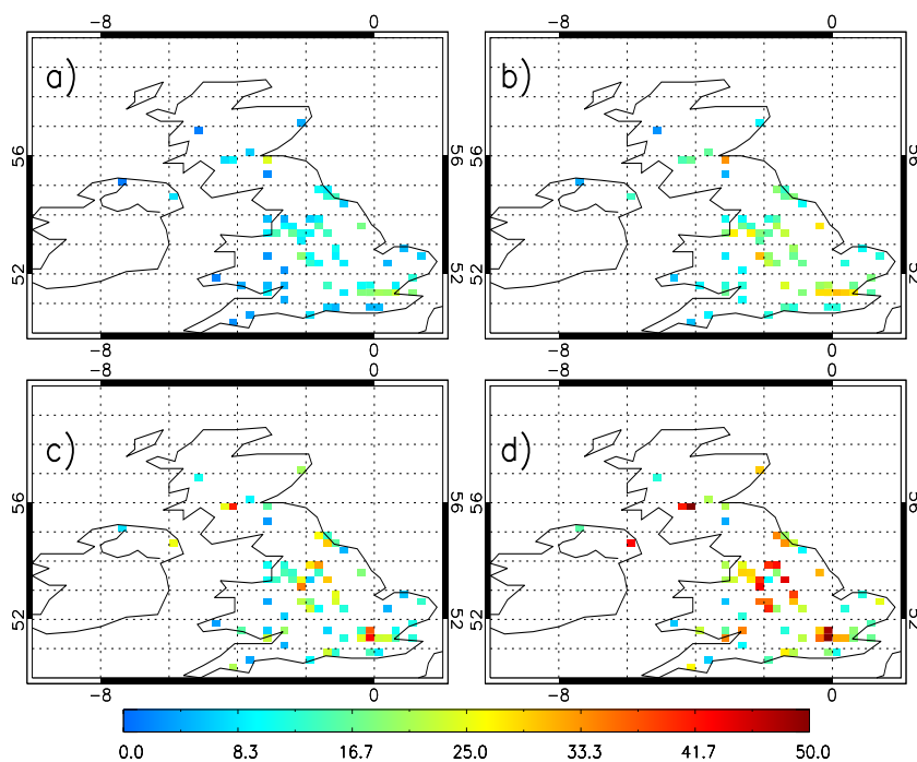
Figure 4.14: Surface NO 2 ( \mu\text{g}/\text{m}^3 ) for 2006 of (a) AQUM Run MACC summer, (b) AQUM Run MACC winter, (c) AURN summer and (d) AURN winter.
