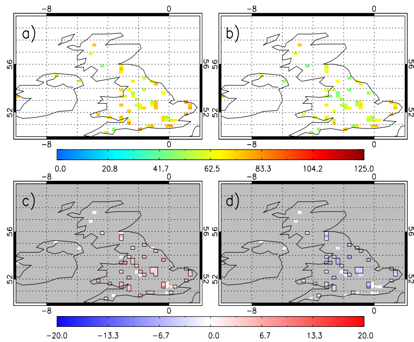
Figure 5.14: Composites of summer AURN surface \text{O}_3 ( \mu\text{g}/\text{m}^3 ), 2000-2010, for (a) anti-cyclonic conditions, (b) cyclonic conditions, (c) anticyclonic anomalies and (d) cyclonic anomalies.
