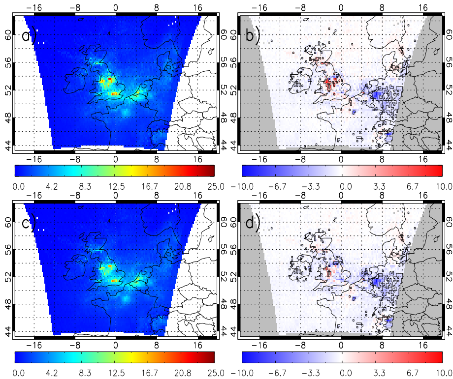
Figure 4.20: Tropospheric column NO 2 ( \times 10^5 molecules/cm 2 ) for JJA 2006 of (a) AQUM Run E3 and (c) AQUM Run E4. AQUM - OMI MB for (b) Run E3 (RMSE= 3.51 \times 10^5 molecules/cm 2 and FGE=0.66) and (d) Run E4 (RMSE= 3.15 \times 10^5 molecules/cm 2 and FGE=0.66).
