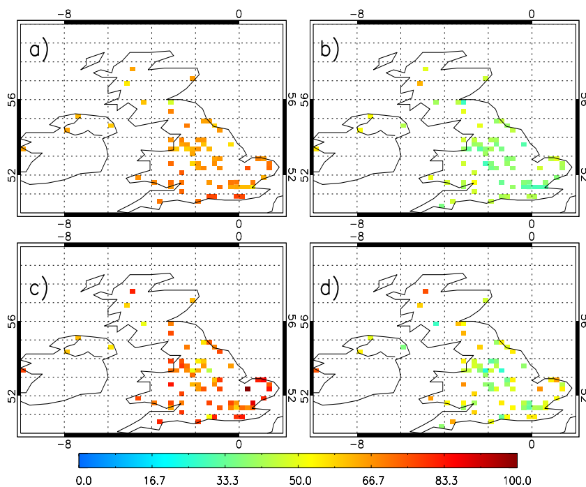
Figure 4.10: Surface O 3 ( \mu\text{g}/\text{m}^3 ) for 2006 of (a) AQUM Run C summer, (b) AQUM Run C winter, (c) AURN summer and (d) AURN winter.
