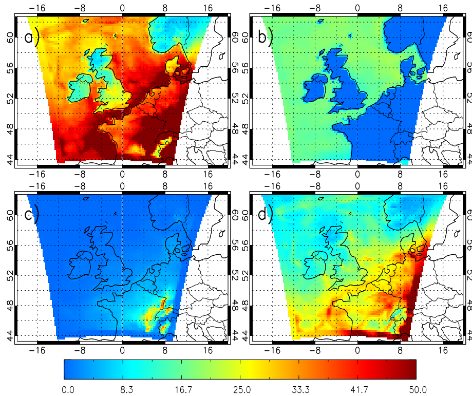
Figure 4.3: AQUM aerosol surface area ( \times 10^{-7} \text{ cm}^2/\text{cm}^3 ) for JFM 2006 of a) total aerosol, b) sea salt, c) ammonium nitrate and d) ammonium sulphate.
