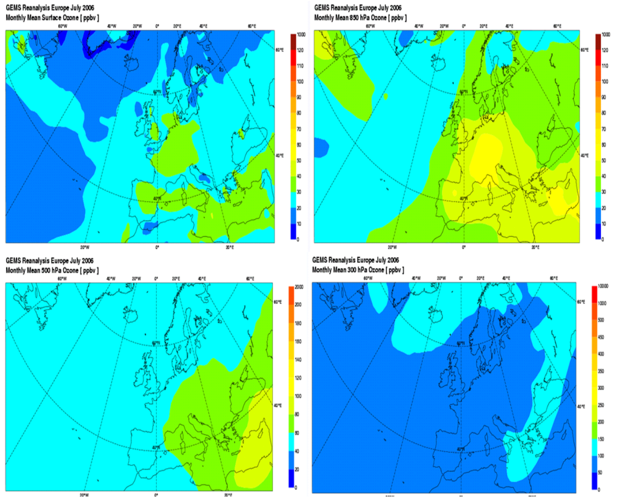
Figure 3.14: GEMS reanalysis O_3 (ppbv) for July 2006 at the surface (top left), 850 hPa (top right), 500 hPa (bottom left) and 300 hPa (bottom right).
