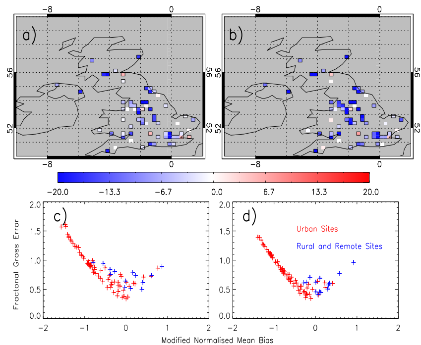
Figure 4.9: Surface NO 2 ( \mu\text{g}/\text{m}^3 ) AQUM Run C - AURN mean bias for 2006 of (a) summer and (b) winter. AQUM - AURN MNMB and FGE for (c) summer and (d) winter.
