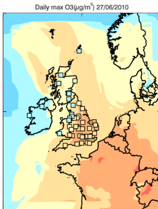
Figure 3.2: AQUM domain showing maximum modelled hourly ozone concentrations ( \mu\text{g}/\text{m}^3 ) for 27 th June 2010, with observed concentrations over-plotted within squares (taken from Savage et al. (2013)).
