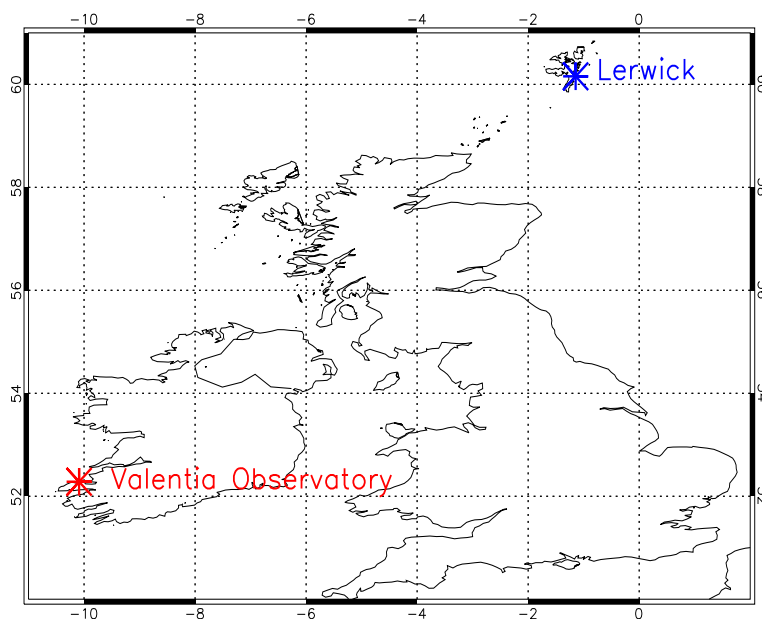
Figure 3.17: Ozonesonde release sites for 2008; Lerwick, Shetlands and the Valentia Observatory, Ireland.
