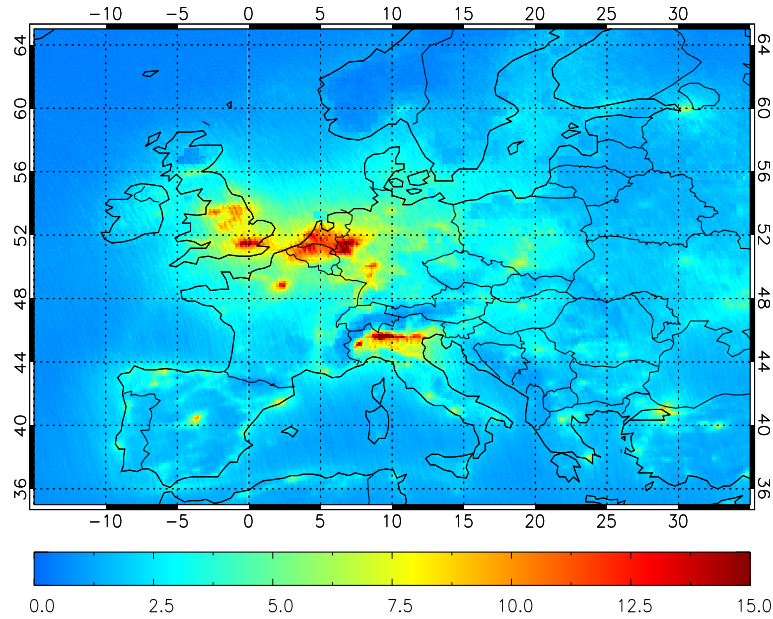
Figure 1.2: European tropospheric column NO 2 measured from space ( \times 10^{15} molecules/cm 2 , 2005-2013 average).
