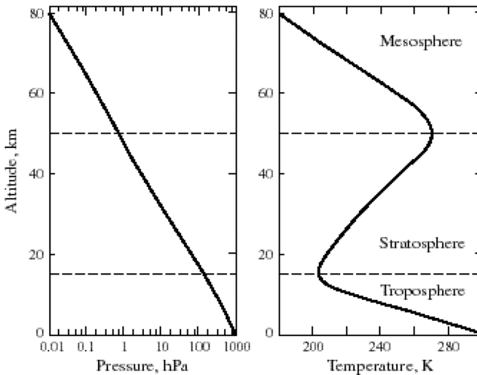
Figure 2.1: Typical pressure (left panel) and temperature (right panel) vertical profiles in the atmosphere at 30^\circ N for March. From from Jacob (1999).
