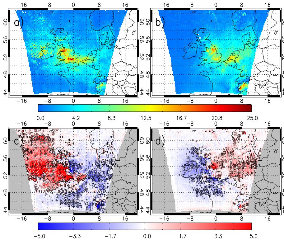
Figure 6.6: Composites of AQUM column NO 2 ( 10^{15} molecules/cm 2 ) under different wind flow directions and the differences of these with respect to the 5-year average. (a) South-easterly flow, (b) south-westerly flow, (c) south-easterly difference and (d) south-westerly difference.
