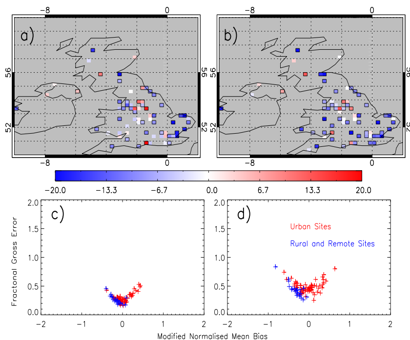
Figure 4.11: Surface O 3 ( \mu\text{g}/\text{m}^3 ) AQUM Run C - AURN mean bias for 2006 of (a) summer and (b) winter. AQUM - AURN MNMB and FGE for (c) summer and (d) winter.
