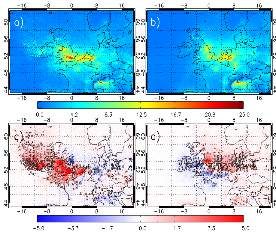
Figure 5.5: Composites of OMI column NO 2 ( \times 10^{15} molecules/cm 2 ) under different wind flow directions and difference of these with respect to 7-year average. (a) South-easterly flow, (b) south-westerly flow, (c) south-easterly anomalies and (d) south-westerly anomalies.
