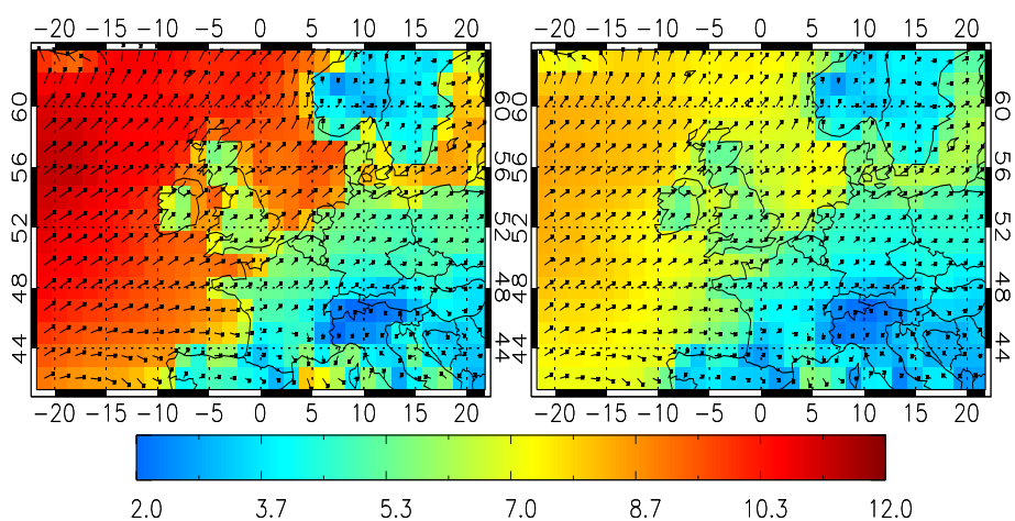
Figure 6.11: ECMWF ERA-Interim 12:00 UT 2006-2010 mean wind speeds (m/s) and directions for (left) winter and (right) summer.
