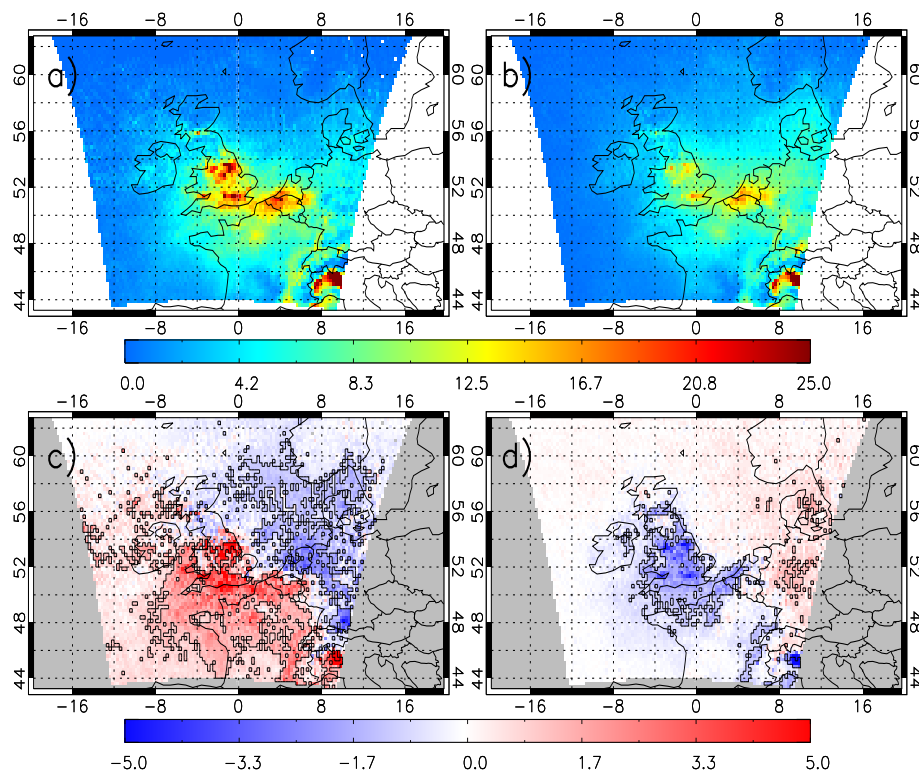
Figure 5.20: Composites of AQUM column tracer ( \times 10^{15} molecules/cm 2 ) between 2006-2010 for (a) PWC 5 (Drizzle) conditions, (b) PWC 8 (Showers) conditions, (c) PWC 5 (Drizzle) anomalies and (d) PWC 8 (Showers) anomalies.
