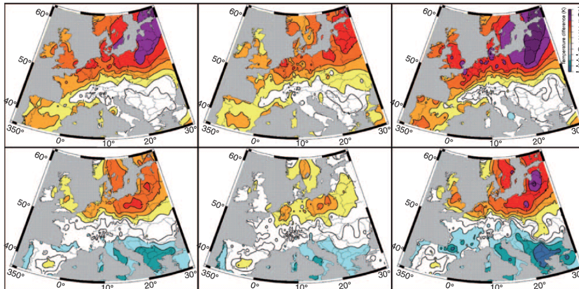
Figure 3.1: Differences between July 2006 and June 2003 (top)/August 2003 (bottom) average (left), minimum (middle) and maximum (right) surface air temperature (K) (Rebetez et al., 2009).
