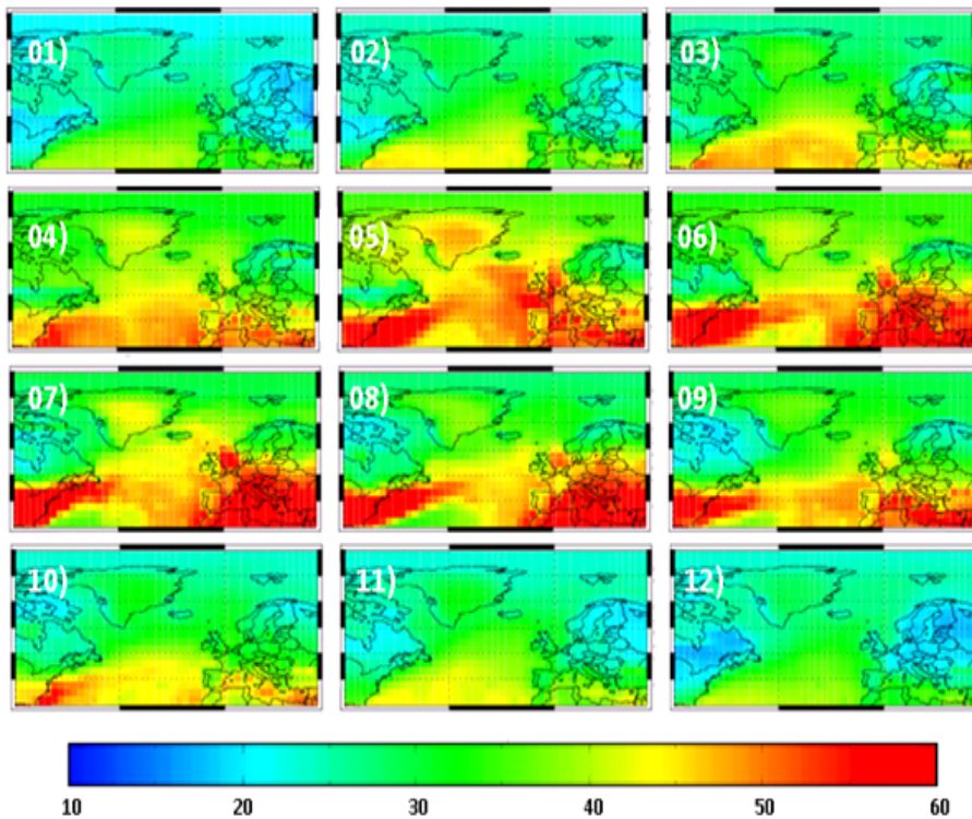
Figure 3.20: TOMCAT 2008 surface Atlantic O 3 (ppbv).
