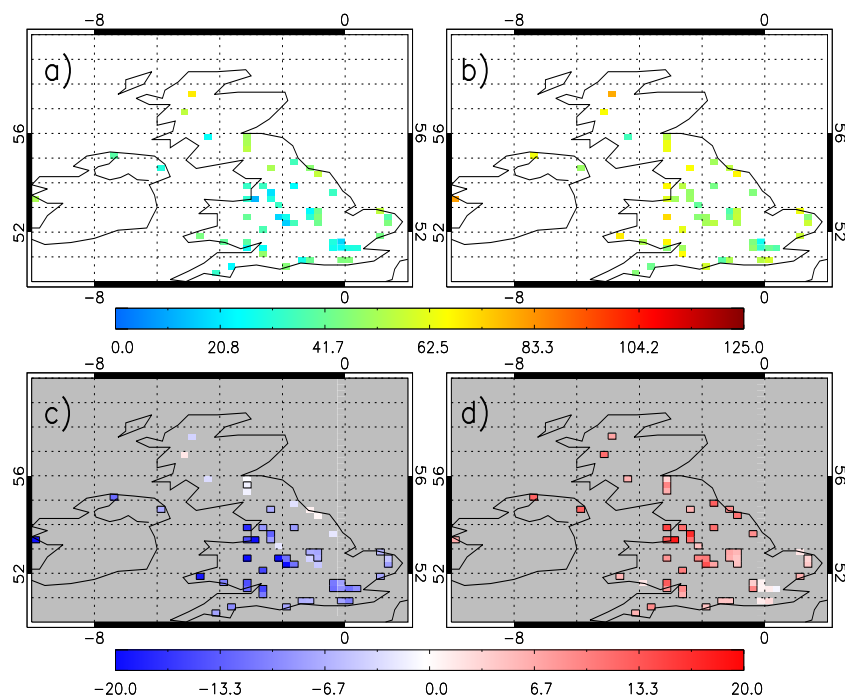
Figure 5.17: Composites of winter AURN surface \text{O}_3 ( \mu\text{g}/\text{m}^3 ), 2000-2010, for (a) south-easterly flow, (b) north-westerly flow, (c) south-easterly anomalies and (d) north-westerly anomalies.
