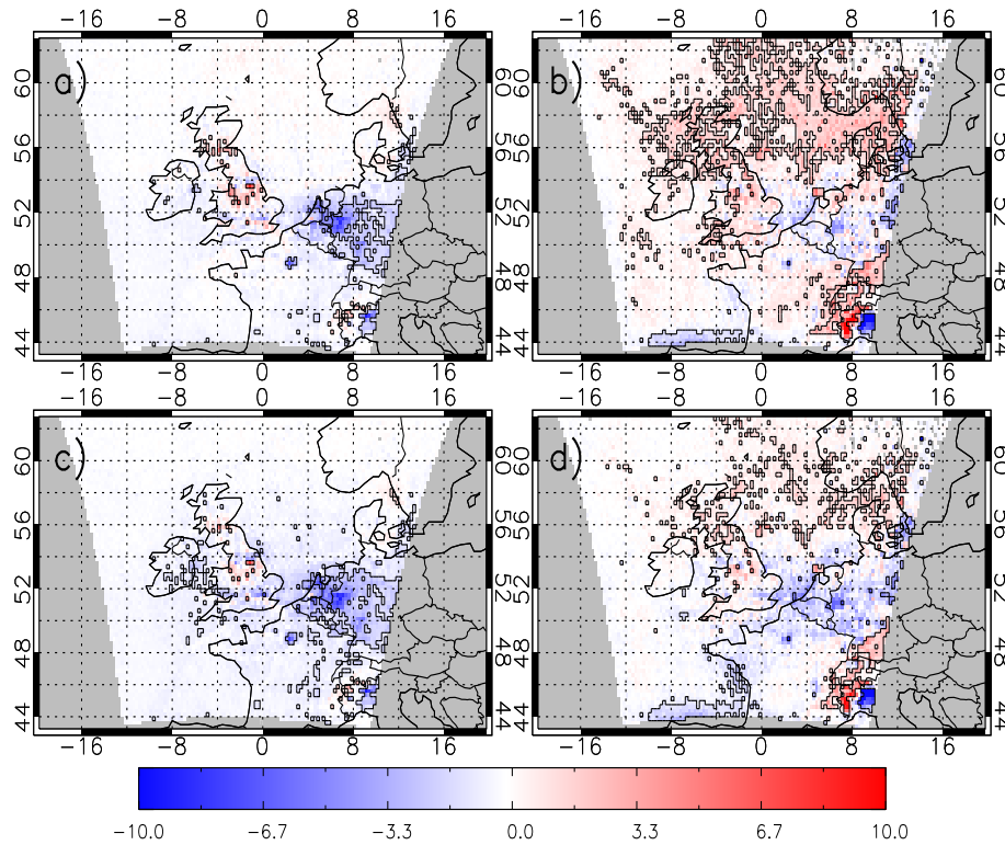
Figure 4.22: MB in tropospheric NO 2 column ( \times 10^{15} molecules/cm 2 ) for 2006 between AQUM (AKs applied) - OMI for (a) summer \gamma=0.001 (RMSE= 3.39 \times 10^{15} molecules/cm 2 and FGE=0.65), (b) winter \gamma=0.001 (RMSE= 5.05 \times 10^{15} molecules/cm 2 and FGE=0.62), (c) summer \gamma=0.02 (RMSE= 3.08 \times 10^{15} molecules/cm 2 and FGE=0.67) and (d) winter \gamma=0.02 (RMSE= 4.48 \times 10^{15} molecules/cm 2 and FGE=0.60).
