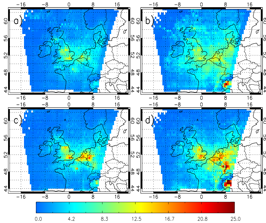
Figure 4.6: Tropospheric NO 2 column ( \times 10^{15} molecules/cm 2 ) for 2006 of (a) AQUM Run C (with AKs applied) summer, (b) AQUM Run C (with AKs applied) winter, (c) SCIAMACHY summer and (d) SCIAMACHY winter.
