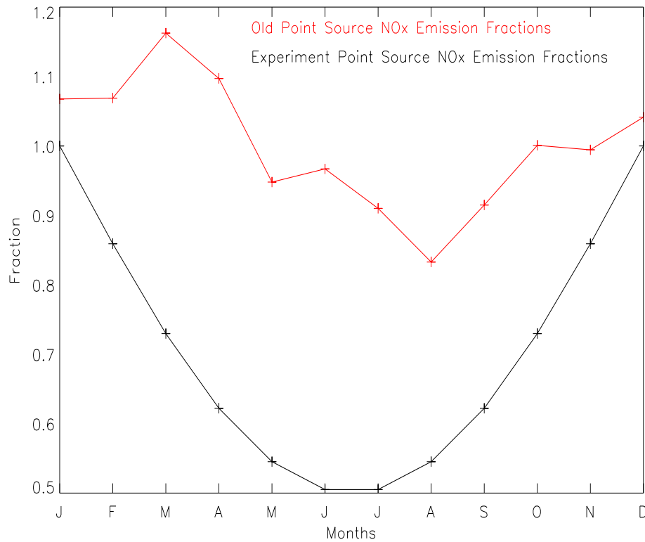
Figure 4.21: Seasonal cycles forced onto the NAEI NO x emissions; Red is the old seasonal cycle (SC) and black is the experiment based on SC = 1 - 0.5 \sin(\pi(m_0 \dots m_{11}) / (n-1)) , where n = \text{number of months} = 12 and m = 0, 1 \dots n-1 .
