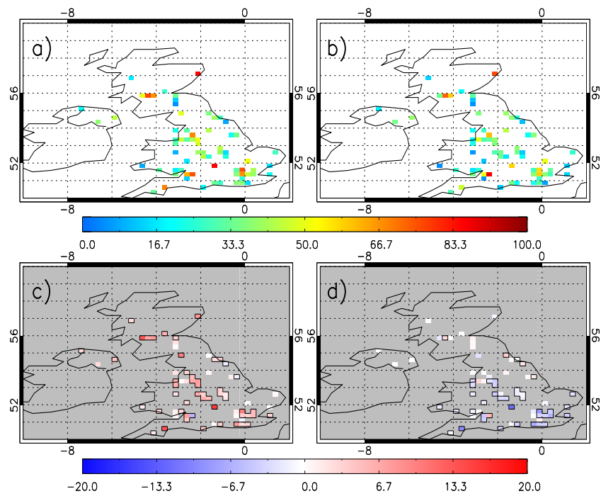
Figure 5.11: Composites of winter AURN surface NO 2 ( \mu\text{g}/\text{m}^3 ), 2000-2010, for (a) anticyclonic conditions, (b) cyclonic conditions, (c) anticyclonic anomalies and (d) cyclonic anomalies.
