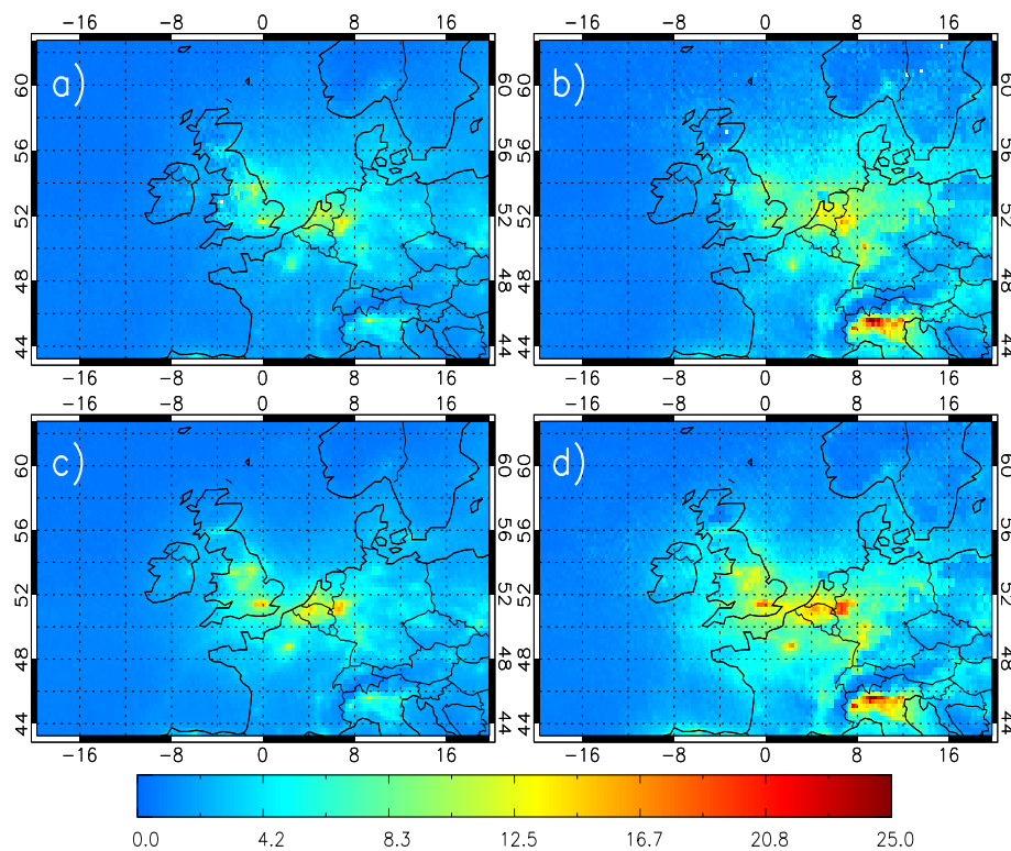
Figure 5.2: Composites of OMI column NO 2 ( \times 10^{15} molecules/cm 2 ) for (a) summer cyclonic, (b) winter cyclonic, (c) summer anticyclonic and (d) winter anticyclonic conditions.
