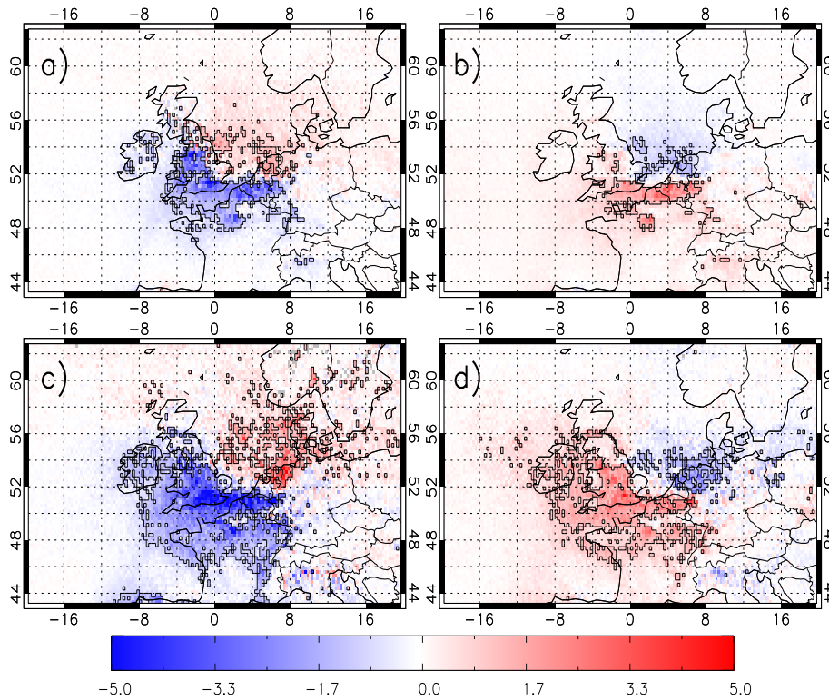
Figure 6.2: Anomalies of OMI column NO 2 composites compared to the seasonal 5-year average ( 10^{15} molecules/cm 2 ) for (a) summer cyclonic, (b) summer anticyclonic, (c) winter cyclonic and (d) winter anticyclonic conditions. Black boxes indicate where the anomalies are statistically significant at the 95% level.
