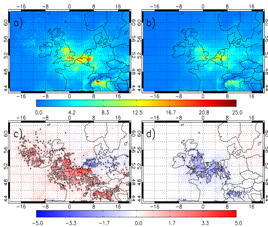
Figure 5.18: Composites of OMI column NO 2 ( \times 10^{15} molecules/cm 2 ) between 2006-2010 for (a) PWC 5 (Drizzle) conditions, (b) PWC 8 (Showers) conditions, (c) PWC 5 (Drizzle) anomalies and (d) PWC 8 (Showers) anomalies. Black boxes indicate where the anomalies are statistically significant at the 95% level.
