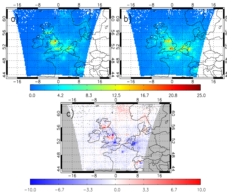
Figure 3.4: July 2006 tropospheric column \text{NO}_2 ( 10^{15} molecules/cm 2 ): a) AQUM, b) OMI and c) mean bias. White pixels in a) and b) and grey pixels in c) indicate no satellite data.
