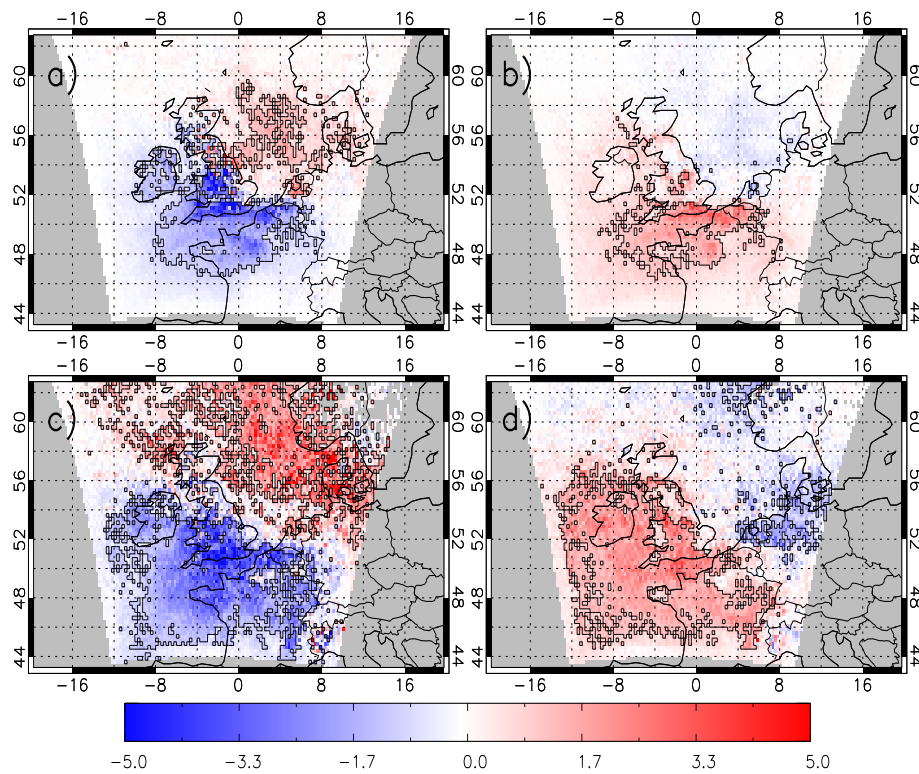
Figure 6.5: Anomalies of AQUM column NO 2 composites compared to the seasonal 5-year average ( 10^{15} molecules/cm 2 ) for (a) summer cyclonic, (b) summer anticyclonic, (c) winter cyclonic and (d) winter anticyclonic conditions.
