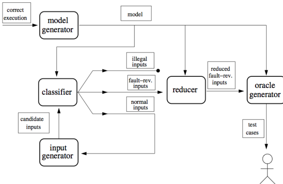
Figure 2.12: The input selection technique. Implicit in the diagram is the program under test. Rectangles with rounded corners represent steps in the technique, and rectangles with square corners represent artifacts [3]
