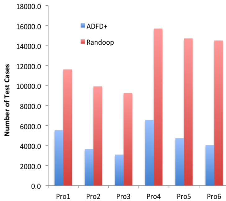
Figure 6.3: Number of test cases taken to find failure domains
