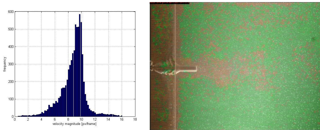
Figure 4-9 – Histogram of velocity ( l ) and vector plot ( r ) with n=1 standard deviation filter applied and removed vectors interpolated.
