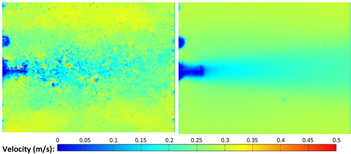
Figure 6-23 – 16mm diameter support structure, far upstream turbine.
