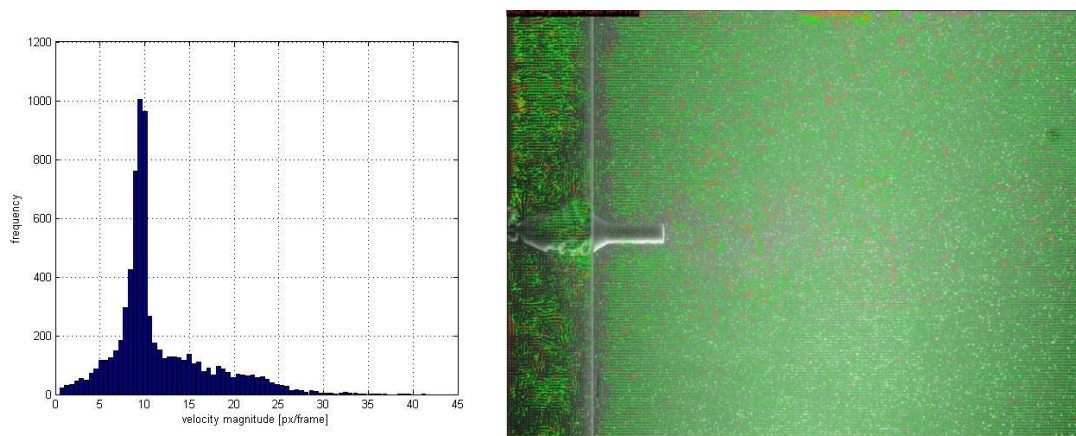
Figure 4-11 – Histogram of velocity ( l ) and vector plot ( r ) with n=7 standard deviation filter applied and removed vectors interpolated.
