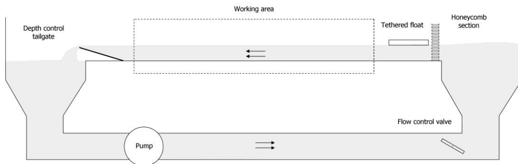
Figure 3-2 – Water channel layout schematic.
