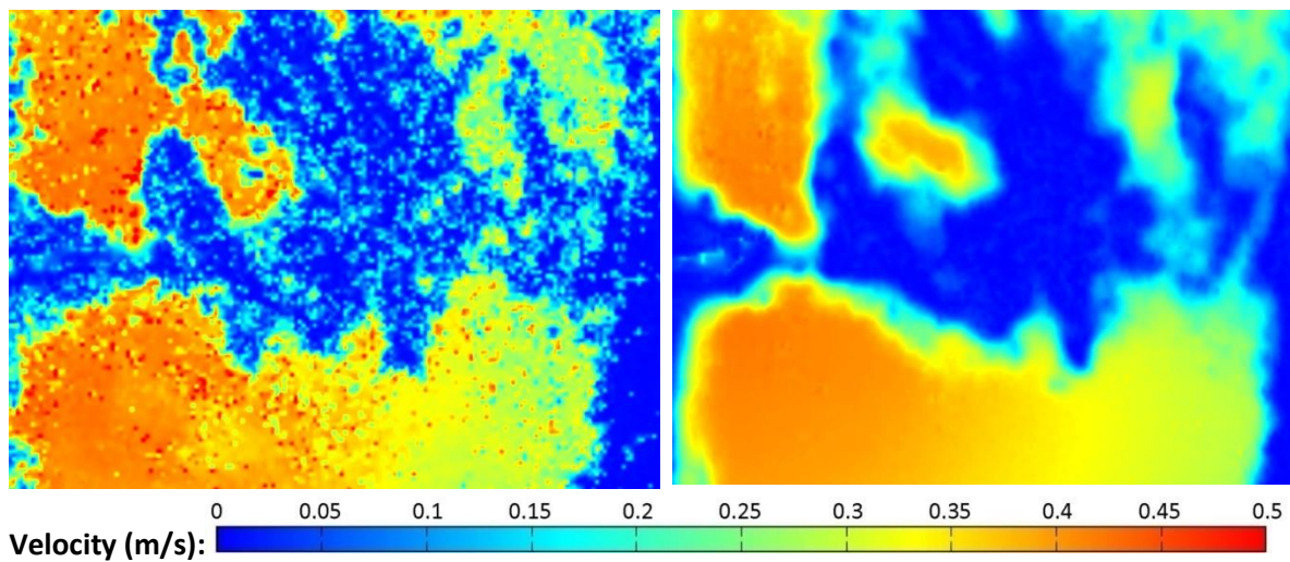
Figure 6-30 – 11mm diameter support structure, near upstream turbine.
