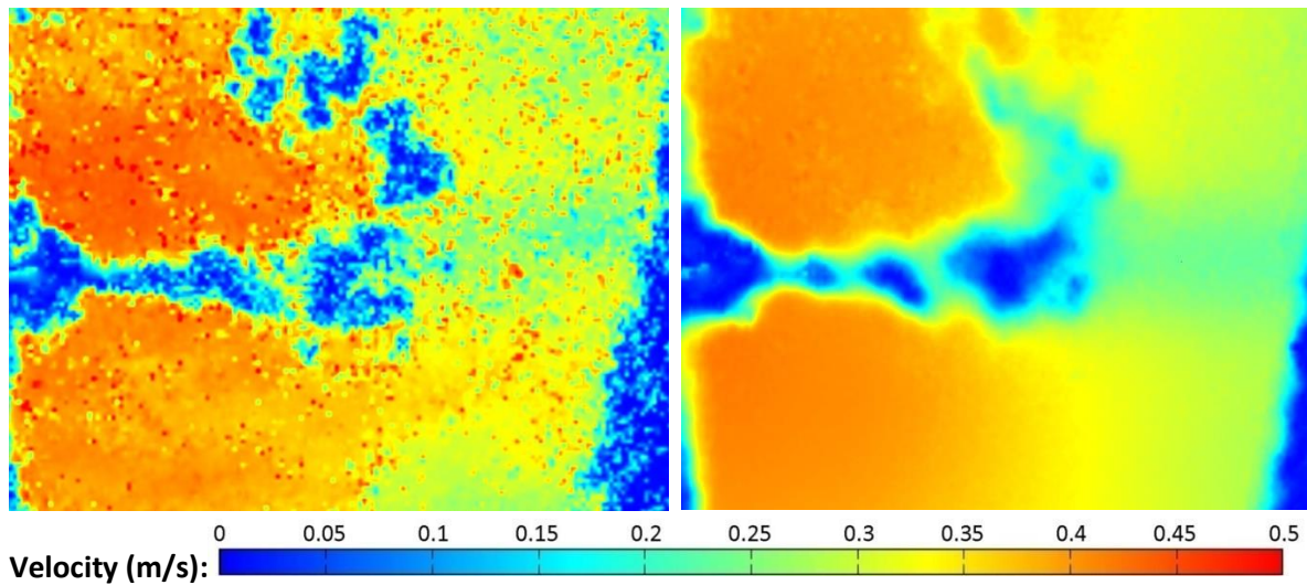
Figure 6-29 – 11mm diameter support structure, far upstream turbine.
