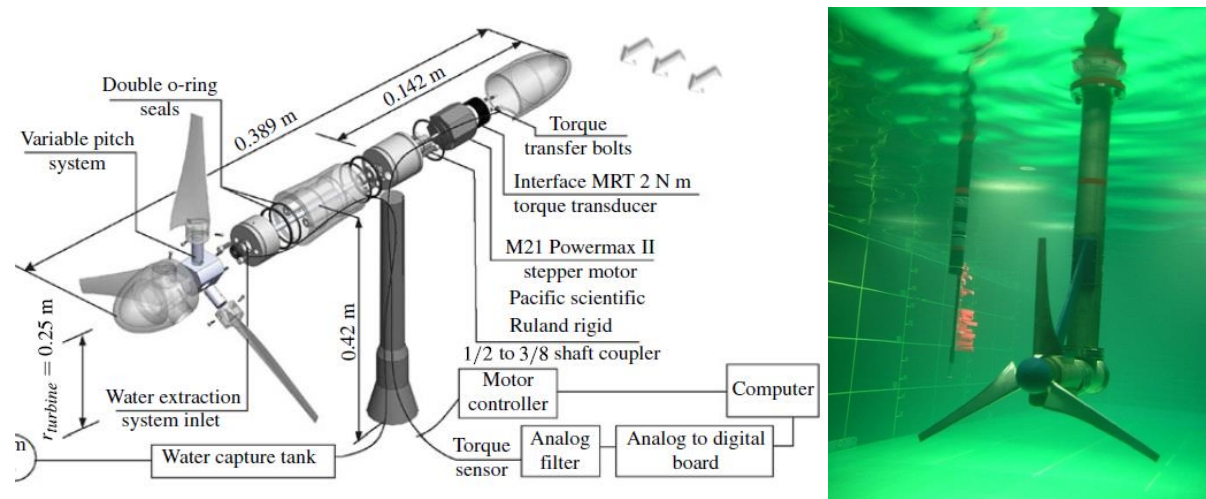
Figure 2-40 – Active turbine models (from [140] (l) and [52] (r)).
