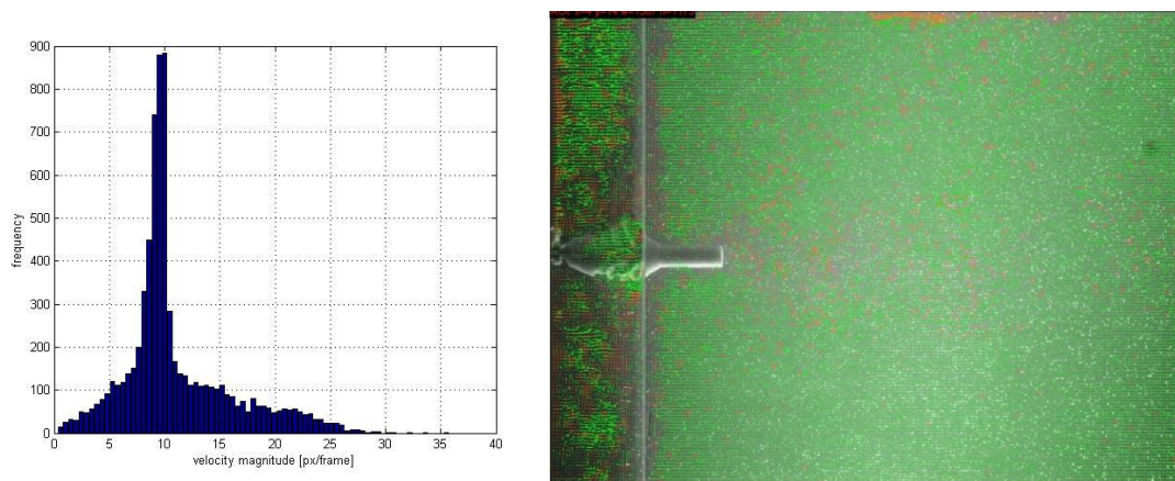
Figure 4-10 – Histogram of velocity ( l ) and vector plot ( r ) with n=3 standard deviation filter applied and removed vectors interpolated.
