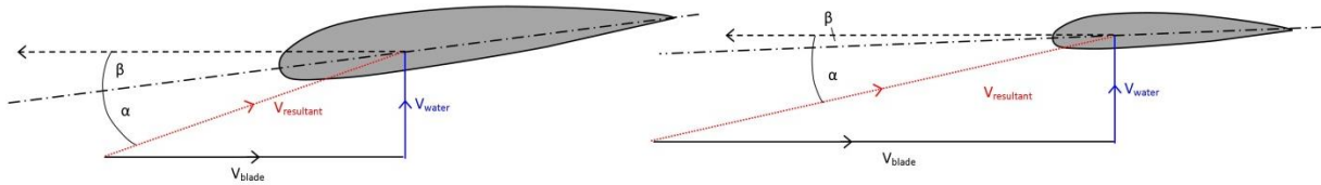
Figure 2-22 – Blade twist to give constant \alpha : Root (l) and tip (r).
