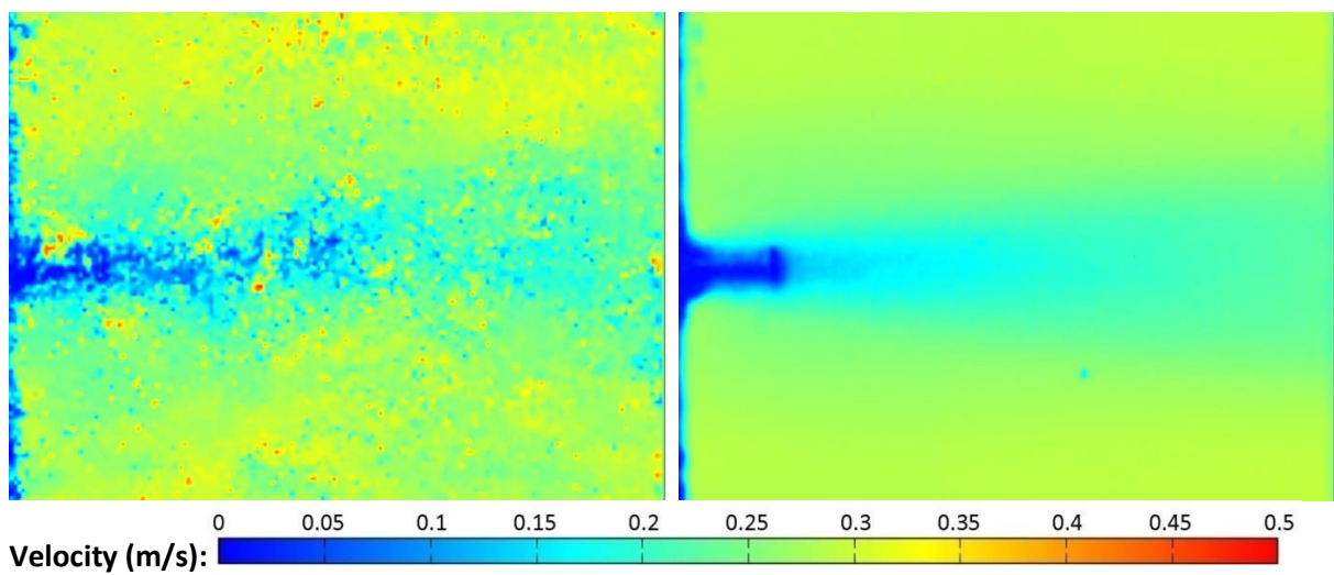
Figure 6-24 – 16mm diameter support structure, near upstream turbine.
