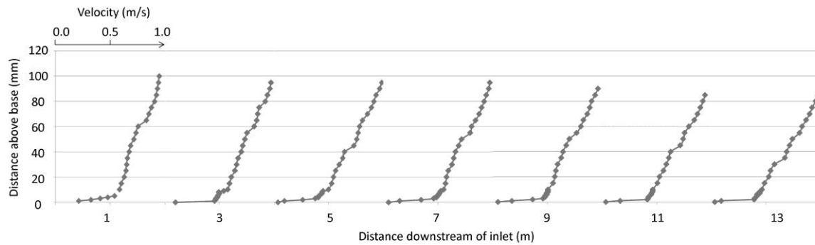
Figure 3-4 – Centreline velocity profiles as recorded during characterisation
