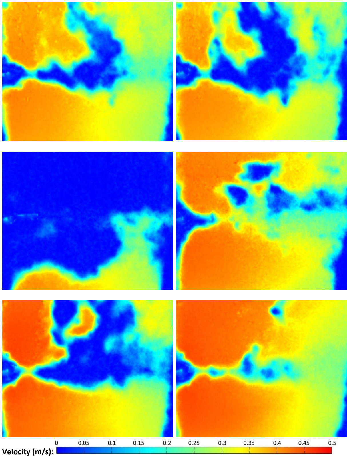
Figure 6-44 – Far ( 10D ) upstream turbine, offset 0.5D (l) & 1D (r). Downstream turbine support structure diameter 11mm (top), 16mm (middle), 20mm (bottom).
