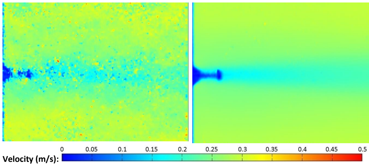
Figure 6-20 – 11mm diameter support structure, far upstream turbine.
