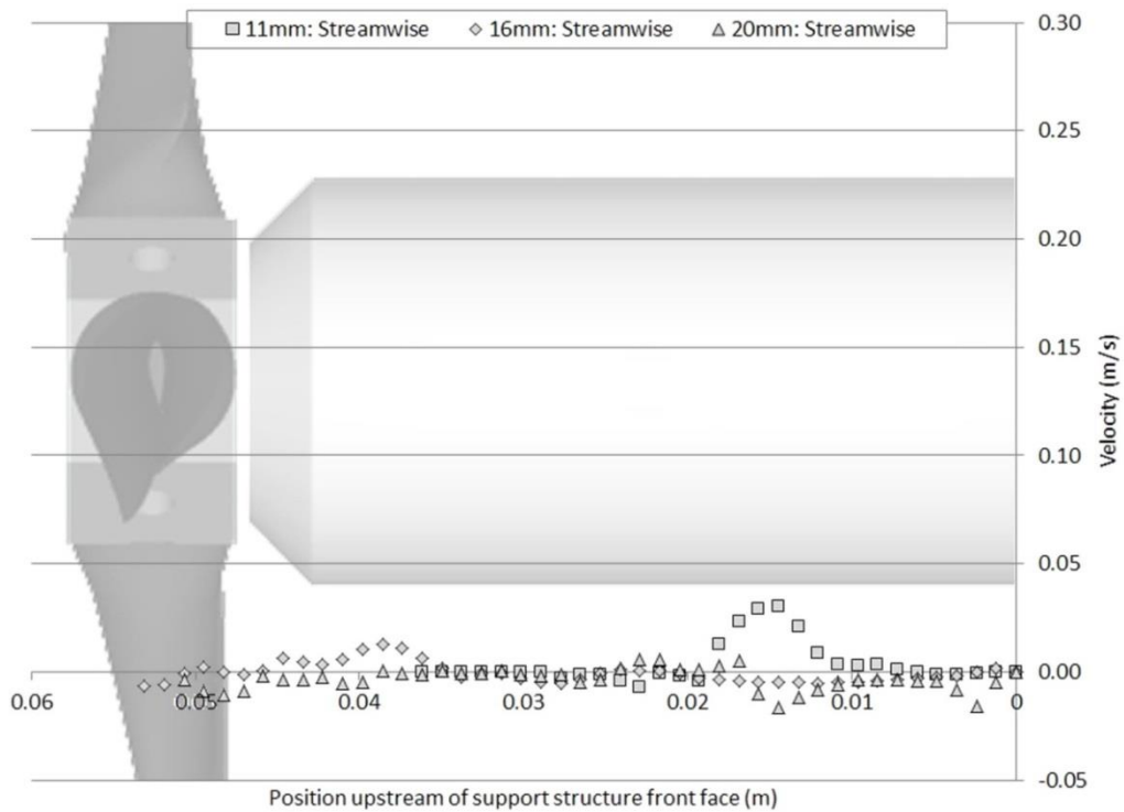
Figure 5-37 – Time-averaged streamwise velocity in upstream region of 11mm, 16mm and 20mm diameter support structure located in back position at 66mm above channel base (flow from left to right).
