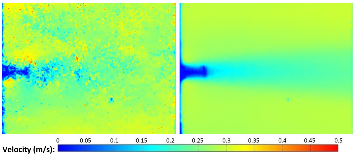
Figure 6-22 – 16mm diameter support structure, no upstream turbine.
