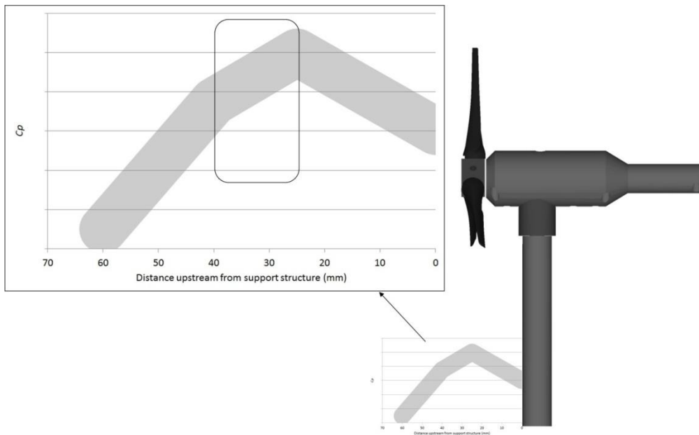
Figure 5-64 – Diagram illustrating the location of the suggested optimal performance region and surrounding regions.
