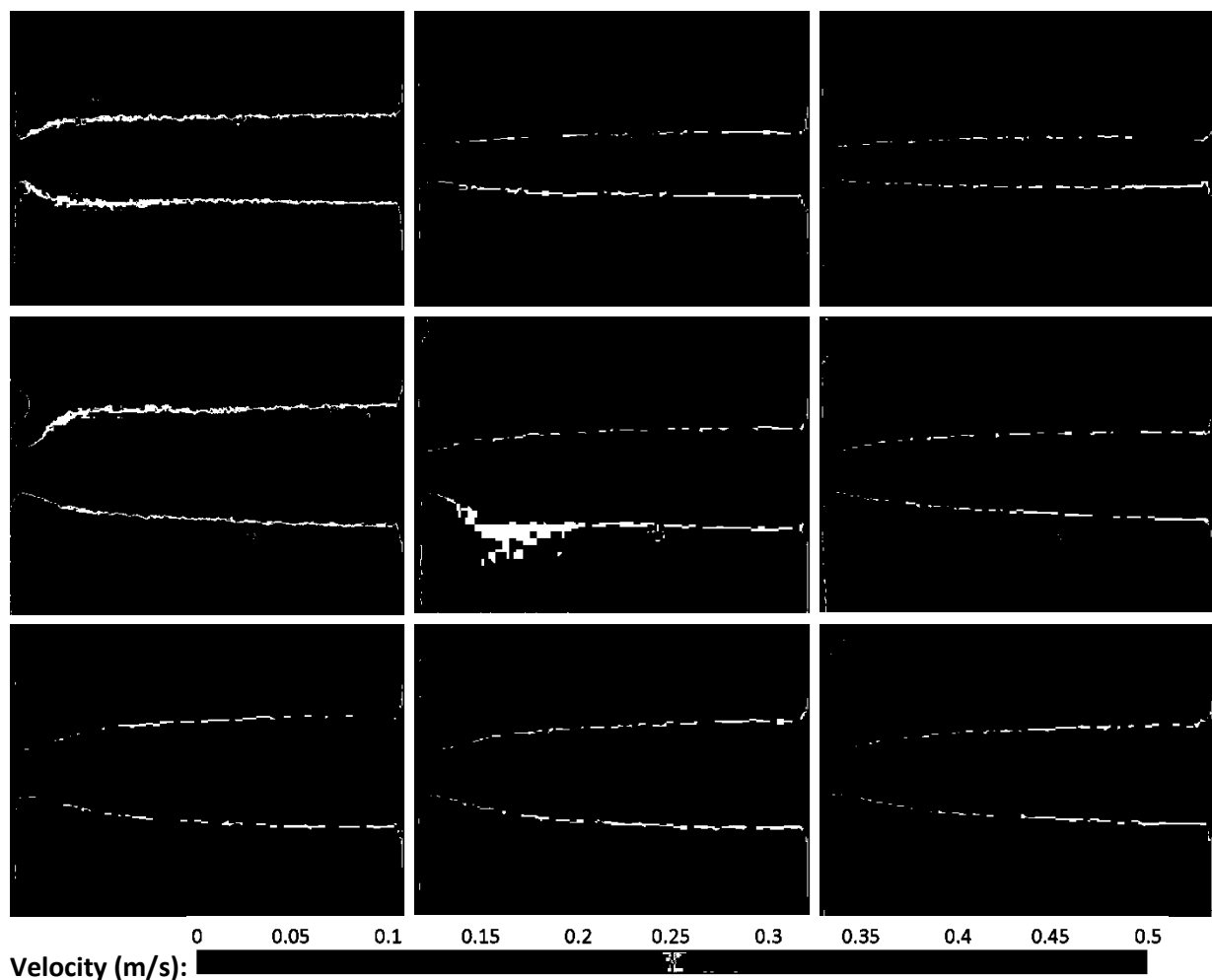
Figure 6-42 – Far ( 10D ) upstream turbine, offset 0D (l), 0.5D (m) & 1D (r). Downstream turbine support structure diameter 11\text{mm} (top), 16\text{mm} (middle), 20\text{mm} (bottom).
