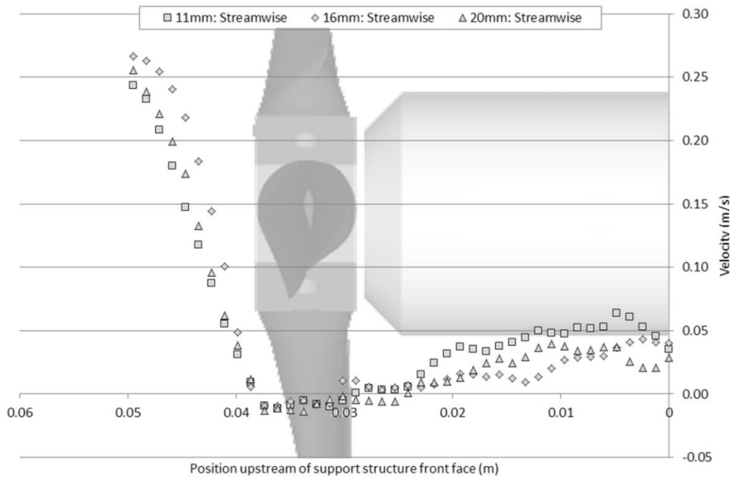
Figure 5-36 – Time-averaged streamwise velocity in upstream region of 11mm, 16mm and 20mm diameter support structure located in centre position at 66mm above channel base (flow from left to right).
