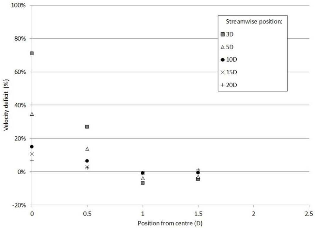
Figure 5-13 – Cross-stream position vs. velocity deficit at 3, 5, 10, 15 and 20D downstream (Porosity = 39%, C_T = 0.80 ).
