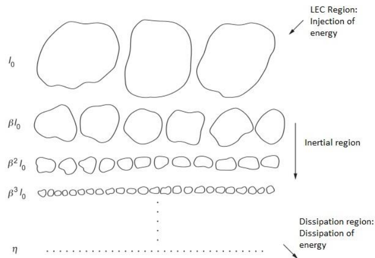
Figure 2-3 – Energy cascade as described by Kolmogorov [49].
