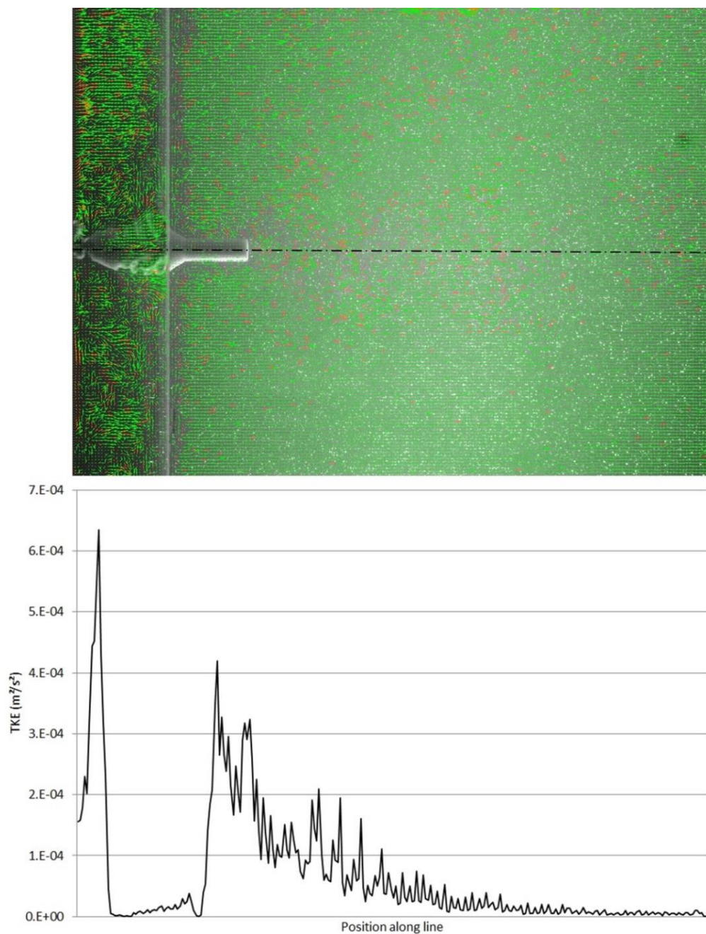
Figure 4-13 – Sample horizontal plane TKE plot at support structure mid height (flow case 2).
