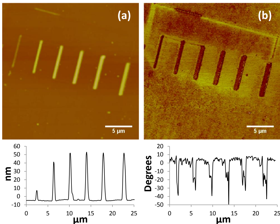
Figure 3.22: AFM tapping mode images and corresponding line-sections showing, (a) height and (b) phase contrasts of a set of 6 lines of polyOEGMA brush grown from lines drawn by SNP into an NPPOC-silane film with an increasing number of traces, each offset by 100 nm, from 1, 2, 3, 4, 5 and 6 lines (going from left to right).
