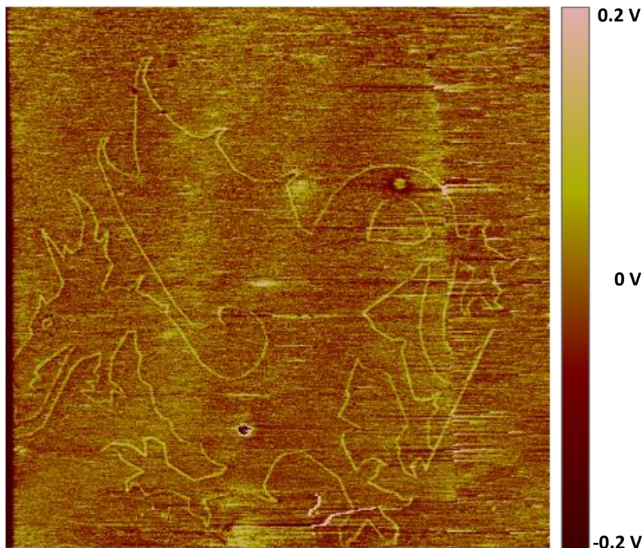
Figure 3.17: 60 \mu\text{m} x 60 \mu\text{m} FFM image of a dragon picture drawn by SNP into a NPPOC-silane film using 325 nm wavelengths at a scan speed of 100 \text{nm s}^{-1} . The line of deprotected NPPOC-silane was derivatised with adipoyl chloride to enhance the contrast difference.
