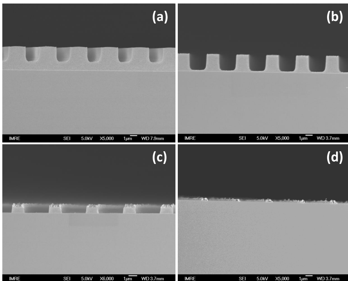
Figure 4.3: SEM cross-section images of a 2\ \mu\text{m} thick layer of PMMA imprinted with a 2\ \mu\text{m} grating mould after receiving an anisotropic etch with \text{O}_2 gas, for (a) 0 min, (b) 1 min, (c) 2 min and (d) 3 min.
