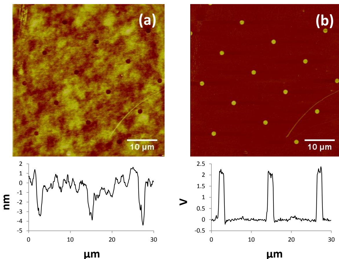
Figure 4.8: AFM (a) tapping mode height image and (b) contact mode subtracted (trace – retrace) friction image, measured from a surface patterned with 1.5 μm diameter dots of APTES surrounded by PEG-silane. Patterns were fabricated from a 1 μm thick layer of PMMA, imprinted by a 2 μm diameter hole mould. The corresponding line-sections are shown below each image.
