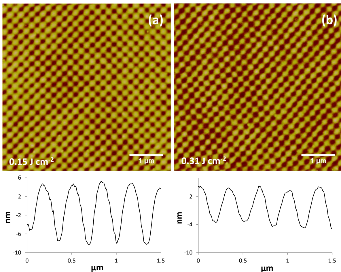
Figure 3.16: 5 \mu\text{m} \times 5 \mu\text{m} AFM height images and corresponding line-sections of an OEGMA brush grown from an initiated NPPOC-silane film patterned by a double exposure at 90^\circ , with doses of (a) 0.15 \text{ J cm}^{-2} and (b) 0.31 \text{ J cm}^{-2} .
