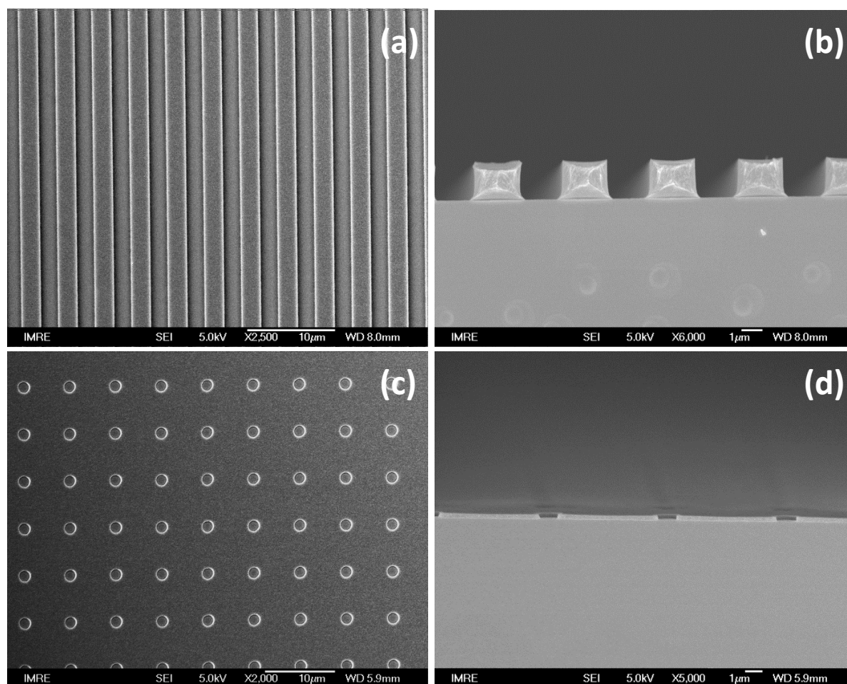
Figure 4.4: SEM images showing 2 different mould imprints. A 2 µm grating, imprinted into a 1 µm thick layer of PMMA, showing (a) the top view and (b) the cross-section. An array of holes 1 µm diameter, imprinted into a 0.5 µm thick layer of PMMA, showing (c) the top view and (d) the cross-section.
