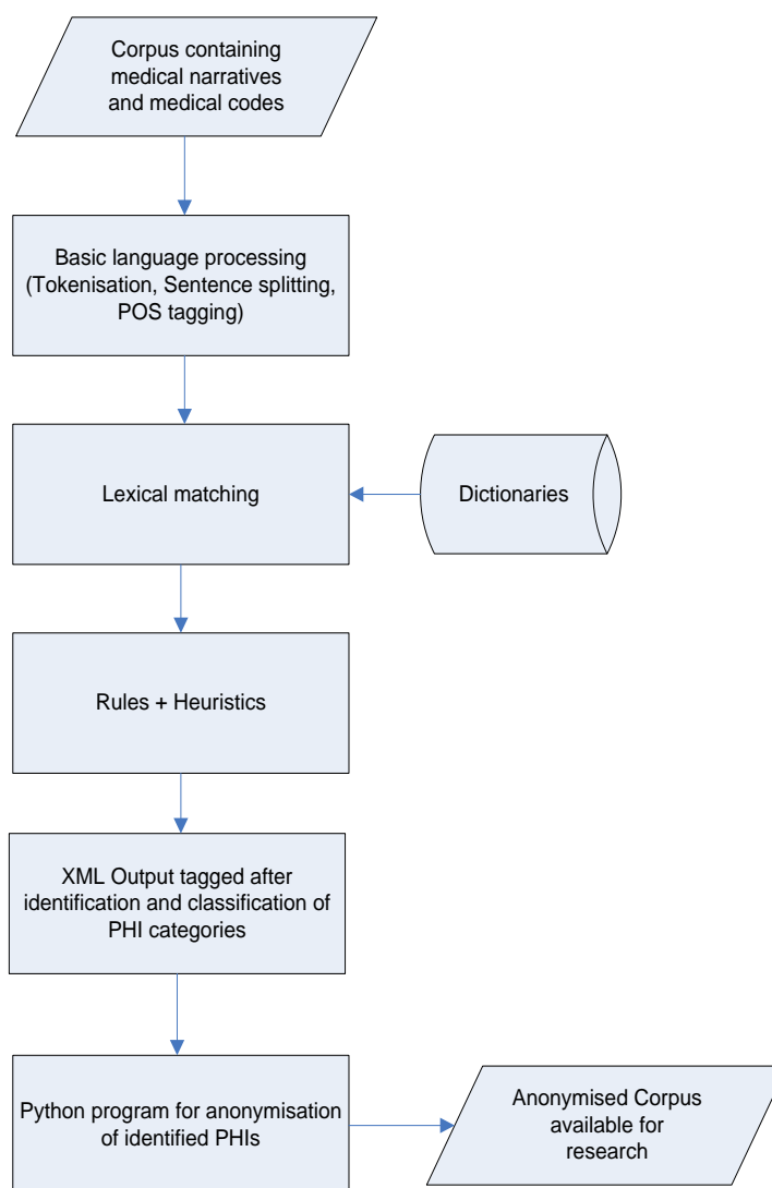
Figure 3-6: System flow of anonymization module.
