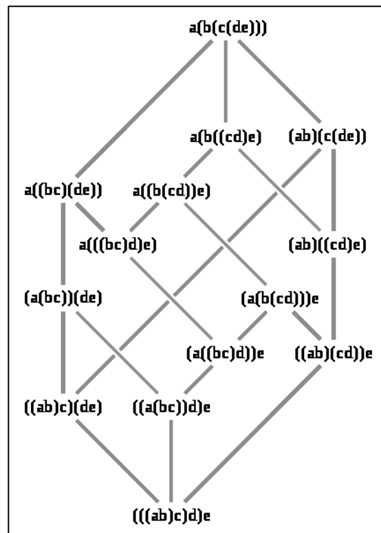
Figure 12.1: The different permutations of 4 predicates – diagram is called an associahedron and is credited to David Eppstein { WWW.ICS.UCL.EDU/~EPPSTEIN }.
