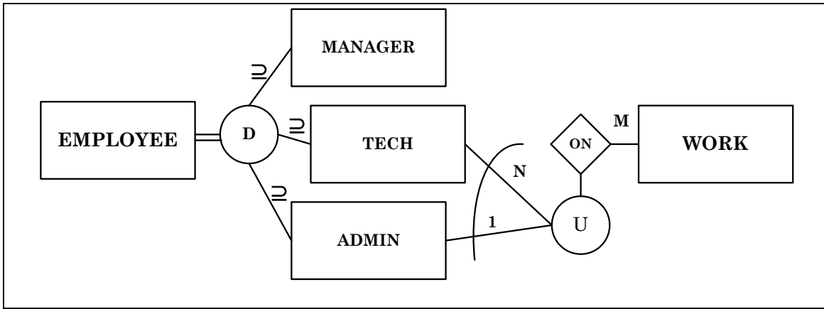
Fig. 2.6 – An EERM with a category (or EOR) artefact – i.e. arc.
