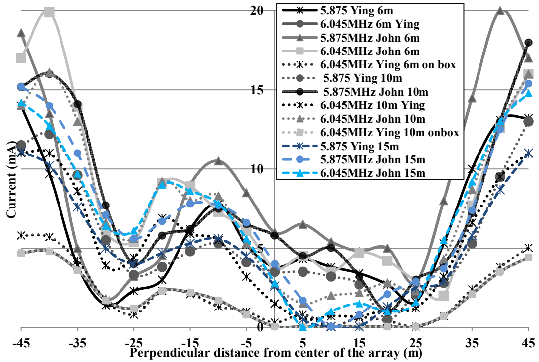
Measured ankle current
