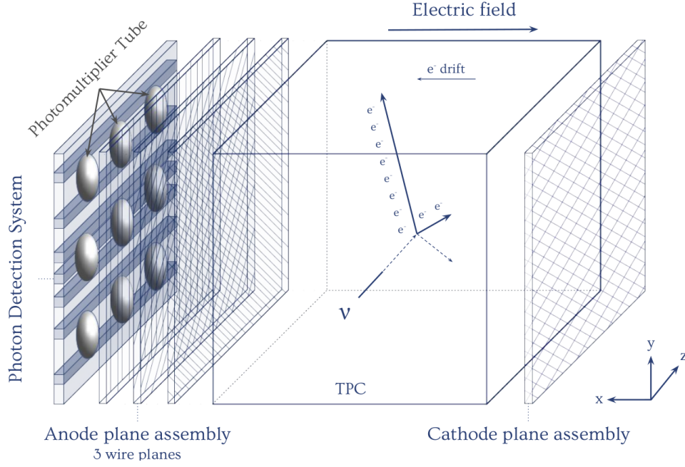
Fig. 3.1 Diagram illustrating the operating principles of a LArTPC [54].
