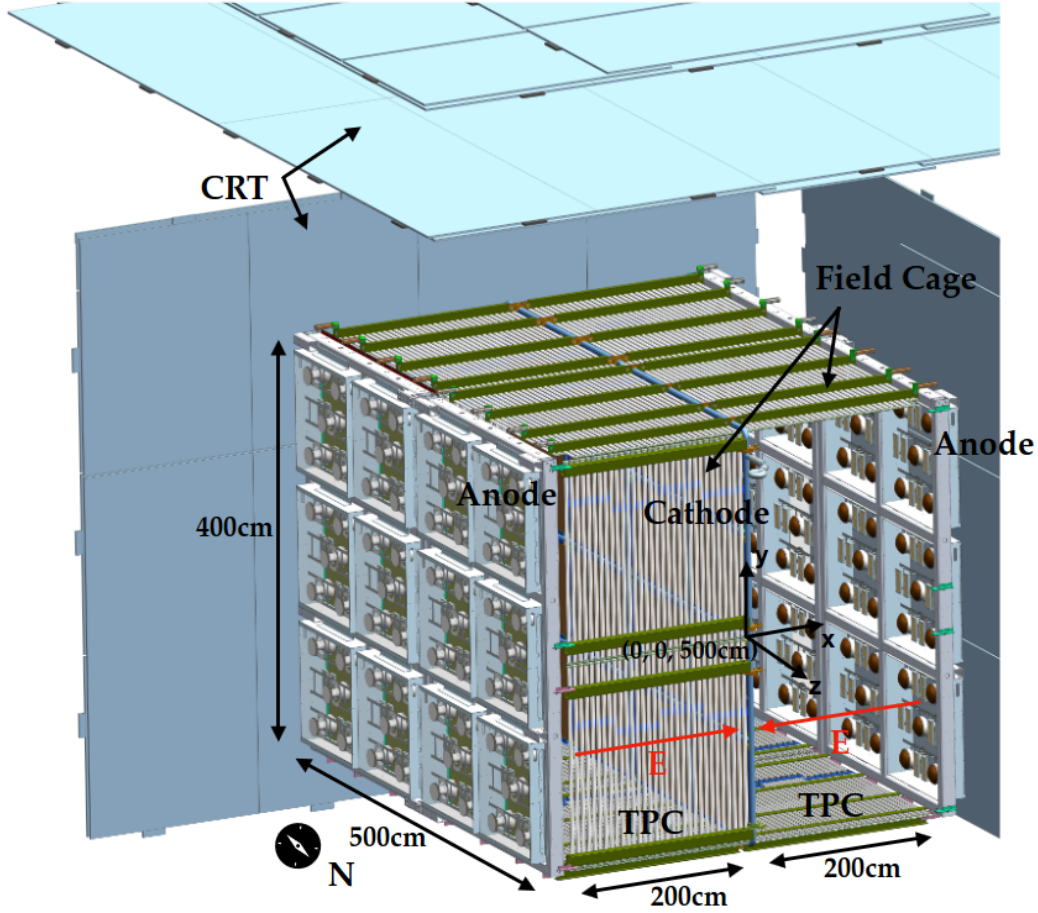
Fig. 4.2 3D model of the SBND detector, showing the LArTPC surrounded by 4 out of the 7 CRT walls [73].
