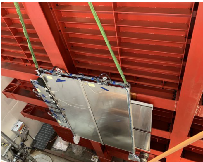
Fig. 7.3 Downstream panels of the CRT Sharps installed on the downstream wall of the SBND cryostat.
