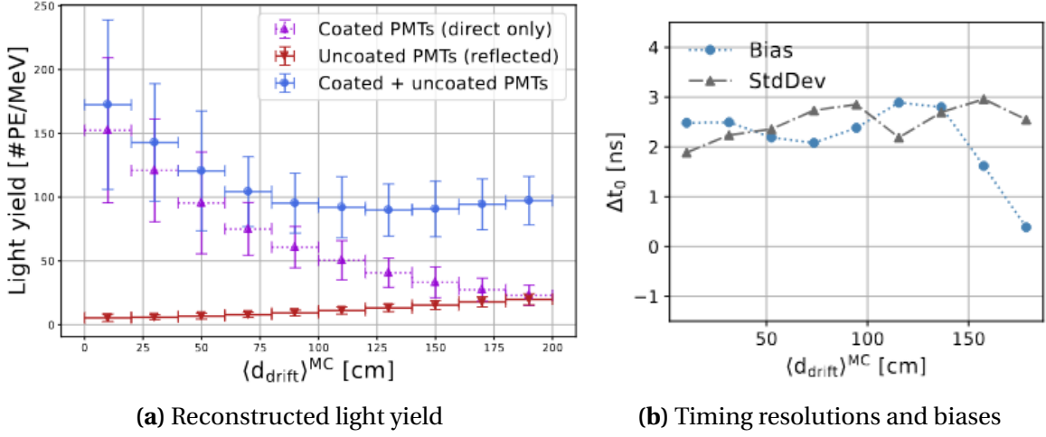
Fig. 6.8 (a) Reconstructed light yield and (b) timing biases and resolutions of reconstructed t_0 after propagation correction as a function of the mean drift distance based on simulation [73].
