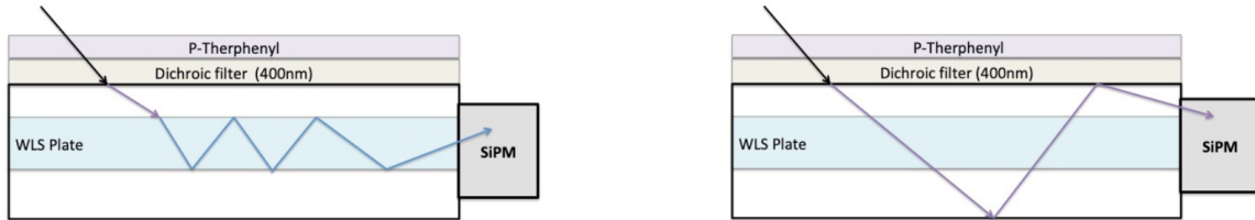
Fig. 3.11 Diagram illustrating the operating principles of a X-ARAPUCA [83].
