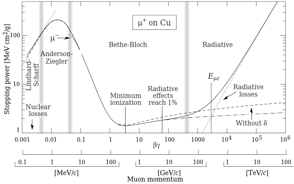
Fig. 3.2 Energy loss in matter for a muon traversing a copper medium [57].
