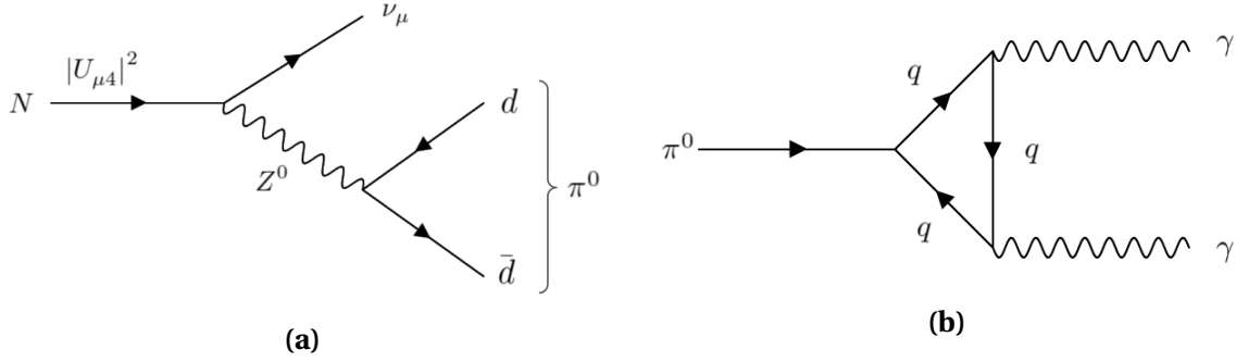
Fig. 2.4 Feynman diagrams of (a) N \rightarrow \nu\pi^0 and (b) \pi^0 \rightarrow \gamma\gamma .
