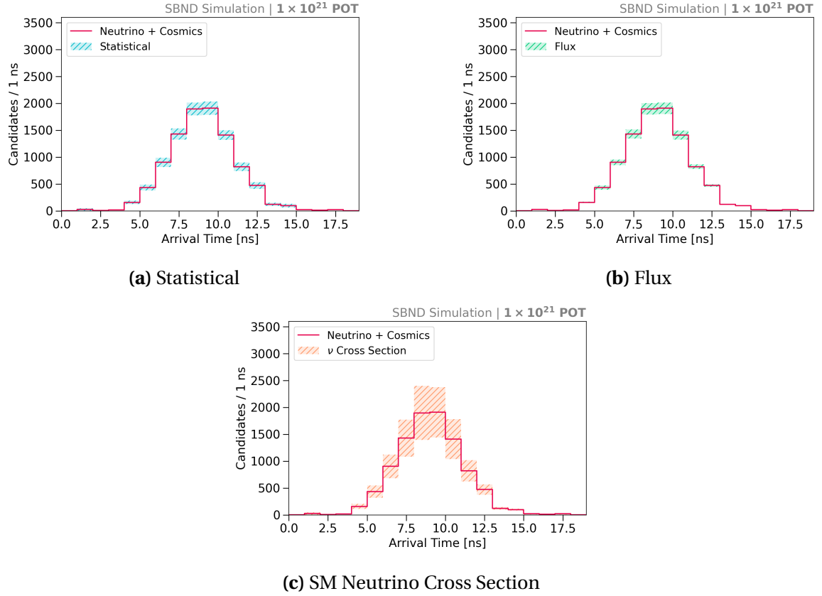
Fig. 10.3 Arrival time distributions of SM neutrino and cosmic backgrounds with (a) statistical, (b) flux and (c) SM neutrino cross section uncertainties, normalised to the exposure of 1 \times 10^{21} POT.
