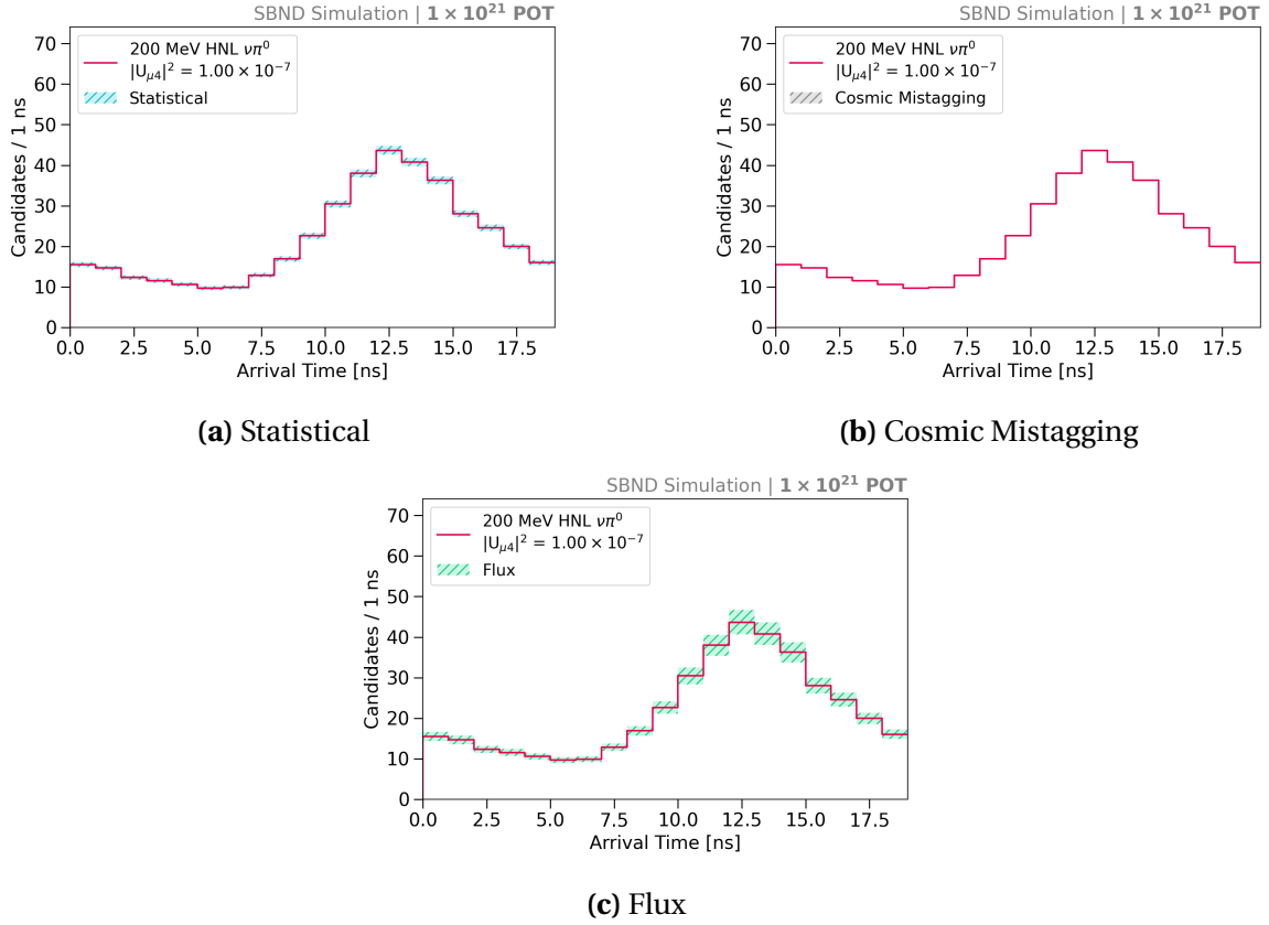
Fig. 10.1 Arrival time distributions of 200 MeV HNLs with (a) statistical, (b) cosmic mistagging and (c) flux uncertainties, normalised to the exposure of 1 \times 10^{21} POT and |U_{\mu 4}|^2 = 1 \times 10^{-7} .
