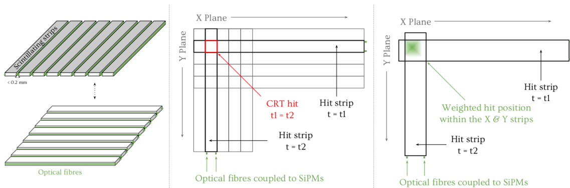
Fig. 4.6 Diagrams showing the operating principles of CRT strips (middle, right) and their perpendicular orientation (left) [54].
