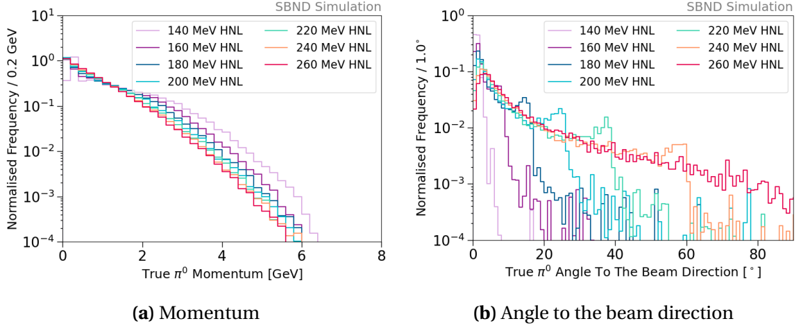
Fig. 5.4 Simulated kinematics distributions of \pi^0 from HNLs decaying inside SBND.
