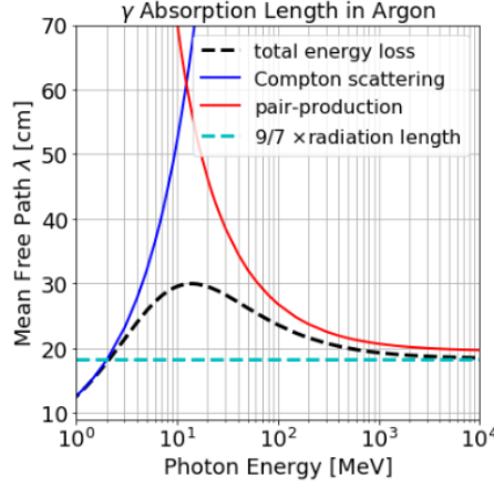
Fig. 3.3 Mean free path of photons traversing in liquid argon as a function of their energies [59].
