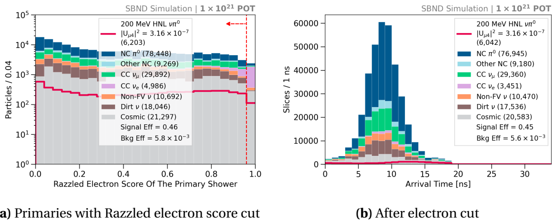
Fig. 9.10 Razzled electron score of the primary shower distribution with the cut (left) and the arrival time distribution after the cut (right).
