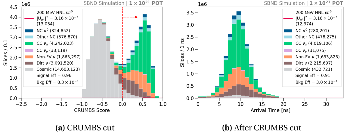
Fig. 9.5 CRUMBS score distribution with the cut (left) and the arrival time distribution after the cut (right).
