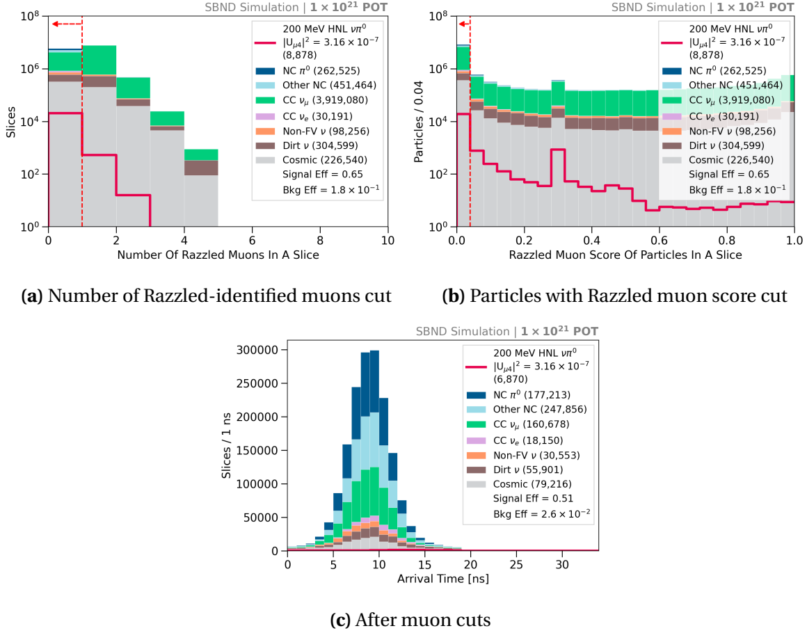
Fig. 9.8 Number of Razzled muons in a slice and Razzled muon score distributions with the cuts (top) and the arrival time distribution after the cuts (bottom).
