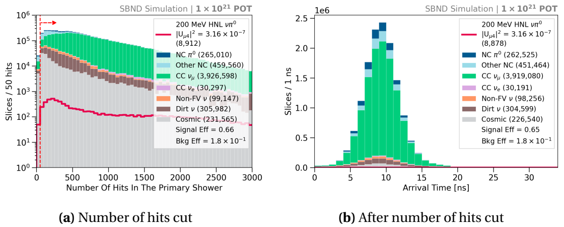
Fig. 9.7 Number of hits in the primary particle distribution with the cut (left) and the arrival time distribution after the cut (right).
