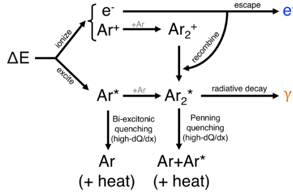
Fig. 3.5 Production of ionisation electrons and scintillation photons from energy deposition processes in liquid argon [61].
