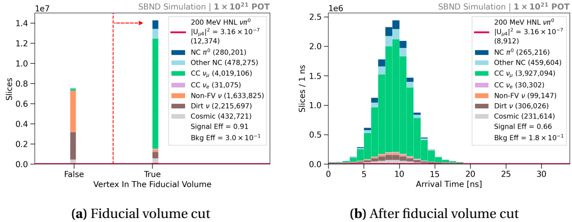
Fig. 9.6 Distribution of vertices reconstructed inside and outside of the FV with the cut (left) and the arrival time distribution after the cut (right).
