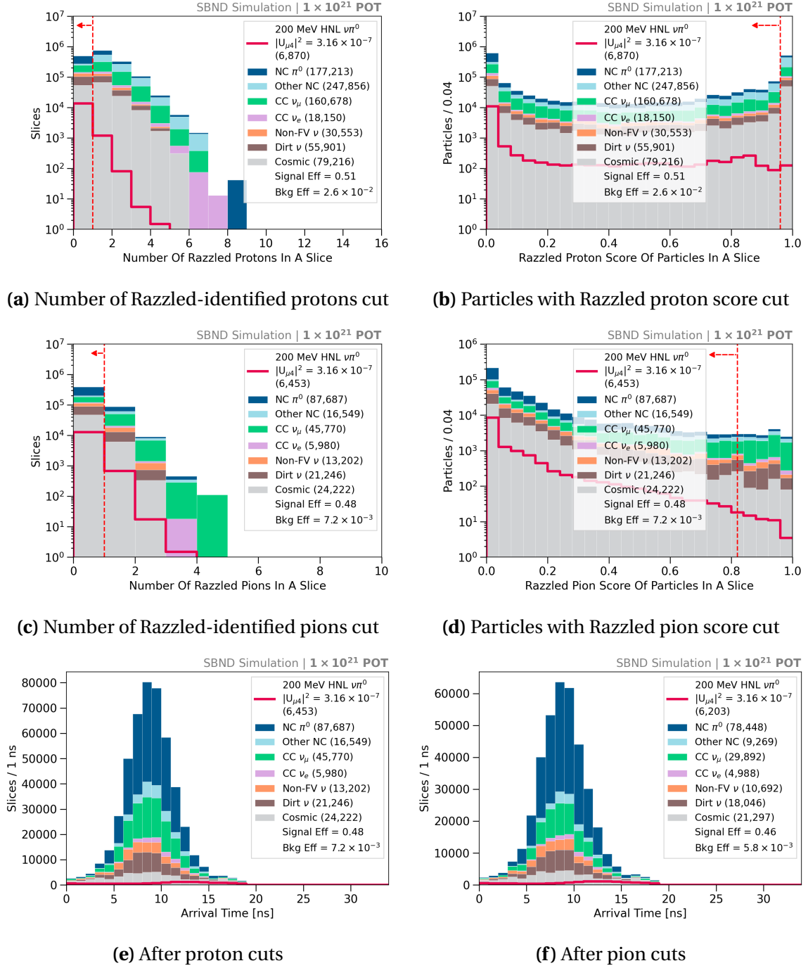
Fig. 9.9 Number of Razzled protons (pions) in a slice and Razzled proton (pion) score distributions with the cuts shown at the top (middle) and the arrival time distribution after the proton (pion) shown at the bottom left (bottom right).
