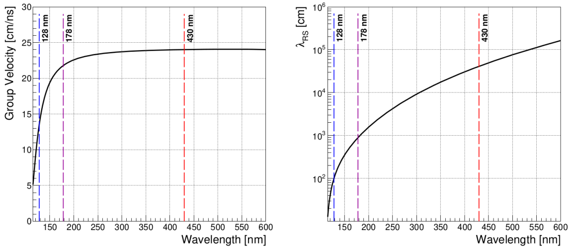
Fig. 3.9 Group velocity (left) and the Rayleigh scattering length (right) as a function of the photon wavelength in liquid argon [79].
