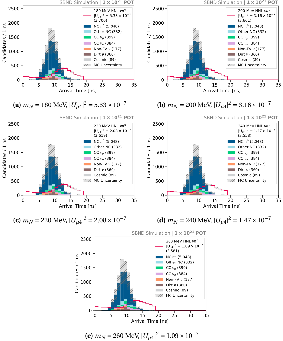
Fig. E.2 Arrival time distributions of HNLs, SM neutrinos and cosmic muons after the stringent selection, normalised to the exposure of 1 \times 10^{21} POT. HNLs of mass m_N is normalised to the listed coupling |U_{\mu 4}|^2 .
