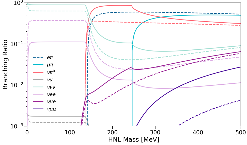
Fig. 2.3 Branching ratios of probable decay channels of an HNL produced from the BNB, with the U_{\mu 4} ( U_{e 4} ) coupling plotted as solid (dashed) lines.
