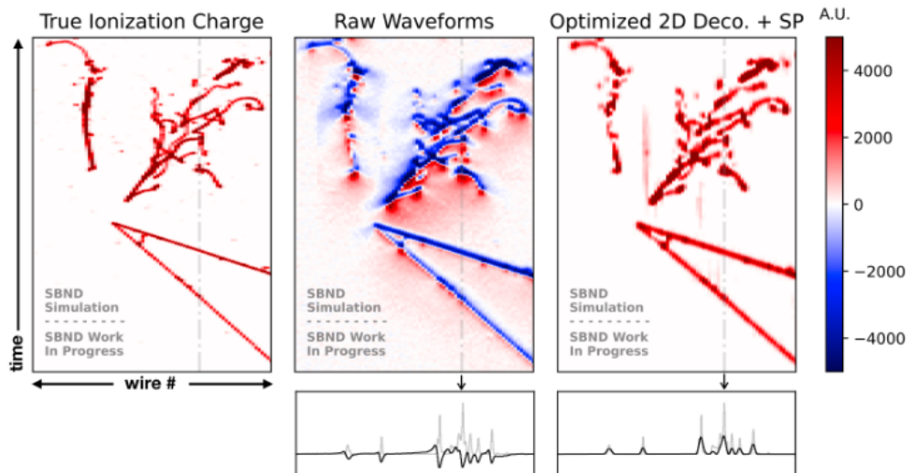
Fig. 6.2 Event displays of a simulated neutrino interaction using true charges (left), raw waveforms (middle) and deconvolved waveforms (right) [120].
