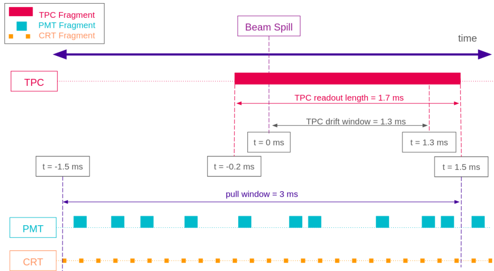
Fig. 4.8 Diagram depicting the chronological structure of a physics event.
