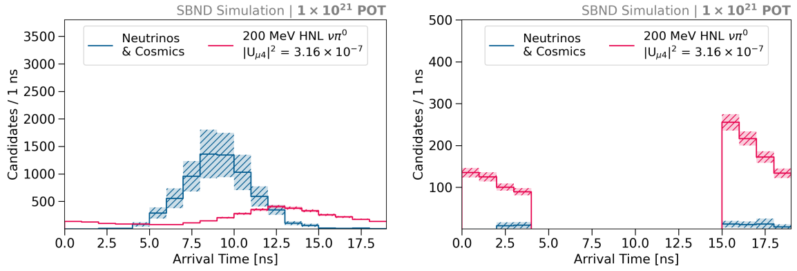
(b) The stringent distribution
