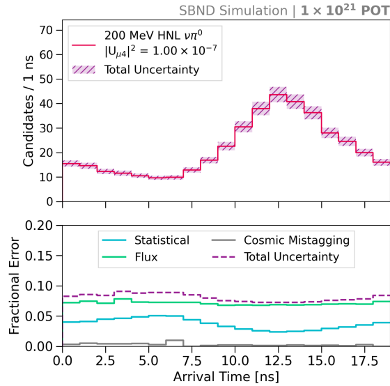
Fig. 10.2 Arrival time distribution of 200 MeV HNLs with the total uncertainty (top) and fractional uncertainties (bottom), normalised to the exposure of 1 \times 10^{21} POT and |U_{\mu 4}|^2 = 1 \times 10^{-7} .
