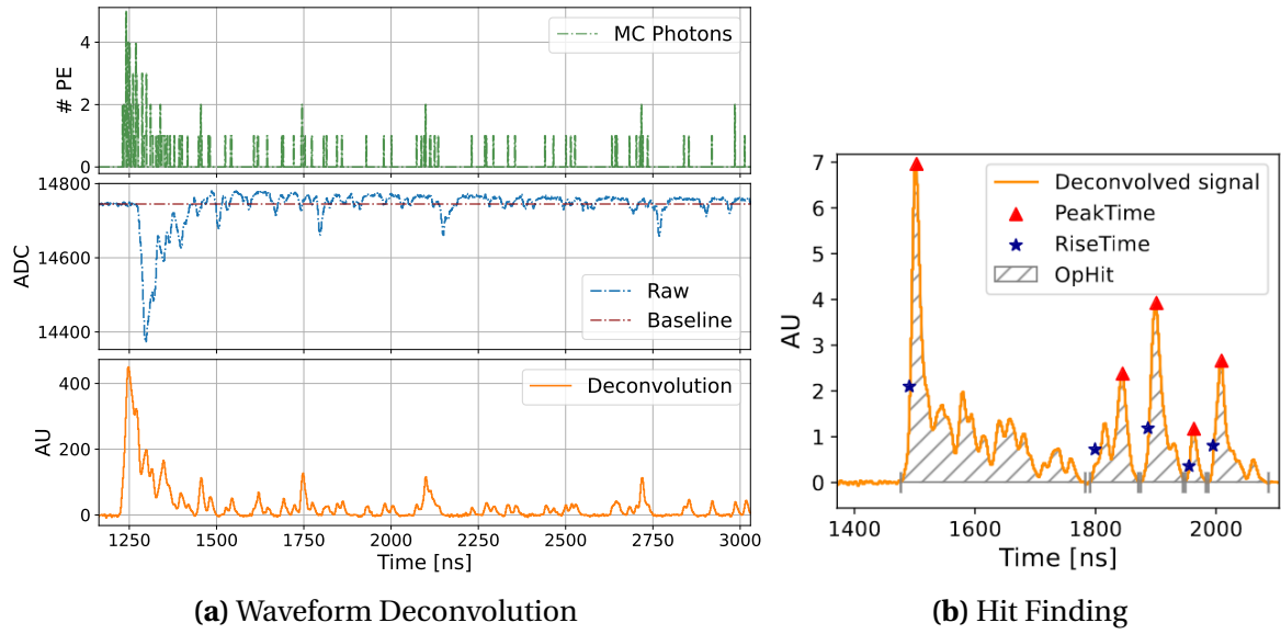
Fig. 6.7 Example demonstrating (a) waveform deconvolution and (b) hit finding applied to a PMT waveform [73].
