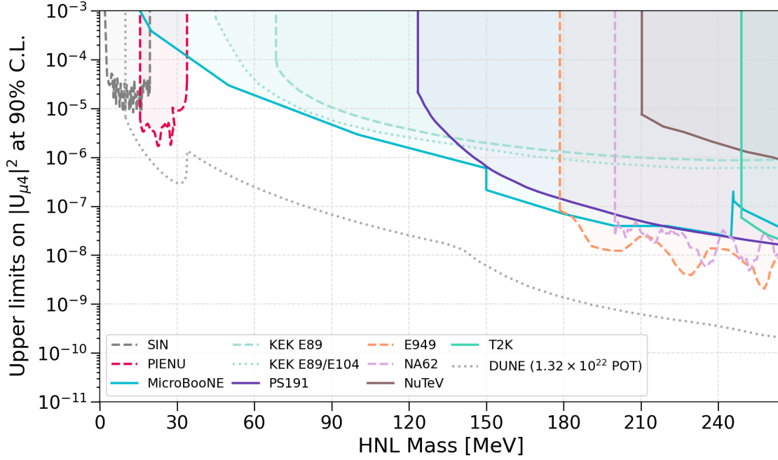
Fig. 2.5 Upper limits on the coupling |U_{\mu 4}|^2 at the 90% confidence level for Majorana HNLs in the mass range of 0 < m_N < 265 MeV, including results from SIN [30], PIENU [31], MicroBooNE [43–45], KEK E89 [33], KEK E89/E104 [34], PS191 [40], E949 [35], NA62 [37], NuTeV [41], T2K [42] and expected results from DUNE [26].
