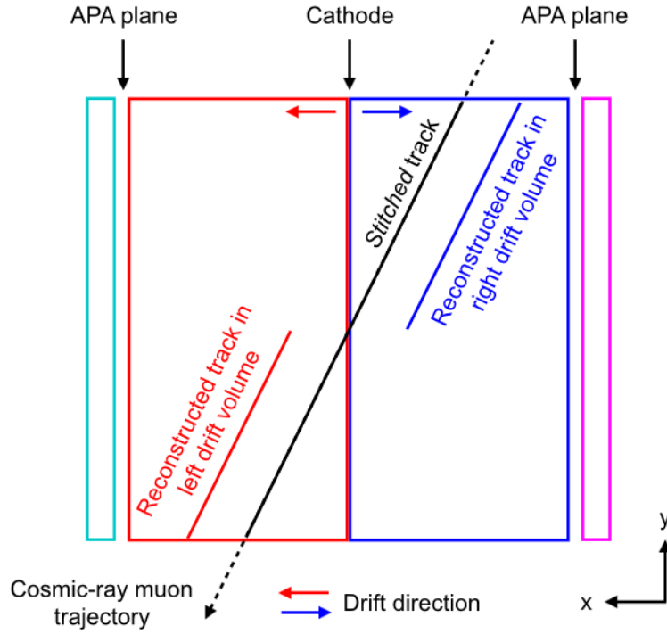
Fig. 8.1 Cathode stitching process to determine the t_0 of cathode-crossing track [132].
