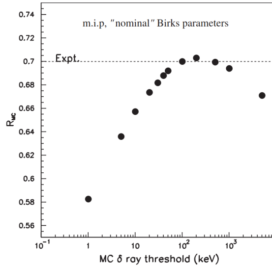
Fig. 8.12 Recombination factor as a function of the delta ray threshold [131].
