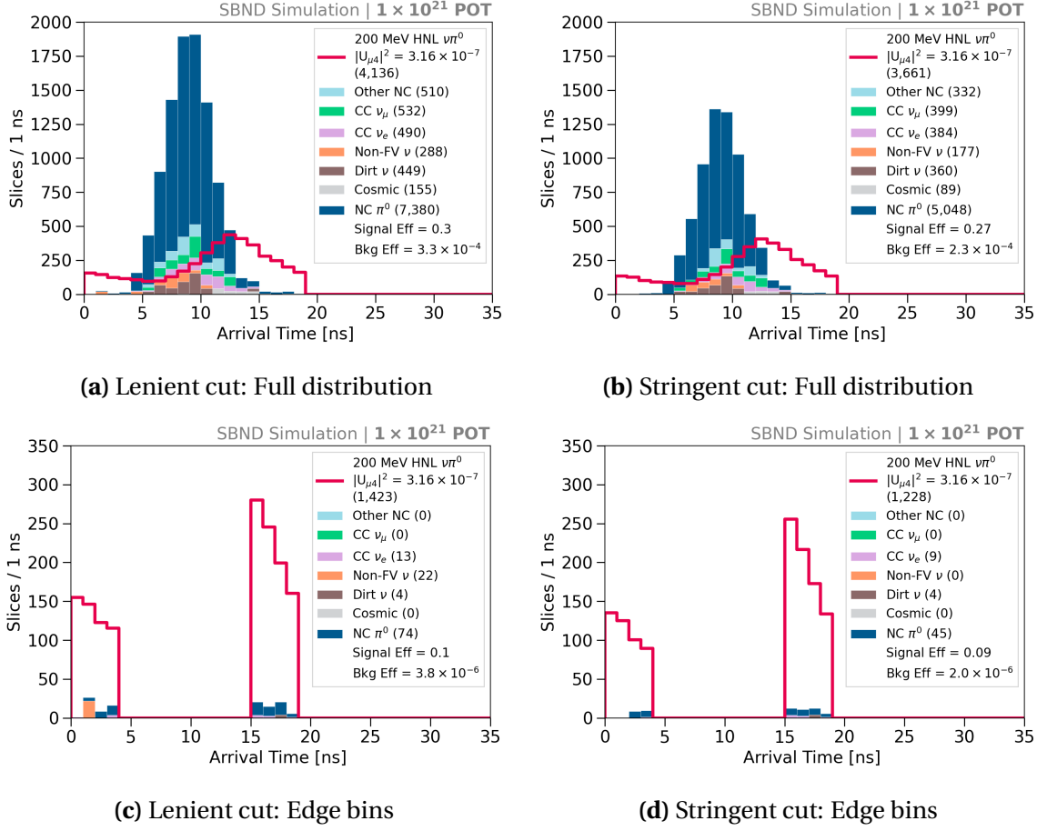
Fig. 9.15 Arrival time distributions after the lenient (left) and stringent cut (right).
