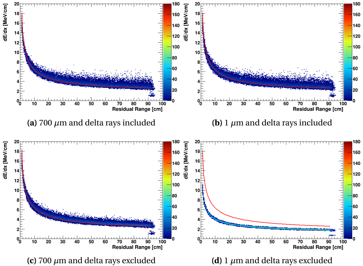
Fig. 8.10 dE/dx as a function of residual range for a 1 GeV proton at the delta ray threshold of 700\ \mu\text{m} (left) and 1\ \mu\text{m} (right), including (top) and excluding (bottom) the energy loss of delta rays.
