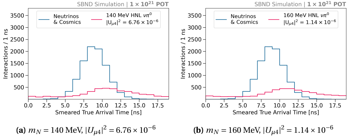
Fig. F.1 Arrival time distributions of HNLs, SM neutrinos and cosmic muons under the assumption of a timing resolution improvement, normalised to the exposure of 1 \times 10^{21} POT. HNLs of mass m_N is normalised to the listed coupling |U_{\mu 4}|^2 .
