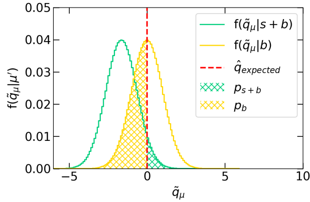
Fig. 10.5 Example of \tilde{q}_\mu distributions using the asymptotic approximation.
