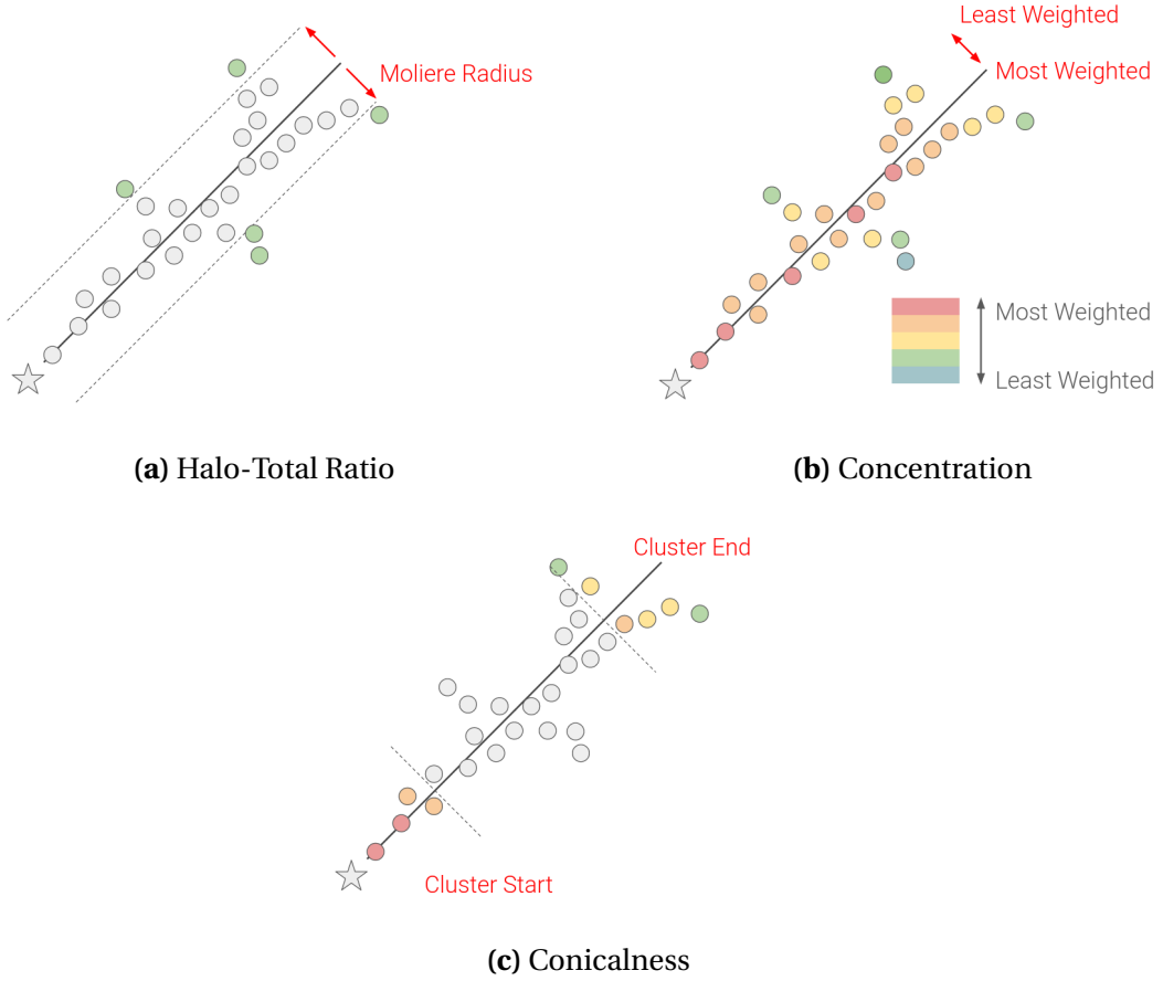
Fig. 6.4 Variables describing how cone-like the charge distribution is.
