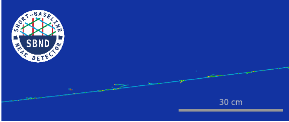
Fig. 8.5 Event display of a simulated cosmic muon track segment, with many delta rays produced along the track.
