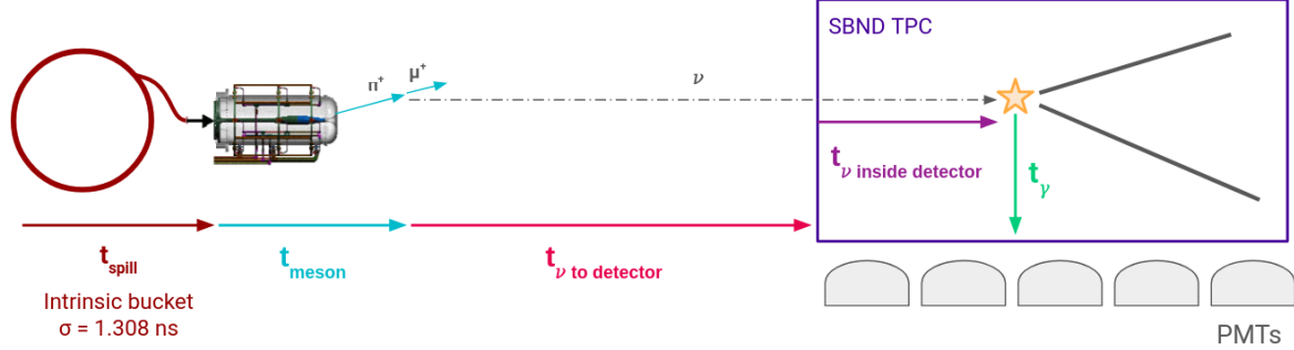
Fig. 9.17 Diagram showing smearing contributors to the arrival time.
