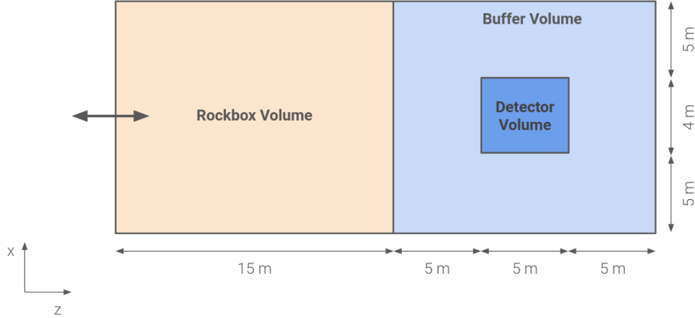
Fig. 5.8 Volume boundary defined by the GENIE generator to simulate neutrino interactions occurring inside and outside of the detector volume.
