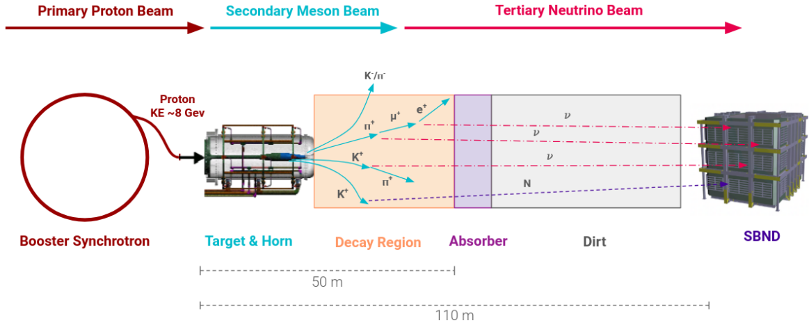
Fig. 4.10 Diagram showing the particle production in the BNB.
