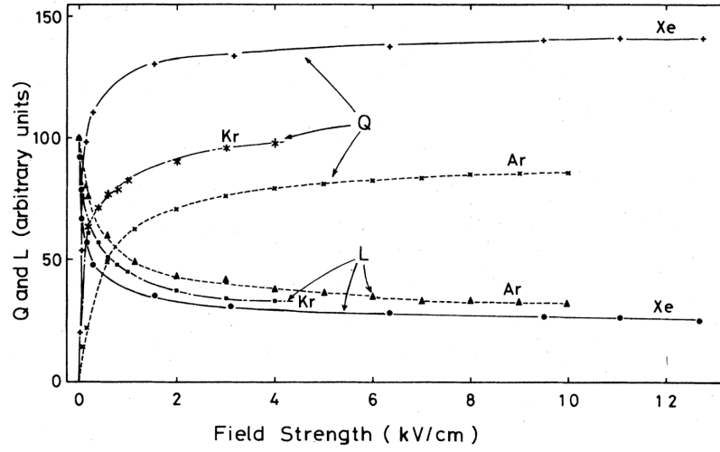
Fig. 3.7 Anti-correlation of charge yield Q and light yield L as a function of the electric field strength [66].
