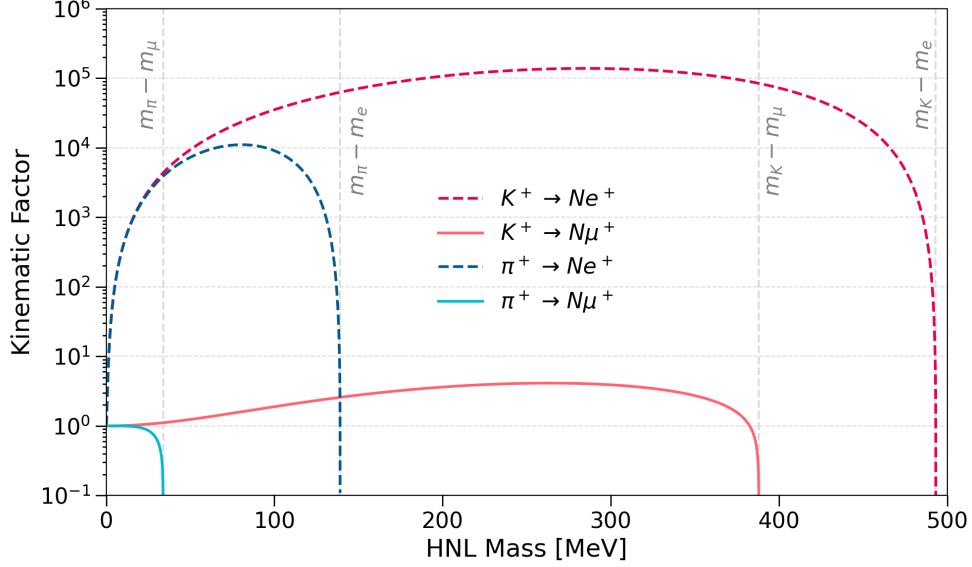
Fig. 2.2 Kinematic factor of the HNL production from meson decays that are probable from the BNB.
