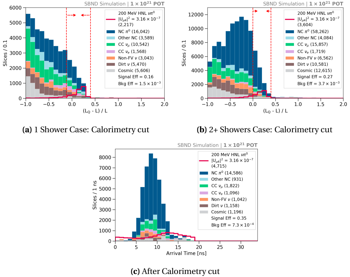
Fig. 9.12 Distributions of the (L_Q - L)/L with the cuts (top) and the arrival time distribution after the cut (bottom).
