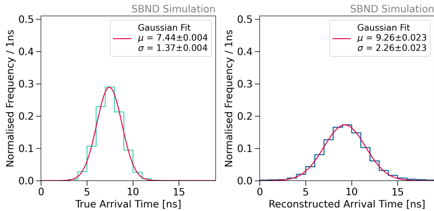
Fig. 9.18 Arrival time distributions of SM neutrinos from true (left) and reconstructed variables (right).
