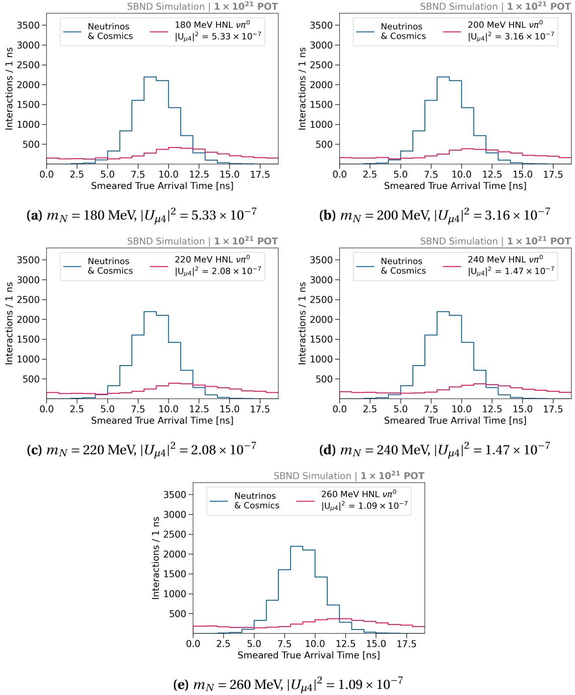
Fig. F.2 Arrival time distributions of HNLs, SM neutrinos and cosmic muons under the assumption of a timing resolution improvement, normalised to the exposure of 1 \times 10^{21} POT. HNLs of mass m_N is normalised to the listed coupling |U_{\mu 4}|^2 .
