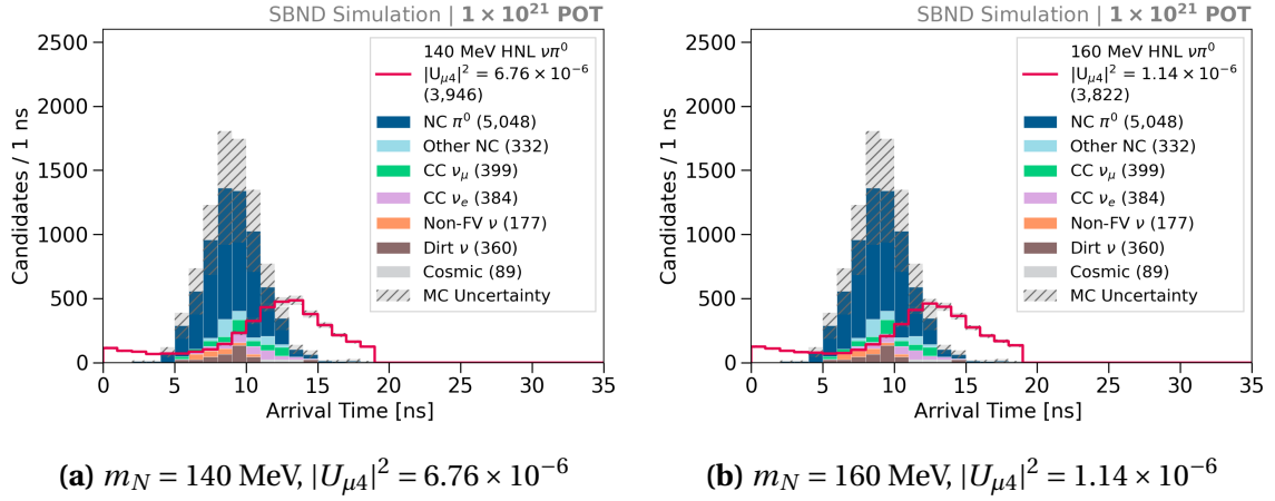
Fig. E.1 Arrival time distributions of HNLs, SM neutrinos and cosmic muons after the stringent selection, normalised to the exposure of 1 \times 10^{21} POT. HNLs of mass m_N is normalised to the listed coupling |U_{\mu 4}|^2 .
