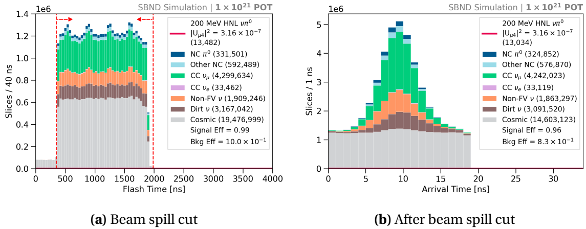
Fig. 9.4 Flash time distribution with the cut (left) and the arrival time distribution after the cut (right).
