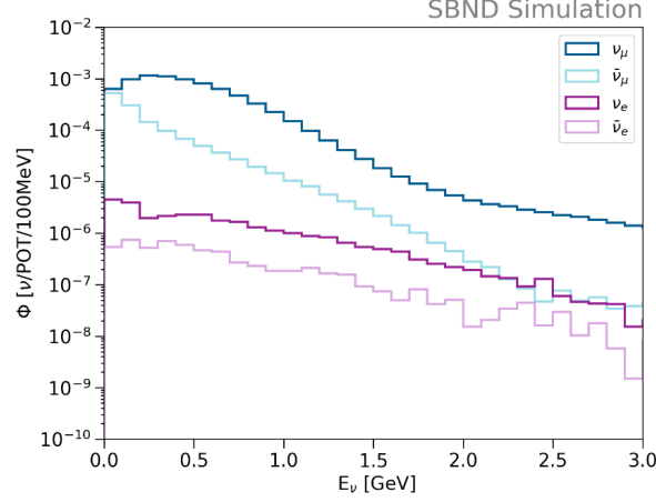
Fig. 4.12 Simulated neutrino fluxes at the front face of SBND.
