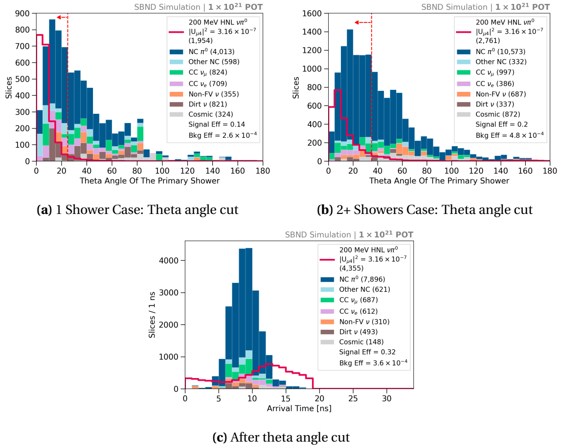
Fig. 9.13 Theta angle distributions with the cuts (top) and the arrival time distribution after the cut (bottom).
