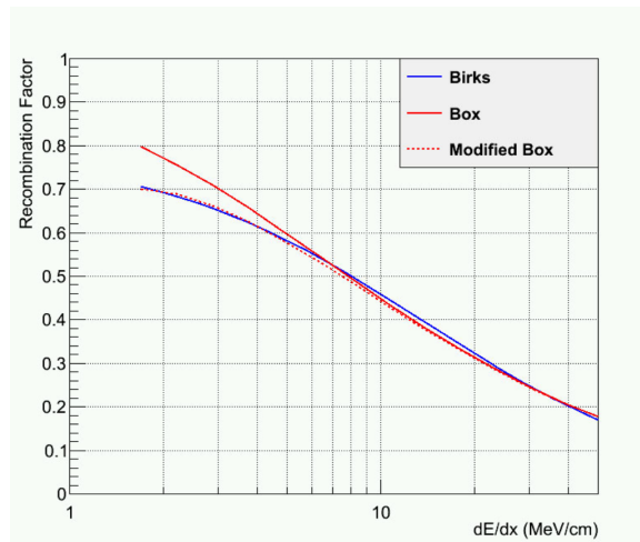
Fig. 3.6 Recombination factor in liquid argon as a function of the deposited energy density for an electric field of 500 V/cm [65].
