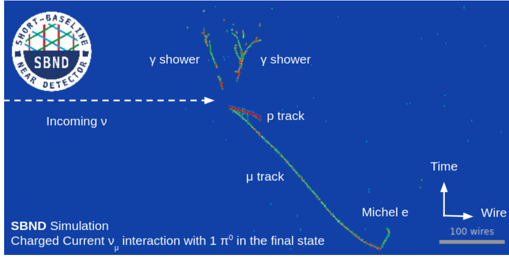
Fig. 3.4 Event display showing a simulated charged current \nu_\mu interaction containing a muon, a proton and a neutral pion in the final state.
