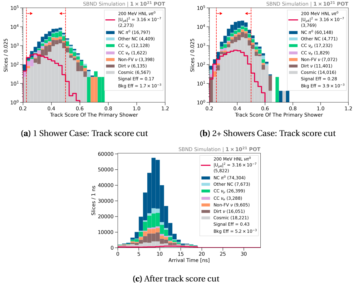
Fig. 9.11 Track score distributions with the cuts (top) and the arrival time distribution after the cut (bottom).
