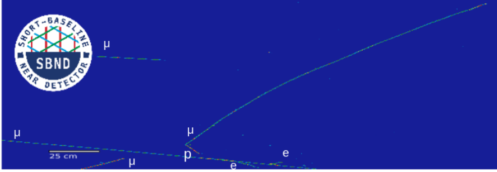
Fig. 9.3 Event display showing a muon and a proton track from a simulated \text{CC } \nu_\mu interaction together with a few cosmic muons.
