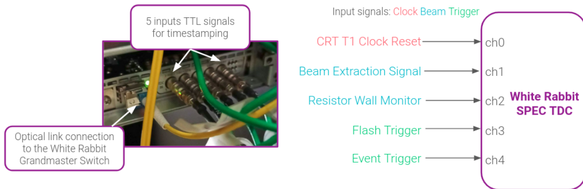
Fig. 7.2 The SPEC-TDC module installed at SBND (left) and signals input to the module for timestamping (right).
