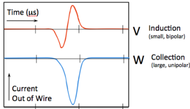
Fig. 3.10 Current signals on the induction and collection wire plane induced by a point-like charge deposition [58].
