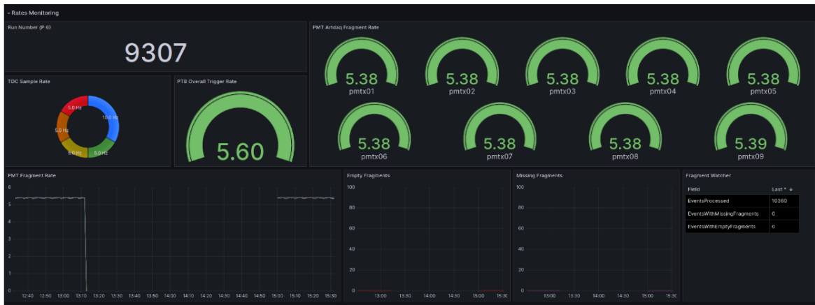
Fig. B.1 Web page showing a section of Grafana for monitoring the status of PMT DAQ.
