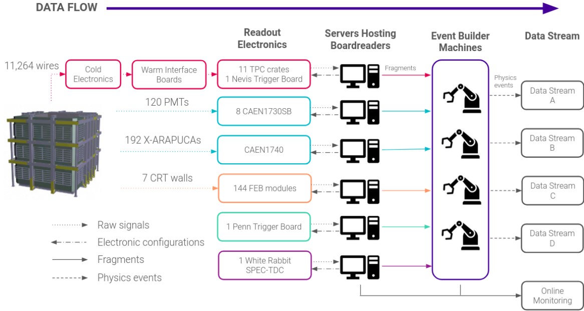
Fig. 4.7 Flow chart showing the data flow of data acquisition.
