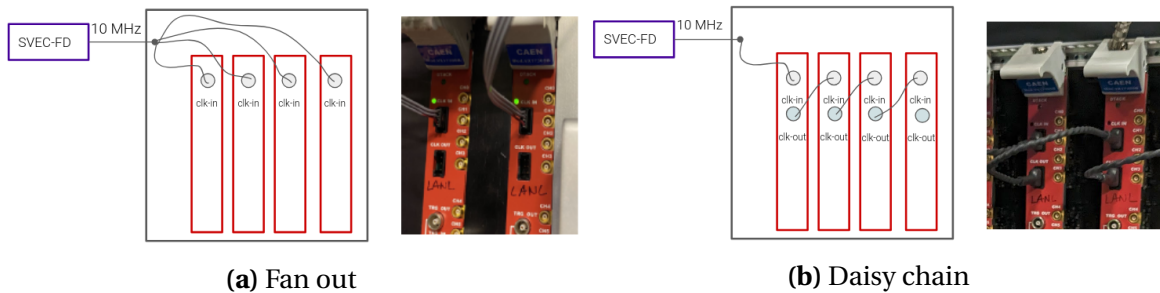
Fig. 7.10 Diagram illustrating two clock synchronisation schemes for CAENV1730SB digitisers, (a) fan out and (b) daisy chain.
