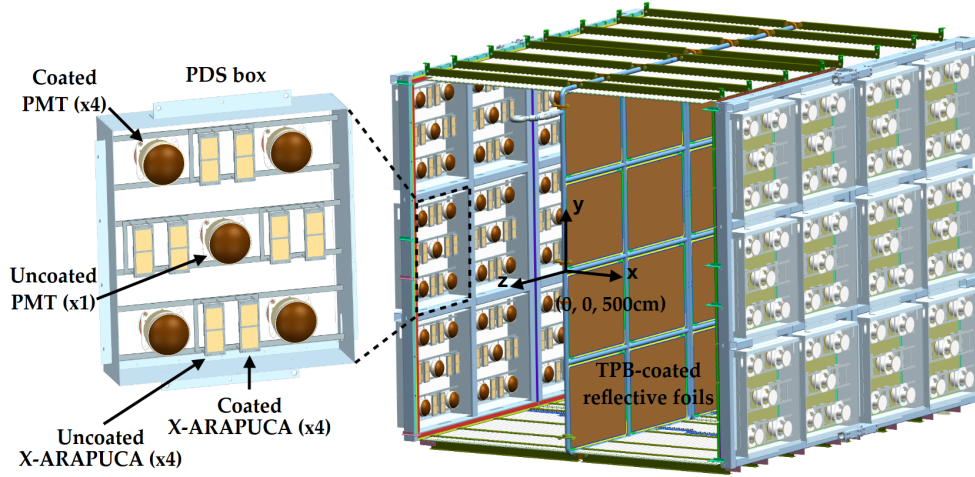
Fig. 4.5 3D model of a PDS box (left) and the PDS box arrangement on the east and west side of the TPC (right) [73].
