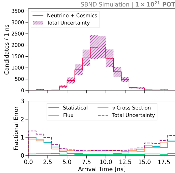
Fig. 10.4 Arrival time distributions of SM neutrino and cosmic backgrounds with the total uncertainty (top) and fractional uncertainties (bottom), normalised to the exposure of 1 \times 10^{21} POT.
