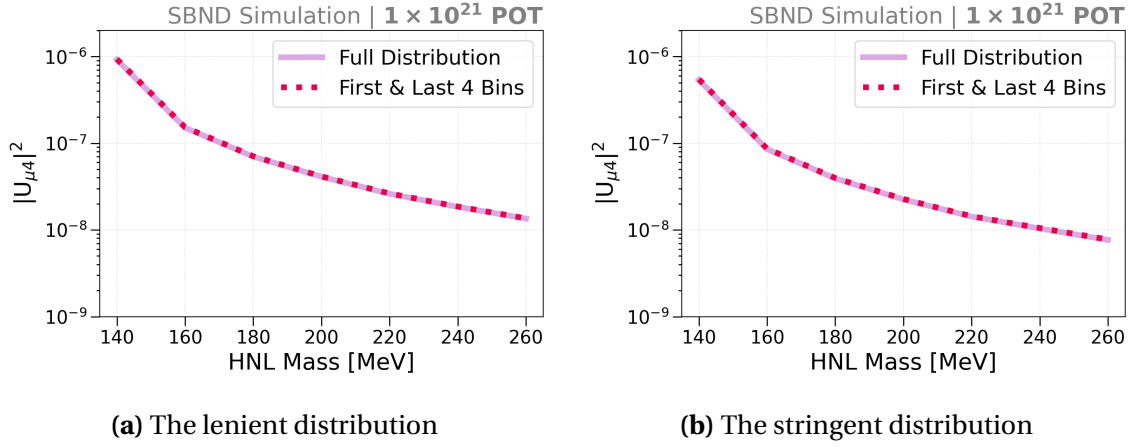
Fig. 10.8 Comparison between limits setting using the entire distribution and only the edge bins of (a) the lenient and (b) stringent arrival time distribution.
