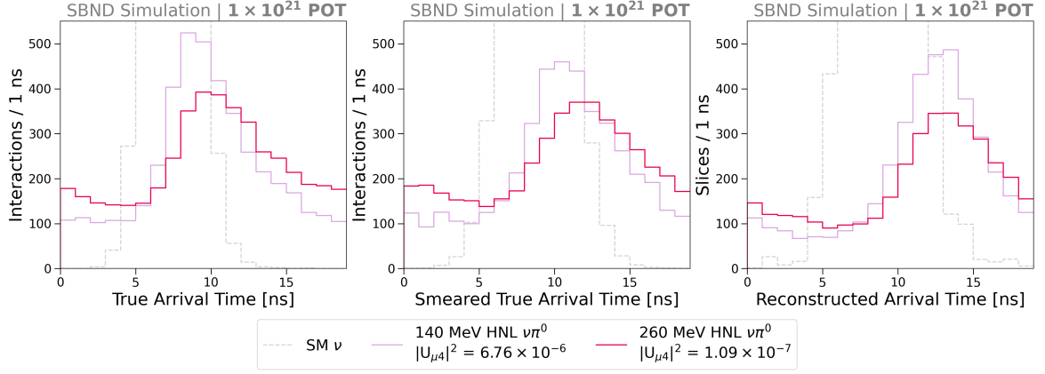
Fig. 9.20 Arrival time distributions of SM neutrinos and HNLs from true (left), smeared true (middle) and reconstructed variables after the lenient selection (right).
