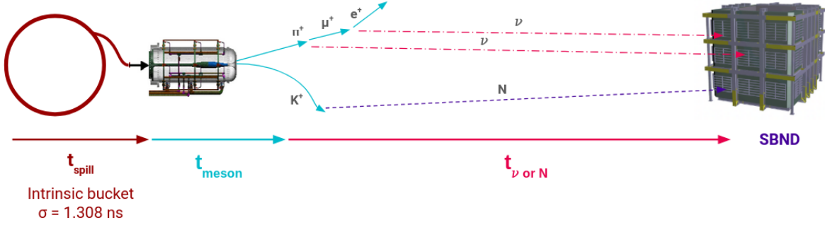
Fig. 5.5 The time of flight of a particle from the production to the detection location in the SBND detector.
