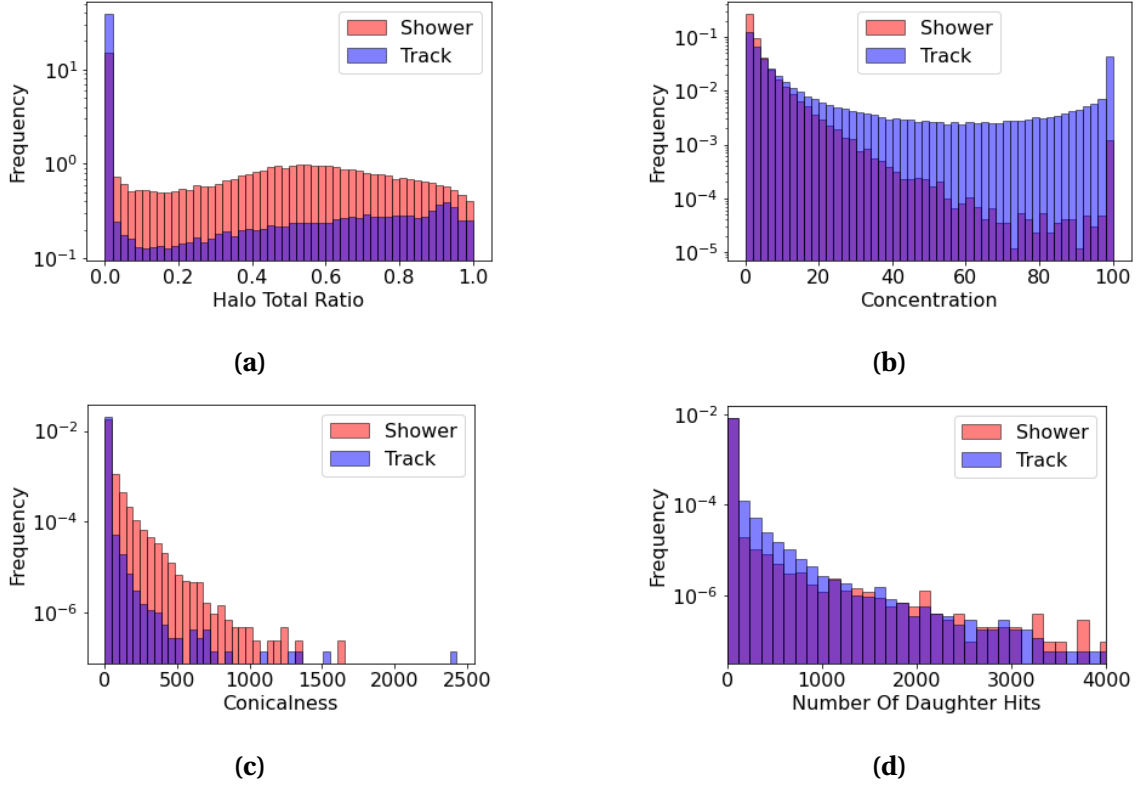
Fig. 6.5 Distributions of four new variables: (a) halo-total ratio, (b) concentration, (c) conicalness and (d) number of daughter hits.
