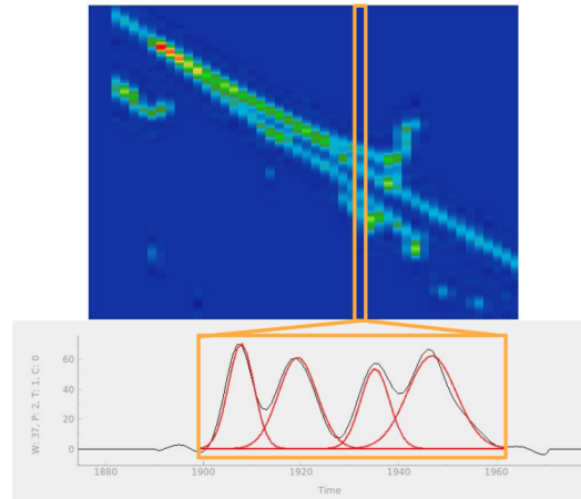
Fig. 6.3 Diagram illustrating the hit finding algorithm on a single wire [122].
