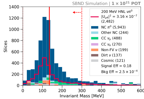
Fig. 9.14 \pi^0 invariant mass distribution with the cut applied to the multiple showers case.
