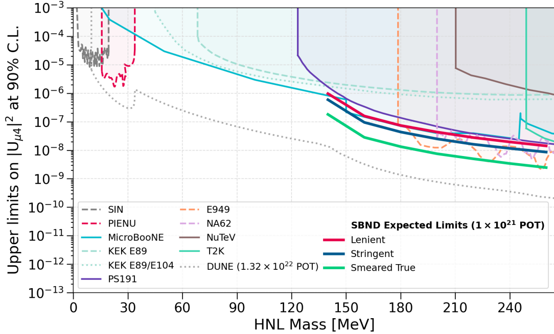
Fig. 10.10 Upper limits on the coupling |U_{\mu 4}|^2 at the 90% confidence level for Majorana HNLs in the mass range of 0 < m_N < 265 MeV. SBND expected limits are compared with existing experimental results, including SIN [30], PIENU [31], MicroBooNE [43–45], KEK E89 [33], KEK E89/E104 [34], PS191 [40], E949 [35], NA62 [37], NuTeV [41], T2K [42] and expected results from DUNE [26].
