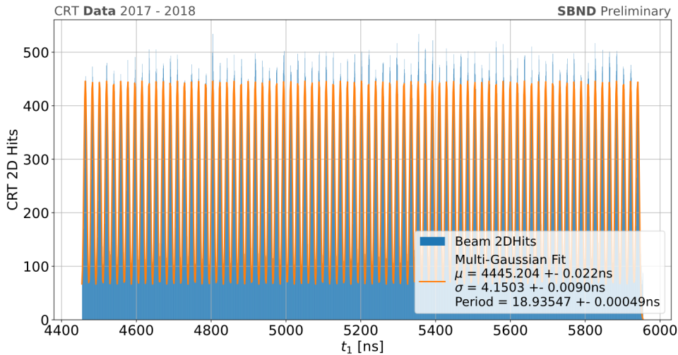
Fig. 4.9 The buckets of the BNB measured by the SBND CRTs during 2017–2018 [100].
