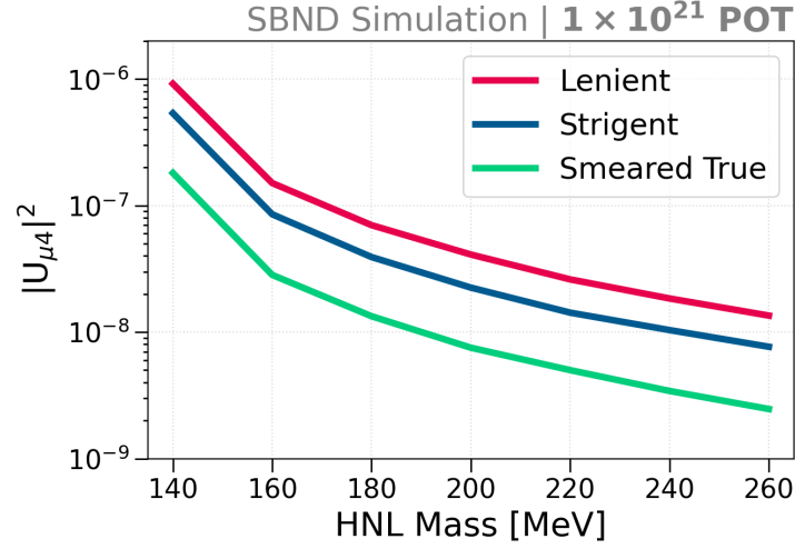
Fig. 10.9 Comparison between limits resulting from the lenient and stringent reconstructed distributions and the smeared true arrival time distribution.
