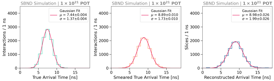
Fig. 9.19 Arrival time distributions of SM neutrinos from true (left), smeared true (middle) and reconstructed variables after the lenient selection (right).
