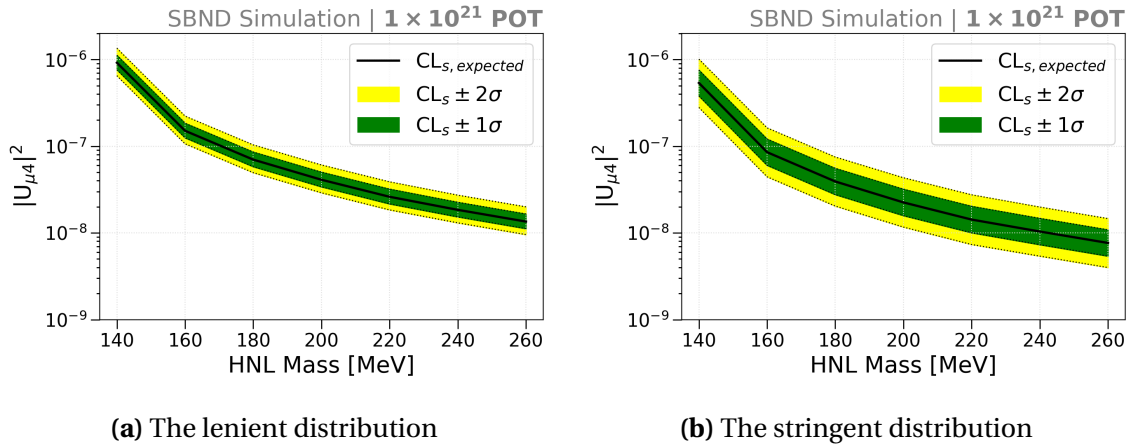
Fig. 10.7 Expected limits and the Brazil bands on the coupling |U_{\mu 4}|^2 for Majorana HNLs from (a) the lenient and (b) stringent arrival time distribution.
