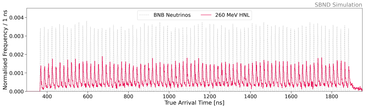
Fig. 5.6 True arrival time distribution at the front face of the SBND detector for SM neutrinos and HNLs.
