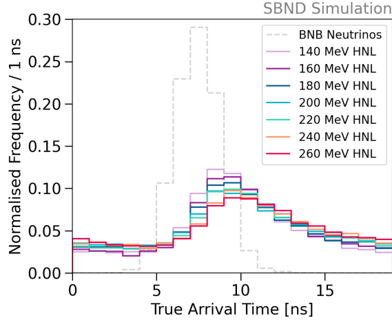
Fig. 5.7 True arrival time distribution for SM neutrinos and HNLs after applying a modulus of 19 ns .
