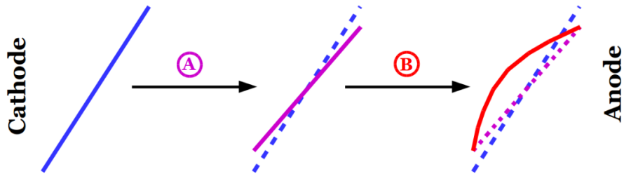
Fig. 3.8 Impacts of SCE on tracks: bending away towards the detector edges (middle) and bowing towards the cathode (right) [72].
