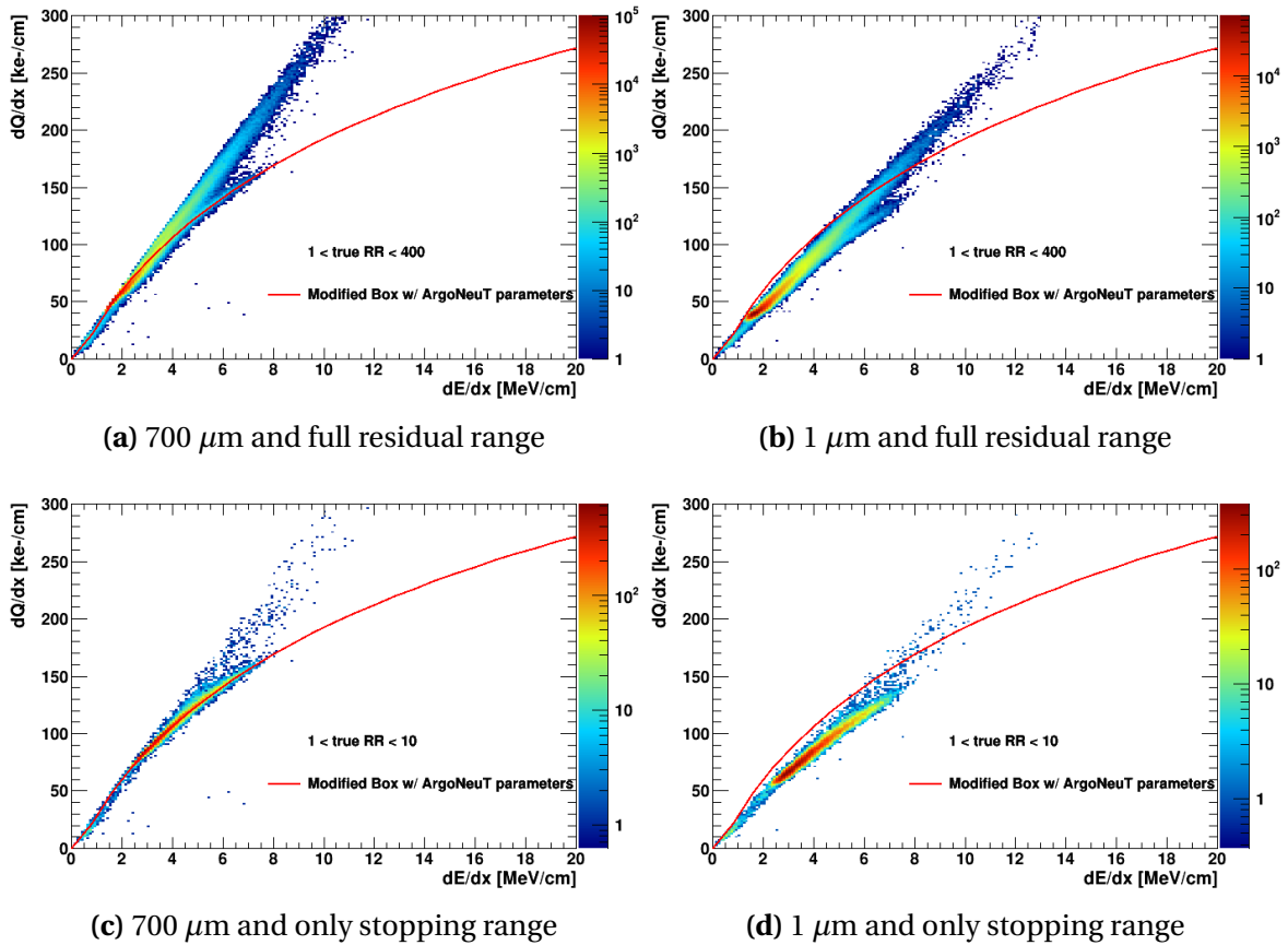
Fig. 8.8 dQ/dx as a function of dE/dx for a 1 GeV muon at the delta ray threshold of 700\ \mu\text{m} (left) and 1\ \mu\text{m} (right) and for the full residual range (top) and only the stopping range (bottom).
