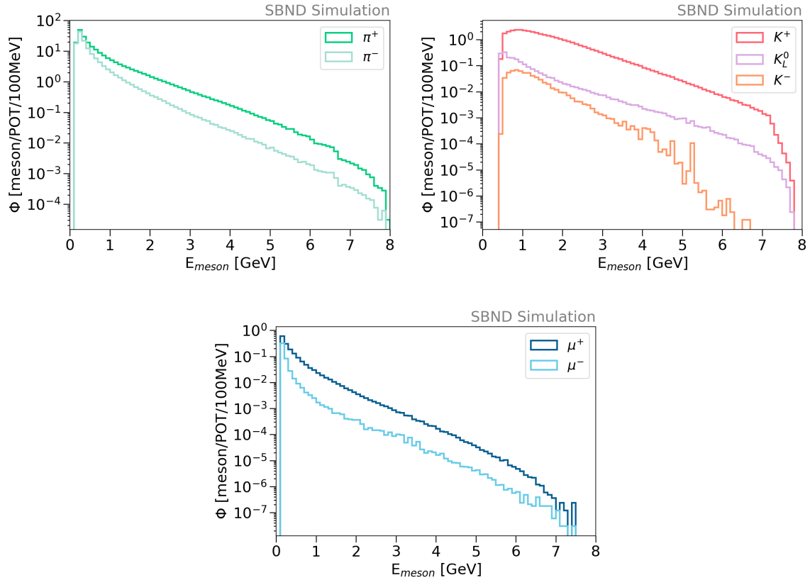
Fig. 4.11 Simulated fluxes for the secondary mesons produced in the BNB.
