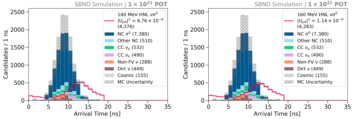
(a) m_N = 140 MeV, |U_{\mu 4}|^2 = 6.76 \times 10^{-6}
