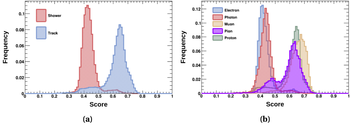
Fig. 6.6 Score distribution of the updated track-shower BDT, plotted for (a) track-like and shower-like particles and (b) different particle types.
