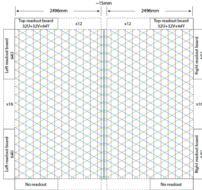
Fig. 4.3 Schematic showing two coupled APAs to form a complete APAs [93].
