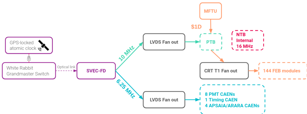
Fig. C.1 Clock signal distribution from the White Rabbit timing system to the DAQ subsystems.
