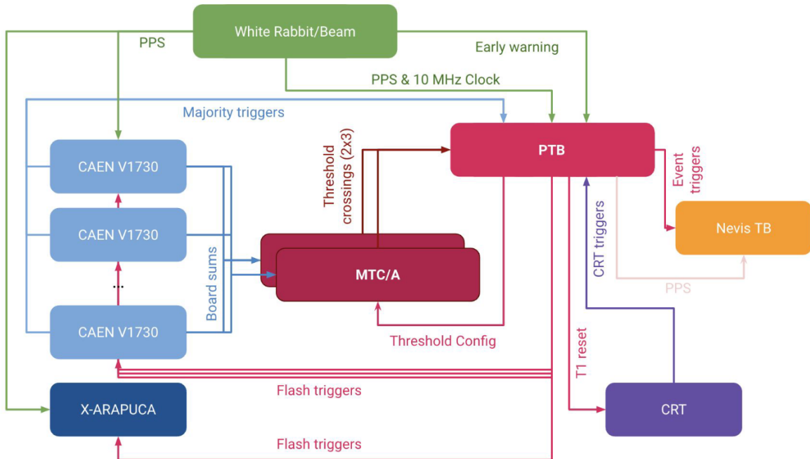
Fig. A.1 Distribution of the signals in the hardware triggering [141].
