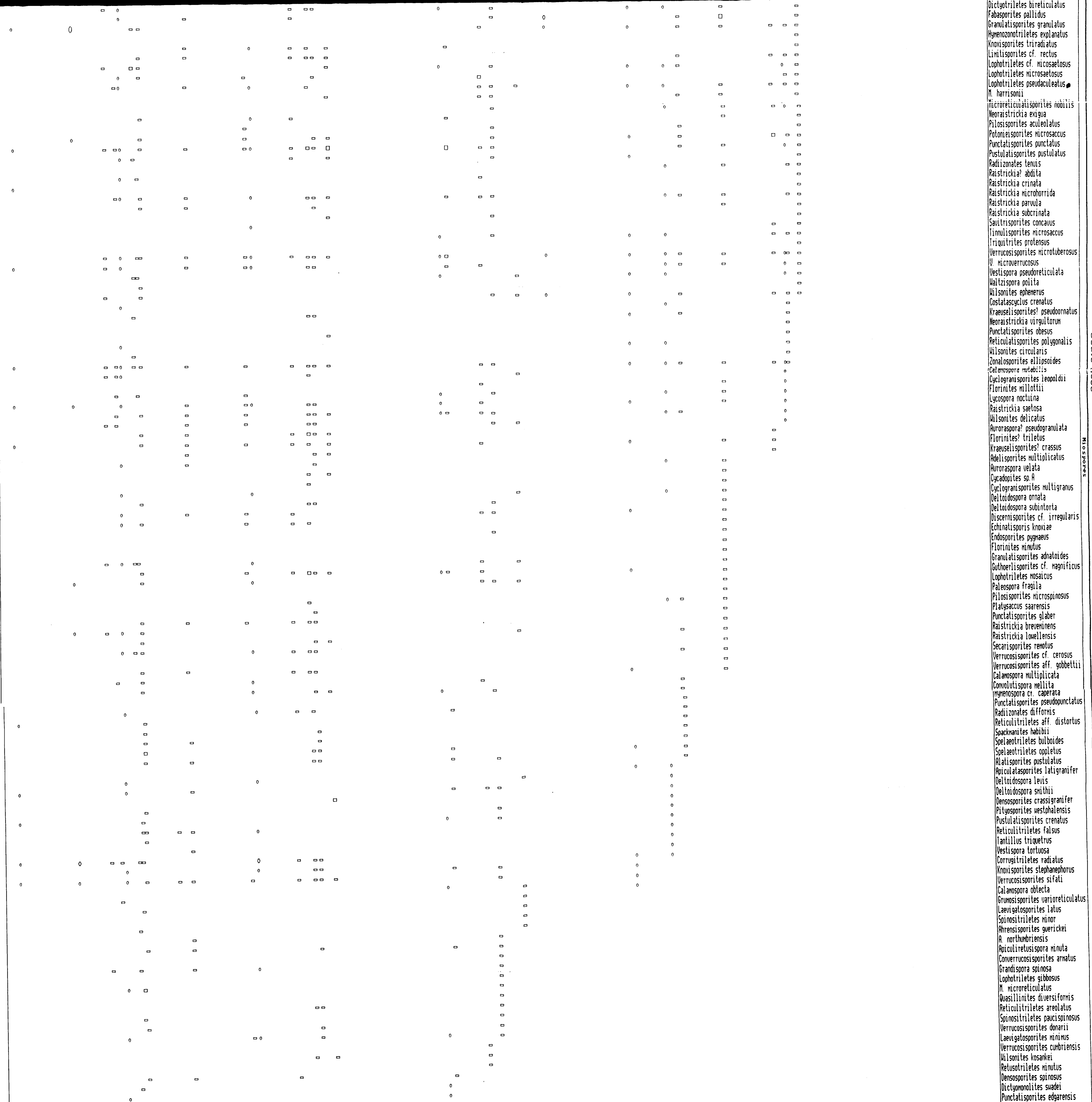
ENCLOSURE 2 STRATIGRAPHIC DISTRIBUTION OF PALYNOFORMS IN WELL 44/22-3. Scale 1:500
