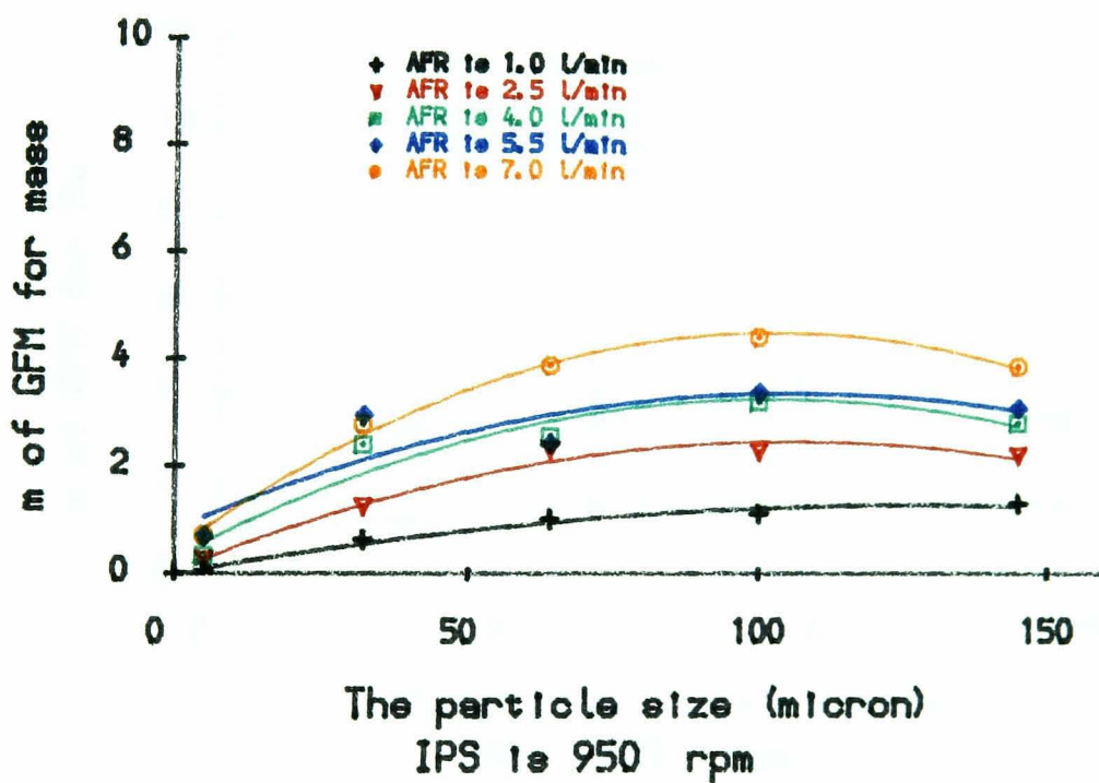
Fig8-31 AFR effect on GFM parameters in mass
