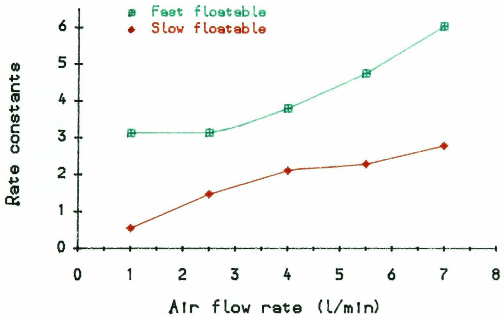
2. Coal flotation (+75)
