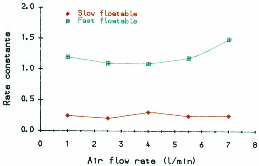
1) Chalcopyrite flotation
