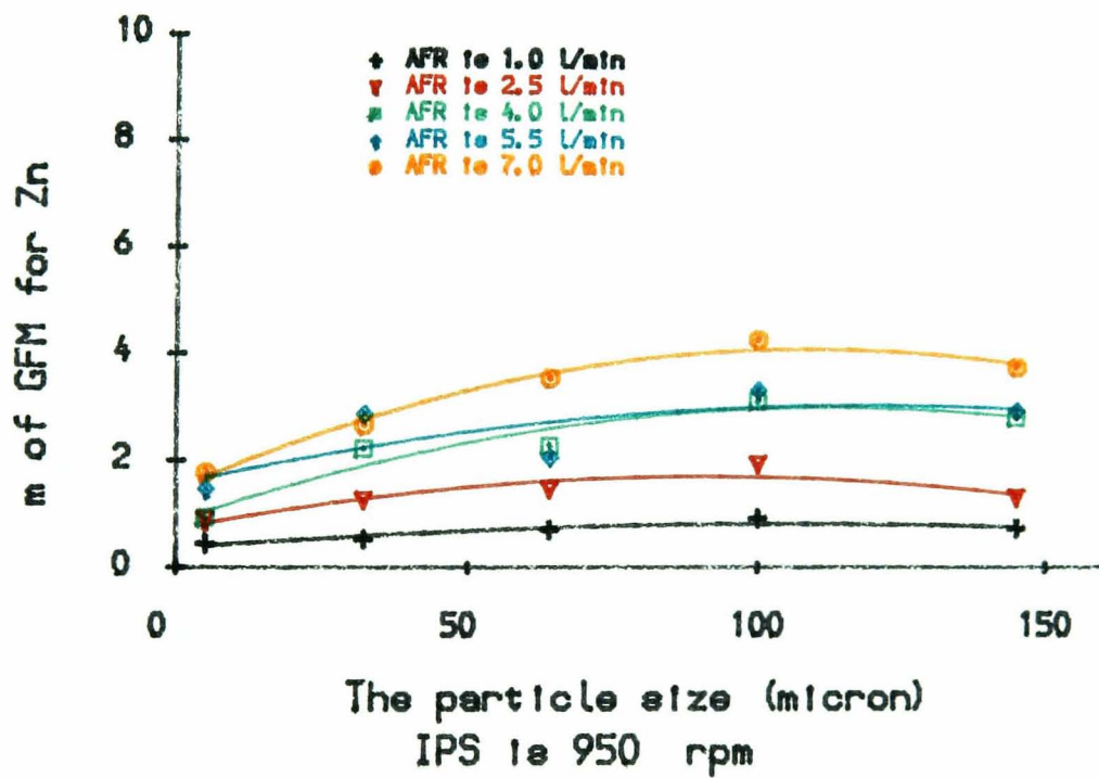
Fig8-33 AFR effect on GFM parameters in Zn
