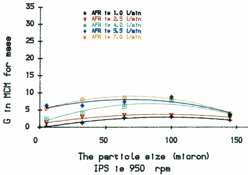
Fig8-17 AFR effect on MCM parameters in mass
