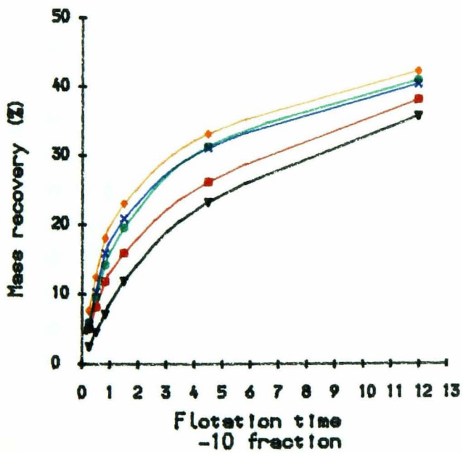
Fig 7-13 IPS effect on Mass recovery of complex sulphide flotation
