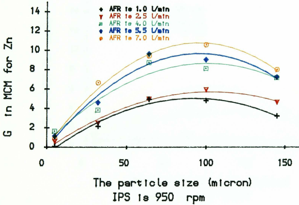
Fig8-19 AFR effect on MCM parameters in Zn
