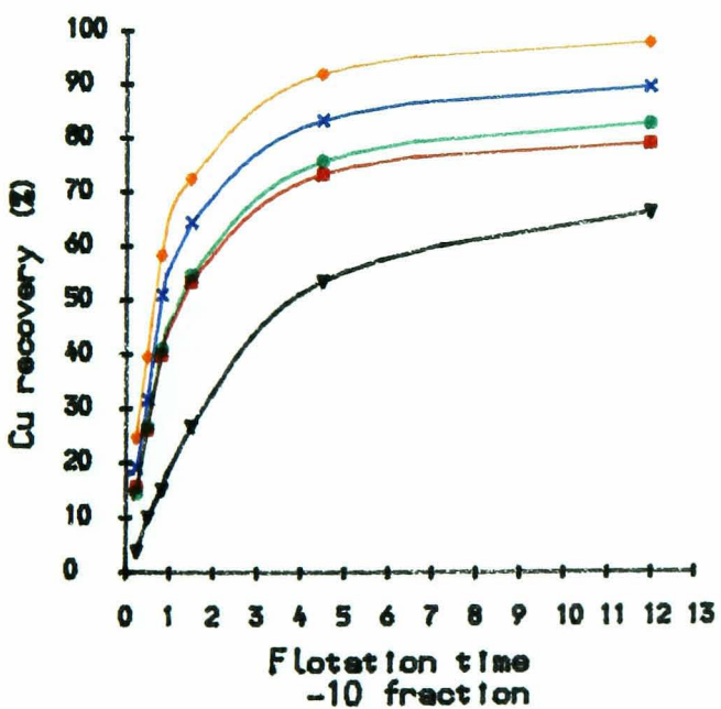
Fig 7-15 IPS effect on Cu recovery of complex sulphide flotation
