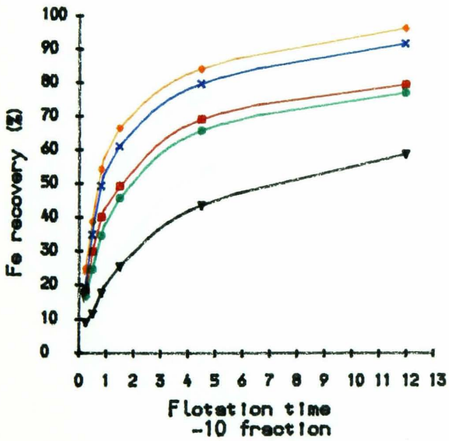
Fig 7-14 IPS effect on Fe recovery of complex sulphide flotation
