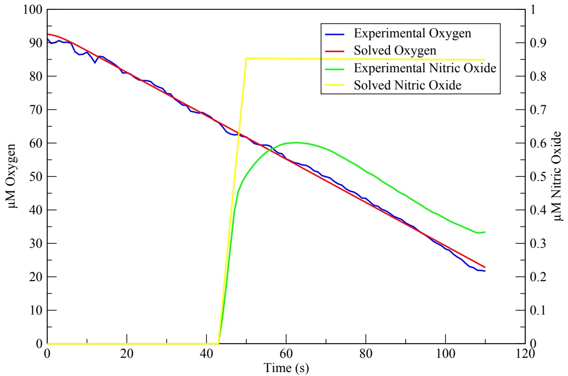
Figure 6.7: Nitric Oxide Reduction in Neisseria meningitidis . This figure shows the first attempt at fitting the model to experimental data using priors determined from literature values. Nitric oxide disappearance is not being modelled at all.
