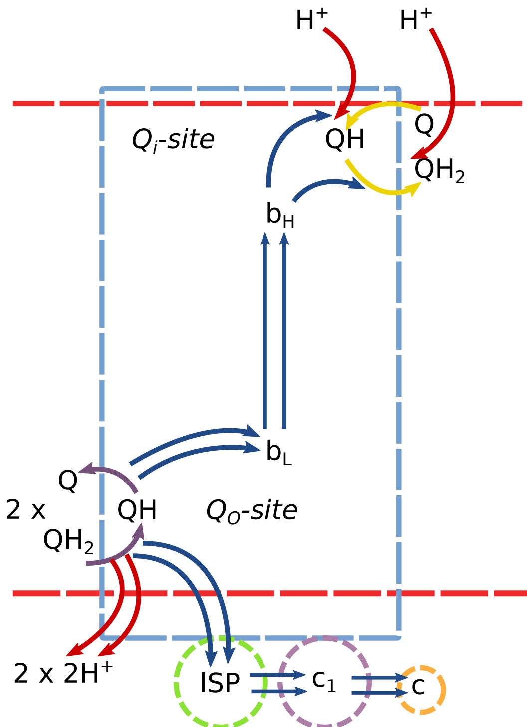
Figure 1.6: The modified Q-cycle used by the bacterial bc_1 complex. The cytochrome b subunit is represented by the dashed blue outline, and contains the Q_o - and Q_i -sites, connected by hemes b_L and b_H . The ISP (Rieske Iron-Sulfur Protein) and cytochrome c_1 catalytic domains and cytochrome c are represented by dashed circles . Electron transfer steps are shown by blue arrows , proton release and uptake by red arrows , binding and release of quinone species by purple arrows for Q_o -site and yellow arrows for Q_i -site. Adapted from Crofts et al. 65 .
