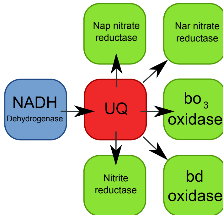
Figure 1.10: Branched electron transport chains of E. coli . Blue denotes initial electron donor, red denotes quinone pool and green denotes terminal reductases. UQ = ubiquinone. Under anaerobic conditions, ubiquinone is replaced by menaquinone. Adapted from Nicholls and Ferguson 74 .
