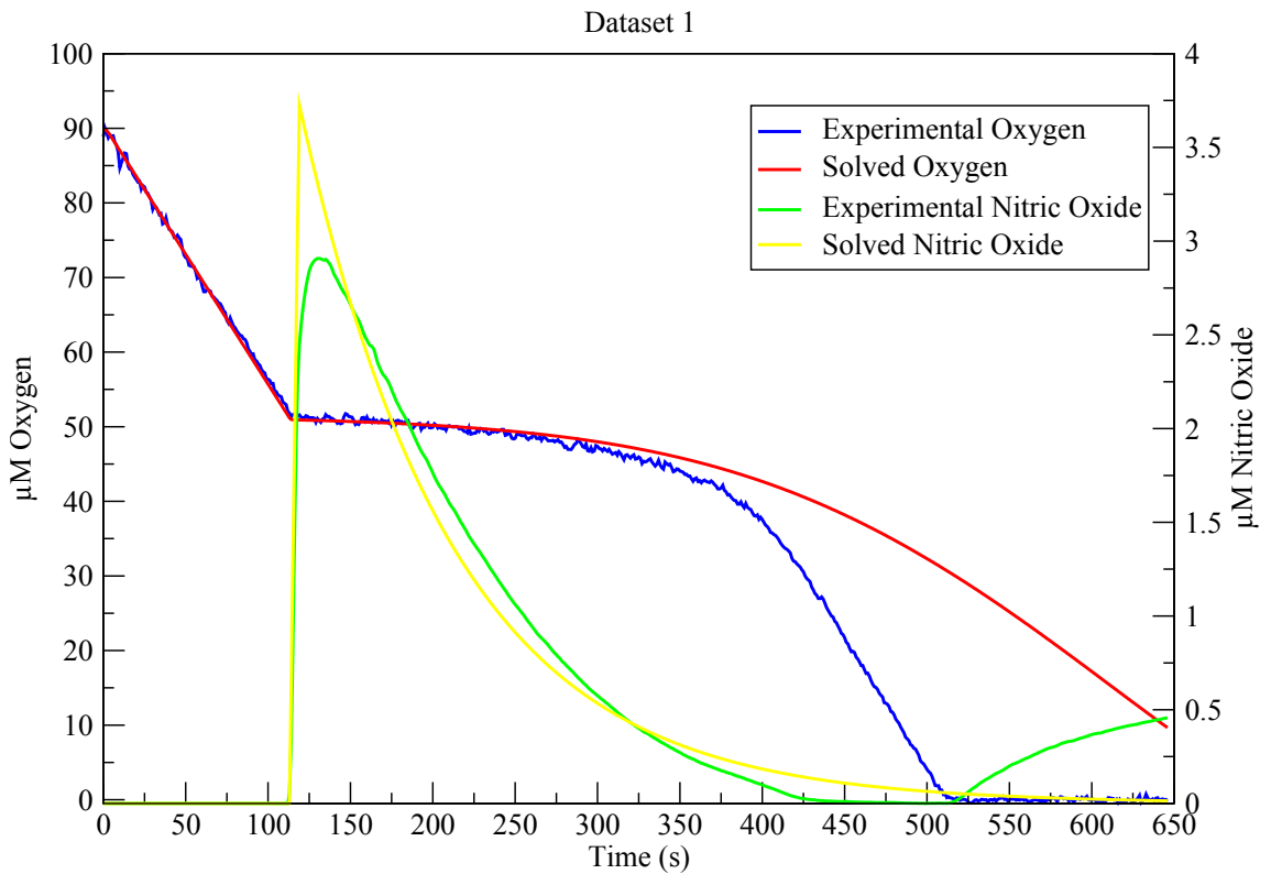
Figure 6.14: Addition of Nitric Oxide to in silico norB - mutant. Solved output from an in silico norB - mutant created by removing NorB from the simulation in Figure 6.11.
