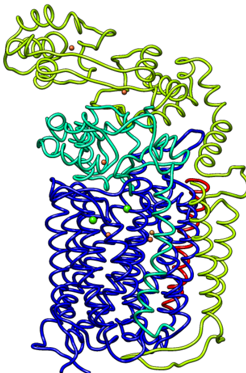
Figure 1.5: 3D Structure of cbb 3 oxidase. This figure shows the structure of cbb 3 from Pseudomonas stutzeri 49 . CcoN is shown by the blue chain, with the heme and copper centres being brown. CcoP is shown by the green chain, and CcoO by the cyan chain. The PDB ID for this structure is 3MK7.
