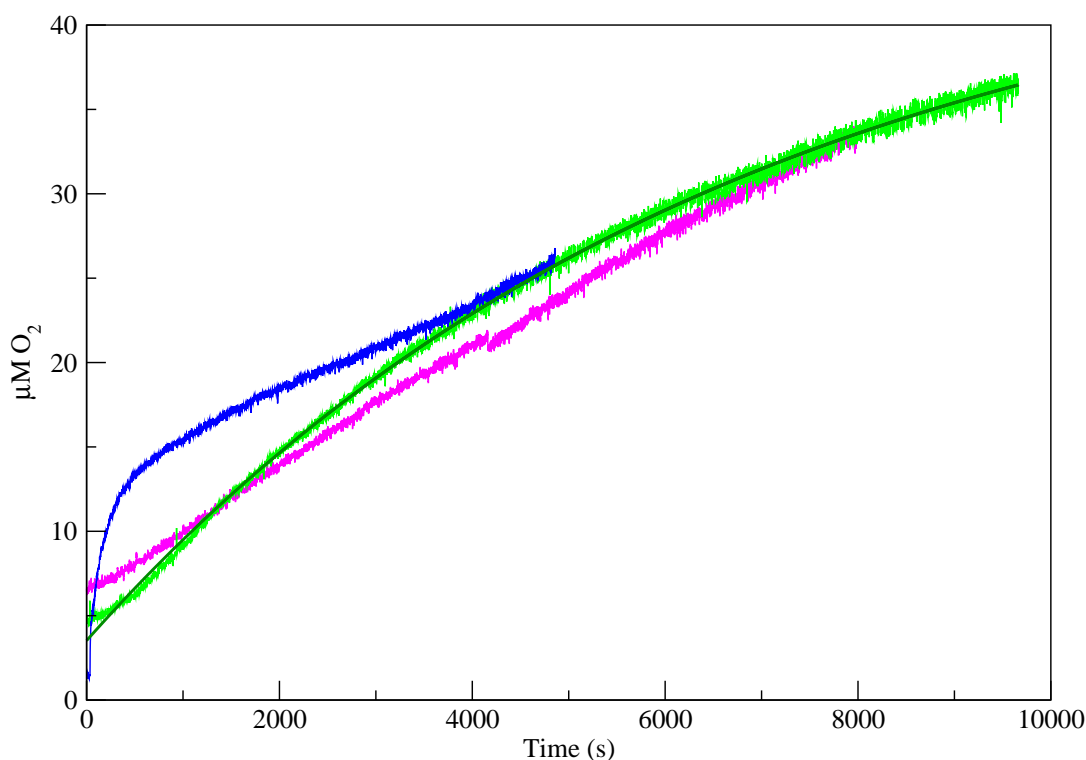
Figure 3.2: Oxygen Diffusion Rates. This figure shows experimentally observed rates of oxygen diffusion back into the electrode chamber. An exponential decay function has been fitted to the green dataset and produces the K_O value (the effective saturation concentration) of \approx 48 \mu\text{M} .
