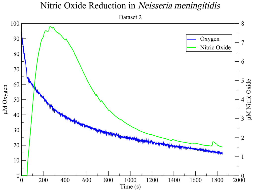
Figure 6.3: Nitric Oxide Reduction in Neisseria meningitidis . This dataset shows the effect on rate of oxygen reduction as a larger amount of nitric oxide (to \approx 7.8 \mu\text{M} ) is introduced to the respiring system.
