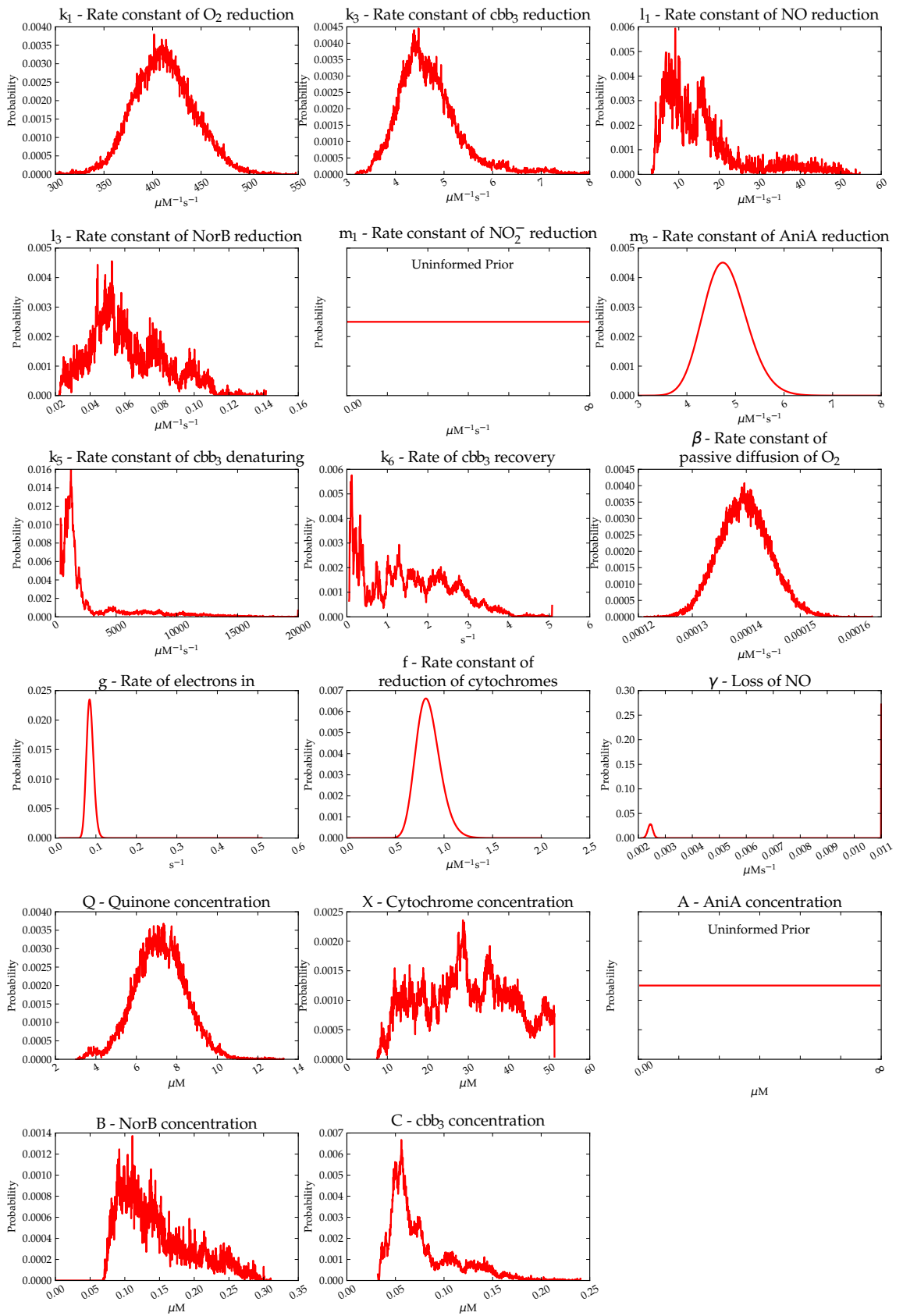
Figure 7.9: Prior probability distributions for microaerobic oxygen and nitrite reduction. These are the modified probability distributions used as priors by the parameter estimation algorithm.
