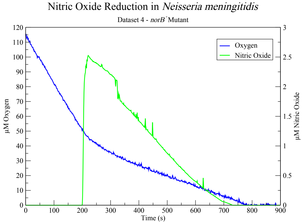
Figure 6.5: Nitric Oxide Reduction in Neisseria meningitidis . This dataset shows the effect on rate of oxygen reduction as nitric oxide (to \approx 2.5 \mu\text{M} ) is introduced to a respiring norB - mutant culture. Any removal of nitric oxide here is due to diffusion and sequestering by cbb 3 alone.
