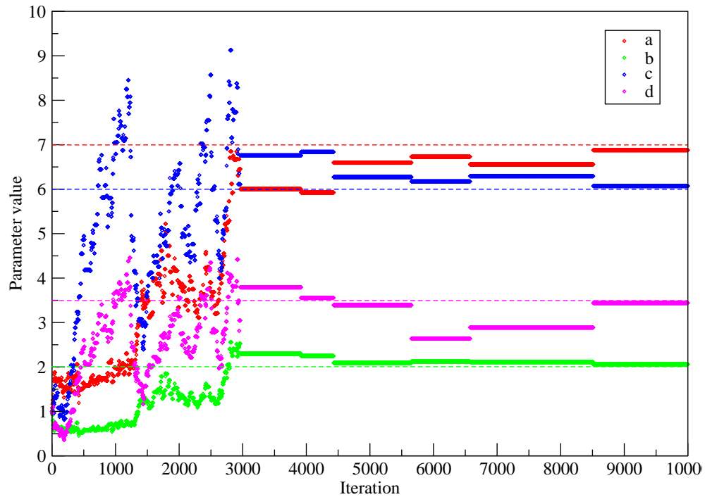
Figure 4.5: MPMC results of the Lotka-Volterra validation run. Note the initial burn-in period followed by the distribution trajectory. True parameter values are indicated by dashed lines in matching colours.
