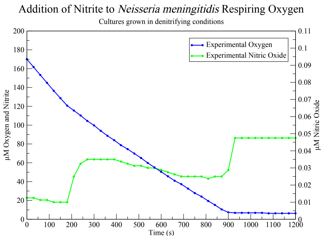
Figure 7.3: Nitrite Reduction in Neisseria meningitidis . This dataset shows the effect of nitrite addition to an aerobically respiring culture. Nitrite is added at 200 s. Oxygen and Nitric Oxide data-points are recorded with much less frequency than in previous datasets hence the inclusion of dots on the plot.
