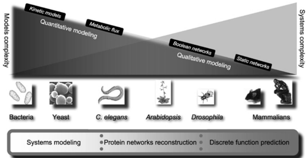
Figure 1.13: System complexity. Diagram showing how system complexity varies across organisms, and how the complexity of the models we can produce is currently the inverse of systems complexity. Kahlem and Birney 80
