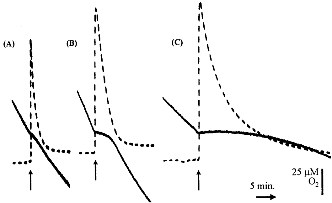
Figure 6.13: Addition of Nitric Oxide to Aerobic Cultures. Figure 5 reproduced from Anjum et al. 29 . Oxygen concentration is represented by solid lines and nitric oxide by dashed lines. a) Addition to wild-type culture, b) Addition to cycP mutant, c) Addition to norB mutant.
