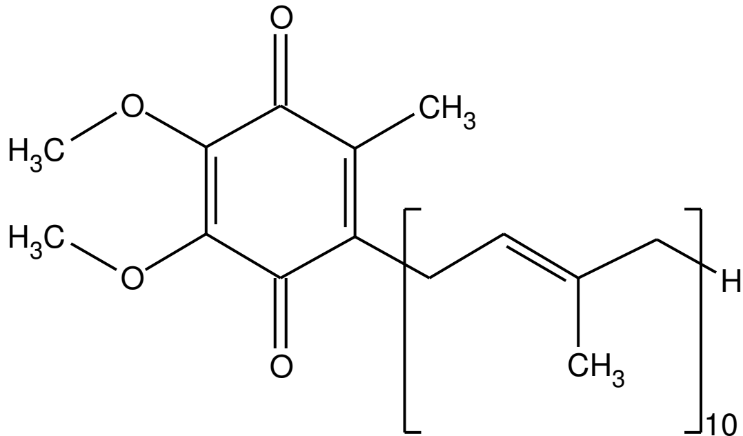
Figure 1.7: Structure of the ubiquinone molecule.
