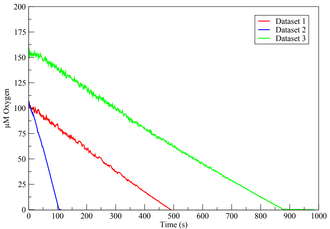
Figure 5.4: Oxygen Reduction in Neisseria meningitidis . These three experimental datasets were used as input data for the parameter estimation algorithm. They all show the same linear oxygen reduction. The different rates are due to differing starting cell densities. The specific rates are very similar at 1.5 \mu\text{Ms}^{-1} per OD unit.
