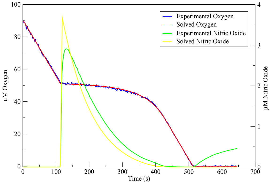
Figure 6.11: Nitric Oxide Reduction in Neisseria meningitidis . This figure shows the third attempt at fitting the model to experimental data using priors determined from literature values in addition to manually adjusted priors. Oxygen reduction is being modelled remarkably well, whereas the rate of nitric oxide reduction appears to be slightly too high in the solved output.
