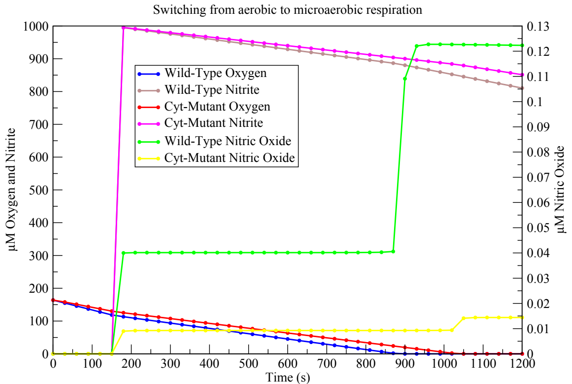
Figure 8.4: In silico Cytochrome Mutant. This figure shows the effect of reducing the total amount of cytochromes while leaving all other components unchanged. All the reaction rates have slowed as a result of this change.
