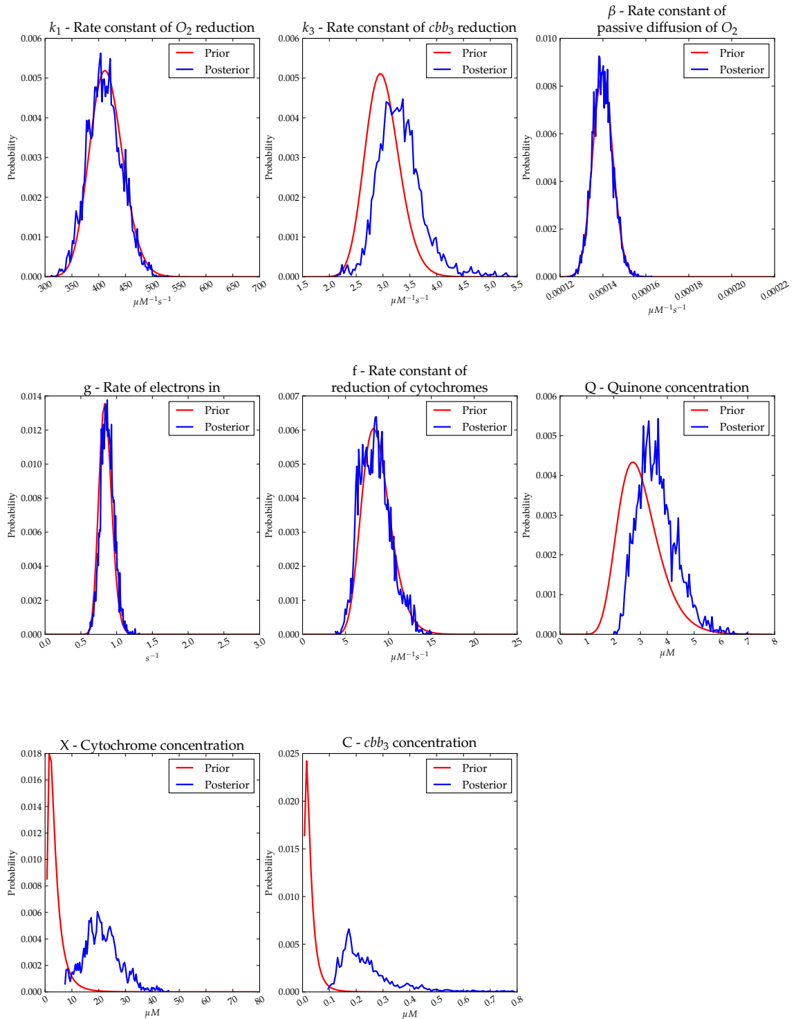
Figure 5.11: Oversampled Posterior Distributions. The posterior probability distributions for dataset 1 of oxygen reduction are oversampled from the prior probability distributions. This is not directly obvious by the probability distributions alone, but in conjunction with the input dataset which lacks features present in datasets 2 and 3. In this case both k_1 and k_3 are skewed towards the prior probability distributions, and this causes the distribution of C to be very wide as it can take a very broad range of values without affecting the goodness of fit of the simulated data to the experimental data.
