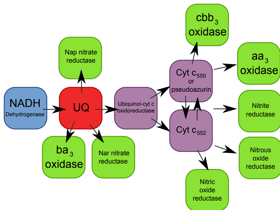
Figure 1.9: Branched electron transport chains of Paracoccus species. Blue denotes initial electron donor, red denotes quinone pool, purple denotes cytochrome electron transporters and green denotes terminal reductases. UQ = ubiquinone. Electron transfer between cytochromes c_{552} and c_{550} has not been demonstrated experimentally but is possible, given the redox potential of the proteins. Adapted from Baker et al. 73 .
