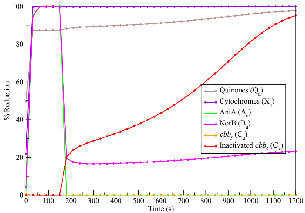
Figure 7.8: Reduction States During Nitrite Reduction. This figure shows how the reduction states of the enzymes involved in nitrite reduction change during respiration.
