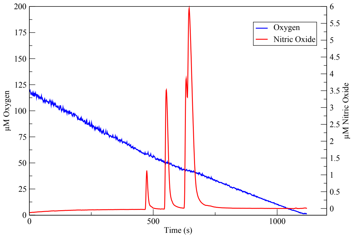
Figure 8.2: Nitric Oxide Reduction in an nsrR^- Mutant. This figure shows nitric oxide and oxygen reduction in an aniA^-nsrR^- mutant. In this case the aniA^- mutation has no effect as no nitrite is being reduced. Addition of nitric oxide has only a very small effect on the rate of oxygen reduction as it is being removed very quickly by the constitutively expressed NorB.
