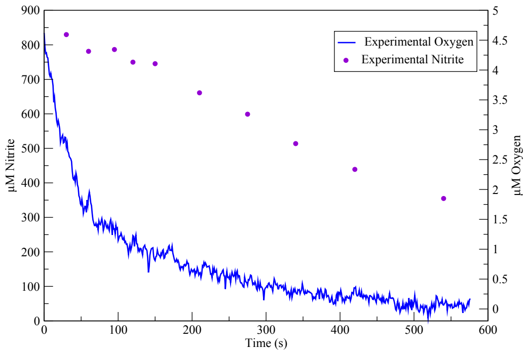
Figure 7.2: Nitrite Reduction in Neisseria meningitidis . This dataset shows the effect on oxygen respiration of nitrite respiration as nitric oxide is produced. This culture is an nsrR^- mutant which is expressing AniA and NorB in an essentially constitutive manner.
