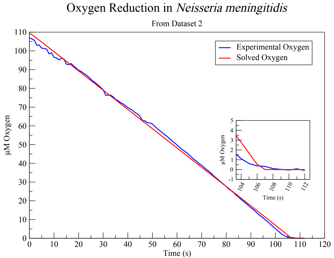
Figure 5.6: Oxygen Reduction in Neisseria meningitidis . This dataset shows the simple linear reduction of Oxygen in aerobic conditions. The high affinity of cbb_3 for oxygen is evidenced by very little non-linearity at low oxygen concentrations. The solved output is a representative result of the parameter estimation system. The inset shows that the solved output is achieving much higher affinity than the experimental data.
