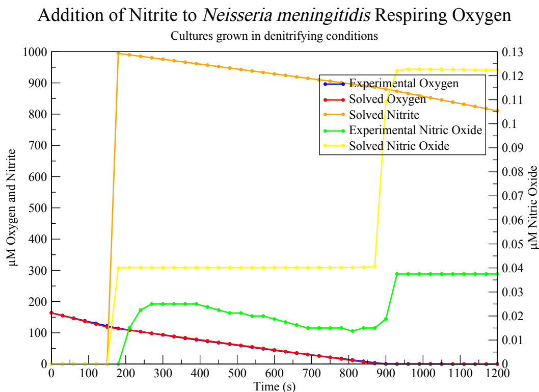
Figure 7.10: Effect of Nitrite Addition on Aerobically Respiring Cultures. This figure shows the second attempt at fitting the model to experimental data. Oxygen respiration appears to be modelled well. Nitric oxide production is being modelled well qualitatively, as the major features of the experimental data are present. Clearly though further rounds of parameter estimation are in order to improve the quantitative fit.
