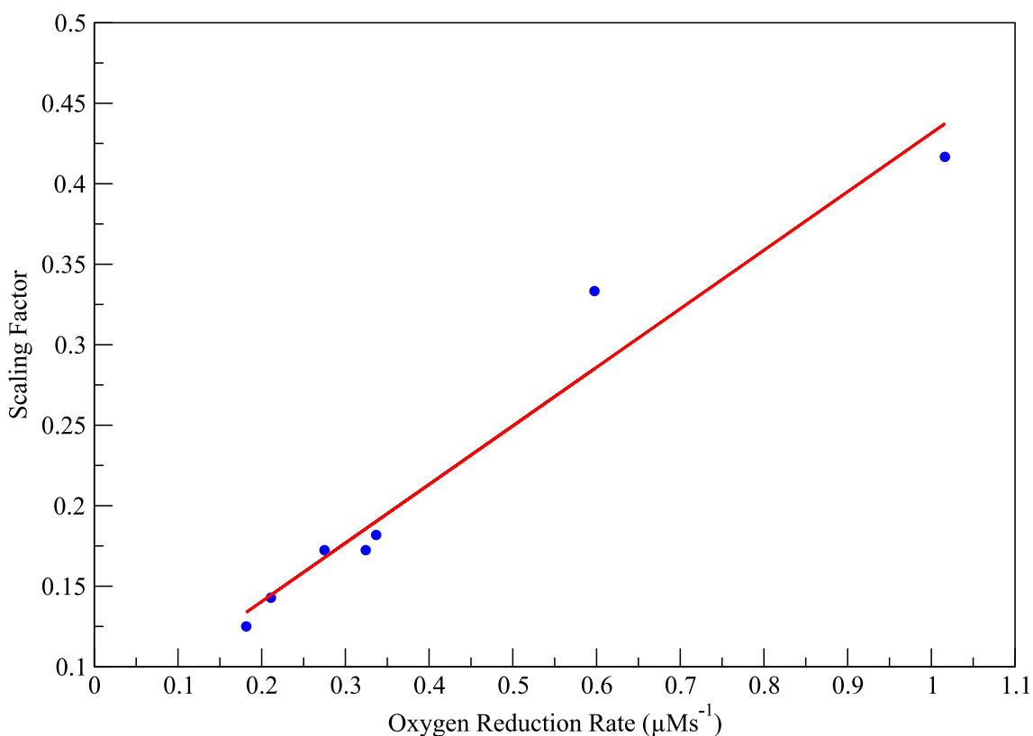
Figure 8.7: Dataset Scaling Factors. This figure shows the magnitude of the scaling factor relative to the experimental oxygen reduction rates. The red lines indicates a linear regression through the datapoints.
