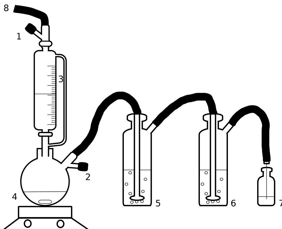
Figure 2.3: NO making apparatus. 1 & 2 - N_2 release valves. 3 - Pressure equalizing dropping funnel, containing 50 ml 4 M H_2SO_4 . 4 - Stirred, round-bottomed flask, containing 200 ml 2 M NaNO_2 . 5 - Dreschel bottle with sintered bulb, containing \approx 200 ml 1 M NaOH ( \frac{2}{3} full). 6 - Dreschel bottle with sintered bulb, containing \approx 200 ml dH_2O ( \frac{2}{3} full). 7 - Small glass bottle with rubber septum and needle entry valve, containing dH_2O \frac{2}{3} full. This bottle either needs to also have a gas exit needle, or at least not be sealed during the process.. 8 - To N_2 gas bottle. Viton rubber tubing is used for all the flexible hoses in this apparatus.
