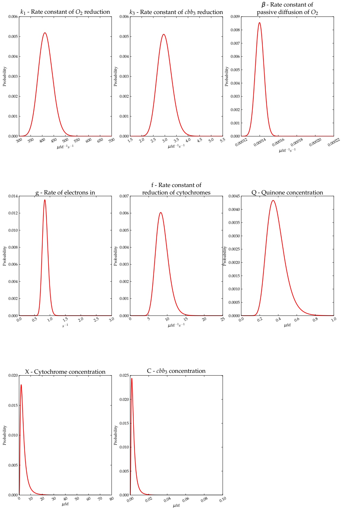
Figure 5.5: Prior probability distributions for oxygen reduction. These are the probability distributions used as priors by the parameter estimation algorithm.
