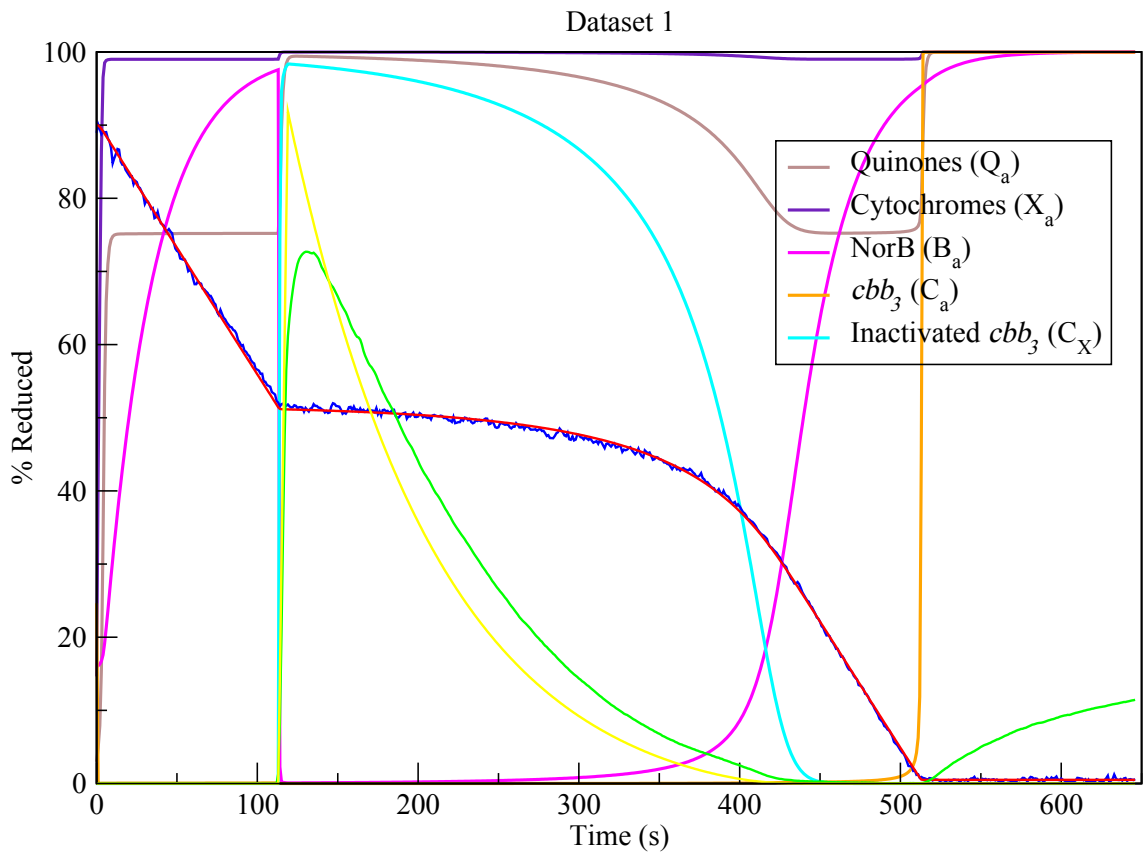
Figure 6.15: Reduction States During Nitric Oxide Reduction. This figure shows how the reduction states of the enzymes involved in respiration changes as the culture respire oxygen and then nitric oxide. The experimental and solved observed data are shown as thinner lines for reference.
