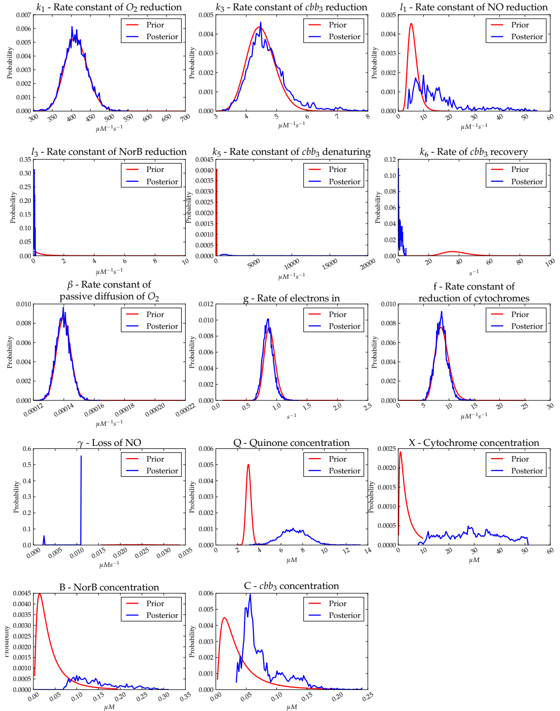
Figure 6.12: Posterior Distributions for Datasets 1 and 4. The posterior probability distributions for datasets 1 and 4 of nitric oxide removal.
