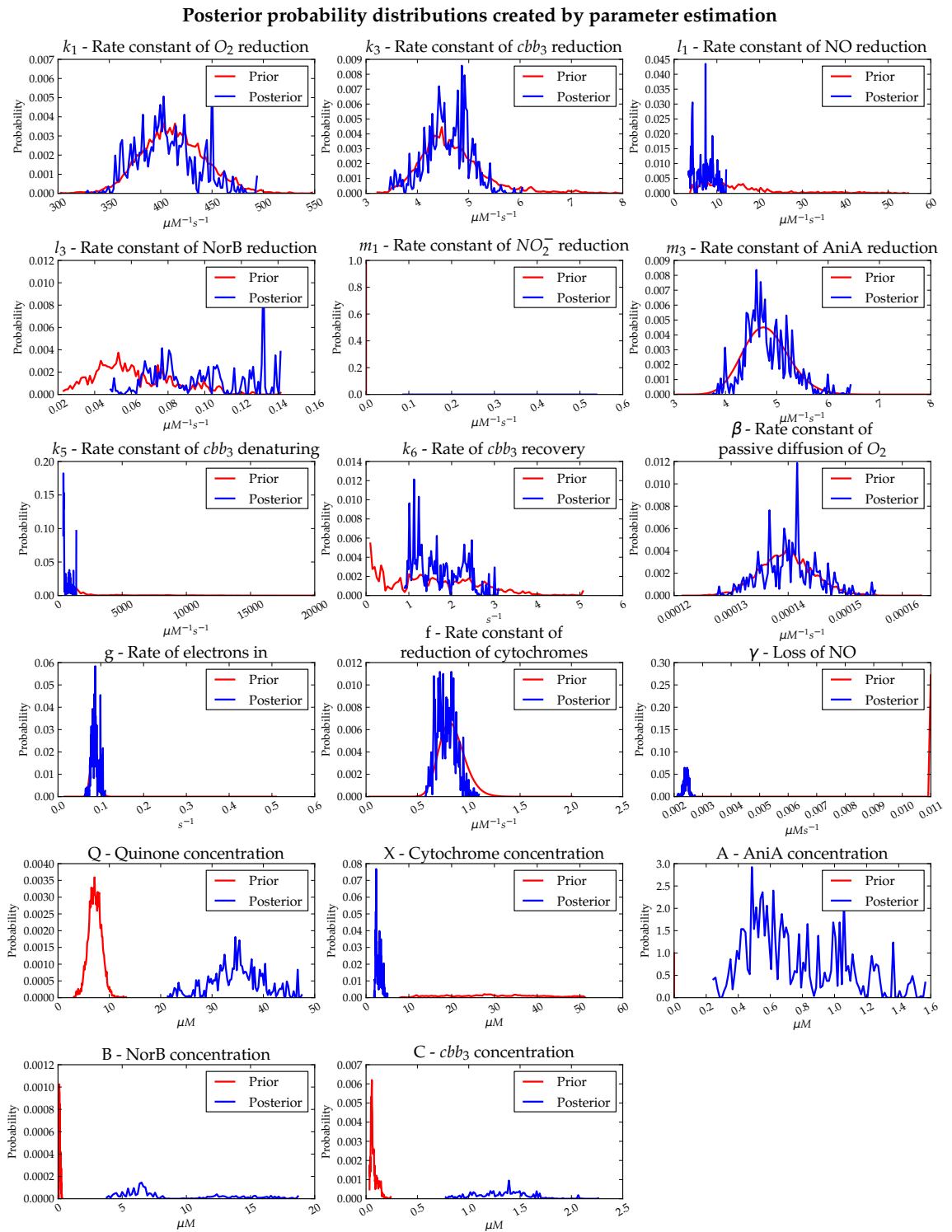
Figure 7.12: Posterior probability distributions for microaerobic oxygen and nitrite reduction. These are the final posterior probability distributions generated by the parameter estimation system for microaerobic oxygen and nitrite reduction, all concentrations have been normalised to assume an OD_{600} of 1.
