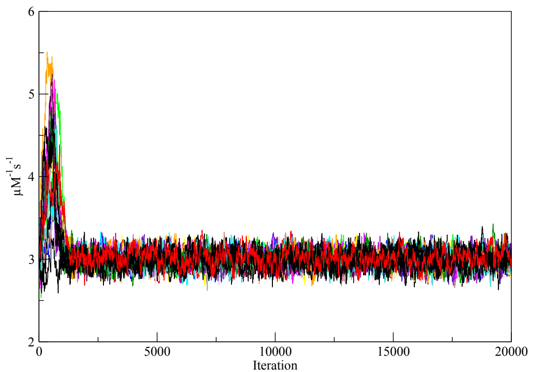
Figure 5.8: Individual parameter trajectories for multiple runs on the same experimental dataset. This figure shows the trajectories for the same parameter, in this case k_3 - the rate constant for ccb_3 reduction, from 20 individual runs of parameter estimation upon the same input data. The trajectories show clear convergence after the “burn-in” period.
