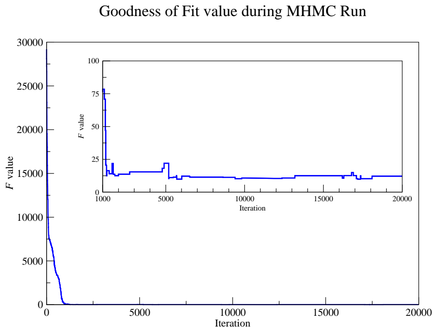
Figure 5.7: Simulation F value improves as parameter estimation progresses. This is a representative figure constructed from a single run on one dataset. Initially the F value is high showing that the simulated result does not match the experimental dataset. As the parameter estimation algorithm progresses, the F value decreases as the simulated result approaches the experimental dataset. The inset shows a zoomed in view of the F value after the “burn-in” process has finished.
