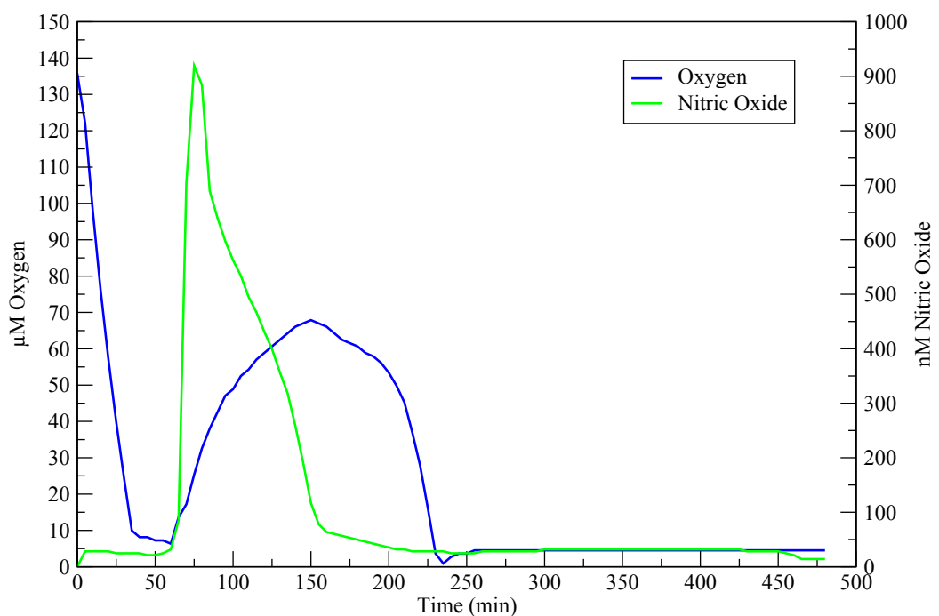
Figure 9.2: Effect of Expression of AniA and NorB. This figure shows an aerobically respiring culture in media with nitrite present. When oxygen is depleted, AniA and NorB begin to be expressed causing an increase and then decrease of NO. While NO is being reduced, Oxygen concentration slowly rises due to diffusion, and begins to be reduced once more when NO is depleted. Data from Rock et al. 20 .
