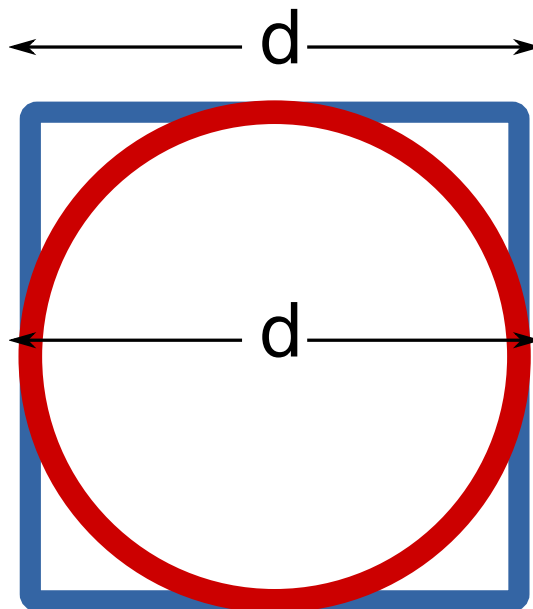
Figure A.1: Circle circumscribed by a square. A Circle of diameter d inside a square of side d .
