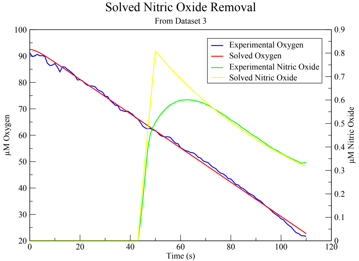
Figure 6.9: Nitric Oxide Reduction in Neisseria meningitidis . This figure shows the second attempt at fitting the model to experimental data using priors determined from literature values in addition to manually adjusted priors. Oxygen reduction is modelled almost perfectly, and the shape of the nitric oxide reduction curve is captured well also.
