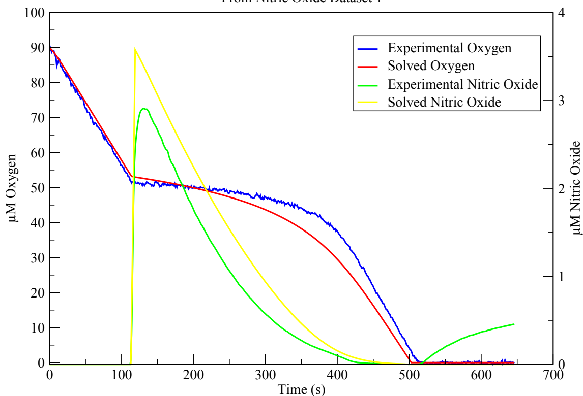
Figure 8.6: Improved Fit with Scaling Factor. This figure shows the best fit achieved using a scaling factor rather than an approximate OD to calculate component concentrations. Compare with 7.14.
