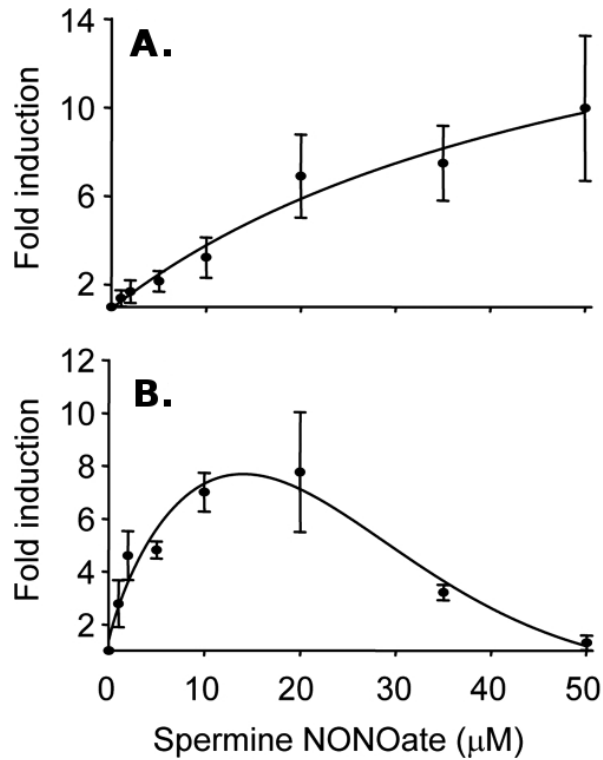
Figure 9.1: Effect of Nitric Oxide on NsrR and FNR Dependent Gene Expression. Expression of (A) NorB and (B) AniA in wild-type Neisseria meningitidis . Figure adapted from Heurlier et al. 30 .
