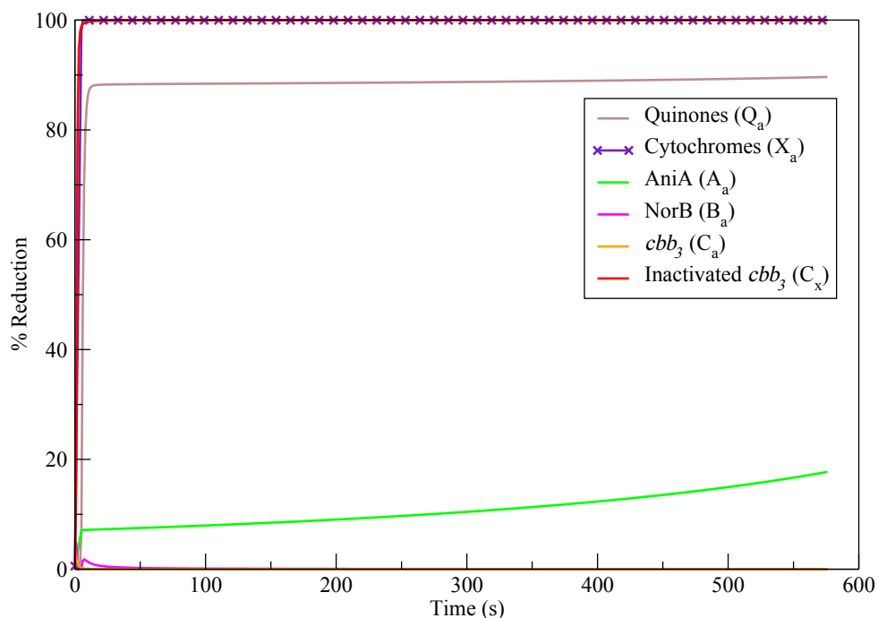
Figure 7.6: Reduction States During Nitrite Reduction. This figure shows how the reduction states of the enzymes involved in nitrite reduction change during respiration.
