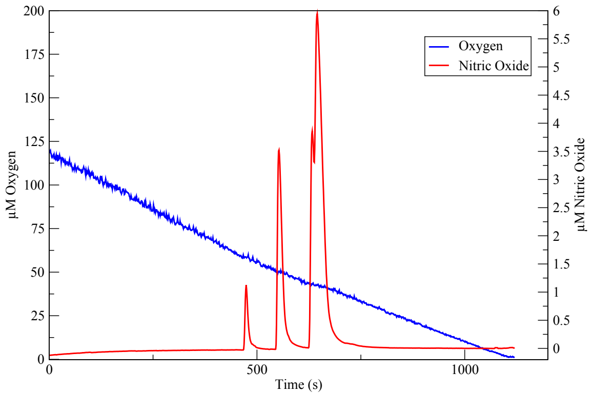
Figure 6.16: Nitric Oxide Reduction in an nsrR - Mutant. This figure shows nitric oxide and oxygen reduction in an aniA - nsrR - mutant. In this case the aniA - mutation has no effect as no nitrite is being reduced. Addition of nitric oxide has only a very small effect on the rate of oxygen reduction as it is being removed very quickly by the constitutively expressed NorB.
