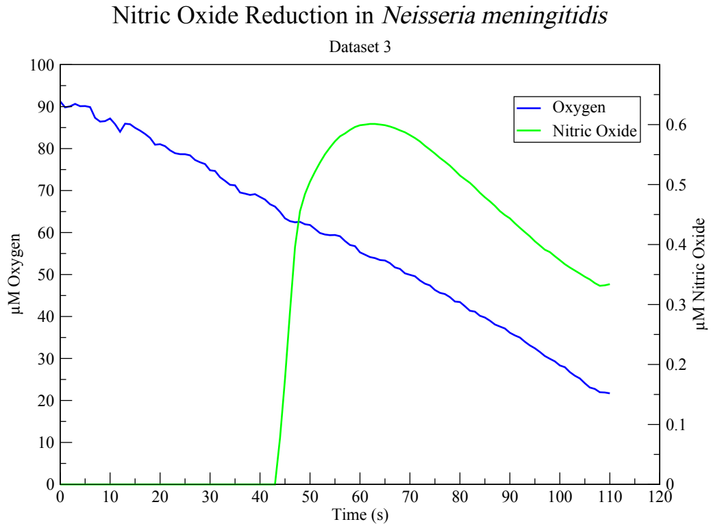
Figure 6.4: Nitric Oxide Reduction in Neisseria meningitidis . This dataset shows the effect on rate of oxygen reduction as a small amount of nitric oxide (to \approx 0.6 \mu\text{M} ) is introduced to the respiring system.
