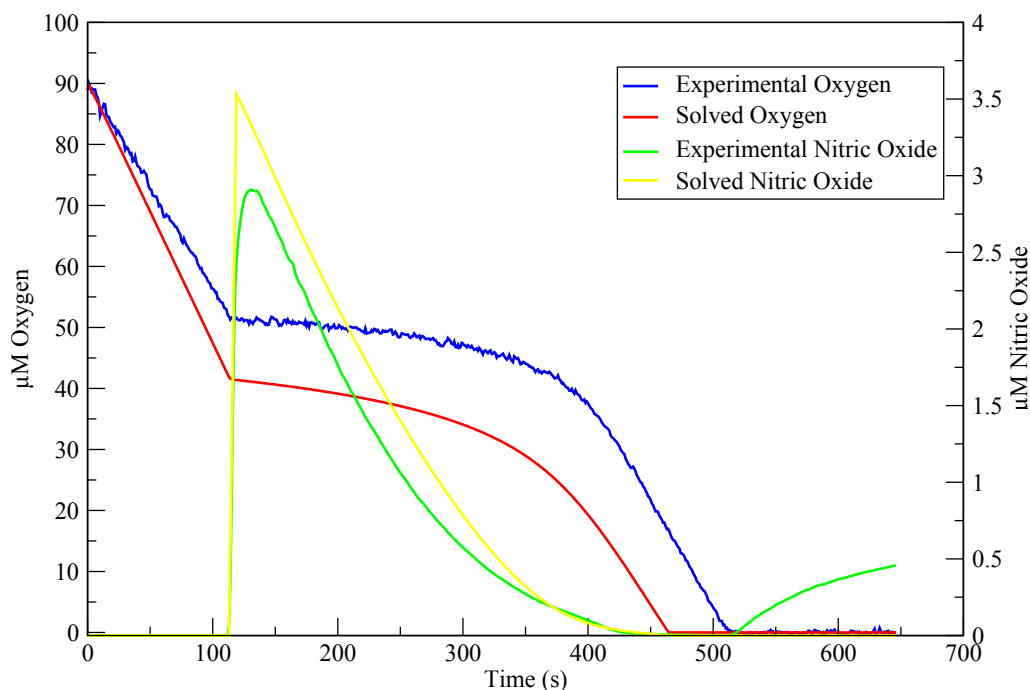
Figure 7.14: Aerobic Oxygen Respiration with Nitric Oxide Addition with Nitrite Posteriors. This figure shows the simulation results using the posteriors from nitrite parameter estimation with appropriately scaled concentrations. The concentration of NorB ( B ) had to be reduced significantly to obtain a similar nitric oxide reduction rate, and the value of k_5 had to be increased 66x to create a similarly shaped oxygen reduction curve.
