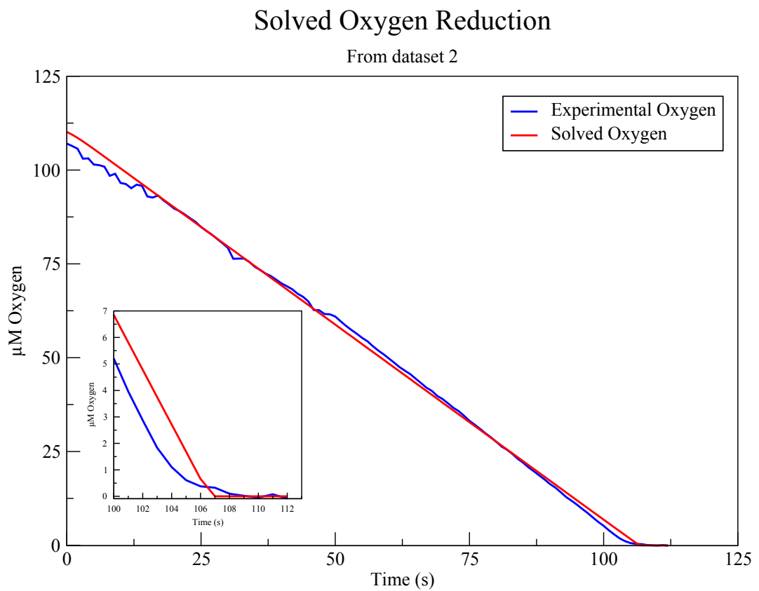
Figure 5.13: Oxygen Reduction in Neisseria meningitidis . This figure shows how well the best simulated data fits against the experimental data from dataset 2. The inset shows again, that the solved output is achieving much higher affinity than the experimental data.
