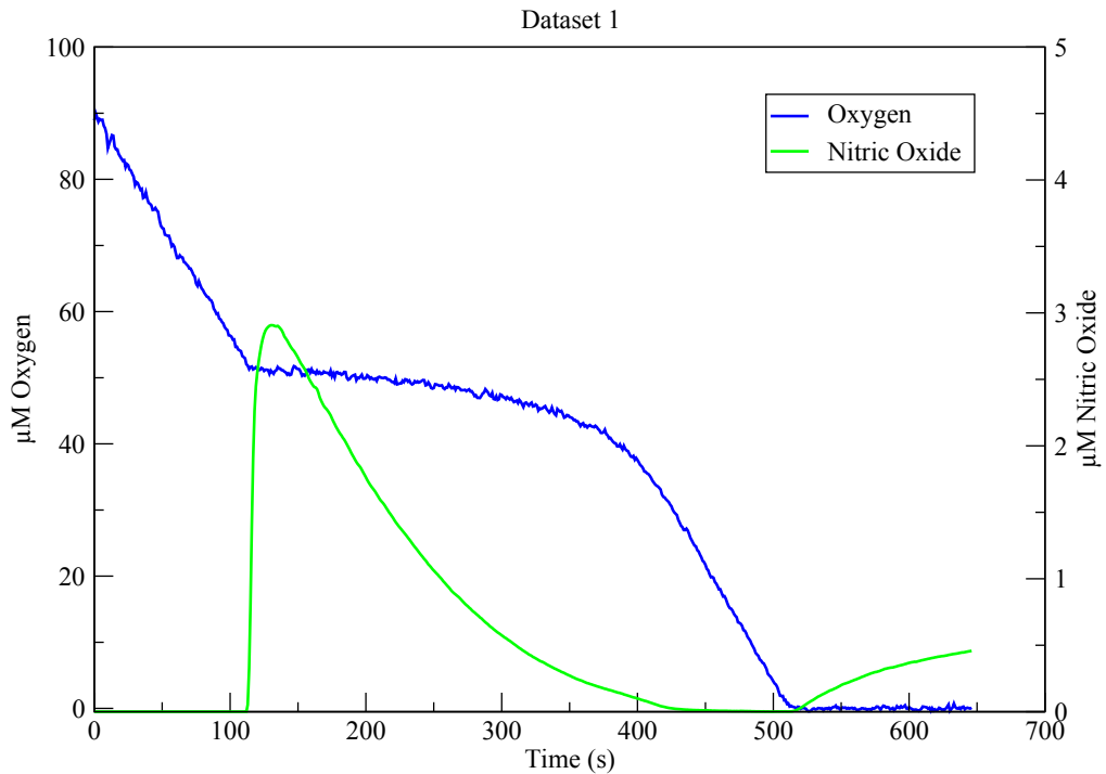
Figure 6.2: Nitric Oxide Reduction in Neisseria meningitidis . This dataset shows the effect on rate of oxygen reduction as nitric oxide (to \approx 3 \mu\text{M} ) is introduced to the respiring system which also appears to have been partially primed for nitric oxide reduction. Note that the increase in nitric oxide concentration seen at the end of the dataset is most likely due to drift in the electrode.
