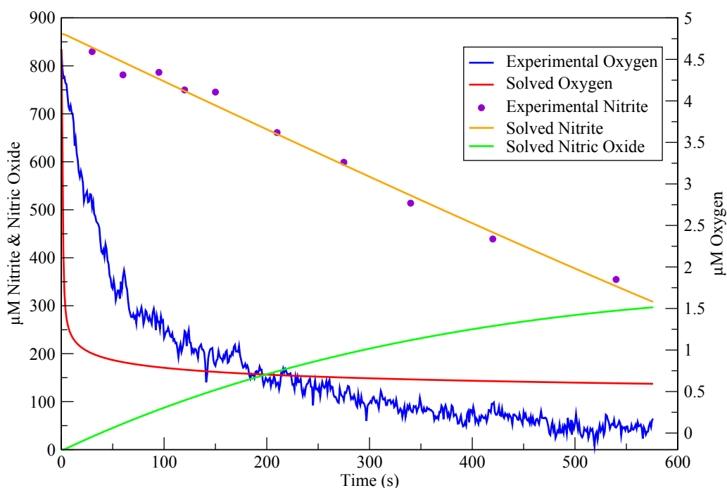
Figure 7.5: Solved Nitrite Reduction in Neisseria meningitidis . This figure shows the first attempt at fitting the model to experimental data. Nitrite reduction is being modelled well, whereas oxygen reduction is being modelled quite poorly as the solved data shows to high a rate of oxygen reduction. Nitric oxide is solved purely as a product of nitrite reduction and is not compared to any experimental data.
