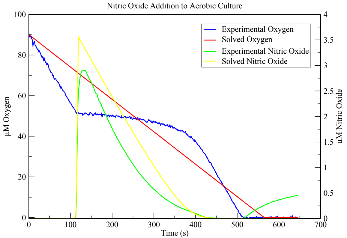
Figure 6.8: Nitric Oxide Reduction in Neisseria meningitidis . This figure shows the first attempt at fitting the model to experimental data using priors determined from literature values. Nitric oxide disappearance is now being modelled much more accurately than in Figure 6.7. Oxygen reduction is not being modelled correctly and the best fitting parameters generate a straight line rather than capturing the stopping and restarting of oxygen reduction.
