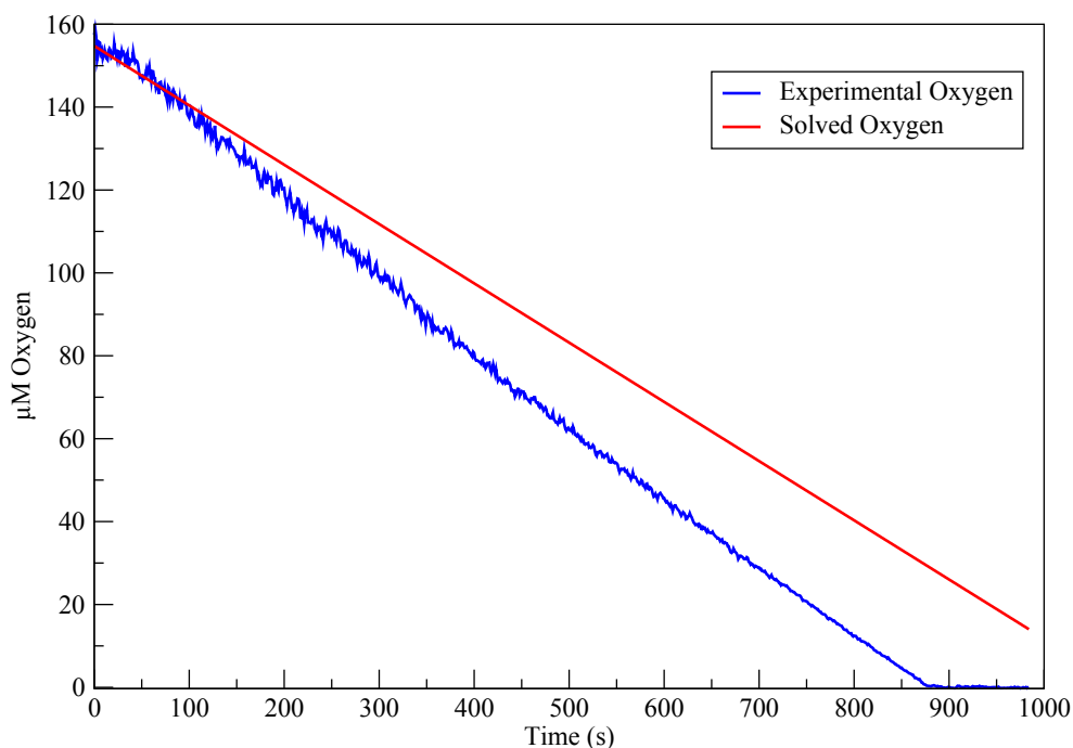
Figure 7.13: Aerobic Oxygen Respiration with Nitrite Posteriors. This figure shows the simulation results using the posteriors from nitrite parameter estimation with appropriately scaled concentrations.
