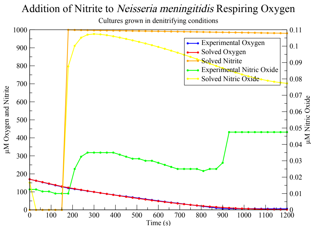
Figure 7.7: Effect of Nitrite Addition on Aerobically Respiring Cultures. This figure shows the first attempt at fitting the model to experimental data. Oxygen respiration appears to be modelled quite well, but nitric oxide is being modelled particularly badly. The most significant feature of the nitric oxide dataset is absent in the solved data.
