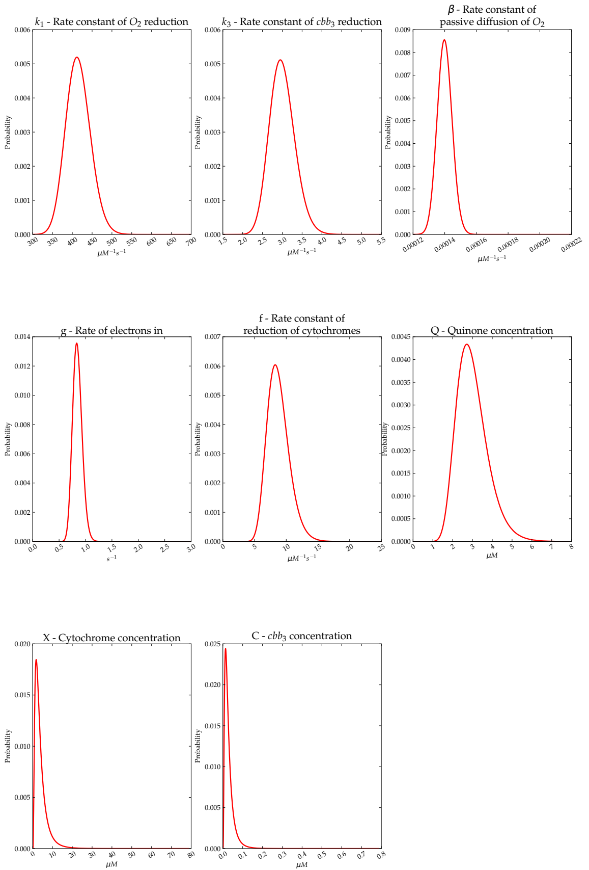
Figure 5.10: Prior probability distributions for oxygen reduction. These are the probability distributions used as priors by the parameter estimation algorithm.
