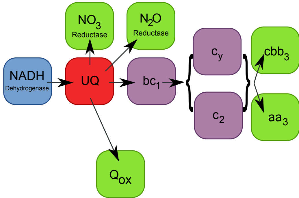
Figure 1.11: Branched electron transport chains of Rhodobacter sphaeroides . Blue denotes initial electron donor, red denotes quinone pool and green denotes terminal reductases. UQ = ubiquinone. This diagram does not include any of the photosynthetic pathways that R. sphaeroides also has. Adapted from Ferguson et al. 77 , Daldal et al. 78 , Pappas et al. 79
