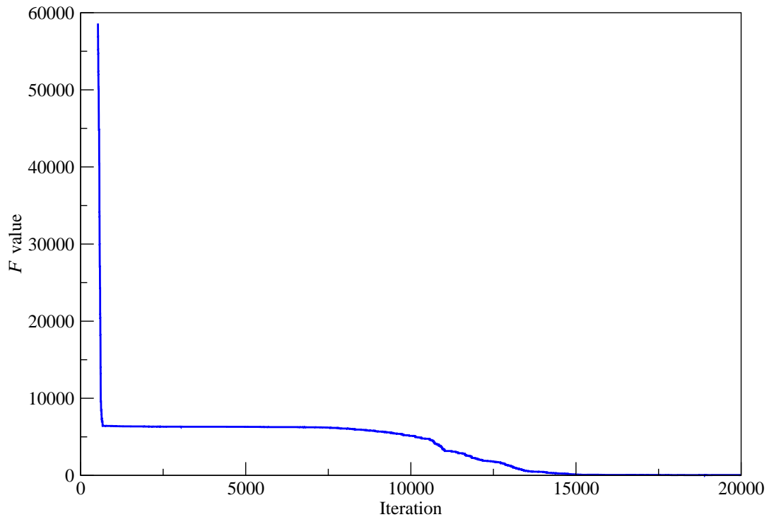
Figure 6.10: Local Fitness Minima During Parameter Estimation. This figure shows the F value as the MHMC progresses on dataset 1. A local fitness minimum is clearly visible at a F value of approximately 7000 where the parameter estimation algorithm has settled on a straight line for oxygen reduction. After a variable number of iterations the MHMC run exits the local fitness minimum and progresses towards a much better fitting set of parameters. This is a typical plot of the F values, however in some runs the fitness minimum is exited much more abruptly rather than the gradual change seen here.
