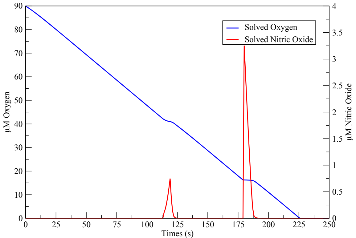
Figure 8.3: Nitric Oxide Addition to In silico nsrR - Mutant. This figure shows the effect of adding two aliquots of increasing concentration of nitric oxide to a simulated nsrR - mutant.
