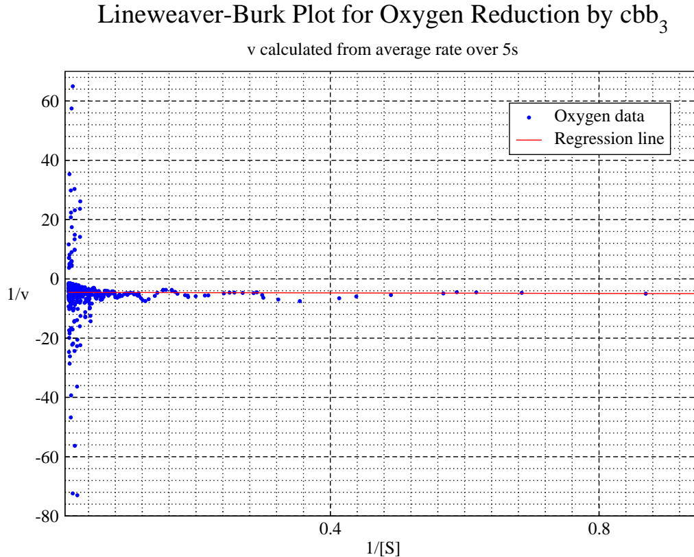
Figure A.2: Lineweaver-Burk Plot for Oxygen Reduction in Neisseria meningitidis . V was calculated as a 5 second rolling average rate to try and smooth out some of the data. The rates are largely negative as oxygen was being removed from the system. The regression line shown is a simple linear regression through all datapoints.
