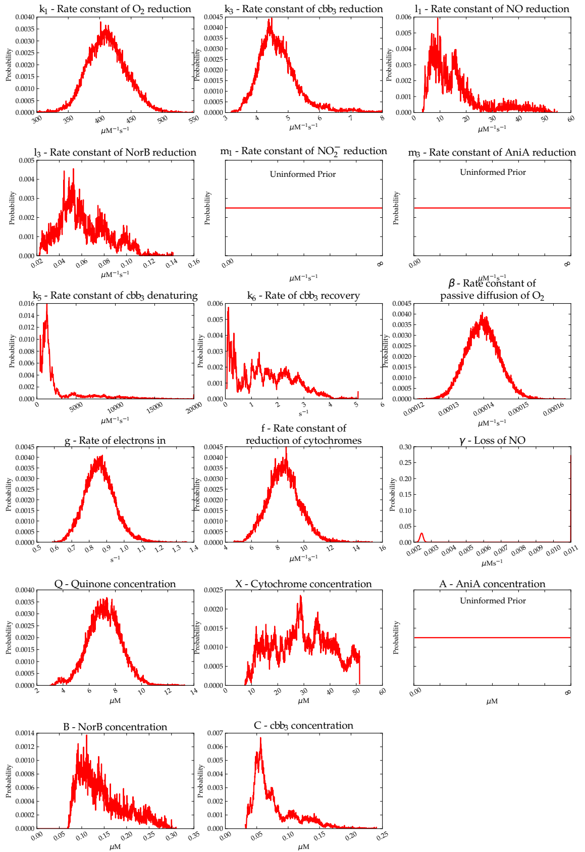
Figure 7.4: Prior probability distributions for microaerobic oxygen and nitrite reduction. These are the probability distributions used as priors by the parameter estimation algorithm.
