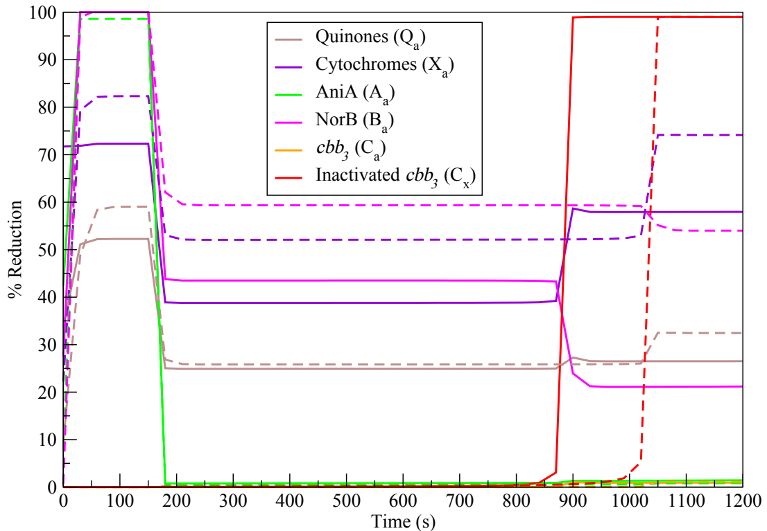
Figure 8.5: In silico Cytochrome Mutant Redox States. This figure shows the effect on the enzymatic reduction states of reducing the total number of cytochromes to simulate a cytochrome knockout mutant. The wild-type is represented by solid lines, and the synthetic mutant by dashed lines.
