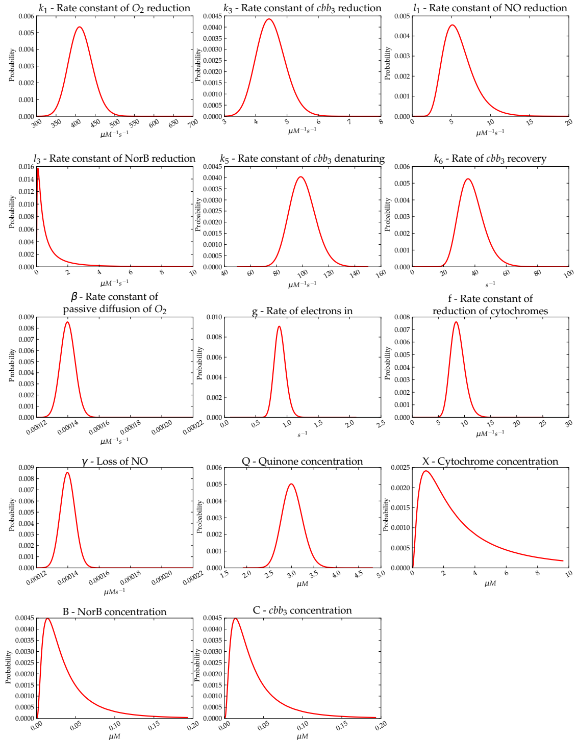
Figure 6.6: Prior probability distributions for aerobic nitric oxide reduction. These are the probability distributions used as priors by the parameter estimation algorithm.
