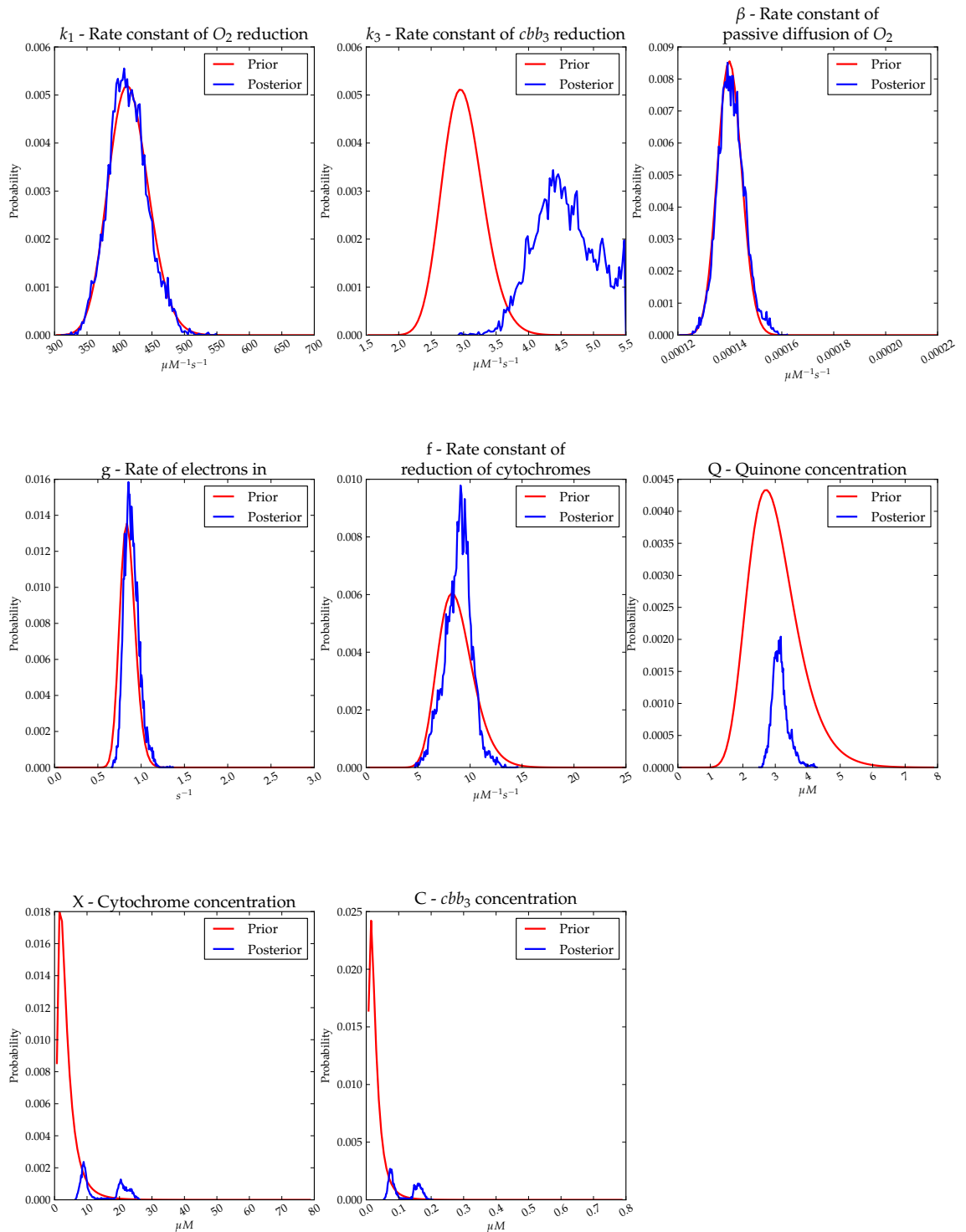
Figure 5.12: Posterior probability distributions for oxygen reduction. These are the probability distributions generated by parameter estimation on 2 oxygen reduction datasets. These have been overlaid onto the prior probability distributions used by the parameter estimation algorithm, also shown in Figure 5.10.
