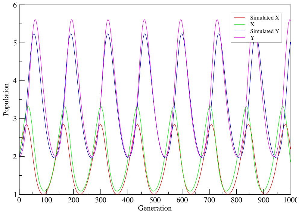
Figure 4.4: Simulation results of the Lotka-Volterra validation run.
