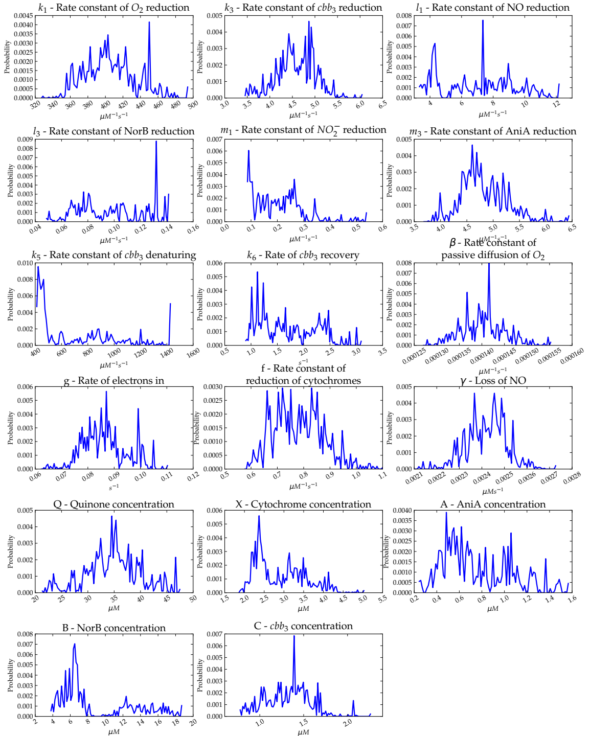
Figure 8.1: Final Posterior probability distributions. These are the final posterior probability distributions generated by the parameter estimation system, all concentrations have been normalised to assume an OD_{600} of 1. Note the value of k_5 will be significantly different from that shown.
