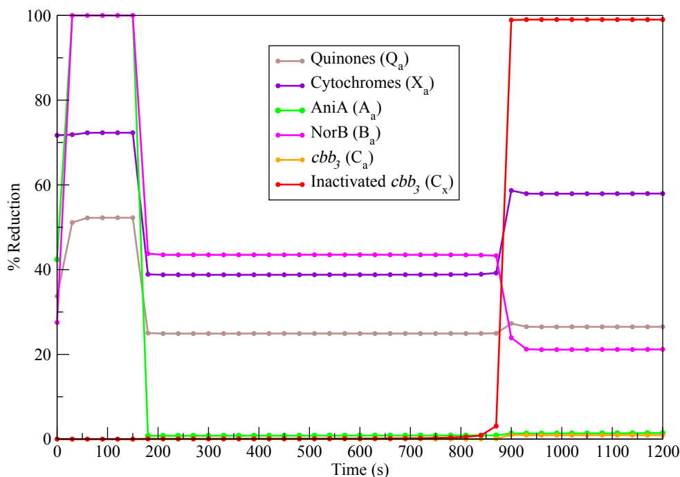
Figure 7.11: Reduction States During Nitrite Reduction. This figure shows how the reduction states of the enzymes involved in nitrite reduction change during respiration.
