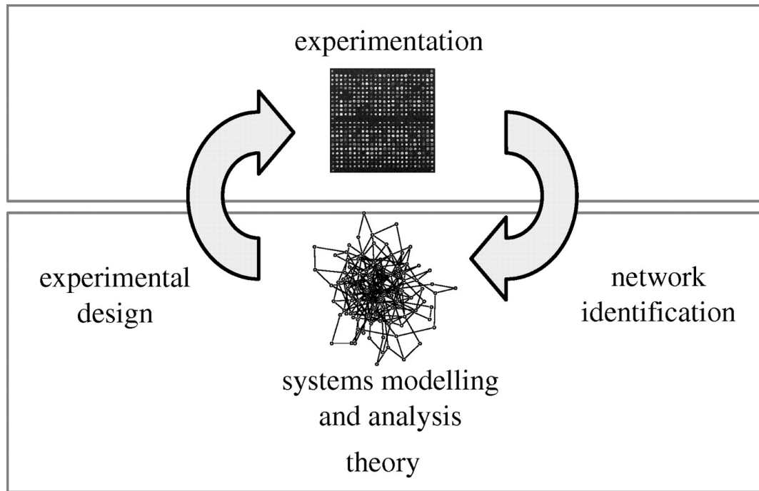
Figure 1.12: Systems biology cycle. Interactions between experimental analysis and theoretical approaches, and the main tasks for theory at the interfaces. Doyle and Stelling 81
