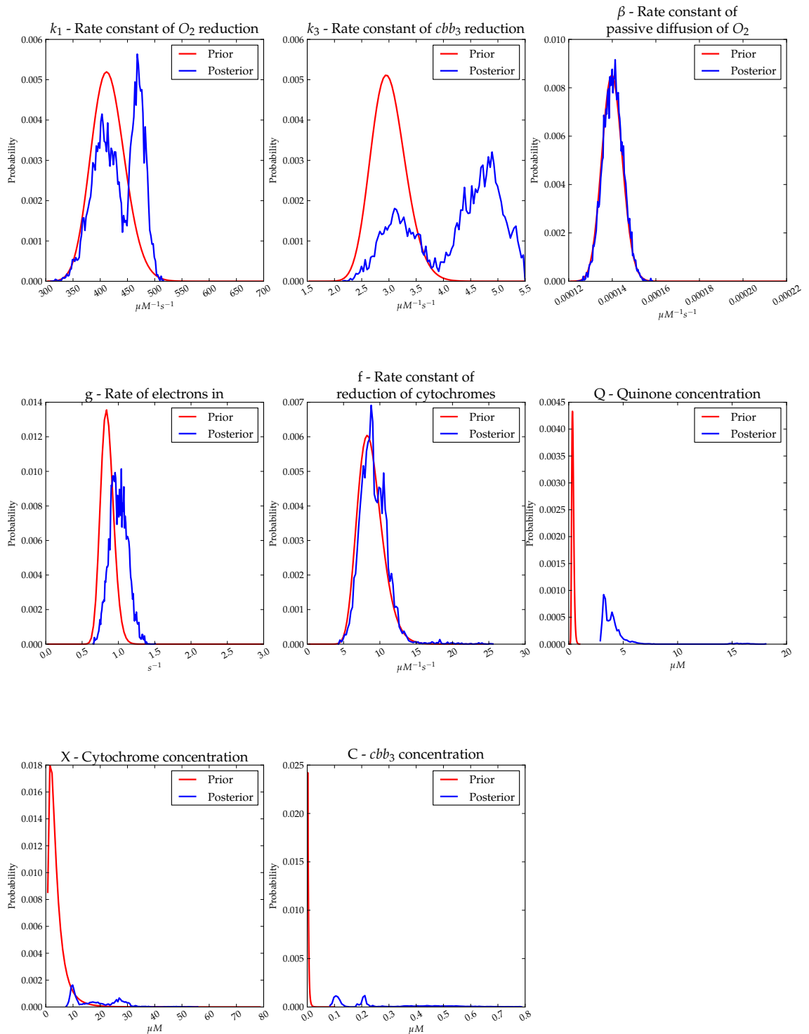
Figure 5.9: Posterior probability distributions for oxygen reduction. These are the probability distributions generated by parameter estimation on 3 oxygen reduction datasets. These have been overlaid onto the prior probability distributions used by the parameter estimation algorithm, also shown in Figure 5.5. The various posterior distributions displayed here are all marginal distributions of a single joint distribution. This applies to all subsequent probability distributions.
