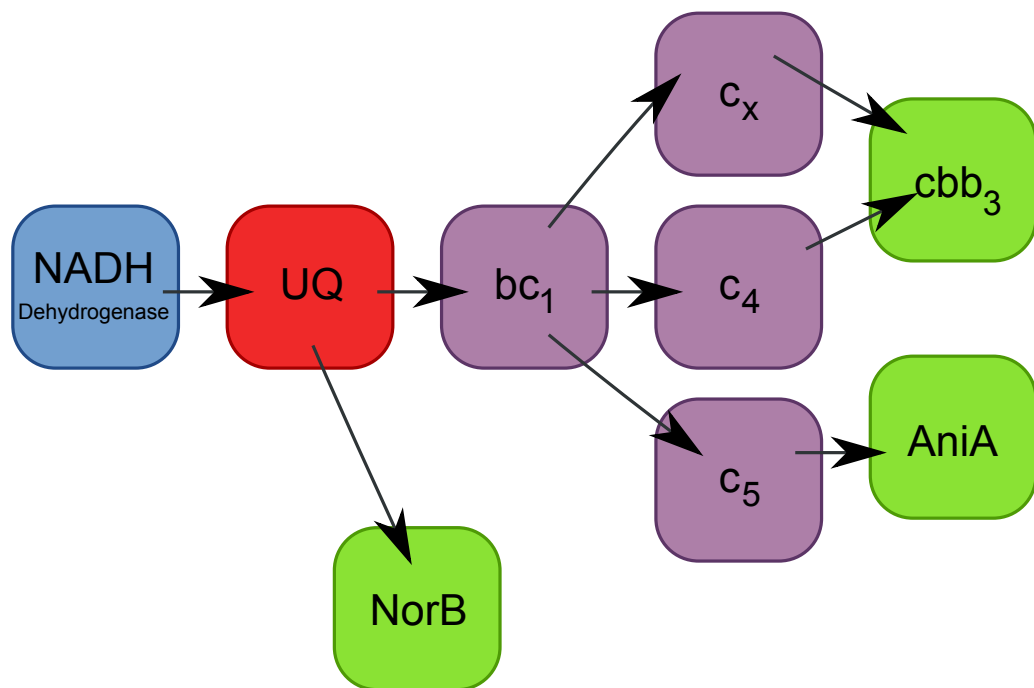
Figure 1.8: Branched electron transport chains of N. meningitidis . Blue denotes initial electron donor, red denotes quinone pool, purple denotes cytochrome electron transporters and green denotes terminal reductases. UQ = ubiquinone.
