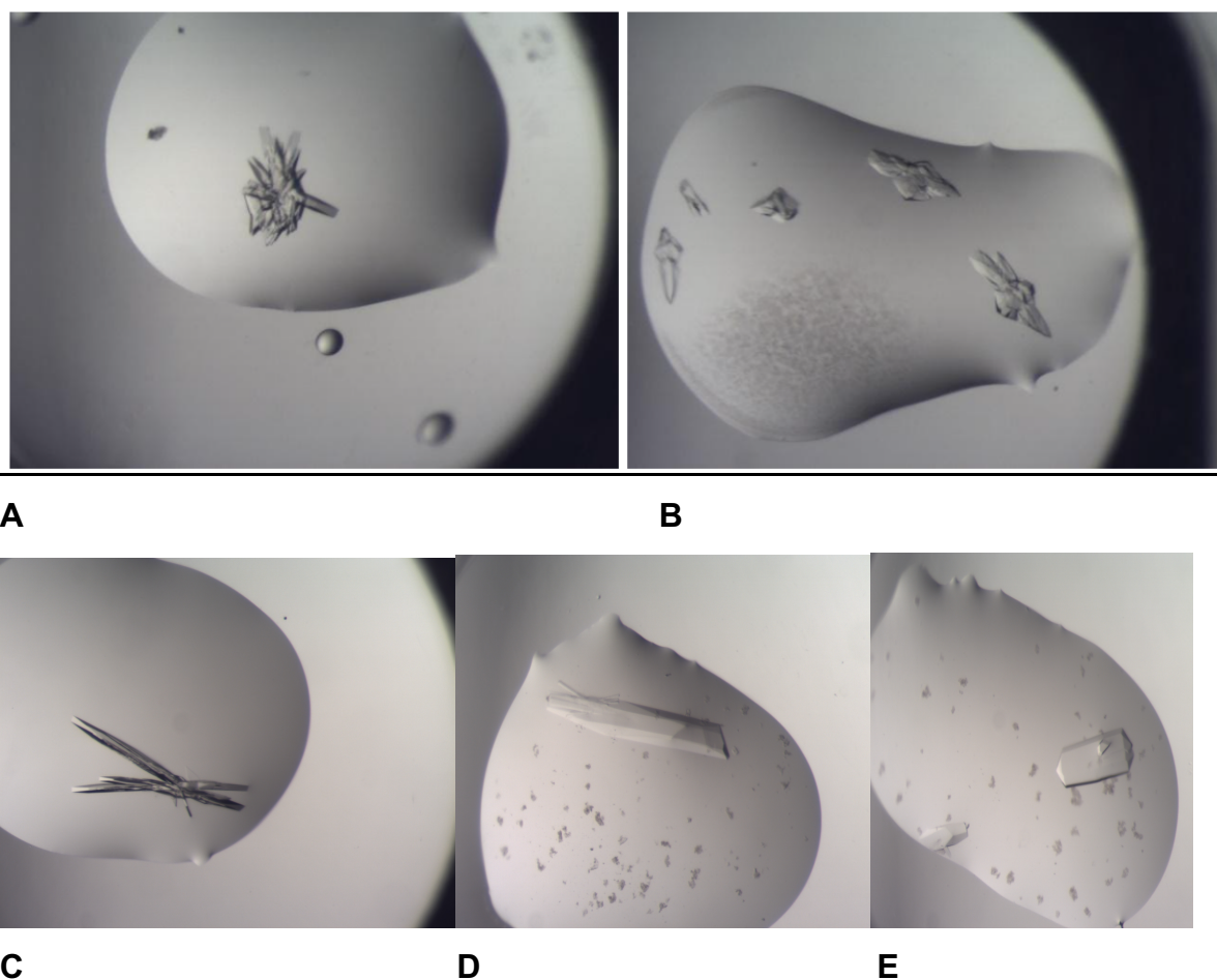
Figure 16- Crystals shown after an INDEX screen A) crystals grown in the A5 condition (0.1 M HEPES pH7.5, 2.0 M ammonium sulphate), B) crystals grown in the A6 condition (0.1 M Tris pH 8.5, 2.0 M Ammonium sulphate), C) crystals grown in A4 condition (0.1M BIS-TRIS pH6.5, 2.0M Ammonium sulfate), D) crystals grown in the F12 (0.2 M Sodium chloride, 0.1 M HEPES pH 7.5, 25% w/v Polyethylene glycol 3,350), condition, E) crystals grown in H12 (0.15 M potassium bromide, 30% w/v polyethylene glycol monomethyl ether 2,000).
