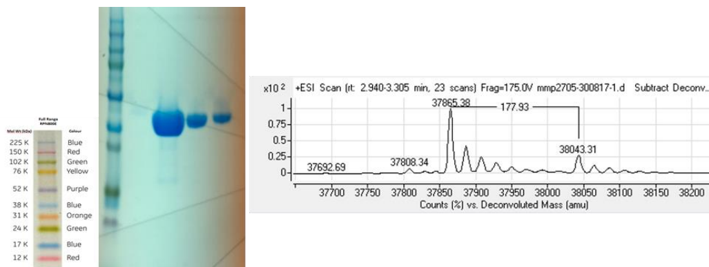
Figure 54. The QC of pure PTP1B(1-301) by SDS-PAGE and HPLC-MS.
