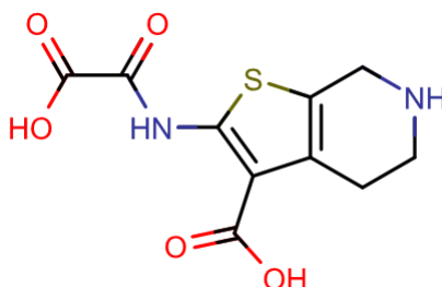
Figure 78. The chemical structure of PTP1B active site-directed inhibitor TCS401.
