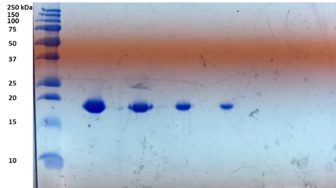
Figure 12. The QC of ^{15}\text{N} -HASPA with SDS-PAGE on 15% polyacrylamide gel.
