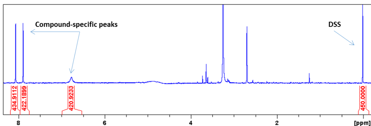
Figure 147. Solubility assessment of a 500 \mu\text{M} fragment by integration using 1D ^1\text{H} NMR and DSS as a reference.
