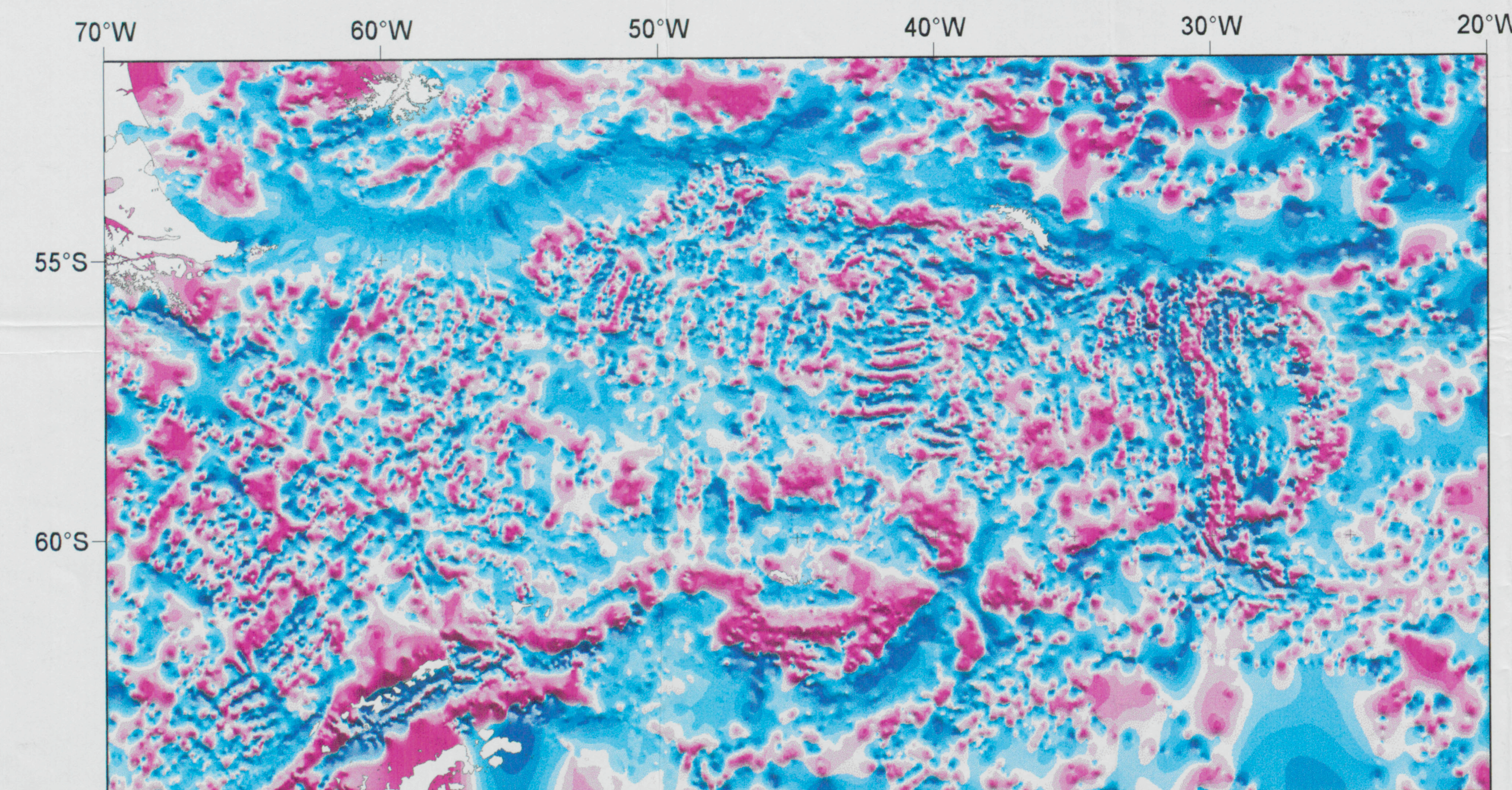
Total field anomaly
