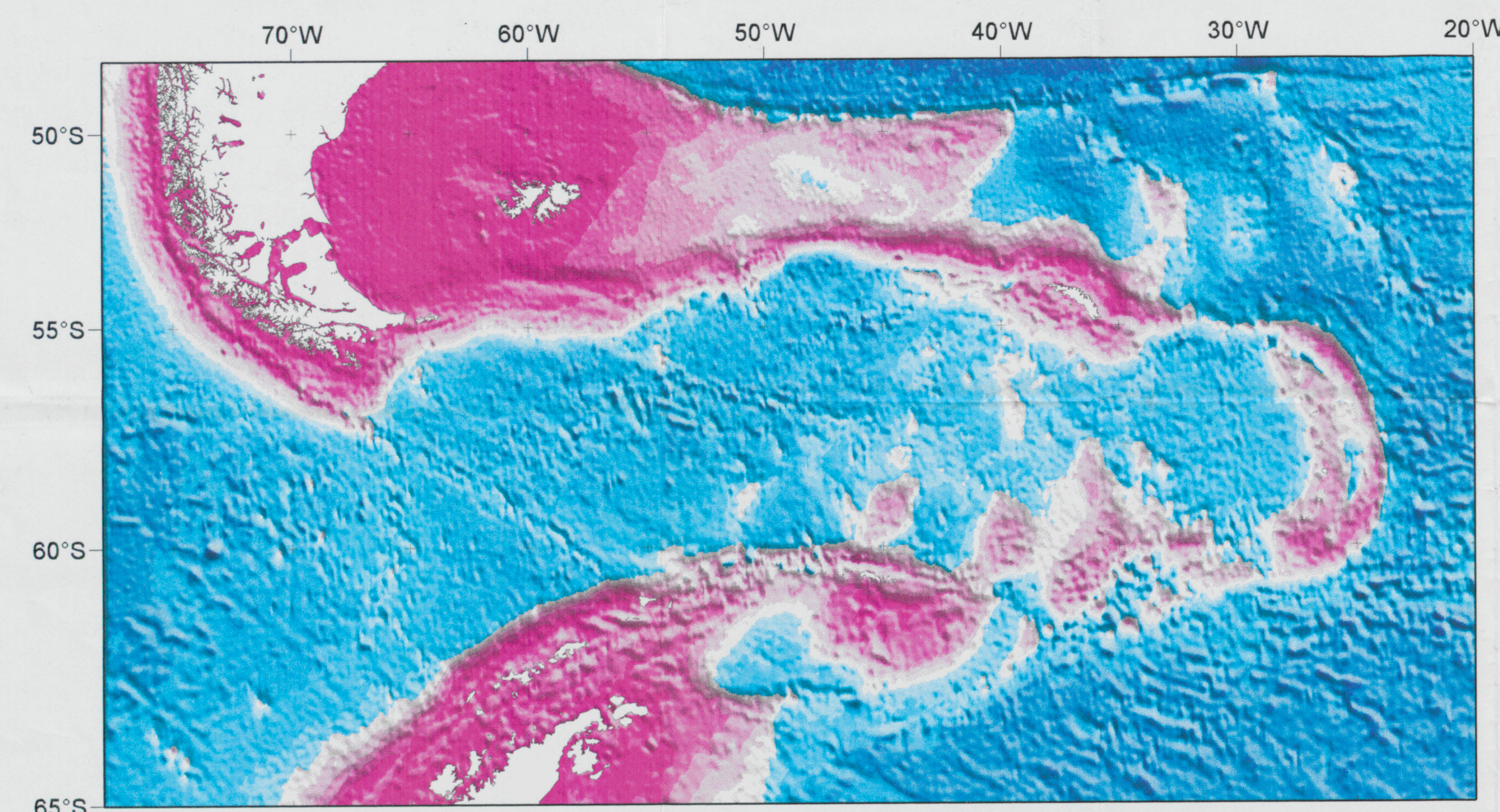
Bouguer anomaly
