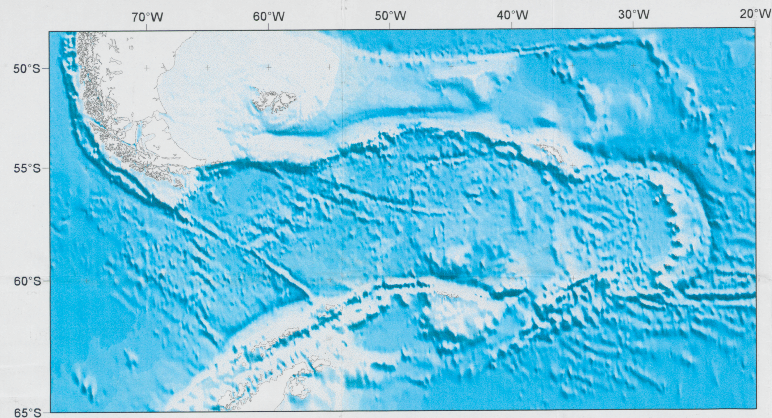
Bathymetry
