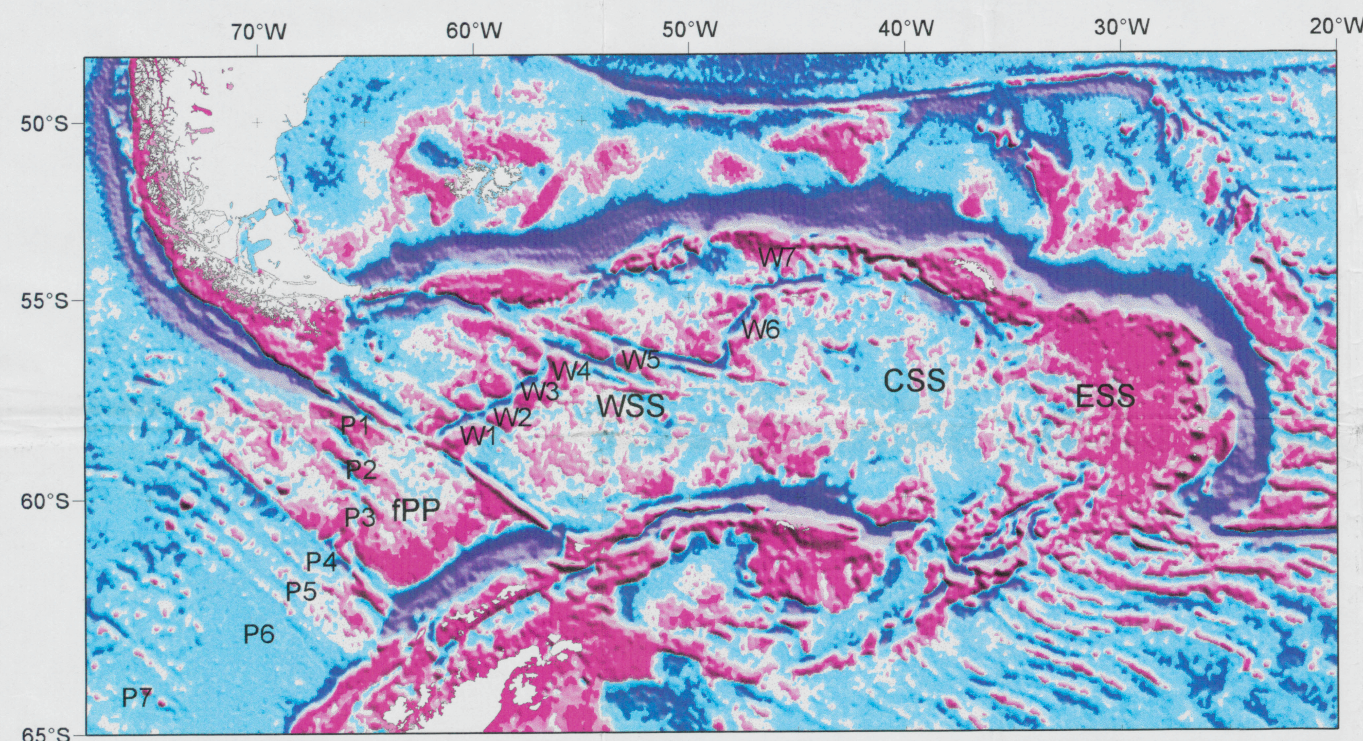
Free-air anomaly
