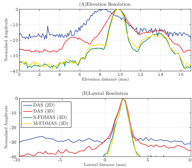
Fig. 5: (A) The point spread function for the carbon fibre rod in the elevation direction and (B) the point spread function for the carbon fibre in the lateral direction.
