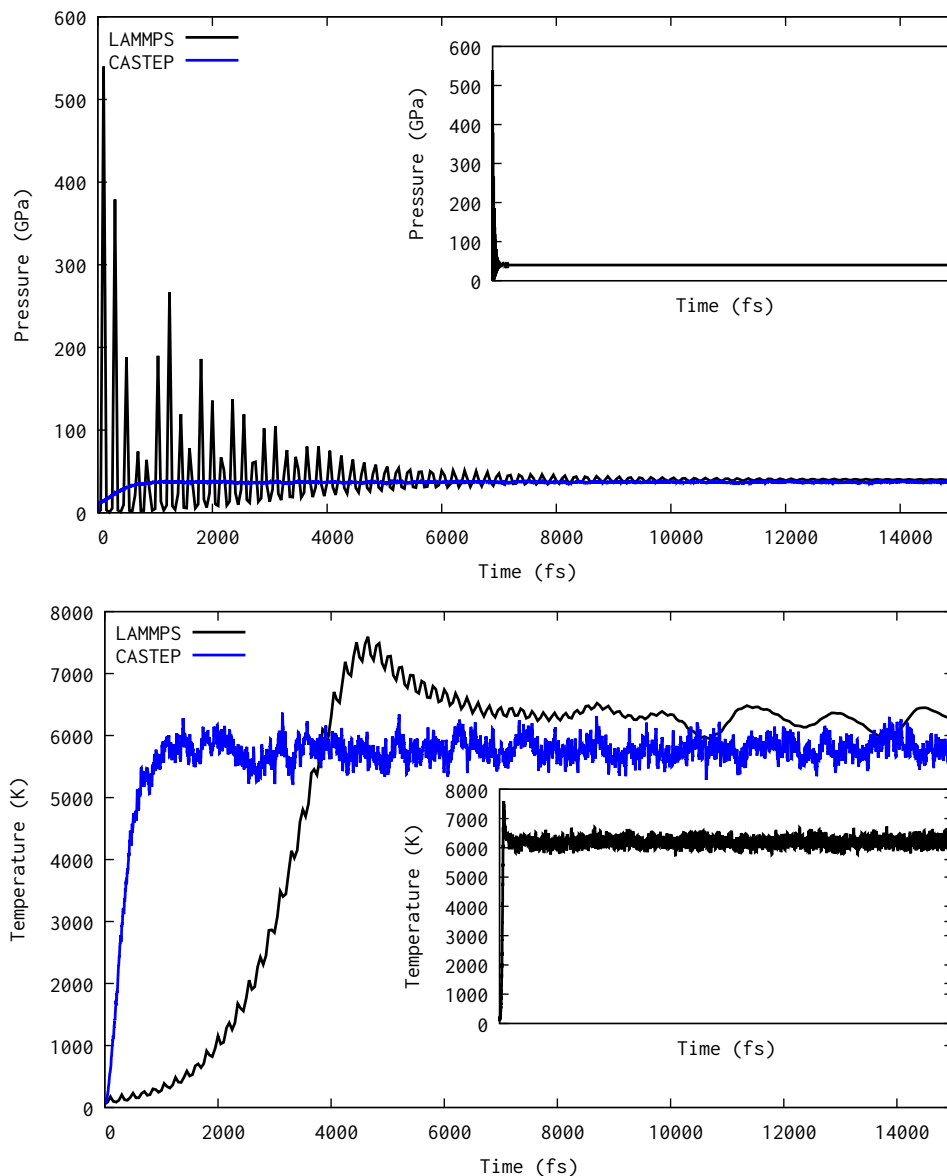
Figure 5.8: Plot to demonstrate agreement between this work's implementation of the Hugoniosat and a reference implementation in the LAMMPS code. The results of CASTEP are using an 864-Atom Lennard-Jones perfect FCC cell and the Langevin NVHug method at 60% compression (Approx. 36GPa). LAMMPS' results are those of a Nosé-Hoover NPHug on a 2048-atom Lennard-Jones FCC cell at 40GPa. The inset graphs show the full trajectory of the 500,000fs LAMMPS run to demonstrate its convergence.
