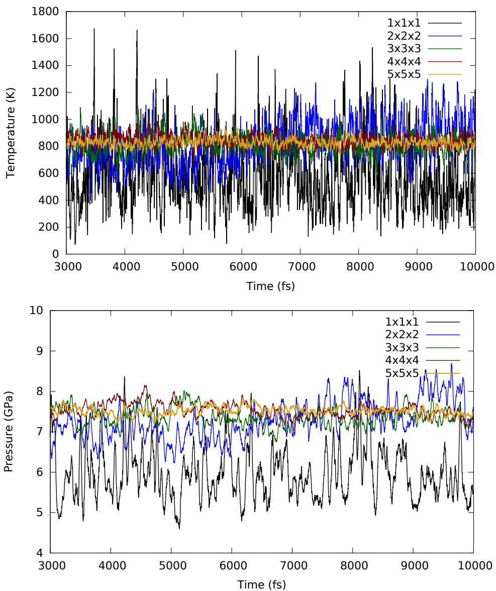
Figure 5.6: A demonstration of the effects of finite cell-size on temperature (top) and pressure (bottom) fluctuations from a 30% compression using the NVHug Langevin formulation (§4.2.1.2). A series of 5 runs with different sizes of supercells of an initially perfect FCC Lennard-Jones cell. 1x1x1 refers to the 8-atom conventional cubic unit-cell and others are respectively larger (64, 216, 512 and 1000 atoms respectively).
