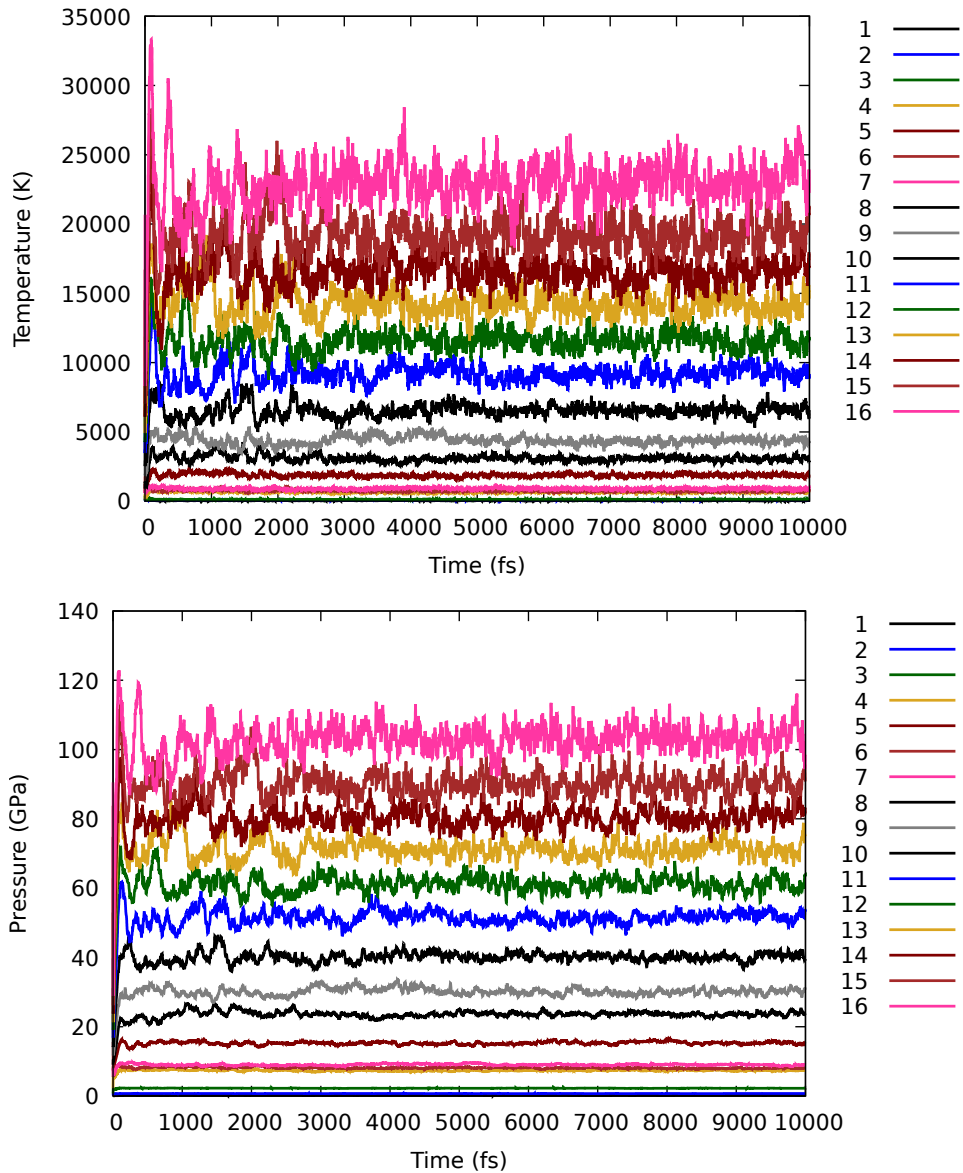
Figure 4.3: Plot showing the accelerated convergence of the Langevin Hugonostat method with moderate damping for 864-Atom Lennard-Jones FCC crystal over first 10ps across entire Hugoniot. Line labels correspond to the predictor (§4.2.2.4) steps.
