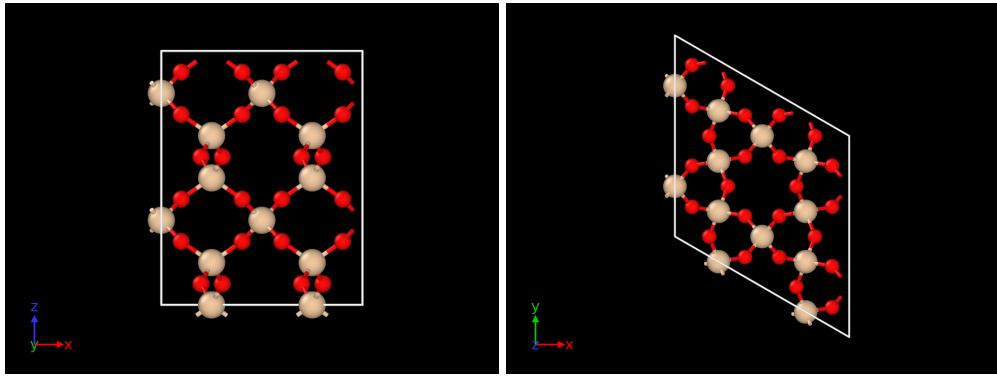
Figure 1.8: A schematic of the \beta -quartz structure. The \alpha -quartz- \beta -quartz transition is simply a rotation of the tetrahedrons, so each silicon is still bound to 4 oxygens in a tetragonal arrangement.
