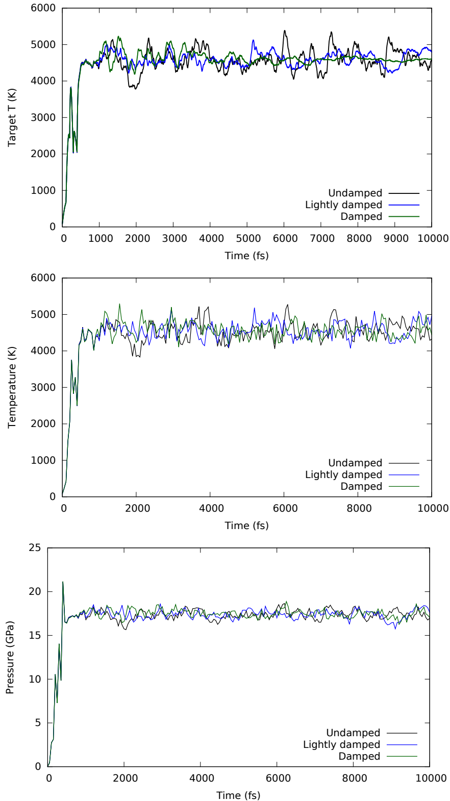
Figure 4.2: Effects of the damping on the Langevin scheme (Eq. 4.2) on a 500-atom Lennard-Jones cell at a 60% compression with an overly strong Hugoniot coupling ( v_H ) of 0.1\text{fs}^{-1} and a damping factor ( \beta_H ) of (Undamped) 0.0, (Lightly Damped) 0.1, (Damped) 0.3, (Top) Convergence of the target temperature to that of the Hugoniot temperature is accelerated and smoothed. (Middle, Low) Convergence of the system properties, with a sample every 50fs. Note that the mean of the system properties are effectively unchanged, but with lower variance.
