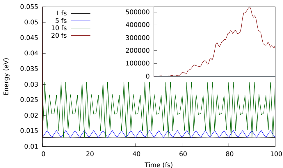
Figure 2.2: Critical instability in energy conservation for a NVE SHO calculation for different time-step lengths. The inset shows the same plot for the 20 fs time-step system which diverges rapidly from physical solution.
