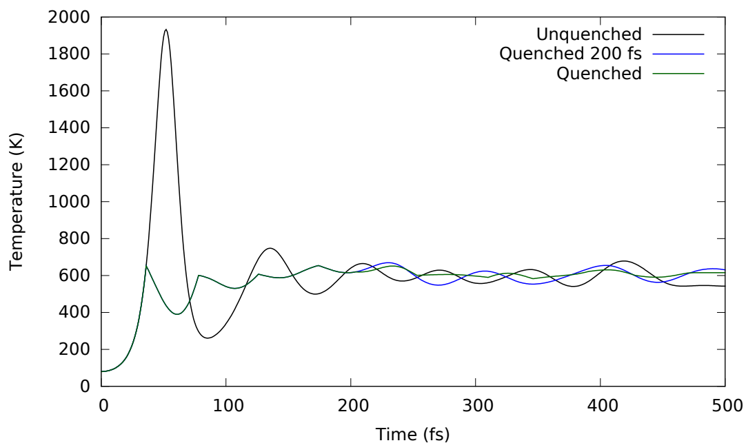
Figure 4.4: The effects of quenching on the temperature of a 30% compressed 500-atom Lennard-Jones system, unquenched line (black) shows a large transient initially, the quenched lines (blue and green) show the elimination of this transient at the expense of “unphysical” temperature dynamics, which are eliminated when the quenching is turned off (blue) after equilibration. It should be noted that all three converge to the same temperature.
