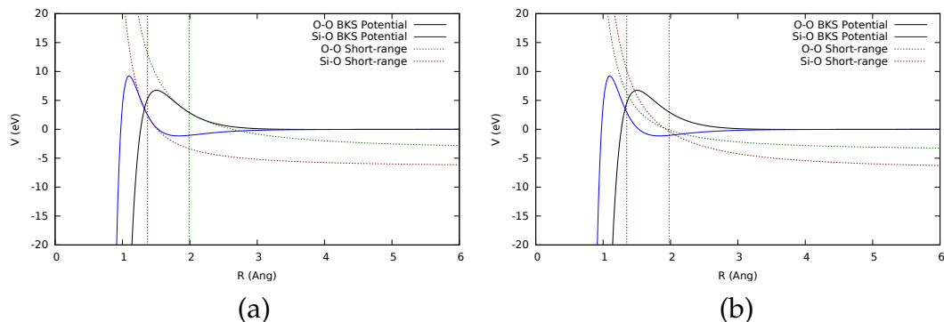
(a:This Work,b:Farrow) Separated energy curves for BKS potential and short range correction. The vertical, dotted lines represent the calculated point of inflexion in the BKS potential, and therefore the switch to the short-ranged potential.
