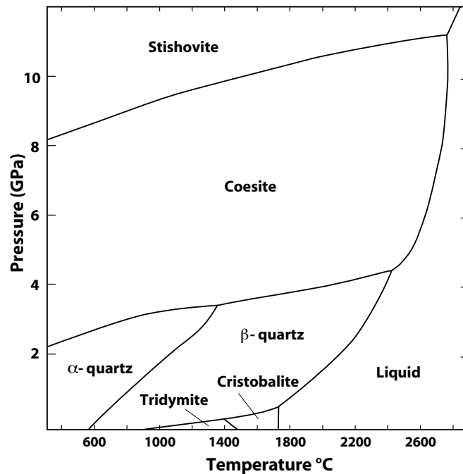
Figure 1.6: A phase diagram of silicate ( \text{SiO}_2 ) minerals. The key phases which will be explored in this work are the \alpha -quartz and \beta -quartz phases, along with the high pressure polymorphs of coesite and stishovite. Taken from SERC based on Swamy et al. [1994].
