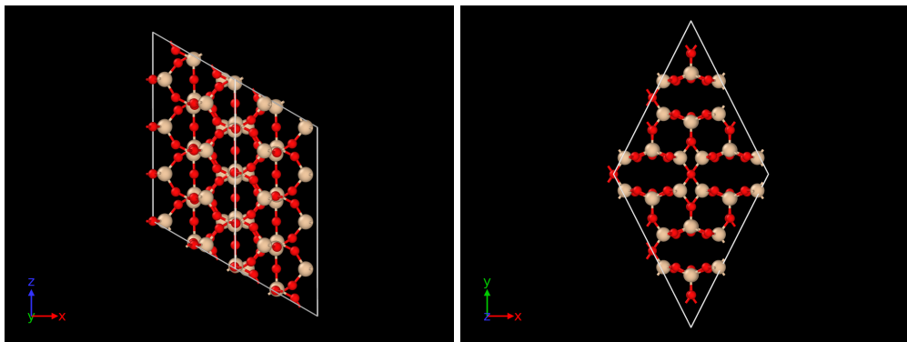
Figure 1.9: A schematic of the coesite structure. The crystal structure of the coesite phase is significantly changed from the \alpha -quartz and \beta -quartz phases, and is a metastable high-pressure, high-temperature state which usually reverts to one of the lower phases when cooling unless quenched. Each silicon is bound to 4 oxygens in a tetragonal arrangement.
