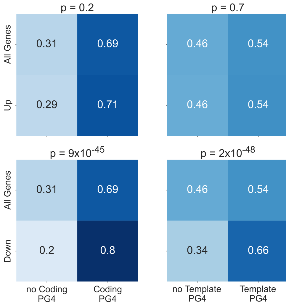
Figure 4.3: NMM downregulated genes are enriched in PG4s Heatmaps showing fractions of genes containing at least one predicted G4 in their gene body for upregulated genes vs all genes (top row) and downregulated genes vs all genes (bottom row) (For down and upregulated genes, FDR < 0.05 and absolute logFC > 0.5). PG4 predictions for the coding strand are in the left hand column whilst PG4 predictions for template strand are on the right. P values for each heatmap are calculated using Chi-squared tests. Genes downregulated by NMM show a particularly strong enrichment of PG4s, and particularly on the template strand.
