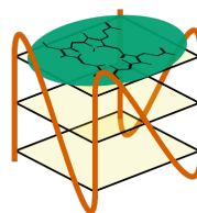
N-Methyl Mesoporphyrin IX
