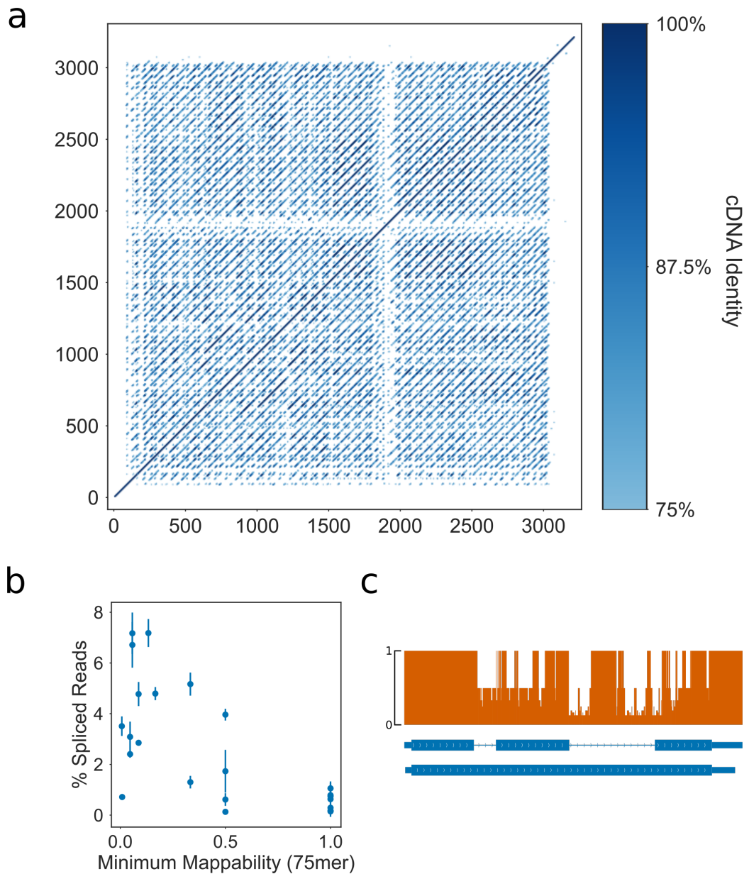
Figure 5.9: Extensin genes with greater spliced mapped reads have low mappability a) Dotplot showing self homology of the EXT9 cDNA (unspliced isoform). Positional identity was calculated using 15bp windows across the gene. Positions with identity less than 75% were filtered to remove noise from the plot. b) Scatter plot showing the minimum mappability score of unspliced Extensin genes against the percentage of spliced reads for that gene in mature root RNAseq samples (Li et al. 2016). Errorbars are standard deviation of three biological replicates. c) Gene track showing the mappability score across EXT9 (orange). Most splice forms cross these low mappability regions, including in the reference annotation Araport11 (shown in blue).
