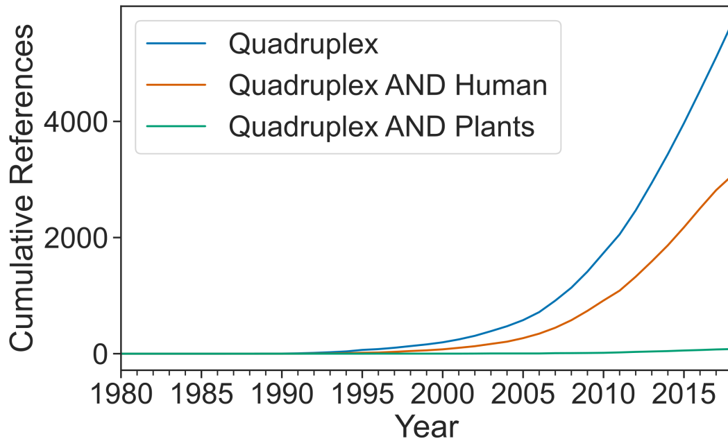
Figure 6.1: Publications in the field of G Quadruplex Biology Cumulative distribution showing the increase in publications listed in the PubMed database containing references to Quadruplexes over the last 40 years. The number of studies in plant species lags far behind studies in humans. Data was generated using MedLine Trends (Dan Corlan, 2004)
