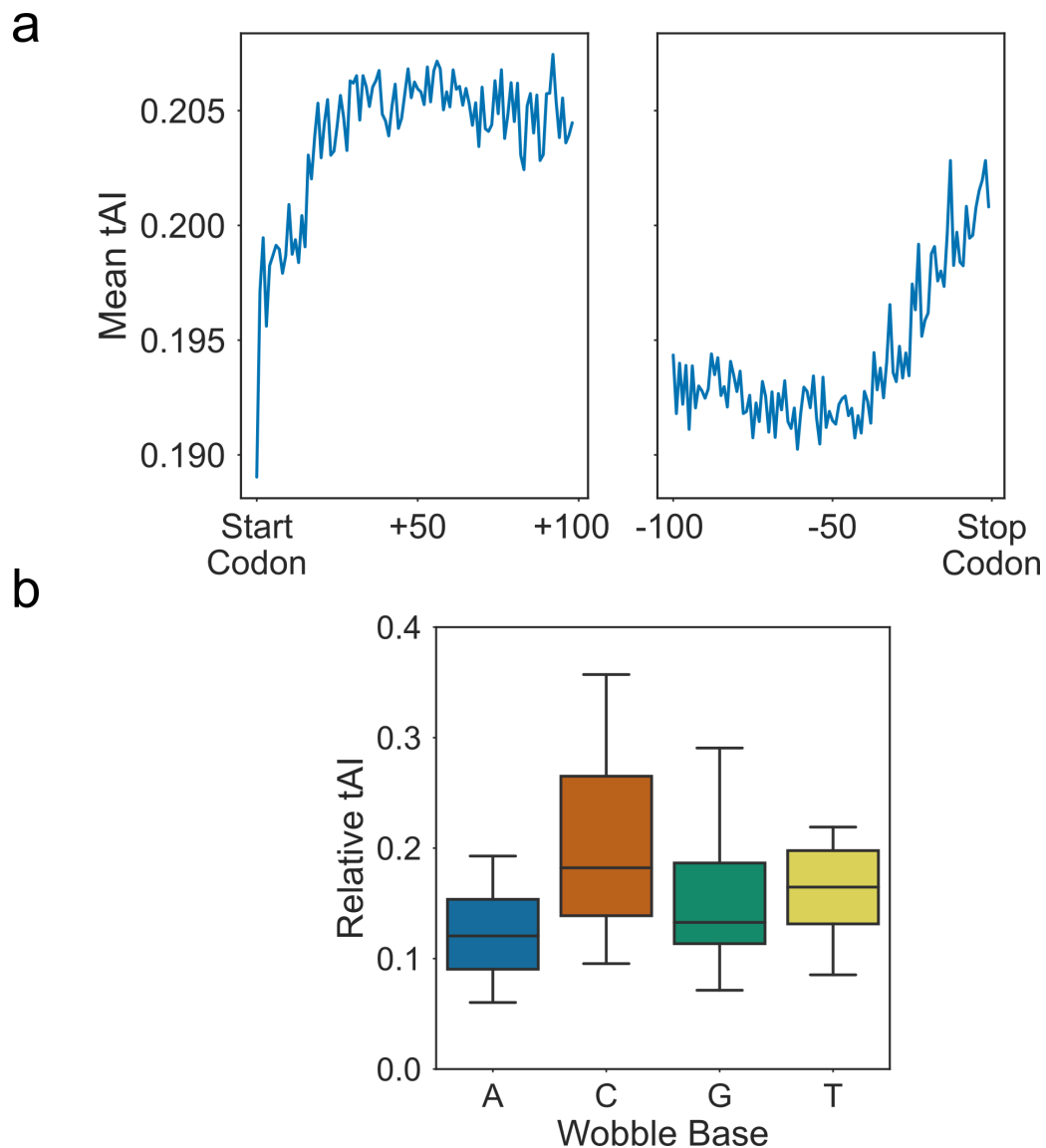
Figure 3.5: tRNA adaptation index of Arabidopsis Coding Regions. a) Metagene profiles showing the mean tAI for the first and last 100 codons of Arabidopsis CDSs. b) Boxplot showing the distribution of tAIs for codons by third (or "wobble") base position.
