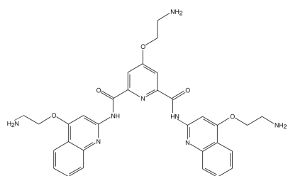
Pyridostatin
