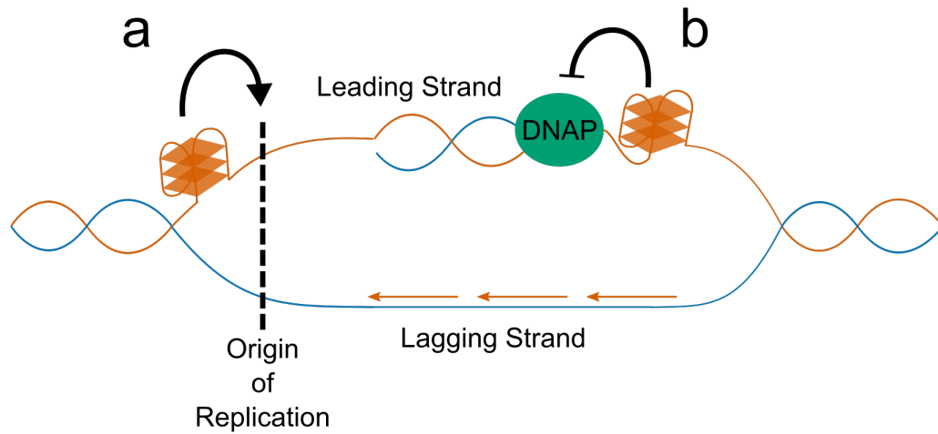
Figure 1.4: Role of G4s in DNA replication Illustration showing the possible mechanisms of G4 involvement in DNA replication. a) Besnard et al. identified that a majority of human replication origins contain a PG4, suggesting that G4s may recruit replication machinery (Besnard et al., 2012). b) In the absence of G4 unwinding helicase FANCD1, Kruisselbrink et al. identified deletions downstream of PG4 loci, suggesting G4s cause replication fork collapse (Kruisselbrink et al., 2008).
