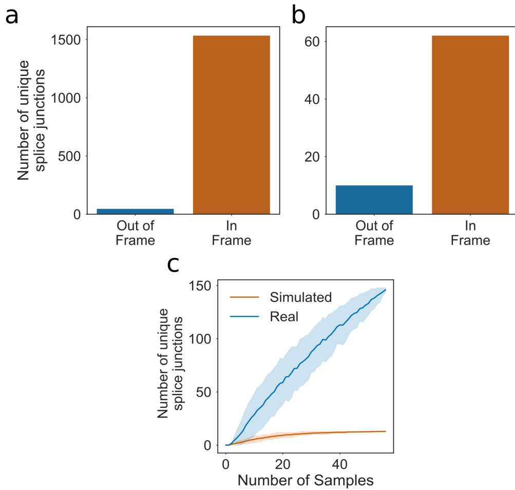
Figure 5.8: Splice junction motifs for EXT9 and LRX3 a & b) Frequency barplots showing number of In/Out of frame splice junctions for EXT9 and LRX3 respectively. c) Bootstrapped splicing simulation showing number of unique EXT9 splice junctions discovered with increasing numbers of samples for real root RNAseq data versus paired simulated RNAseq data. Errorbars are 67% confidence intervals.
