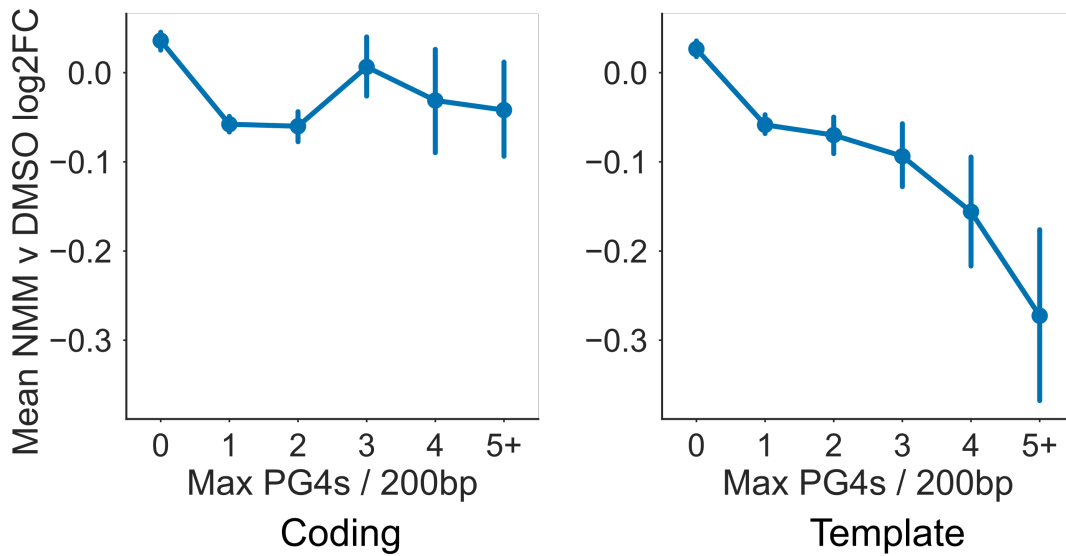
Figure 4.6: NMM regulates genes with large maximal PG4 density Point plot showing mean log fold change in gene expression during NMM treatment for genes binned by maximal PG4 density, defined as the greatest concentration of PG4 motifs within a 200bp sliding window anywhere in the body of the gene (i.e. exon or intron). Left and right panels depict coding and template strands, respectively. Errorbars are 68% confidence intervals for mean generated using 1000 bootstrapped samples.
