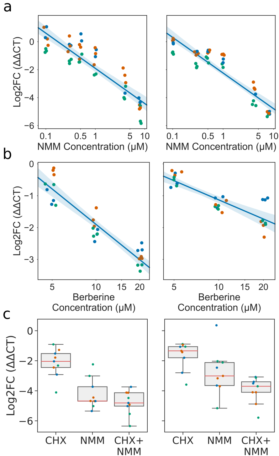
Figure 5.6: Expression of EXT13 and LRX1 during treatment with G4-binding ligands Scatter/strip plots showing qPCR results for EXT13 (left panels) and LRX1 (right panels). Log 2 fold change in expression ( \Delta\Delta\text{CT} ) of Extensin genes decreases with increasing concentrations of a) NMM and b) Berberine. c) NMM downregulation of EXT13 and LRX1 is not affected by concurrent Cyclohexamide treatment, suggesting a mechanism independent of translation. For all panels, each point is a single technical replicate, and colours represent different biological replicates. A small amount of jitter has been added to the X axis for better visualisation of results.
