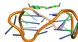
Figure 1.3: G-Quadruplex Stabilising Ligands Structures and mode of action of Pyridostatin (a), NMM (b), and Berberine(c). Crystal structures of human telomeric DNA (parallel G4 form) in complex with NMM and Berberine are from PDB entries 4FXM and 3R6R respectively (Nicoludis et al. 2012, Bazzicalupi et al. 2013). Potassium ions and solvent molecules have been hidden for visualisation purposes.
