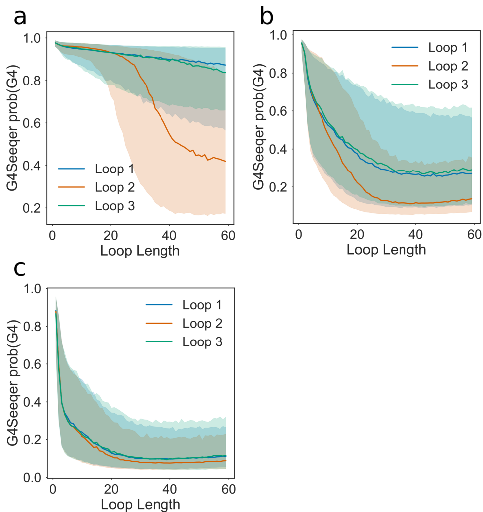
Figure 2.10: Effect of increasing loop length on G4Seeqer score a) Effect of loop length on predicted G4 stability when other loops are held at a constant length of a) 1bp, b) 2bp or c) 3bp. Median value and 68% confidence intervals are produced using 5000 randomly generated sequences (including flanking regions and loop contents) for each pattern analysed.
