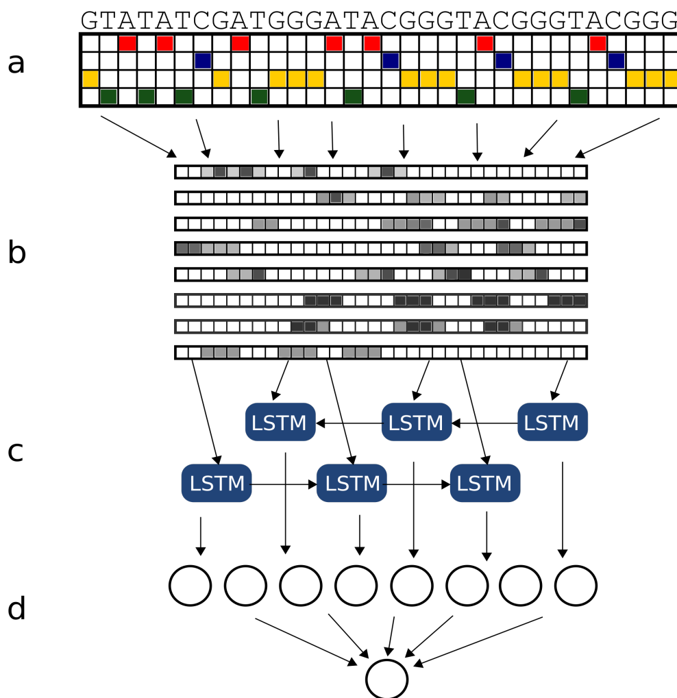
Figure 2.2: G4Seeqer architecture Adapted from Quang & Xie 2016. a) Sequences are one hot encoded to produce a matrix which can be processed by the neural network. b) Input matrices are passed through a convolutional layer. Each layer contains 8 filters which are trained to recognise local patterns on the scale of 3-6bp in size. c) Convolutional features are passed through a bidirectional Long Short Term Memory (LSTM) layer. This layer recognises long distance interactions between features which might combine to produce G4s. d) Finally, features are passed through a fully connected layer. Output from the model is a single probability of whether the sequence forms a G4.
