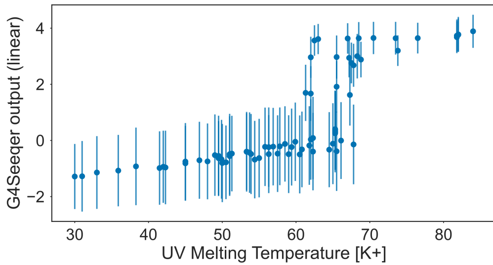
Figure 2.9: G4Seeqer scores correlate with experimentally determined melting temperatures Scatter plot showing median G4Seeqer scores vs. UV melting temperature for sequences from Guédin et al. 2010. Error bars are 68% confidence intervals generated from 1000 iterations of prediction with randomly generated flanking sequences.
