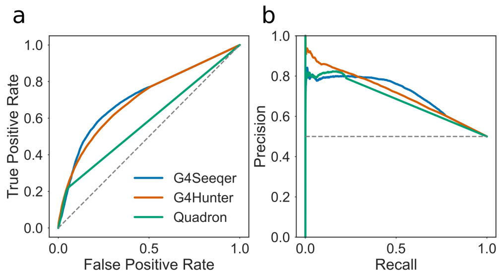
Figure 2.4: Detection by BG4 peak sequences using G4Seeqer a) Receiver Operator Characteristic (ROC) curve showing the performance of G4Seeqer, Quadron, and the G4Hunter method, on BG4 ChIP-seq peaks and randomly shuffled negative sequences.
