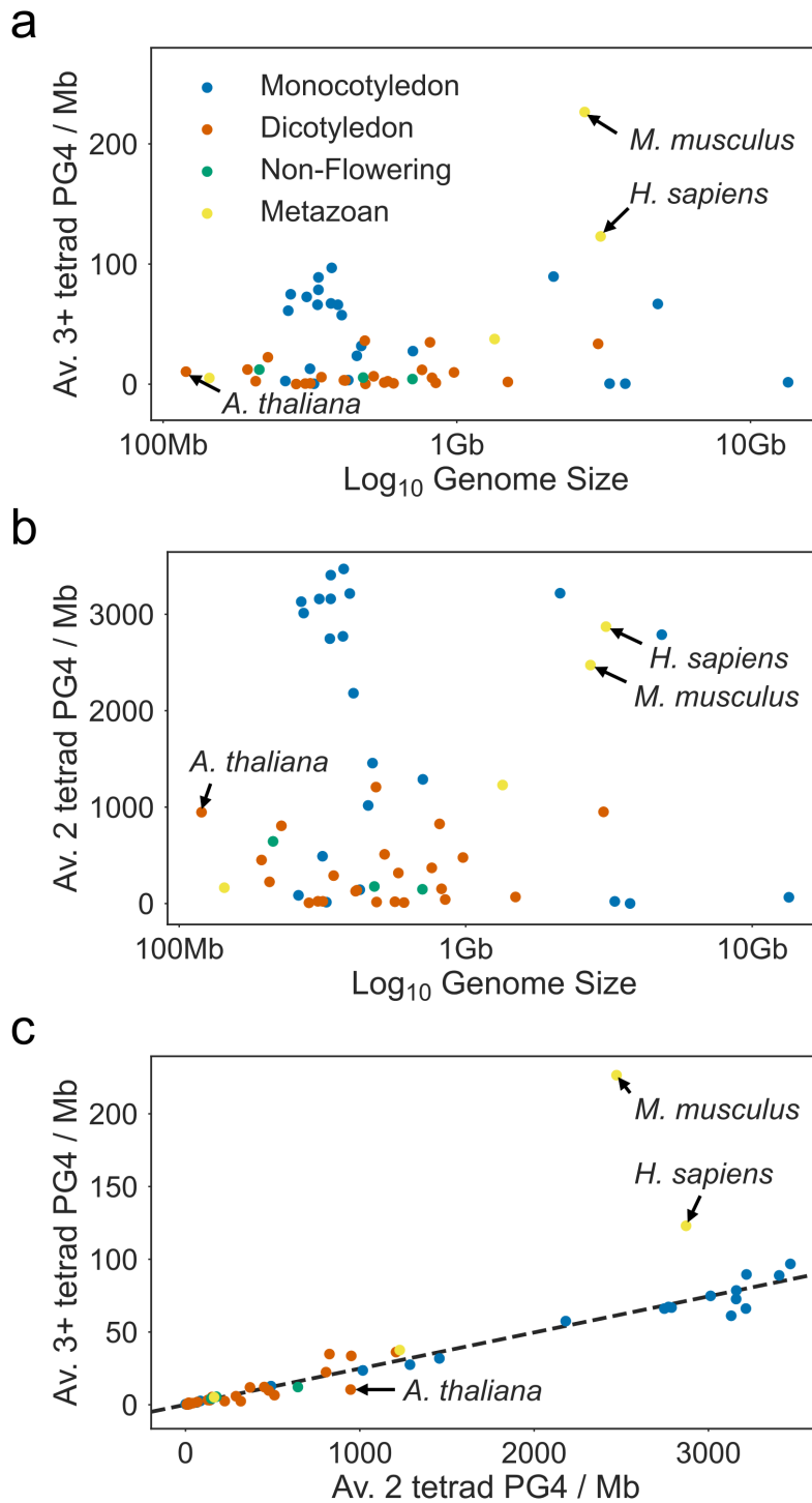
Figure 3.1: PG4 density of Plant Genomes a) and b) Scatter plots showing log 10 genome size vs. the average a) three tetrad or more and b) two tetrad PG4 density per Megabase for 22 Monocotyledons, 21 Dicotyledons, 3 Non-flowering plants and 4 metazoans. Plant genomes are much poorer in three tetrad PG4s than the metazoans H. sapiens and M. musculus , but have more comparable densities of two tetrad PG4s. c) Scatter plot showing the relationship between three tetrad and two tetrad PG4 densities. M. musculus and H. sapiens do not follow the same pattern of relative PG4 densities as plants.
