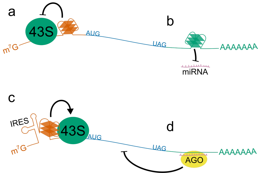
Figure 1.7: G4 function in translation and mRNA stability Schematic showing how 5' and 3' UTR G4s can effect translation of mRNAs. a) G4s in the 5' UTR of mRNAs can cause a reduction in gene expression by preventing scanning of the PIC along the UTR. b) and d) G4 formation in the 3'UTR could block the recognition of miRNA binding sites by Argonaute proteins. c) G4s which form in long and structured 5' UTRs can contribute to internal ribosome entry site (IRES) which promote cap independent initiation of translation
