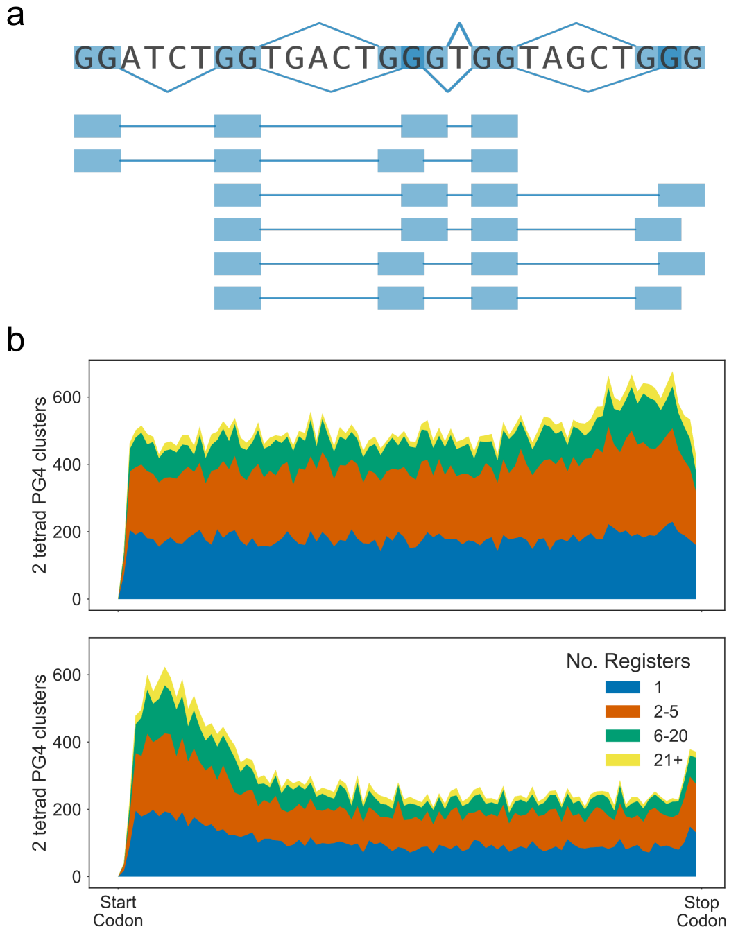
Figure 3.8: PG4 Register does not vary over CDSs a) Diagram showing how a sequence with multiple G-runs can form multiple overlapping PG4 registers and topologies. b) Cumulative metagene profiles showing distribution of PG4 clusters with different numbers of PG4 registers on the coding strand (top panel) and template strand (bottom panel).
