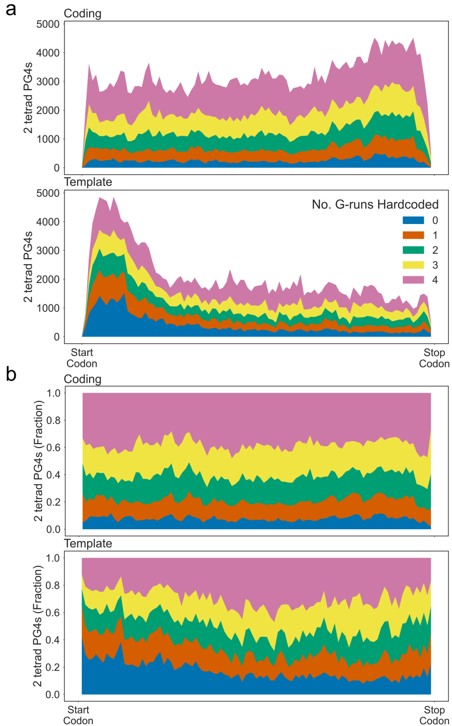
Figure 3.7: Non-hardcoded PG4s levels are greater at the start codon proximal region of CDSs, on the template strand. a) Cumulative metagene profiles showing the distribution of PG4s with different numbers of hardcoded G-runs on the coding (upper panel) and template (lower panel) strands, respectively. b) Same data as shown in a) , represented as the proportion of all PG4s at a position. Coding and template strands are upper and lower panels, respectively.
