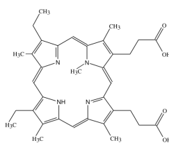
N-Methyl Mesoporphyrin IX
