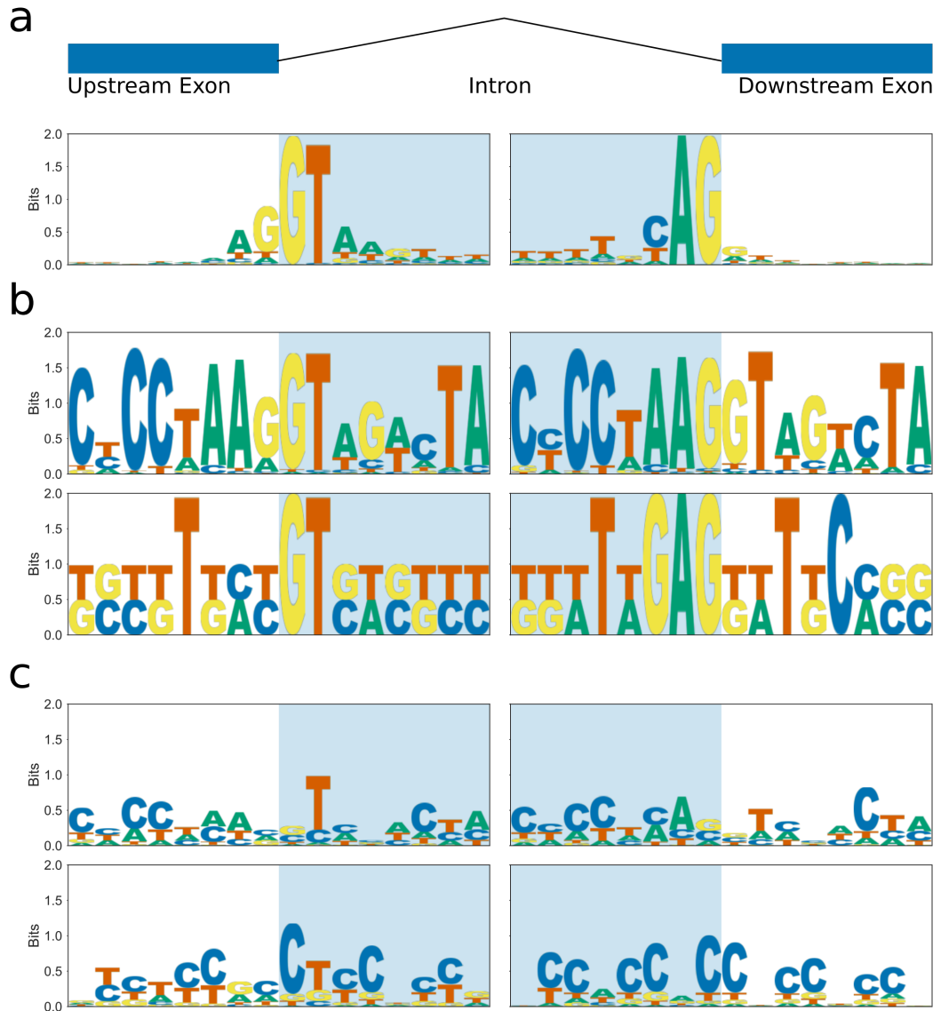
Figure 5.7: Splice junction motifs for EXT9 and LRX3 Sequence logo plots showing consensus splice site sequences around donor (left panels) and acceptor (right panels) splice sites. Putative intronic sequences are shown on shaded blue background. a) Splice junction consensus sequence logo for Arabidopsis, calculated from junctions in the Araport11 annotation. b) Splice junction consensus sequence logo produced from de novo assembled transcripts (Li et al. 2016) for EXT9 and LRX3. c) Splice junction consensus sequence logo produced from unique donor/acceptor pairs identified from spliced reads on EXT9 and LRX3.
