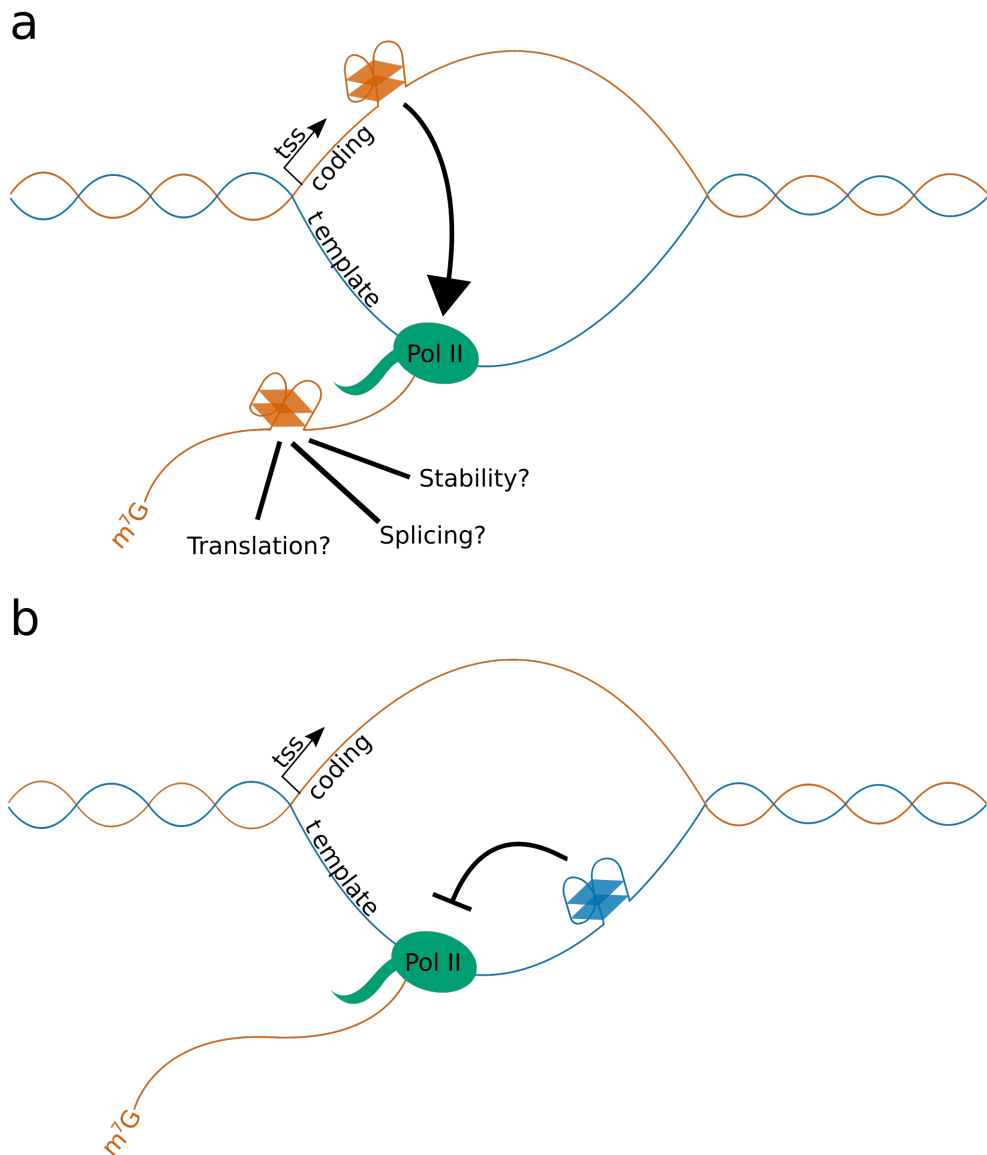
Figure 1.5: Possible Mechanisms for DNA and RNA G4 function in transcription and gene expression a) Possible mechanism for function of G4s located in the coding strand. Since G4s form from single stranded DNA, G4s in the coding strand may promote melting of double stranded DNA, increasing transcription levels. G4s which form in the coding strand of the exonic DNA of a gene will also be present in the mRNA produced from that locus, and G4s which form in the coding strand of introns will be present in pre-mRNA. These RNA G4s might also influence gene expression through alteration of pre-mRNA splicing, mRNA stability, or translation. b) Possible mechanism for the function of G4s located in the template strand. The template strand of genes is scanned by RNA Polymerase II during transcription, and G4s which form in ahead of the transcription complex may cause slowing or stalling if they cannot be correctly resolved. RNA Polymerase II translocation speed is linked to a number of co-transcriptional processes, including splicing. Adapted from Figure 4. Rhodes and Lipps, 2015.
