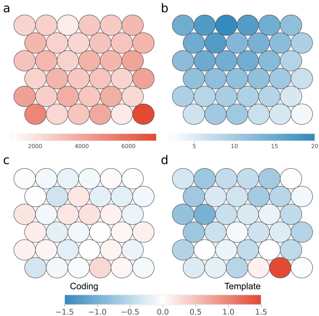
Figure 4.5: Self Organising Maps demonstrate NMM downregulated genes contain specific PG4 types. Self Organising Map (SOM) plots for clustering of Quad-parser predicted two tetrad PG4s by loop length. In each figure, each circle represents a cluster of similar PG4s. a) SOM plot coloured by cluster size. Each cluster contained between 1000 and 8000 PG4s. b) SOM plot coloured by total length in bases of all loops. c) and d) Log 2 fold enrichment of each cluster in the gene bodies of genes downregulated by NMM, on the coding and template strands, respectively. Log 2 fold enrichments were generated by comparing actual overlap of PG4s with downregulated genes, with expected overlap when PG4s were permuted amongst all genes.
