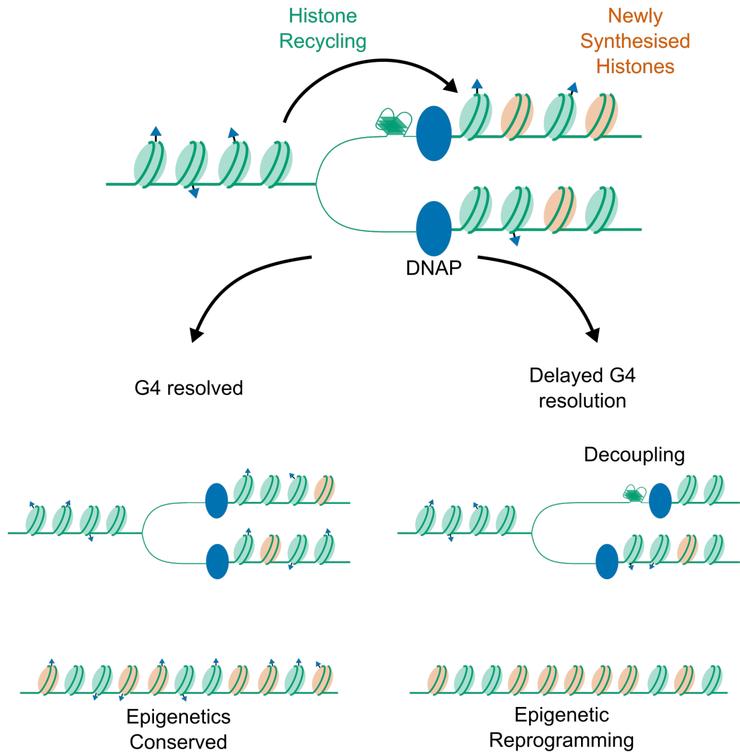
Figure 1.8: G4 stalling causes epigenetic reprogramming Illustration demonstrating the mechanism by which G4 stalling is thought to cause epigenetic reprogramming. Histone recycling from upstream of the replication fork into newly synthesised DNA is tightly linked to DNA replication. This is important to maintain the correct histone modifications in the daughter cells, as recycled histones are mixed with newly synthesised ones and used to seed them with existing modifications. When G4s form in the leading strand of the DNA, they cause blockages that decouple DNA replication from histone removal, resulting in the insertion of longer stretches of newly synthesised histones into the DNA. This causes the loss of histone modifications from this region of the DNA. Adapted from Guilbaud et al. 2017.
