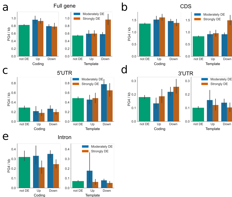
Figure 4.4: Distribution of PG4s in genes differentially regulated by NMM. Bar plots showing the average PG4 densities of genes up or downregulated by NMM, for a) full gene body (exons and introns), b) coding regions, c) 5' UTR, d) 3' UTR, and e) introns, respectively. In each figure, left and right panels represent coding and template strand, respectively. Genesets are separated into three categories by strength of regulation: green: not differentially expressed, blue: moderately differentially expressed ( PPLR < 0.05 , \logFC > 0.5 ), orange: strongly differentially expressed ( PPLR < 0.05 , \logFC > 1 ). Errorbars are 68% confidence intervals for mean generated using 1000 bootstrapped samples. Genes which are strongly downregulated by NMM tend to have higher PG4 densities on the template strand of coding regions and 5' UTRs, whilst moderately downregulated genes tend to have greater PG4 density on the template strand of their 5' UTRs.
