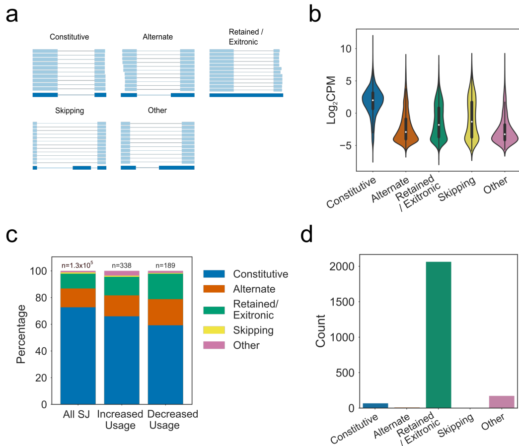
Figure 5.11: Differential Junction Usage during NMM treatment a) Schematic showing the five classes used to categorise splice junctions based on flattened reference annotation. Junctions which are present as introns in the reference are labelled constitutive junctions. Constitutive junctions which cause skipping of an exon are labelled skipping junctions. Junctions which share a donor or acceptor site with one in the reference are labelled alternate junctions. Junctions which are wholly contained within a single exon of the reference are labelled retained/exitronic junctions. Finally, junctions which share no donor or acceptor with the reference and span a mixture of exonic and intronic sequence are labelled "other". b) Violin plot showing distribution of average expression in log 2 counts per million for each junction class. c) Proportion of junction in each class for all splice junctions vs. those with significantly increased or decreased usage during NMM treatment (Absolute logFC > 0.5, FDR < 0.2). d) Categorisation of detected junctions in Extensin genes.
