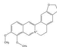
Berberine
