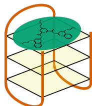
Pyridostatin
