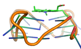
Figure 1.3: G-Quadruplex Stabilising Ligands Structures and mode of action of Pyridostatin (a), NMM (b), and Berberine(c). Crystal structures of human telomeric DNA (parallel G4 form) in complex with NMM and Berberine are from PDB entries 4FXM and 3R6R respectively (Nicoludis et al. 2012, Bazzicalupi et al. 2013). Potassium ions and solvent molecules have been hidden for visualisation purposes.
