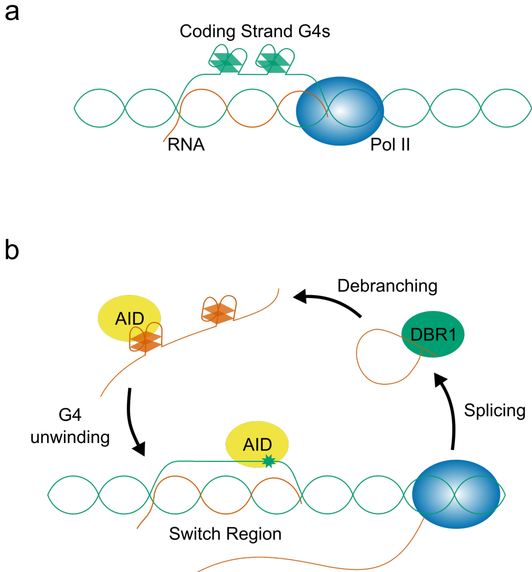
Figure 1.9: An R-loop and G4 dependent mechanism for Class Switch Recombination a) Schematic showing the formation of an R-loop from G-rich RNA and C-rich template DNA, behind transcribing RNA Polymerase II. The G-rich coding strand is left in a single stranded form, and may fold into G4s. b) Proposed mechanism for Class Switch Recombination of IgH gene through R-loop formation. Transcription and splicing of the IgH locus results in a G-rich intron lariat which is debranched by DBR1. This folds into RNA G4s which recruit AID. Resolution of G4s by DDX1 promotes R loop formation and targets AID to the switch region, causing deamination and double strand breaks. Adapted from Zheng et al. 2015.
