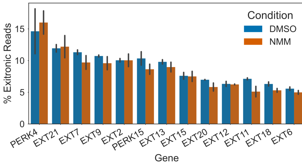
Figure 5.12: NMM does not cause significant changes in the amount of Exitronic Splicing of Extensins Barplots showing a) gene expression in log 2 counts per million, and b) percentage of reads exhibiting Exitronic splicing, for expressed Extensin genes with an average of at least 5% spliced reads. Levels during mock (DMSO) treatment are shown in blue, and levels during NMM treatment are shown in orange. Ordering of genes (by average percent spliced) in upper and lower panels is matched. Errorbars are standard deviation of three biological replicates.
