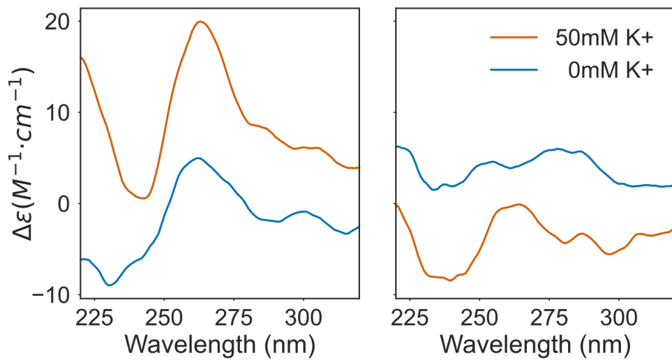
Figure 5.5: The Extensin SP4 motif forms a G-Quadruplex in vitro . a) Schematic showing how the Extensin SP4 protein motif hardcodes a two tetrad PG4 into the template strand of the gene body. b) CD spectroscopy of an Extensin repeat sequence (left) and a mutated control which does not conform the the Quadparser motif (right) show that the Extensin repeat forms a G4 in vitro . This is indicated by the peak in ellipticity at 260nm and the trough at 240nm, which are characteristic of a parallel G4.
