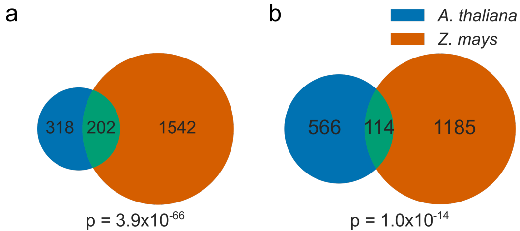
Figure 4.13: NMM expression change of Arabidopsis and Zea mays orthologs Venn diagrams showing the overlap between the set of genes a) upregulated and b) downregulated by NMM in Arabidopsis and the unique set of Arabidopsis orthologs for Z. mays genes regulated by NMM. P values were calculated by hypergeometric test compared to the unique set of Arabidopsis genes with at least one Z. mays ortholog.
