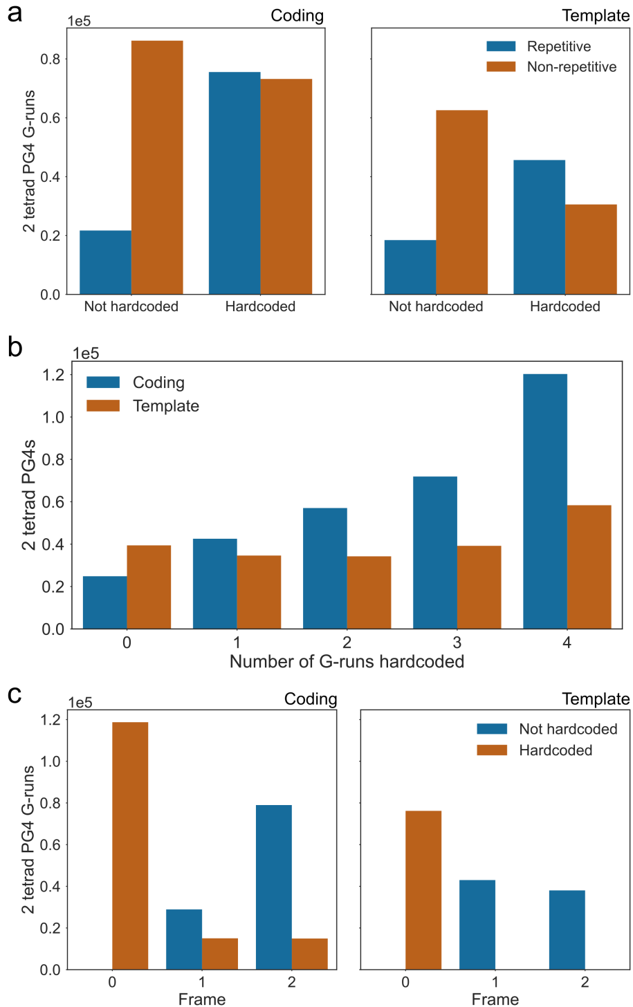
Figure 3.6: 54% of CDS PG4 G-runs are hardcoded by protein sequence. a) Frequency plot showing the total number of G-runs contributing to PG4s which are hardcoded and repetitive. Left and right panels show frequencies on coding and template strands, respectively. Hardcoded G-runs are defined as those GG dinucleotides that cannot be removed from the sequence without changing the amino acid sequence which is coded for. Repetitive G-runs are defined as those which contribute to PG4s where all G-runs are part of codons which encode the same sequence. b) Frequency plot showing the total number of hardcoded G-runs for each overlapping PG4 register on the coding (blue) and template (orange) strands, respectively. c) Frequency plots showing start frame of CDS G-runs vs. hardcoded status. Left and right panels show frequencies on coding and template strands, respectively.
