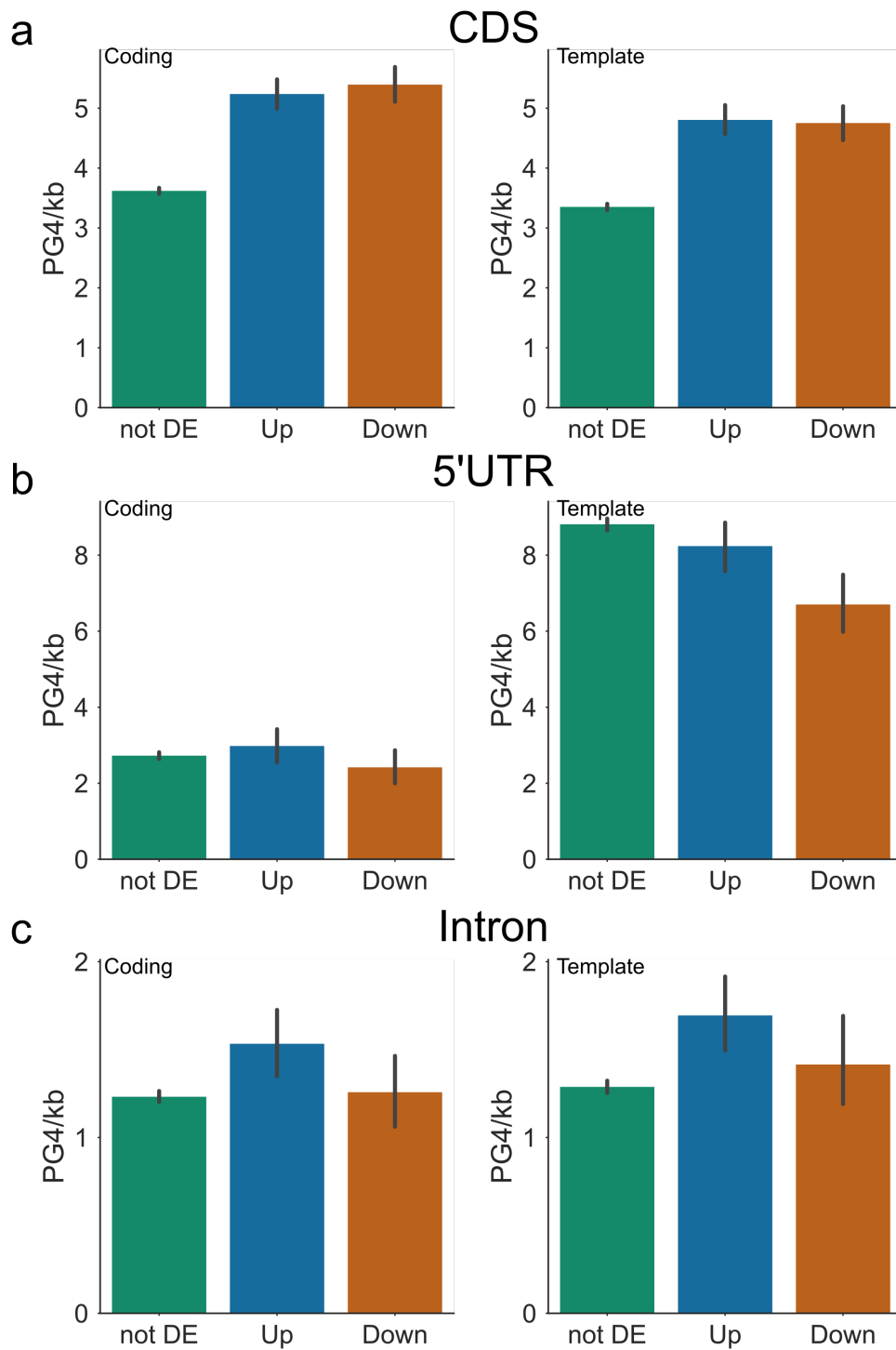
Figure 4.14: Distribution of Two tetrad PG4s in Z. mays genes regulated by NMM Bar plots showing the average PG4 densities of Z. mays genes up or downregulated by NMM, for a) CDSs, b) 5' UTRs and c) introns, respectively. In each figure, left and right panels represent coding and template strand, respectively. Errorbars are 68% confidence intervals for bootstrapped means.
