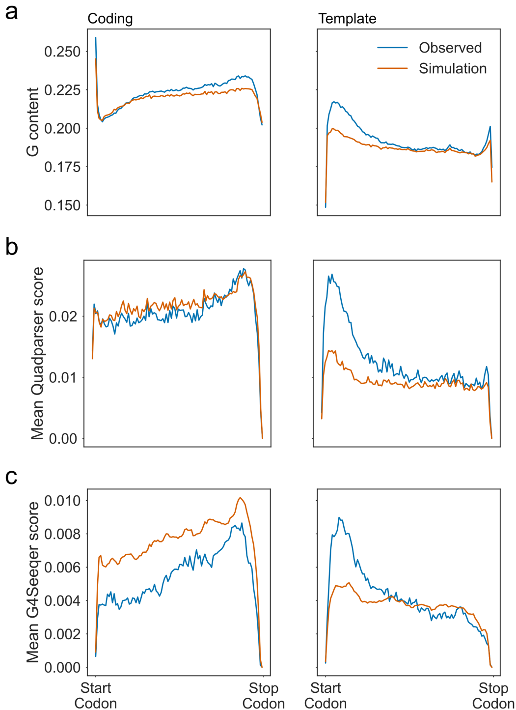
Figure 3.4: Reverse Translation Simulation shows that PG4s are enriched at the Start Codon proximal region of the template strand. Metagene profiles showing a) G content b) Quadparser PG4s and c) G4Seeqer PG4s for real CDS regions (blue) vs. reverse translation simulated potential coding sequences (PCS) (orange).
