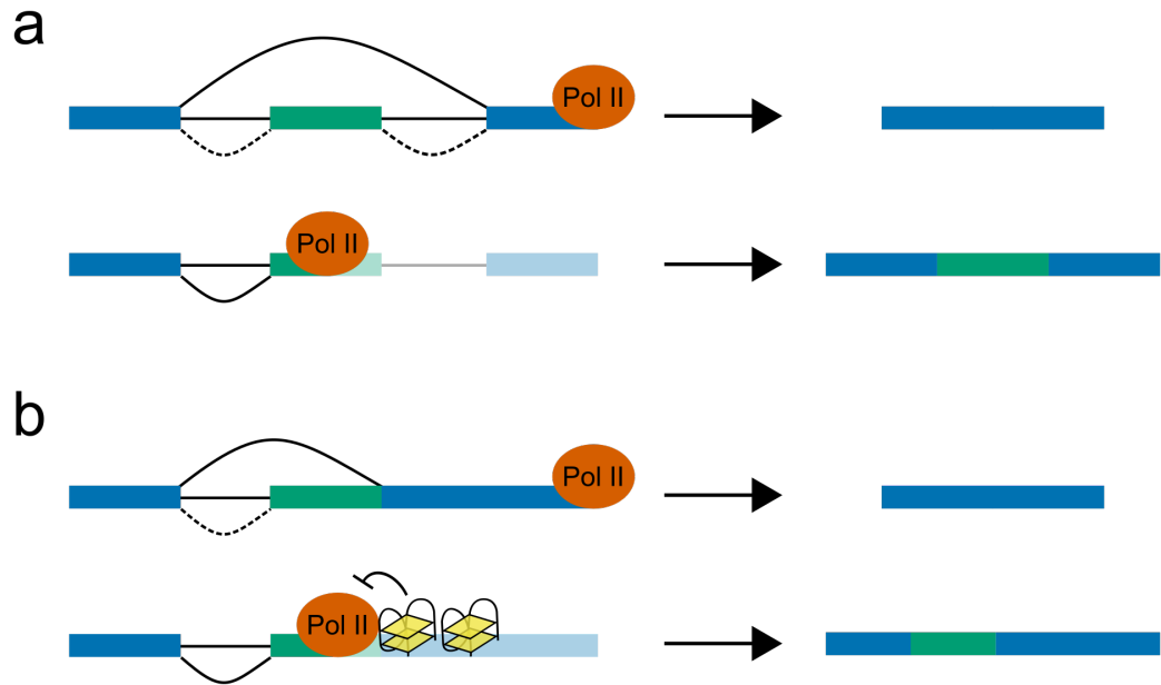
Figure 5.1: Pol II elongation speed affects co-transcriptional splicing a) Mechanism for effect of Pol II speed on co-transcriptional splicing: when elongation occurs rapidly (first row), the more canonical but distal acceptor site is used, resulting in the exclusion of the alternate exon (shown in green). When Pol II elongates more slowly (second row), there is more time for the weaker proximal site to be utilised, resulting in the inclusion of the alternate exon. b) Example mechanism for how G4s could affect splicing. When G4s are not present (top row), the constitutive splice acceptor is used and the green exonic chunk is excluded. When G4s are formed in the template strand of the DNA (second row), these slow down Pol II elongation, allowing the weaker proximal splice junction to be utilised, and including the alternate exon chunk.
