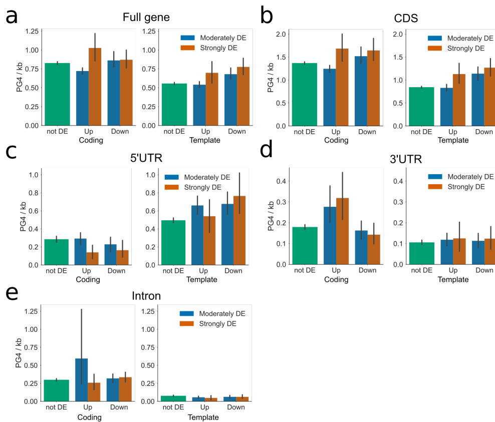
Figure 4.11: Distribution of PG4s in genes differentially regulated by Drought stress. Bar plots showing the average PG4 densities of genes up or downregulated by Drought stress, for a) full gene body (exons and introns), b) coding regions, c) 5' UTR, d) 3' UTR, and e) introns, respectively. In each figure, left and right panels represent coding and template strand, respectively. Genesets are separated into three categories by strength of regulation: green: not differentially expressed, blue: moderately differentially expressed (PPLR < 0.05, logFC > 0.5), orange: strongly differentially expressed (PPLR < 0.05, logFC > 1). Errorbars are 68% confidence intervals for mean generated using 1000 bootstrapped samples. Genes which are downregulated by drought stress tend to have higher PG4 densities on the template strand of coding regions and 5' UTRs. Genes which are upregulated by drought stress are more likely to contain PG4s in their 3' UTRs.
