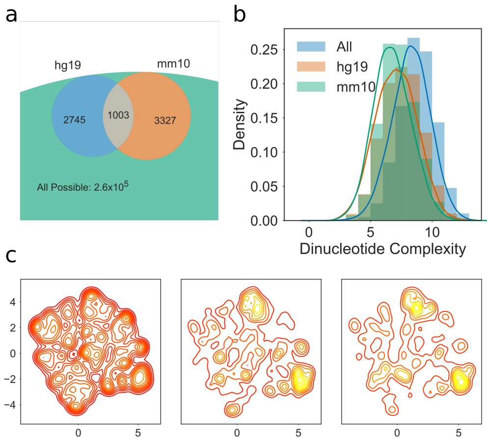
Figure 2.12: Human and mouse genomes contain different G4 subpopulations a) Venn diagram showing overlap of 3 tetrad Quadparser motifs populations with loop lengths of 3bp in the human (hg19) and mouse (mm10) genomes, compared to all possible sequences. b) Histogram and kernel density estimate of dinucleotide complexity for human, mouse and all possible 3 tetrad Quadparser motifs with loop length of 3bp. c) 2D Kernel density estimate plot showing distribution of all possible tetrad Quadparser motifs (left), those found in the human genome (centre) and those found in the mouse genome. Dimensionality reduction was conducted using UMAP with Hamming distance as the metric.
