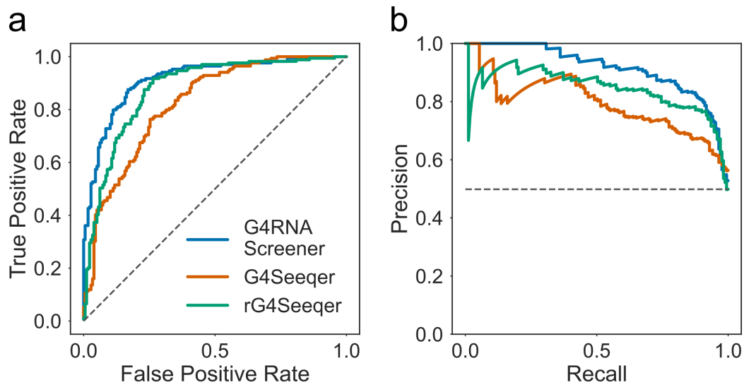
Figure 2.6: Validation of rG4Seeqer on in vitro experimentally categorised RNA sequences a) Receiver Operator Characteristic (ROC) curves showing the performance of rG4Seeqer, G4Seeqer and the G4RNA Screener method (Garant et al. 2017), on the G4RNA dataset curated by Garant et al. b) Precision-recall curves showing the performance of rG4Seeqer, G4Seeqer, and G4RNA Screener on the same dataset.
