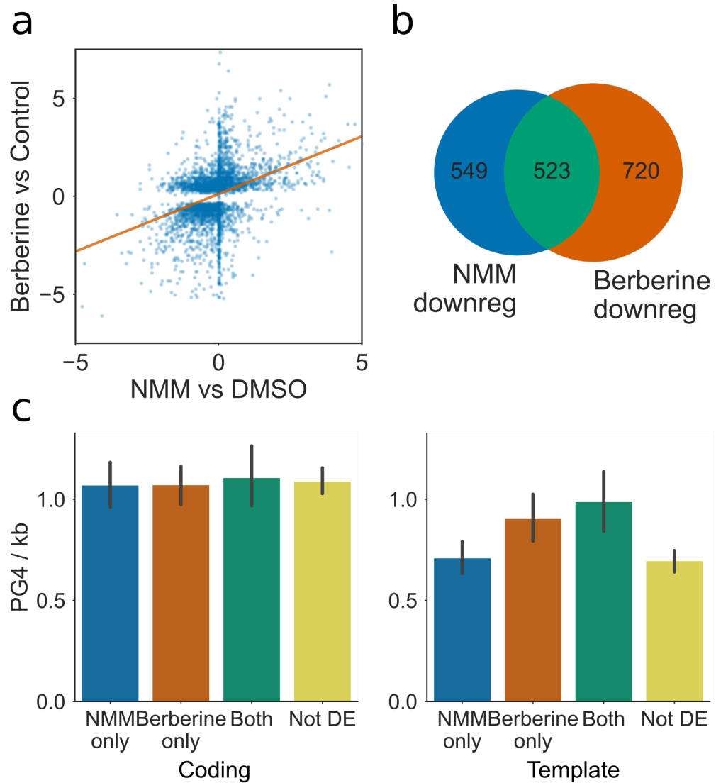
Figure 4.2: Comparison of gene expression during NMM treatment with expression during Berberine treatment. a) Scatter plot with regression line showing the correlation in expression change for NMM vs DMSO and Berberine vs Control. Processed Berberine data was taken from supplementary information of Nakagawa et al. 2012, however only differentially regulated genes were reported. b) Venn diagram reporting the overlap of genes downregulated by NMM with those downregulated by Berberine. c) Bar plot showing the average exonic PG4 densities of NMM and Berberine downregulated genesets, on the coding and template strands, respectively. Bar colours match set colours from Fig 3b. Errorbars are 68% confidence intervals for mean generated using 1000 bootstrapped samples.
