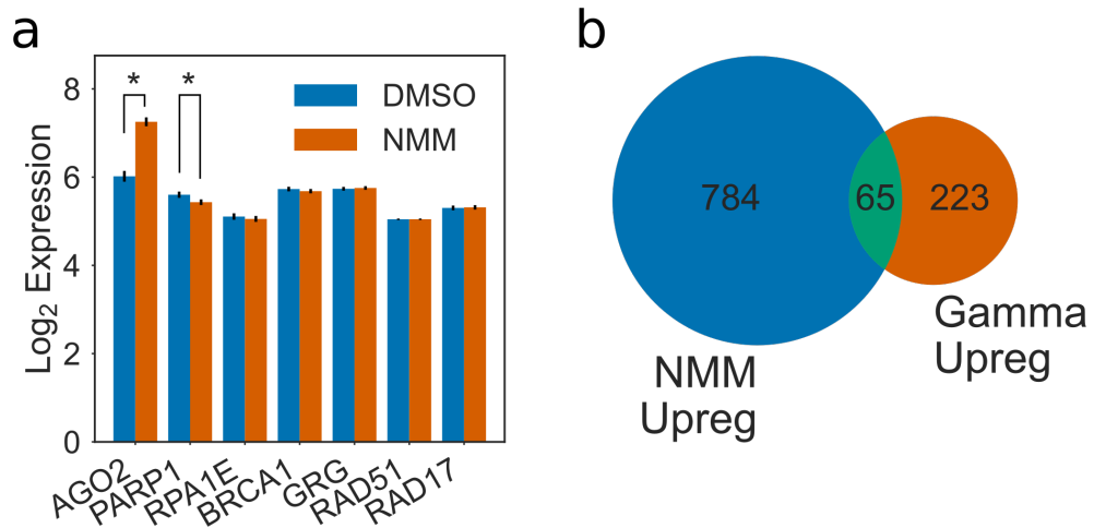
Figure 4.9: NMM does not activate DNA damage response a) Barplot showing normalised log 2 expression of seven DNA damage responsive genes: AGO2, PARP1, RPA1E, BRCA1, GRG, RAD51, and RAD17, in the presence and absence of NMM. Errorbars are standard errors calculated by puma . Asterisks denote significant results. b) Venn diagram showing the overlap between NMM upregulated genes and genes upregulated in response to gamma irradiation.
