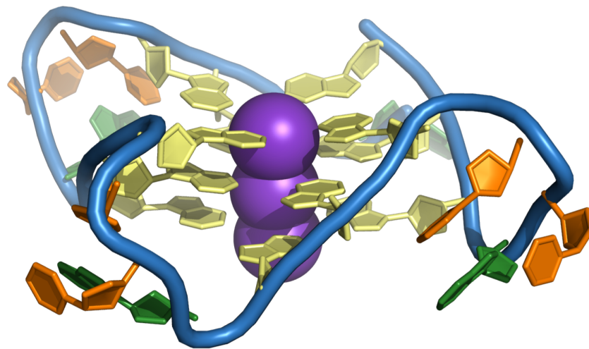
Figure 1.2: The Human Telomeric Sequence forms a G-Quadruplex a) top and b) side view of a parallel G4 structure solved by X-ray crystallography (PDB: 1KF1, Parkinson et al. 2002). The sequence used is (TTAGGG)_4 , corresponding to four of the human telomeric repeat. Gs are coloured in yellow, As in green and Ts in orange. Potassium cations are coloured in purple.
