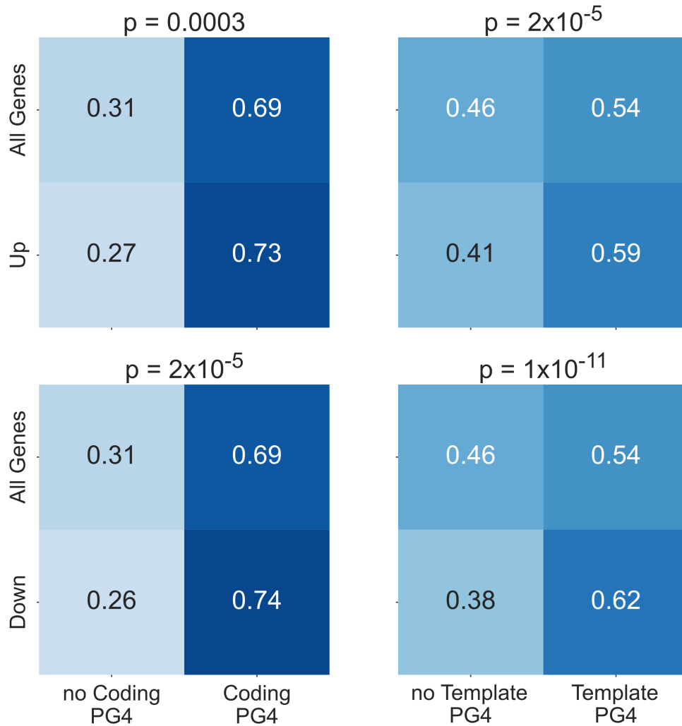
Figure 4.10: Drought downregulated genes are enriched in PG4s Heatmaps showing fractions of genes containing at least one predicted G4 in their gene body for drought upregulated genes vs all genes (top row) and drought downregulated genes vs all genes (bottom row) (For down and upregulated genes, FDR < 0.05 and absolute logFC > 0.5). PG4 predictions for the coding strand are in the left hand column whilst PG4 predictions for template strand are on the right. P values for each heatmap are calculated using Chi-squared tests. Genes downregulated by drought stress show a particularly strong enrichment of PG4s, and particularly on the template strand.
