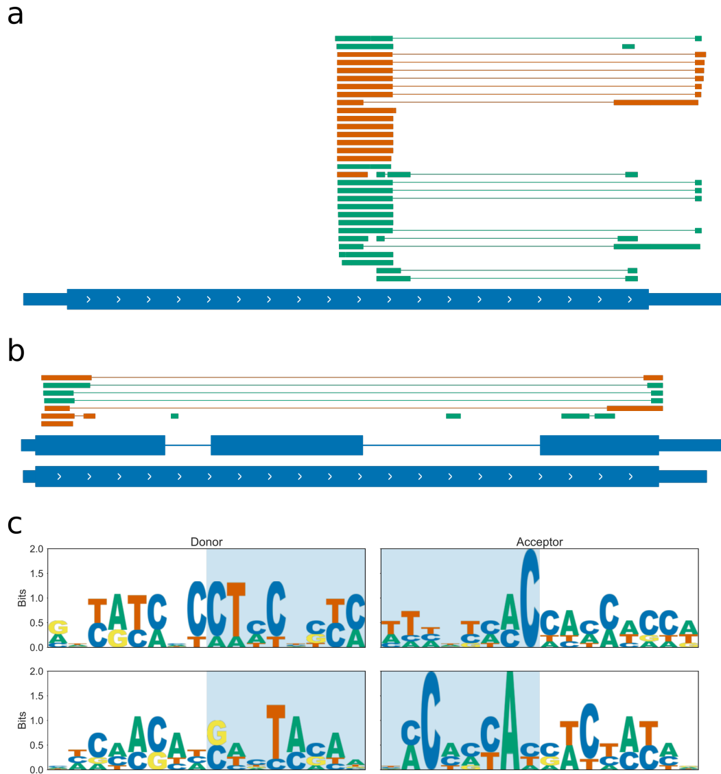
Figure 5.10: Sanger sequencing of LRX1 and EXT9 cDNA identifies spliced forms a) Gene track showing aligned sanger sequencing products for a) LRX1 and b) EXT9. Products aligned to the forward strand are shown in green, and products aligned to the negative strand are shown in orange. Gene models are from the Araport11 annotation. c) Sequence logos for sanger product splice junctions for LRX1 (top panel) and EXT9 (lower panel).
