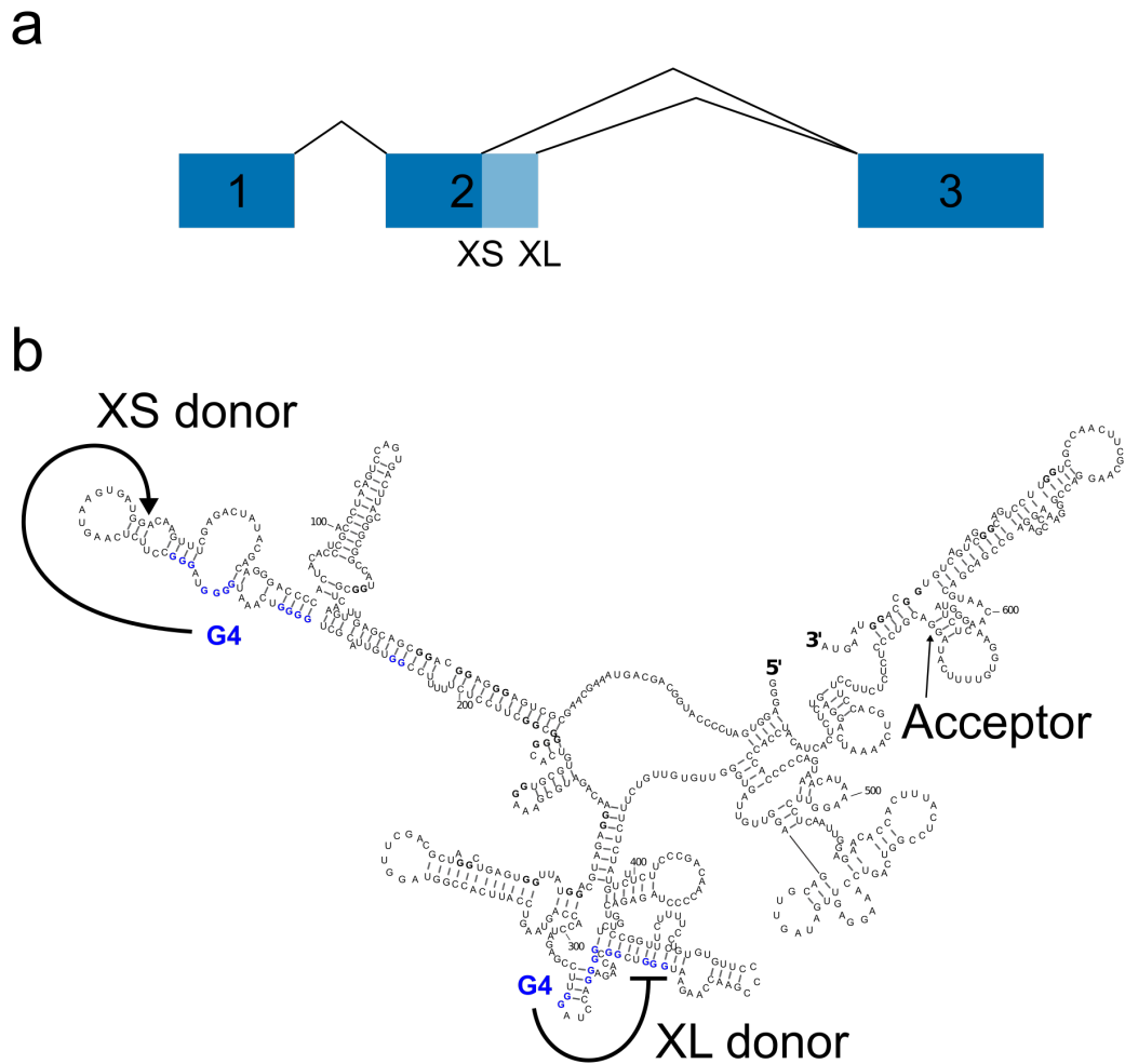
Figure 1.6: G-Quadruplexes control the splicing of Bcl-X pre-mRNA a) Diagram showing the splice isoforms Bcl-XS and Bcl-XL, which are derived from alternative splicing of exon 2. b) RNA structure of Bcl-X-681 (a synthetic transcript derived from Bcl-X) showing positions of G4s and splice donor/acceptor sites. Formation of a G4 near Bcl-XS donor site promotes usage of the XS splice donor. Formation of a G4 near Bcl-XL donor site inhibits usage of the XL splice donor. Adapted from Weldon et al. 2018
