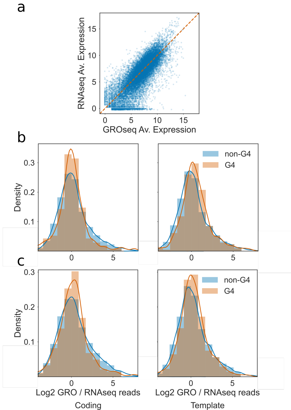
Figure 4.8: Log Ratio of GRO / RNA seq counts per million detects abortive transcription of PG4 dense genes. a) Scatter plot showing measured expression in log 2 counts per million (logCPM) for each gene from GRO-seq vs. RNAseq datasets. Genes which fall below and to the right of the orange line have positive log 2 GRO/RNA ratios. b) Histogram and kernel density estimates of GRO/RNA ratio for genes containing PG4 predicted by G4Seeqer (max G4seeqer score > 0.95) in orange, vs. genes containing no G4s (max G4seeqer score < 0.05) in blue. Left and right panels represent coding and template strand G4 rich genes, respectively. c) Histogram and kernel density estimates of GRO/RNA ratio for genes containing two tetrad maximal PG4 density per 200bp of 3 or greater in orange, vs. genes with maximal PG4 density of 0 (contain no PG4s) in blue. Left and right panels represent coding and template strand G4 rich genes, respectively.
