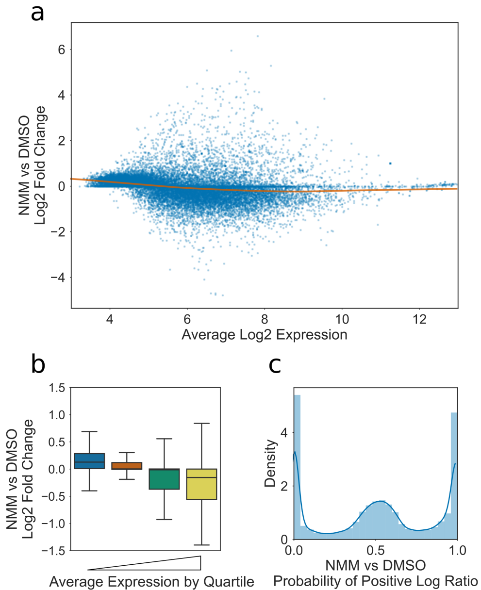
Figure 4.1: Global effect of NMM on Gene Expression. a) MA plot showing relationship between average gene expression and Log2 fold change in expression upon treatment with NMM. Orange line is lowess curve fit showing slight negative correlation between expression and fold change for genes in the expression range 4-8. b) Boxplot of Log2 fold change in expression upon treatment with NMM, cut on quartiles by average expression. Lowest expressed 25% is leftmost, and highest expressed is rightmost. Lower quartile, median, and upper quartile are at 4.6, 5.4, and 6.5, respectively. c) Histogram and kernel density estimate showing distribution of Probability of Positive Log Ratio (PPLR) values. PPLRs which tend towards zero represent negatively differentially expressed genes, whilst PPLRs which tend towards one represent positively differentially expressed genes.
