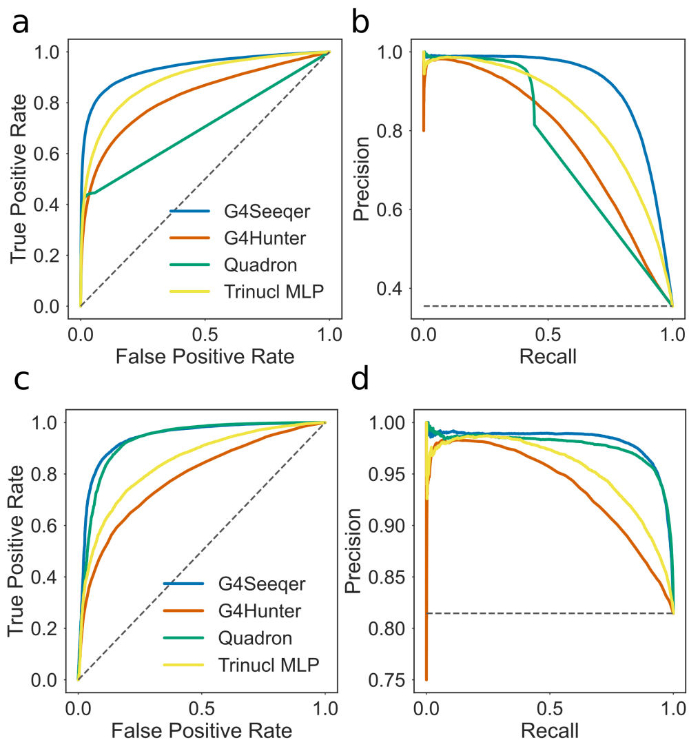
Figure 2.3: Validation curves for G4Seeqer method a) Receiver Operator Characteristic (ROC) curve showing the performance of G4Seeqer, Multi-Layer Perceptron (MLP) trained on trinucleotide contents, Quadron, a Gradient Boosted Machine model (Sahakyan et al. 2017) and the G4Hunter method (Bedrat et al. 2016), on a held out test set of the G4Seq dataset (10% of total dataset). b) Precision-recall curves showing the performance of G4Seeqer, trinucleotide MLP, Quadron, and G4Hunter on the same dataset. c) ROC curve and d) Precision Recall curve showing the performance on sequences from the test set conforming to the Quadparser motif.
