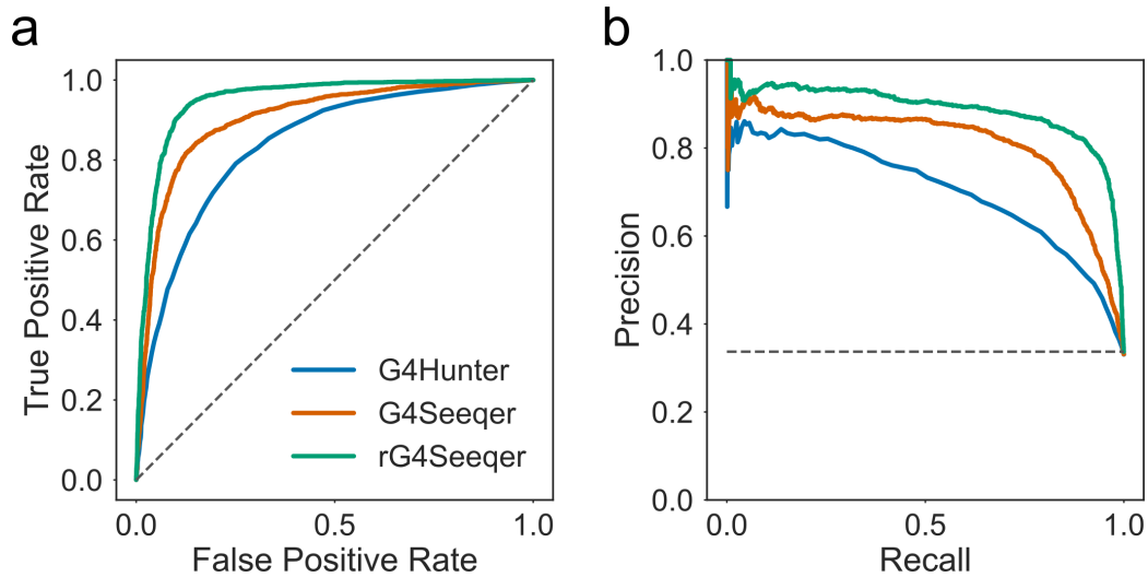
Figure 2.5: Validation curves for rG4Seeqer method a) Receiver Operator Characteristic (ROC) curves showing the performance of rG4Seeqer, G4Seeqer and the G4Hunter method (Bedrat et al. 2016), on a held out test set of the rG4Seq dataset (10% of total dataset). b) Precision-recall curves showing the performance of rG4Seeqer, G4Seeqer, and G4Hunter on the same dataset.
