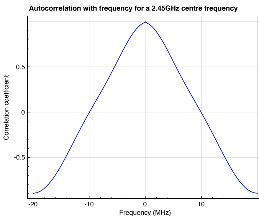
Figure 7.16: Frequency autocorrelation for 2 adjacent cavity transmission (measurement 4)
