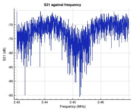
Figure 7.25: Frequency response for diagonal coupling (measurement 7)
