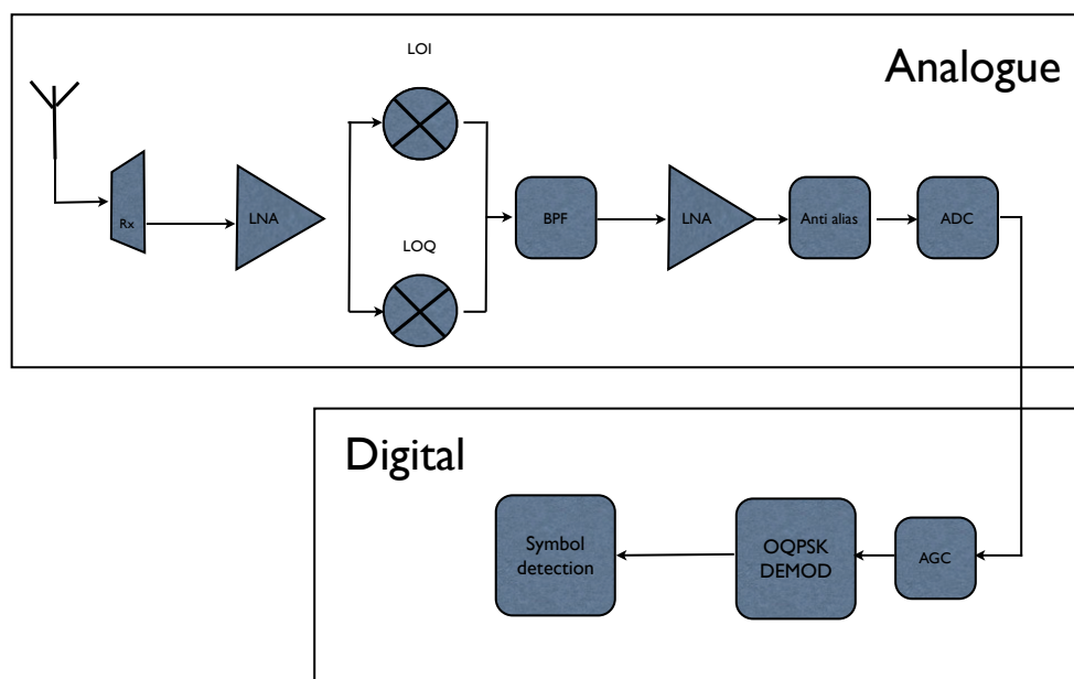
Figure C.1: Overview of Jennic's 5139 chipset receiver section
