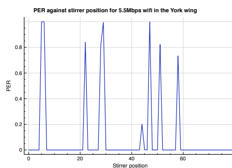
Figure 8.23: 802.11b performance in the empty wing at a data rate of 5-5Mbps with antenna diversity
