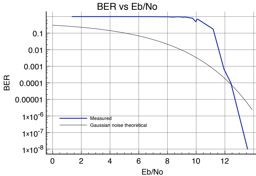
Figure 6.32: BERs against signal to noise ratio for ZigBee in an anechoic chamber
