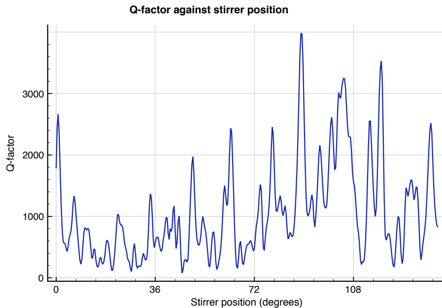
Figure 5.8: Variation of Q-factor for reverb chamber with 6 absorber pieces
