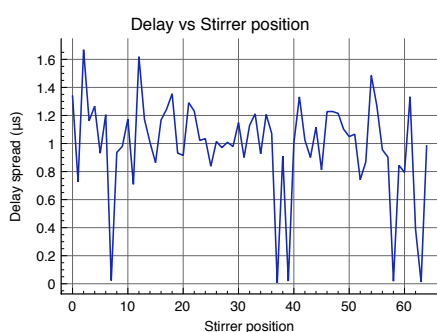
Figure 4.21: Variation of delay spread over 60 independent stirrer positions, 80MHz bandwidth
