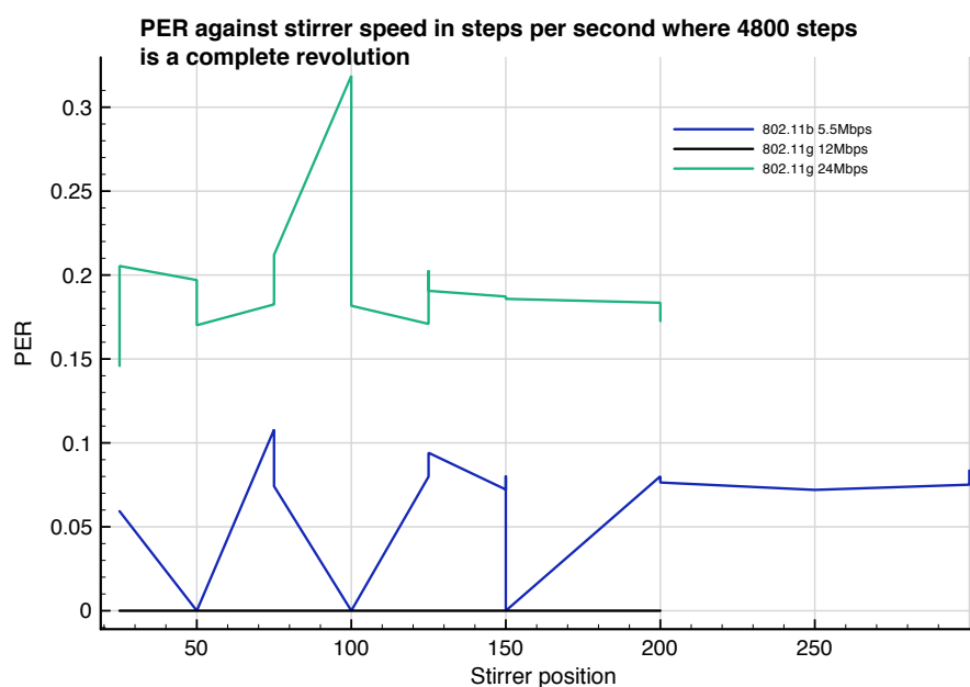
Figure 8.29: 802.11 performance in a time varying channel
