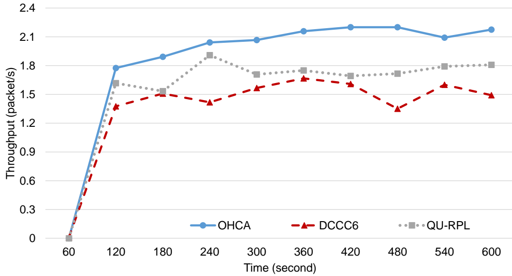
Figure 6.4: Throughput
