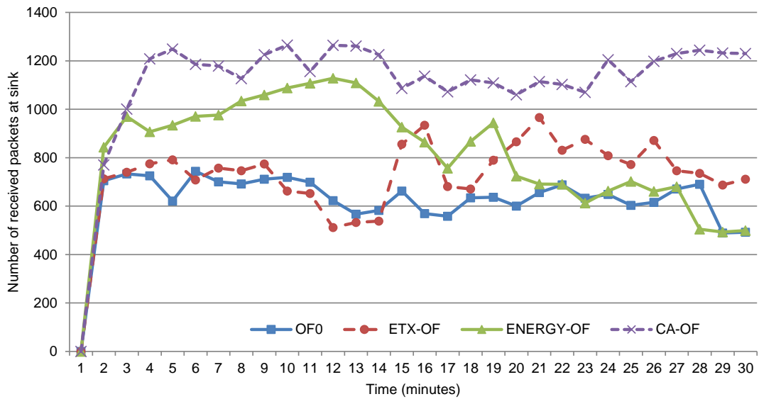
Figure 4.7: Network 2 throughput
