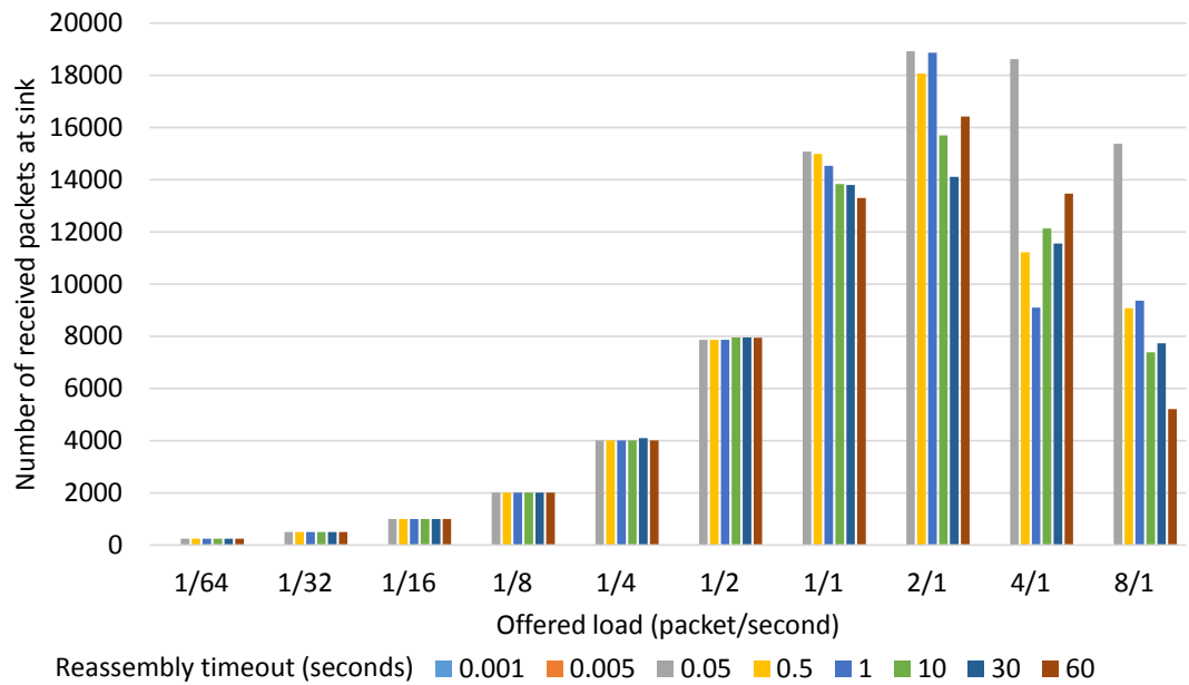
Figure 3.28: Number of received packets (when broken into two fragments) for simulation test
