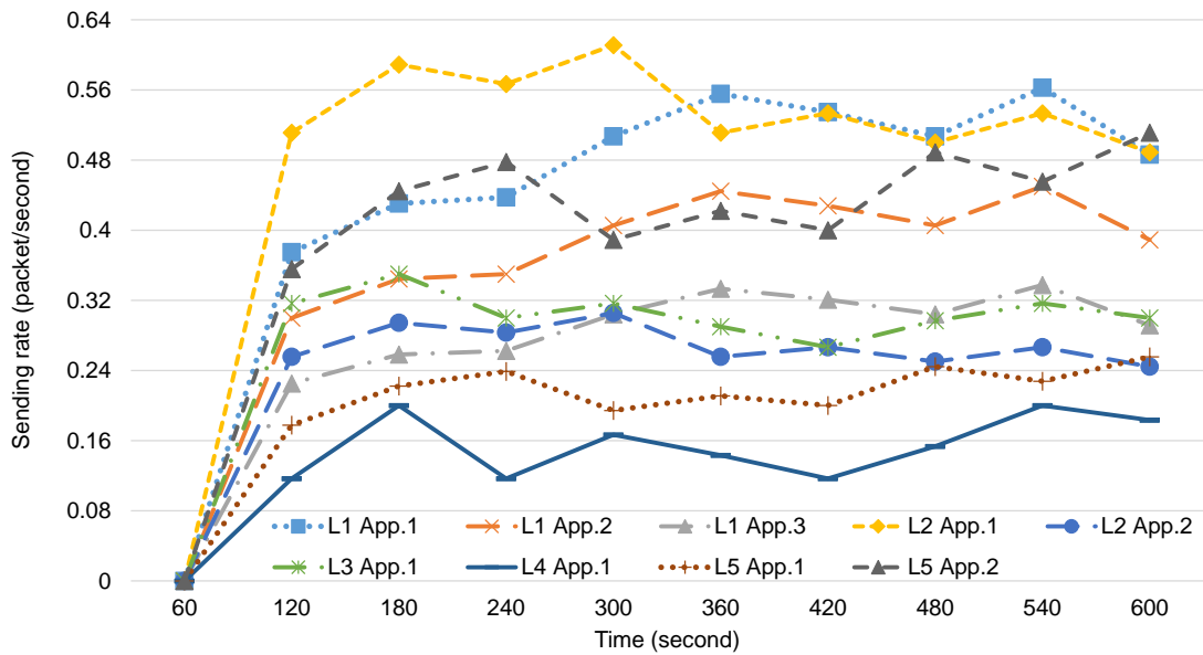
Figure 5.12: Applications' sending rate for GTCCF
