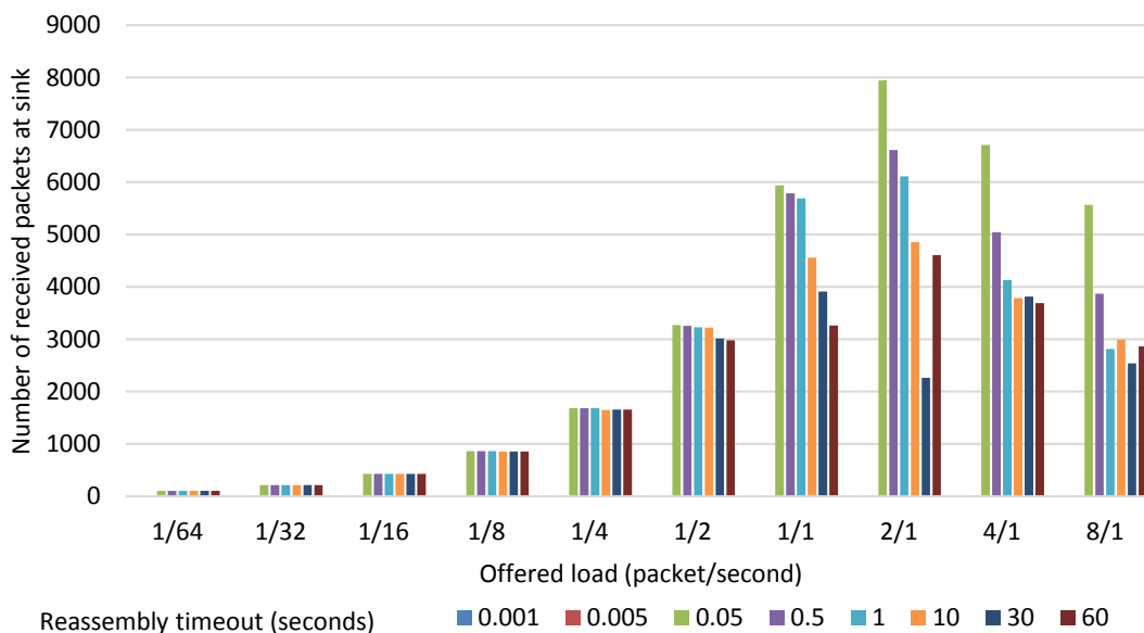
Figure 3.20: Number of received packets (when broken into four fragments) at sink in 5-node network
