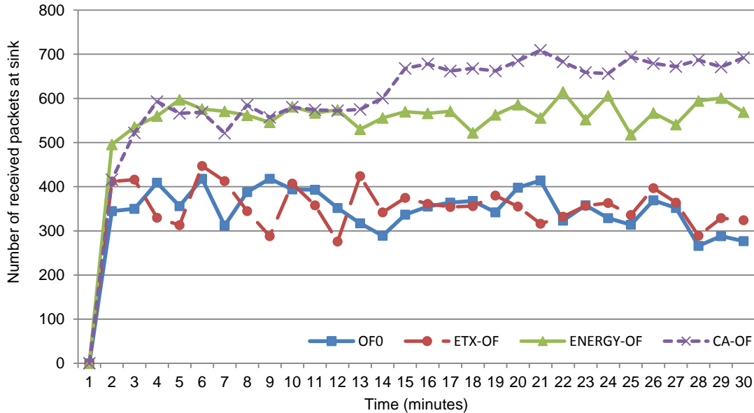
Figure 4.3: Network 1 throughput
