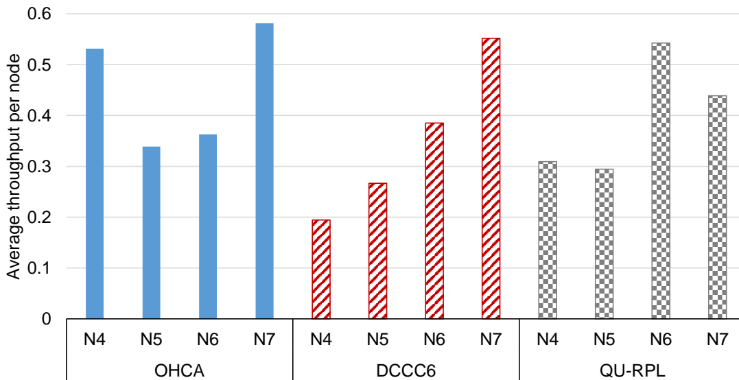
Figure 6.5: Received packets/s from nodes in scenario 1
