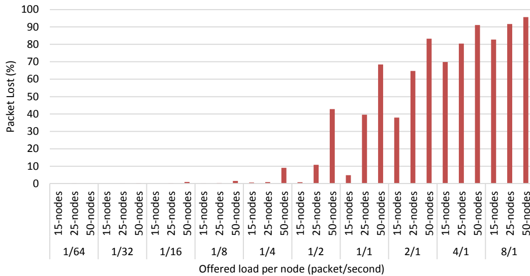
Figure 3.13: Packet loss [buffer size = 16 packets]
