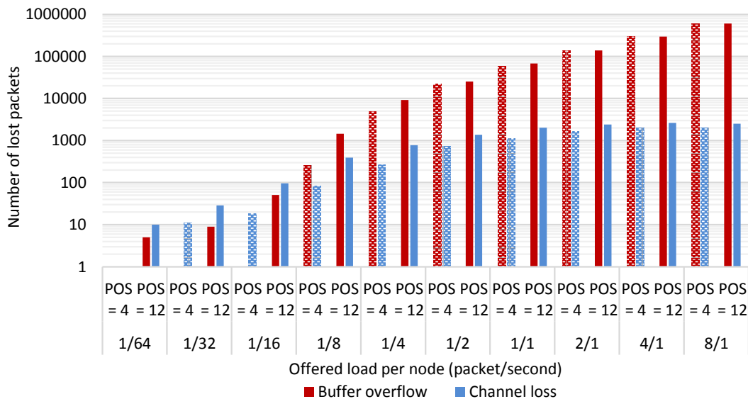
Figure 3.16: Number of lost packets due to buffer overflow and wireless channel loss with varying POS
