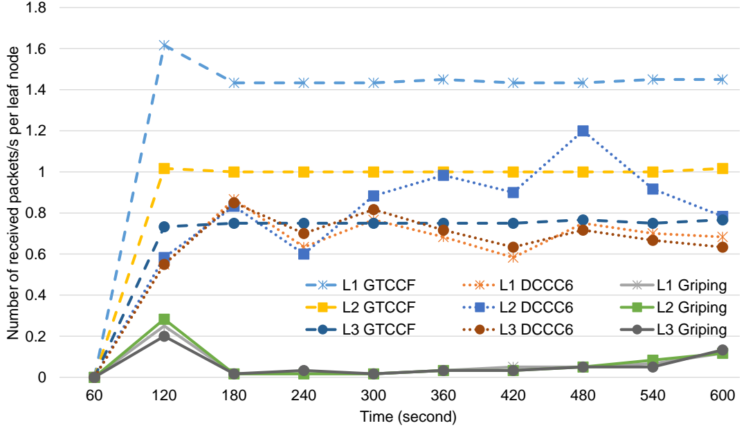
Figure 5.3: Number of received packets/s from leaf nodes at sink
