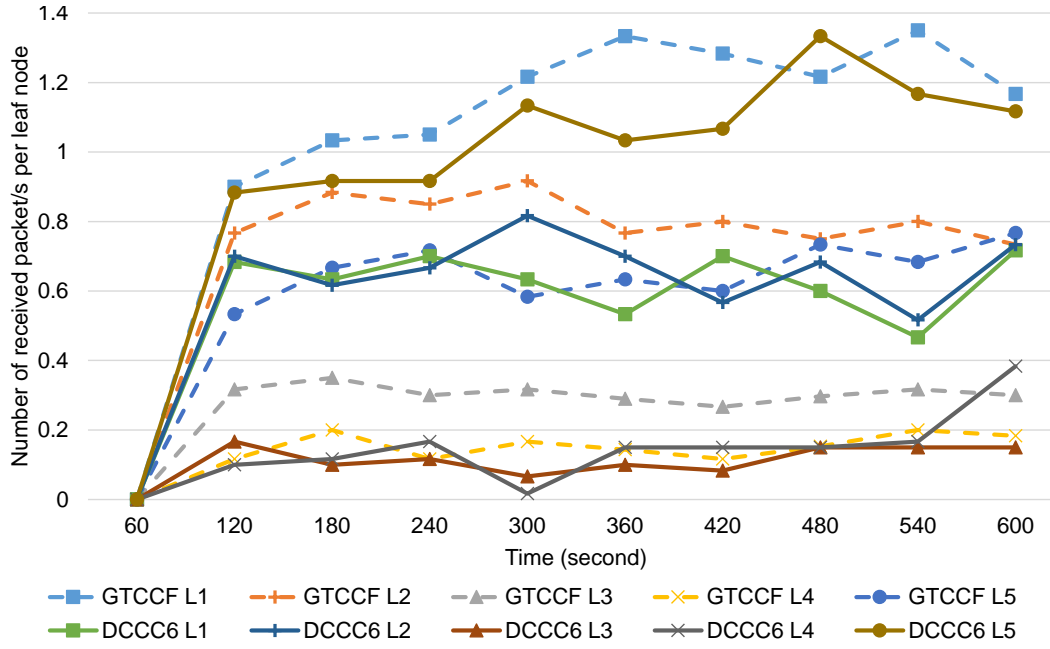
Figure 5.10: Number of received packets/s from leaf nodes at sink
