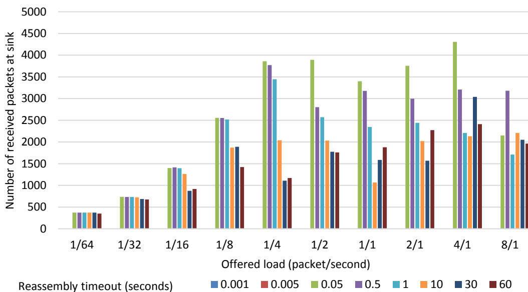
Figure 3.21: Number of received packets (when broken into four fragments) at sink in 15-node network
