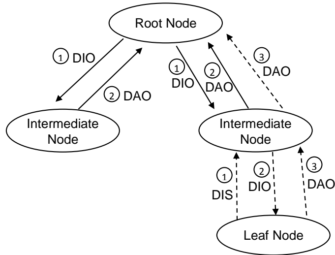
Figure 1.5: DODAG construction process [19]
