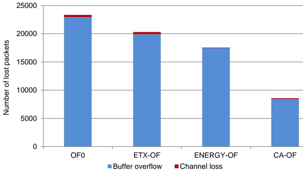
Figure 4.6: Total number of lost packets in network 2
