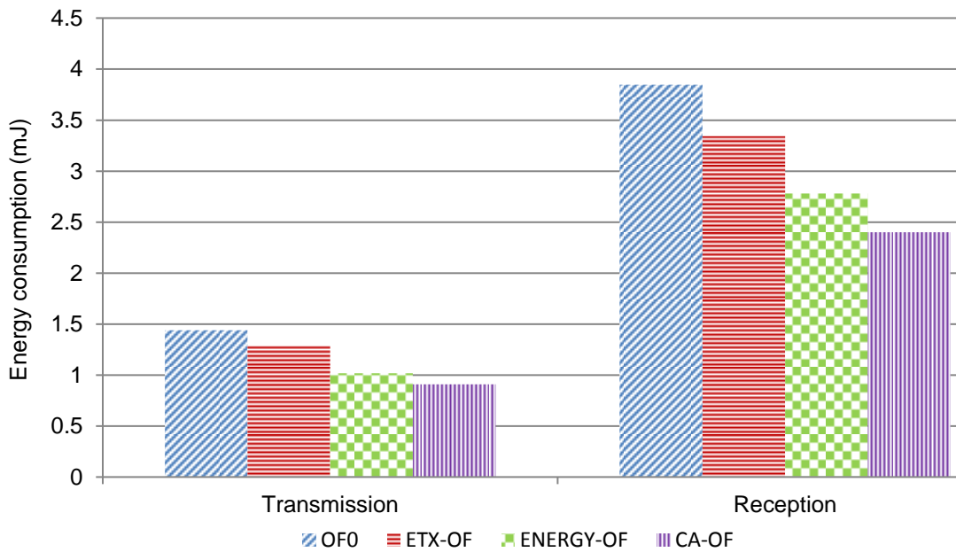
Figure 4.5: Tx and Rx energy consumption per successful packet in network 1
