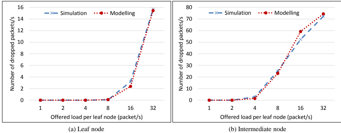
Figure 3.8: Average number of dropped packets with various offered loads
