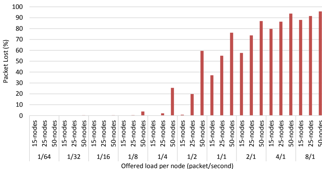
Figure 3.11: Packet loss [buffer size = 8 packets]
