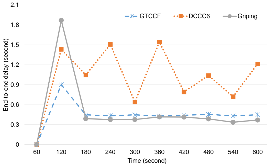
Figure 5.6: End-to-end delay
