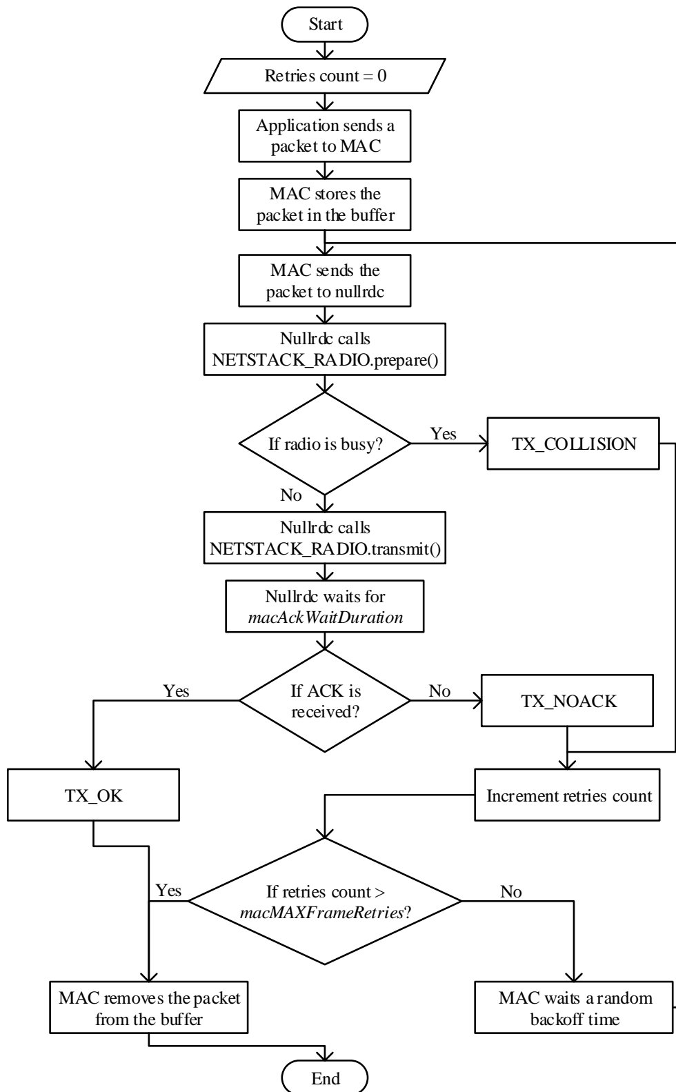
Figure 3.4: Packet transmission process in Contiki OS
