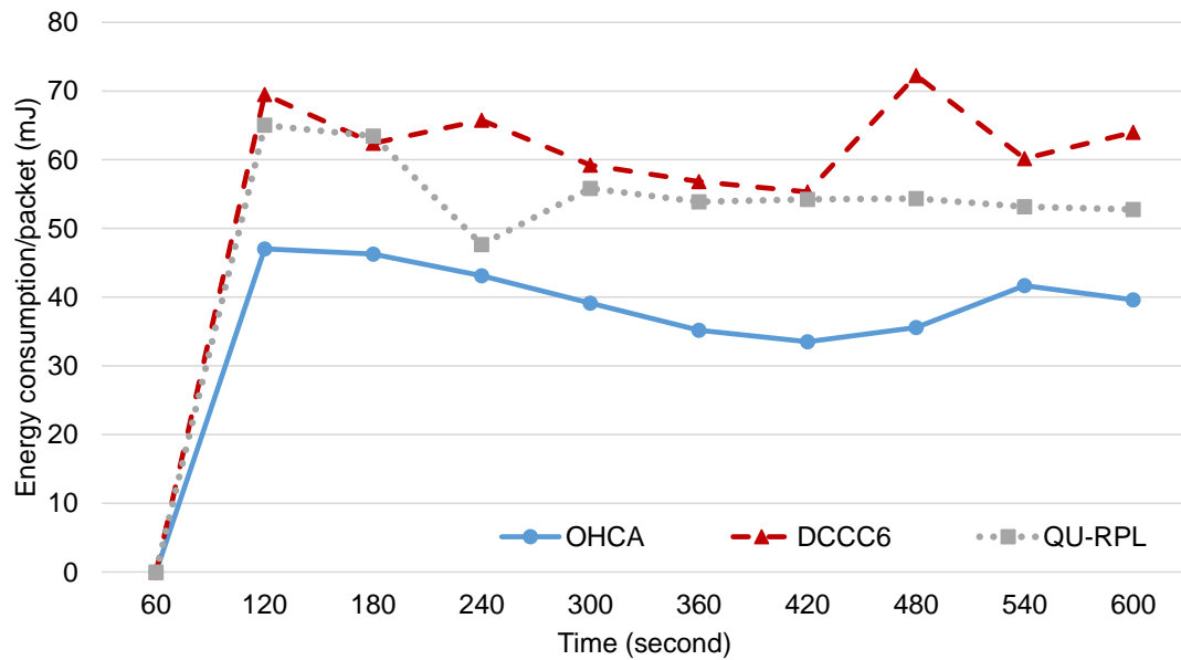
Figure 6.11: Energy consumption per successful packet
