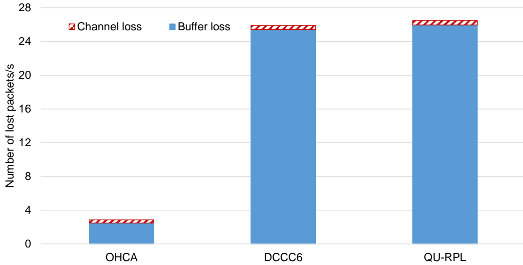
Figure 6.12: Number of lost packets
