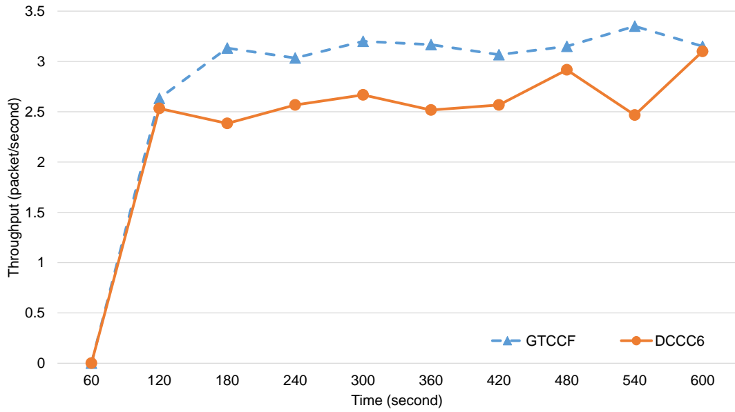
Figure 5.11: Number of received packets/second at sink
