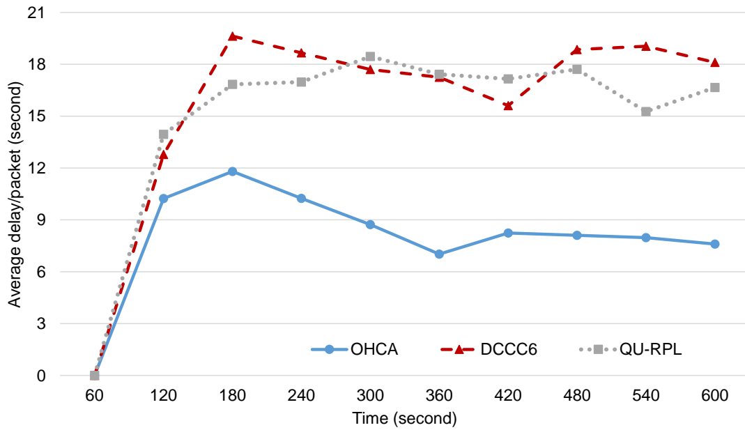
Figure 6.10: End-to-end delay
