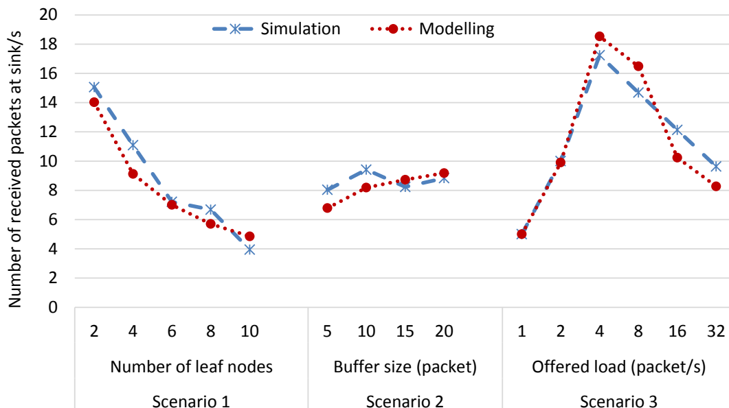
Figure 3.9: Average number of received packets at sink node
