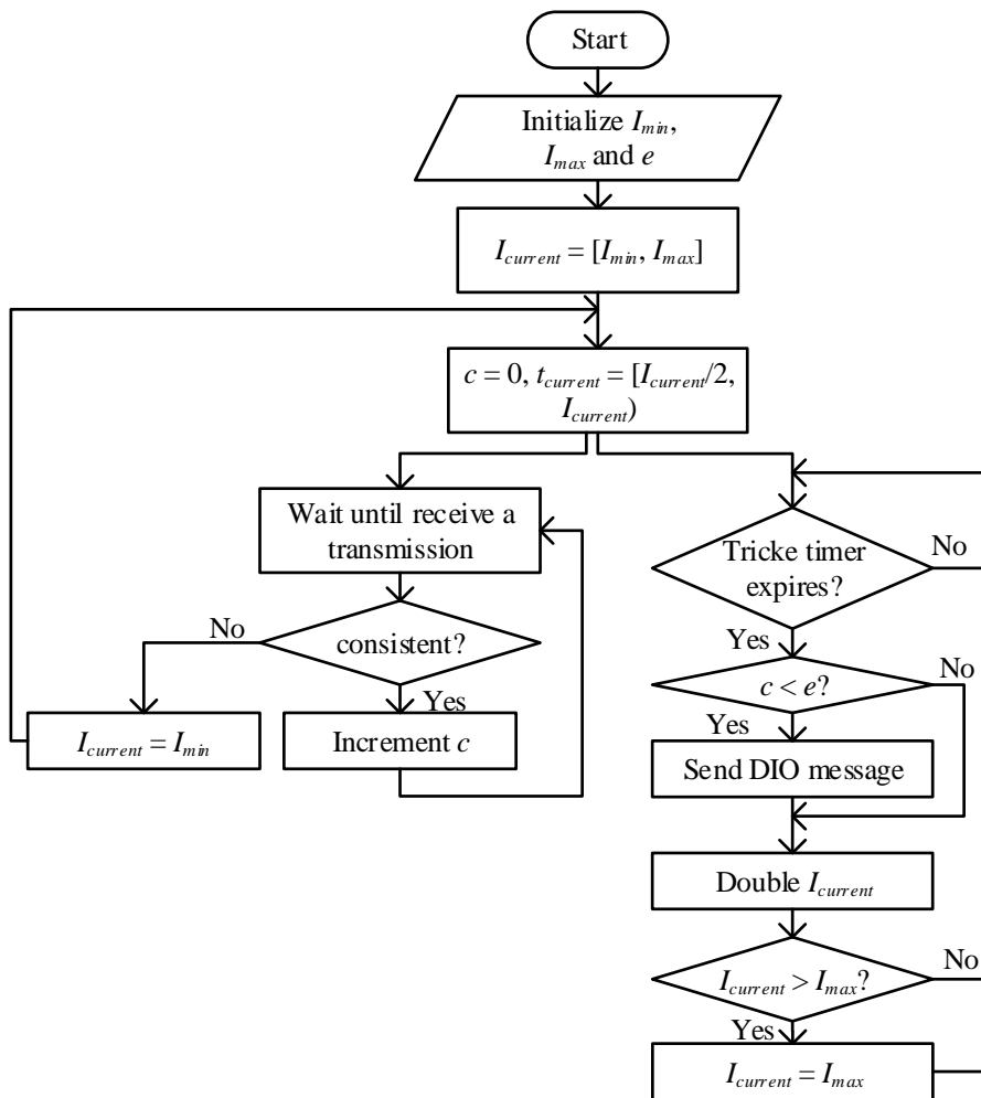
Figure 1.6: Trickle algorithm
