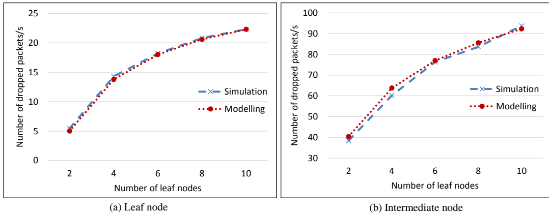
Figure 3.6: Average number of dropped packets with different number of leaf nodes
