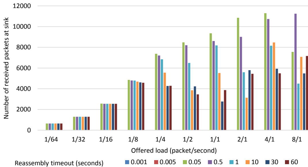
Figure 3.19: Number of received packets (when broken into two fragments) at sink in 25-node network
