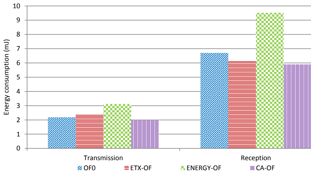
Figure 4.13: Tx and RX energy consumption per successful packet in network 3
