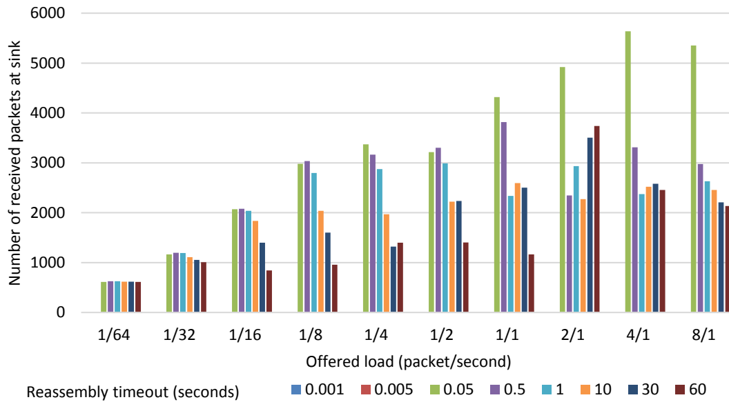
Figure 3.22: Number of received packets (when broken into four fragments) at sink in 25-node network
