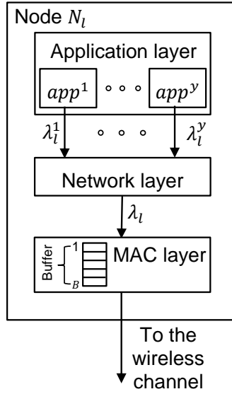
Figure 6.2: Node model
