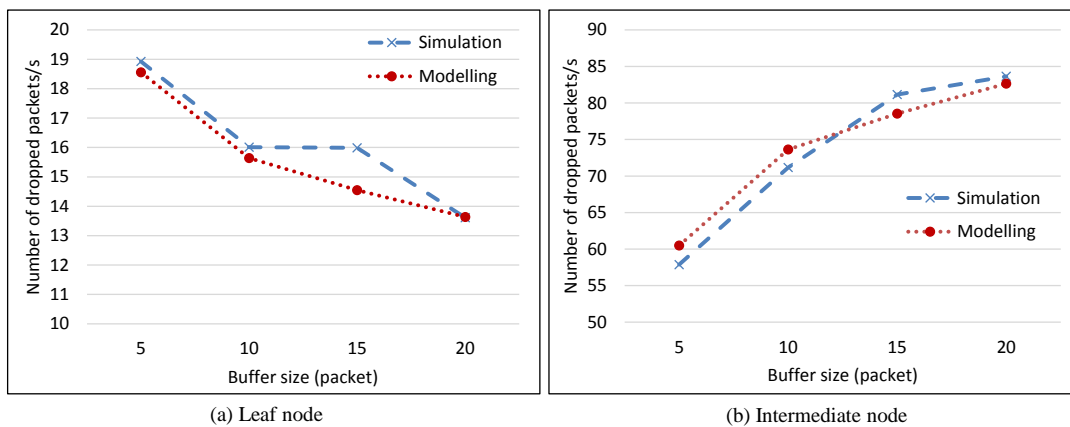
Figure 3.7: Average number of dropped packets with different buffer sizes
