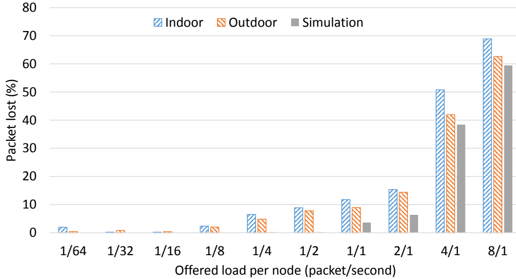
Figure 3.25: Packet loss [buffer size = 16 packets]
