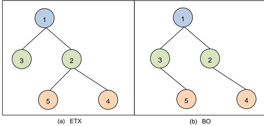
Figure 4.1: Network topology within congestion
