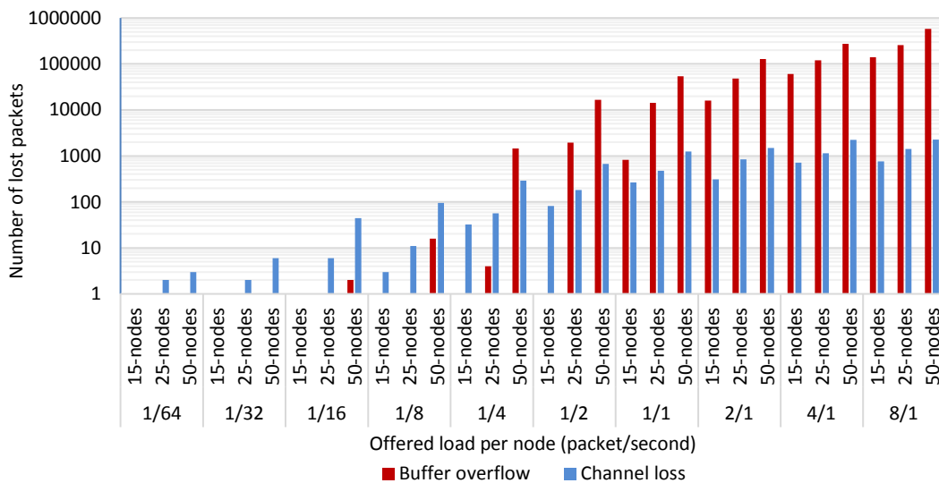
Figure 3.14: Number of lost packets due to buffer overflow and wireless channel loss [buffer size = 16 packets]
