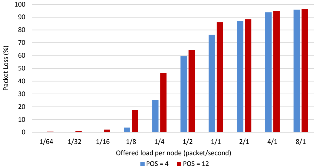
Figure 3.15: Packet loss with varying POS
