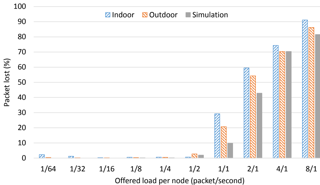
Figure 3.24: Packet loss [buffer size = 8 packets]
