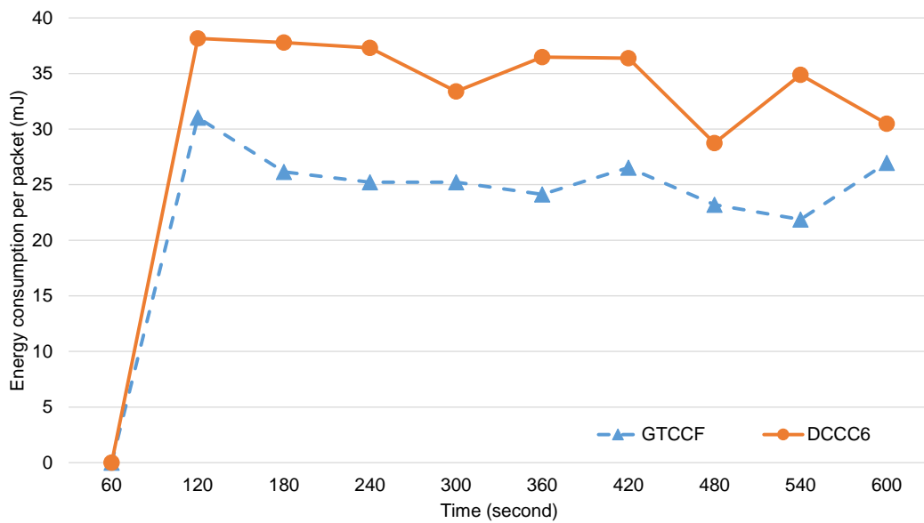
Figure 5.14: Energy consumption per successful packet
