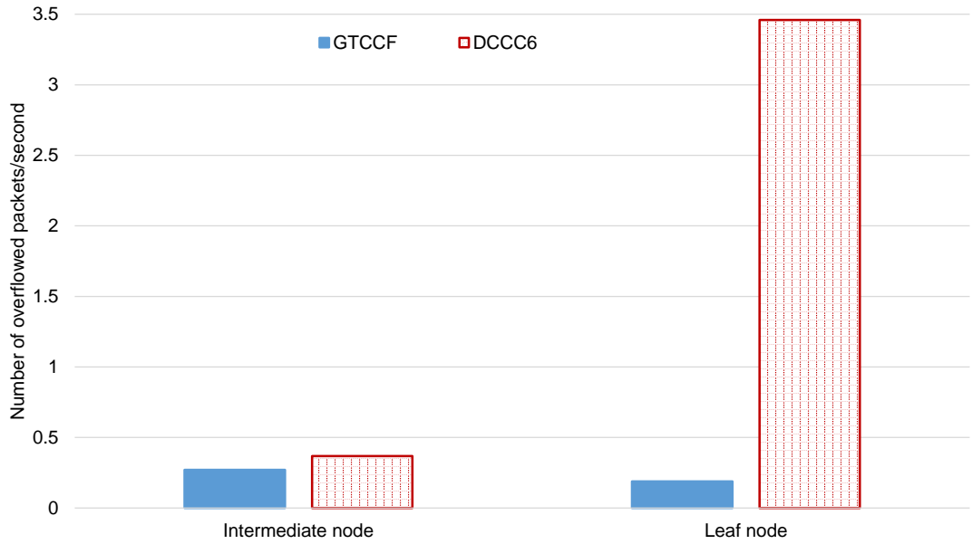
Figure 5.15: Number of lost packets
