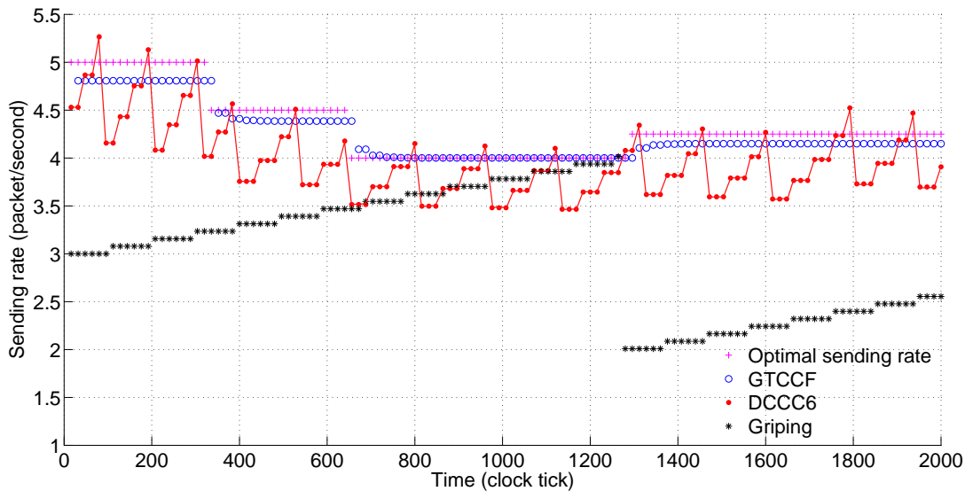
Figure 5.2: Sending rate adaptation comparison
