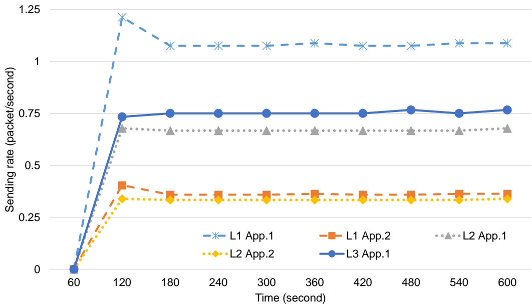
Figure 5.5: Applications' sending rate for GTCCF
