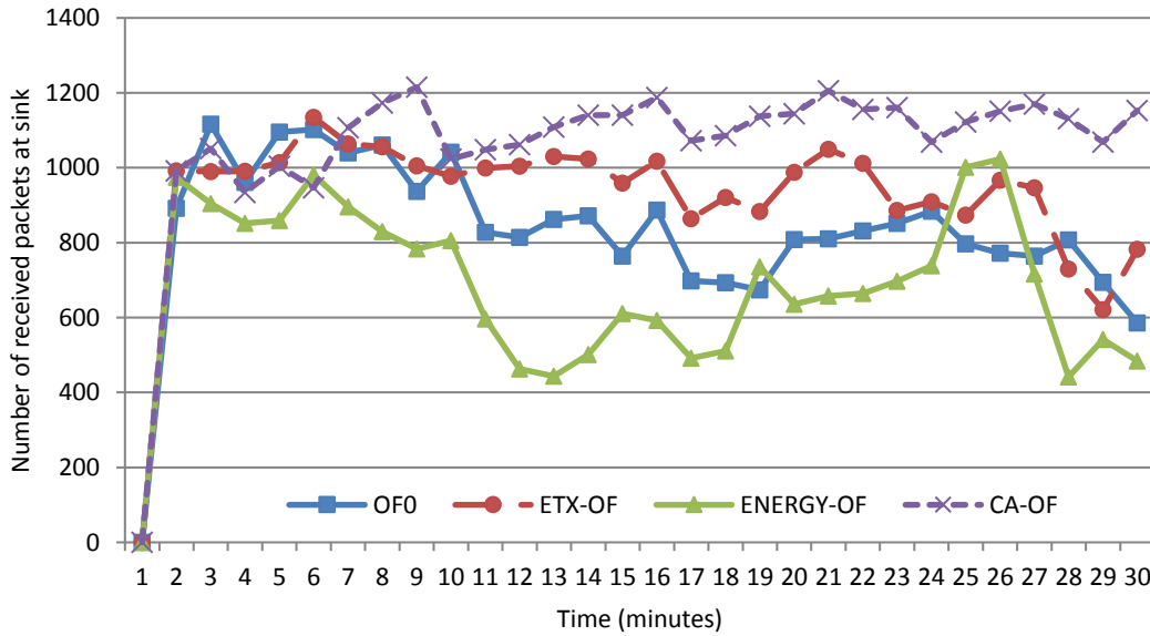
Figure 4.11: Network 3 throughput
