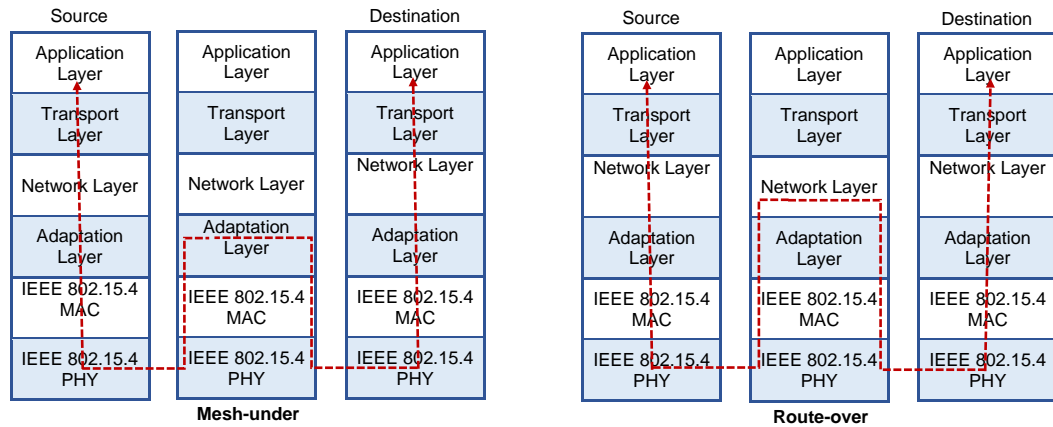
Figure 1.4: Mesh-under vs route-over
