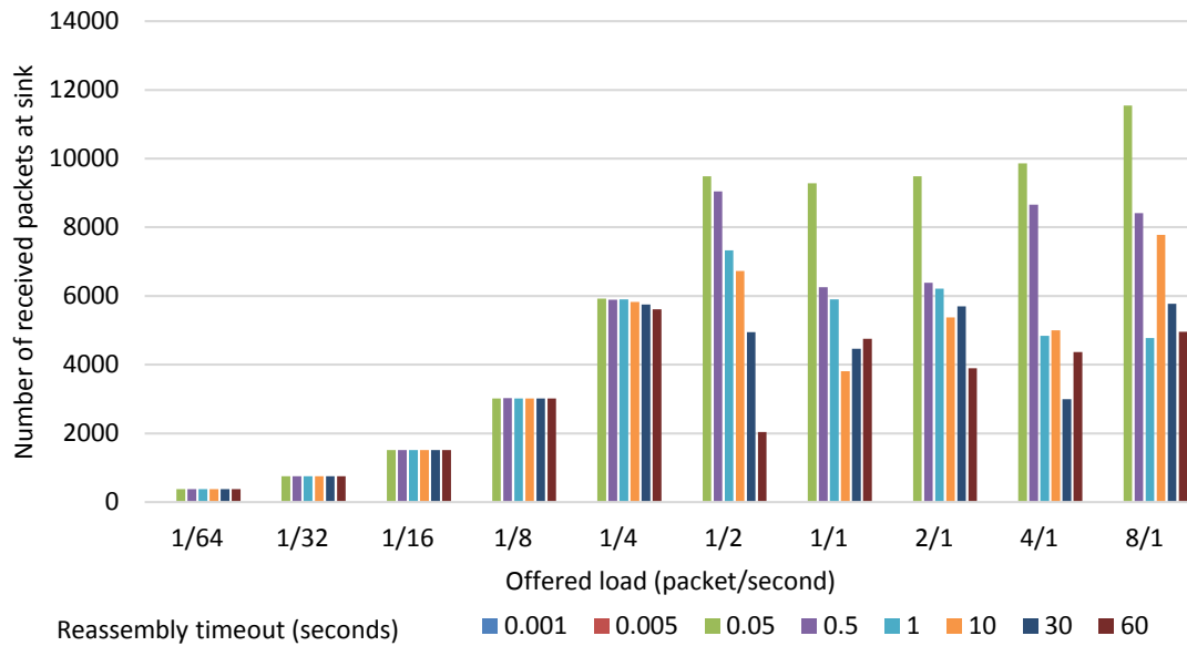
Figure 3.18: Number of received packets (when broken into two fragments) at sink in 15-node network
