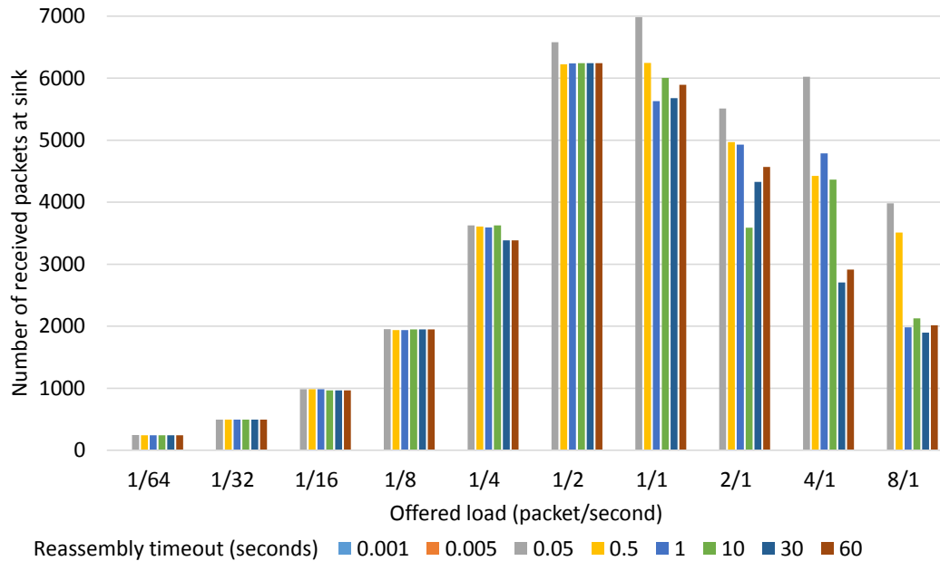
Figure 3.31: Number of received packets (when broken into four fragments) for simulation
