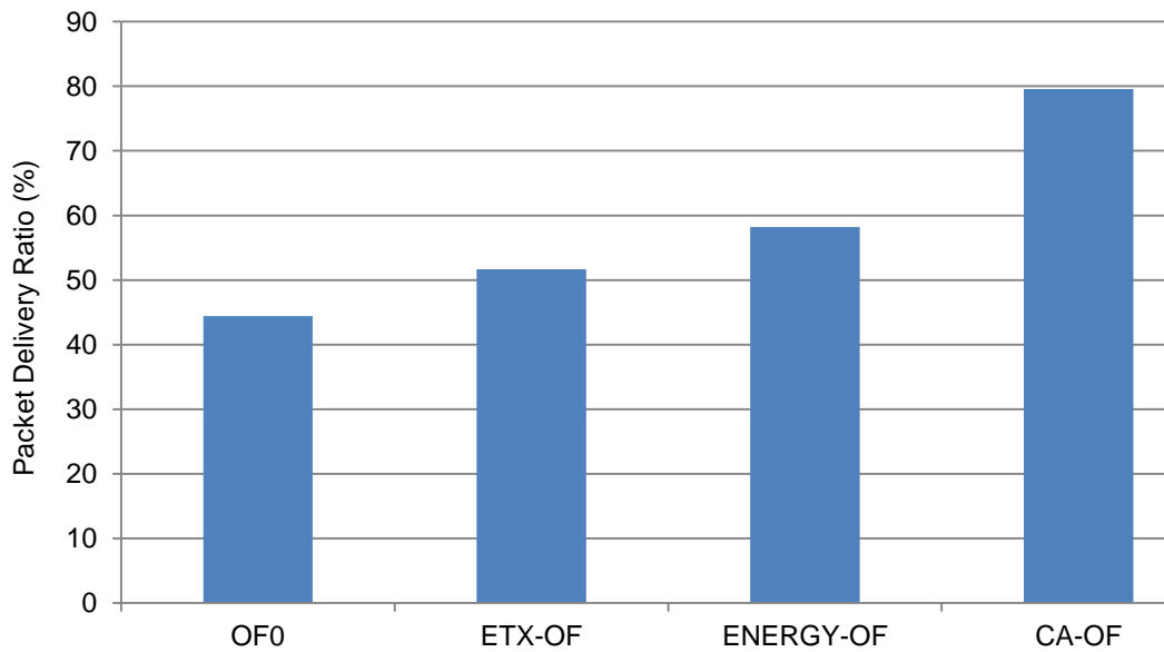
Figure 4.8: Packet Delivery Ratio in network 2
