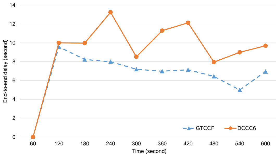
Figure 5.13: End-to-end delay
