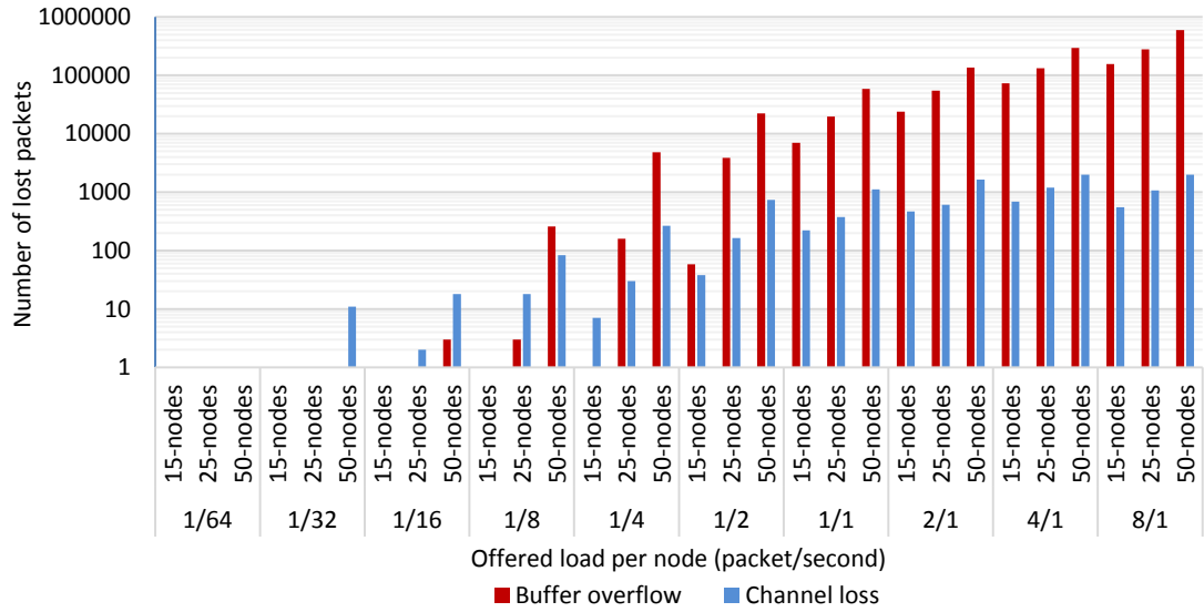
Figure 3.12: Number of lost packets due to buffer overflow and wireless channel loss [buffer size = 8 packets]
