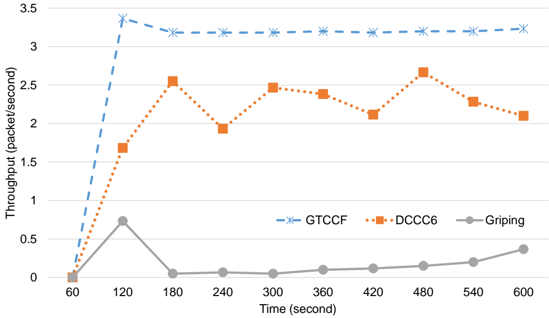
Figure 5.4: Number of received packets/second at sink
