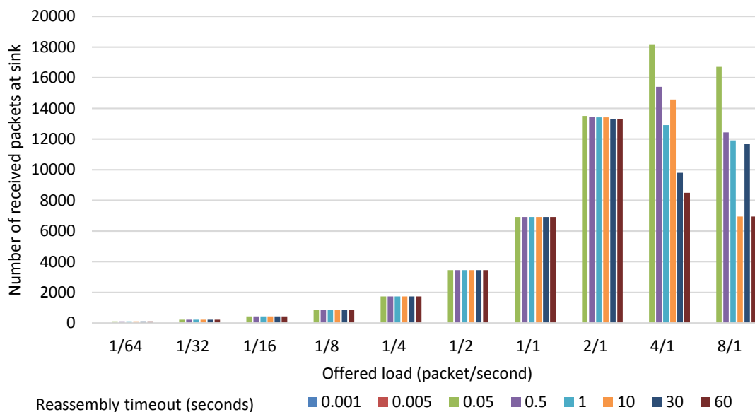
Figure 3.17: Number of received packets (when broken into two fragments) at sink in 5-node network
