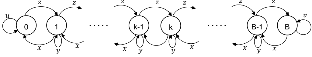
Figure 3.3: State transition diagram
