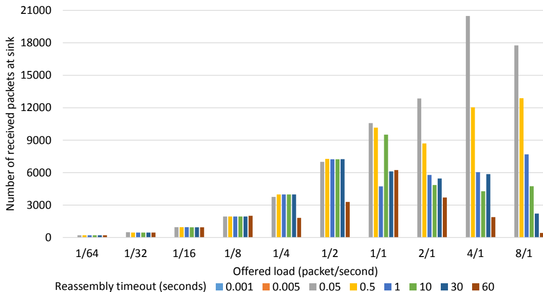
Figure 3.26: Number of received packets (when broken into two fragments) for indoor test
