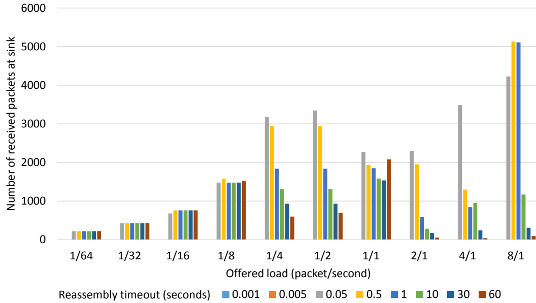
Figure 3.29: Number of received packets (when broken into four fragments) for indoor
