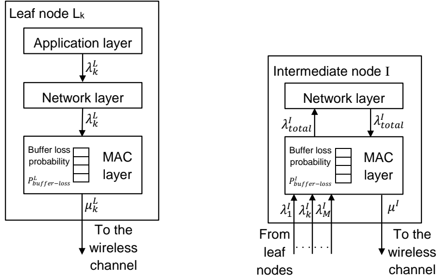
Figure 3.2: Leaf and intermediate nodes model
