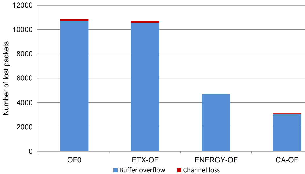
Figure 4.2: Total number of lost packets in network 1
