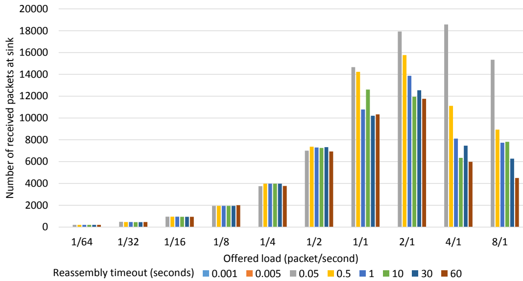
Figure 3.27: Number of received packets (when broken into two fragments) for outdoor test
