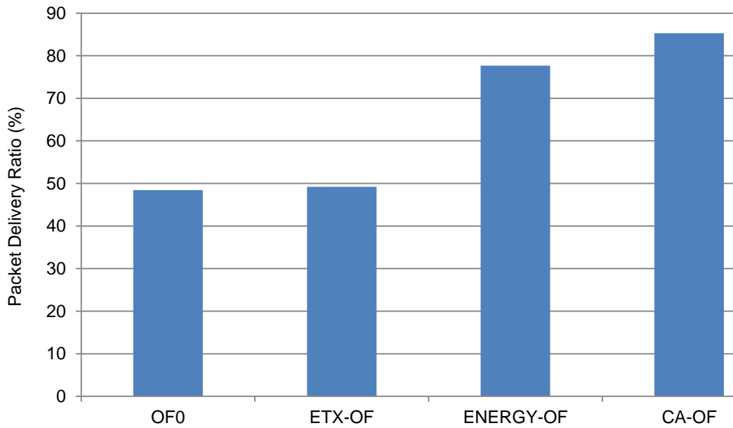
Figure 4.4: Packet Delivery Ratio in network 1
