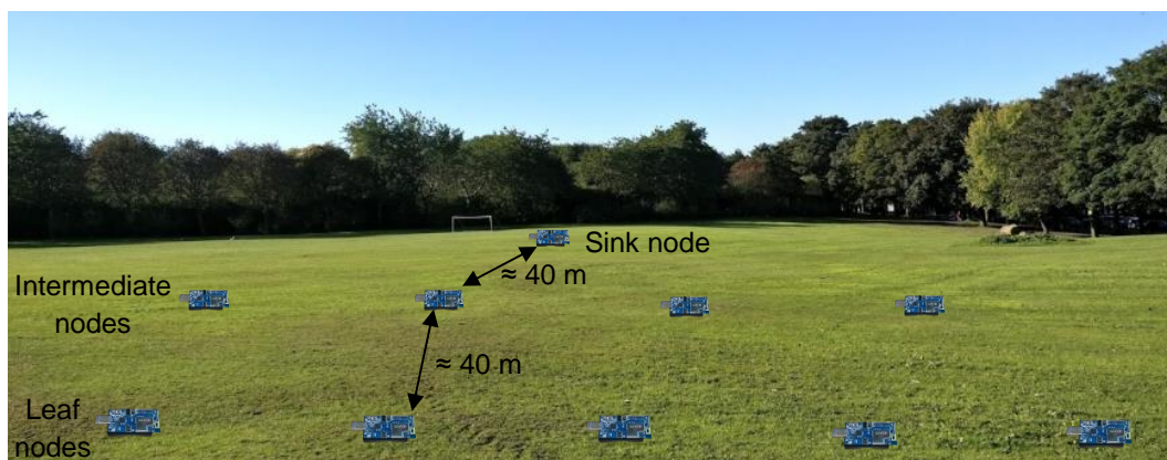
Figure 3.23: Real sensor nodes distribution in testbed experiments
