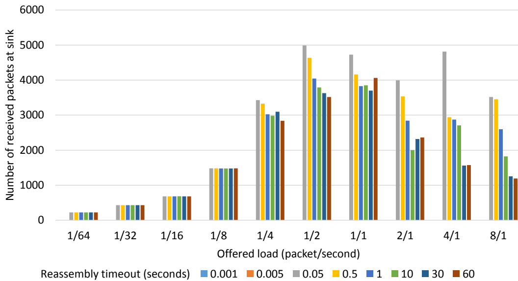
Figure 3.30: Number of received packets (when broken into four fragments) for outdoor
