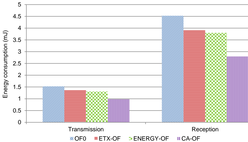
Figure 4.9: Tx and Rx energy consumption per successful packet in network 2
