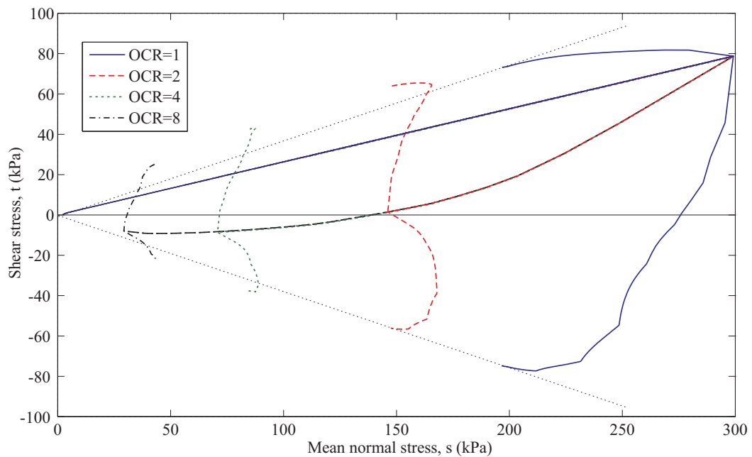
Figure 3.6: Stress path plots for differing overconsolidation ratios
