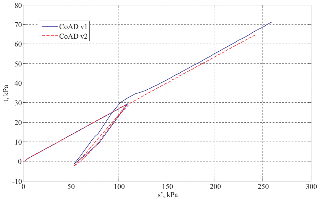
Figure 4.9: Stress path plots for swelling and recompression tests showing the comparison between the two CoAD models
