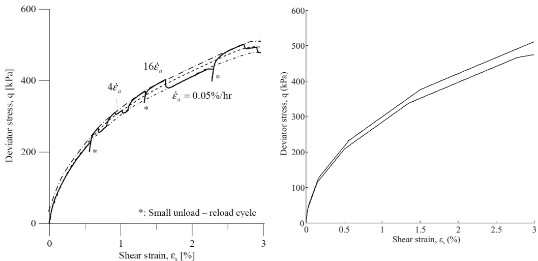
(a) Stress-strain behaviour during triaxial compression tests on London clay (b) Stress-strain behaviour predicted by the SRD model
