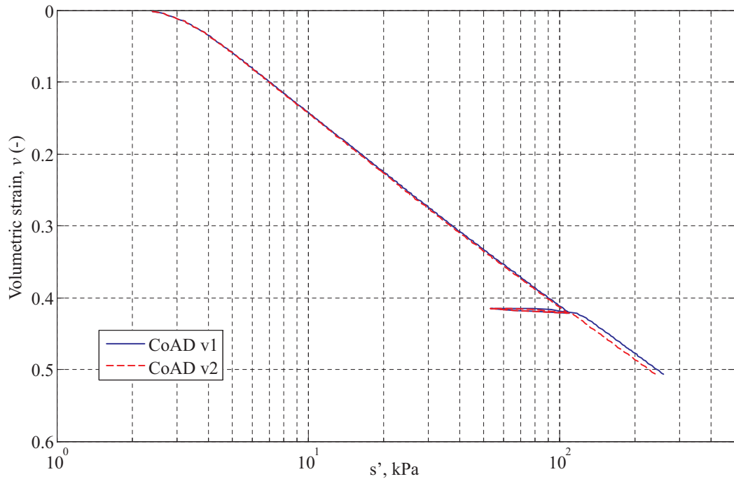
Figure 4.10: Volumetric strain versus mean stress plot for swelling and recompression tests, for both CoAD models
