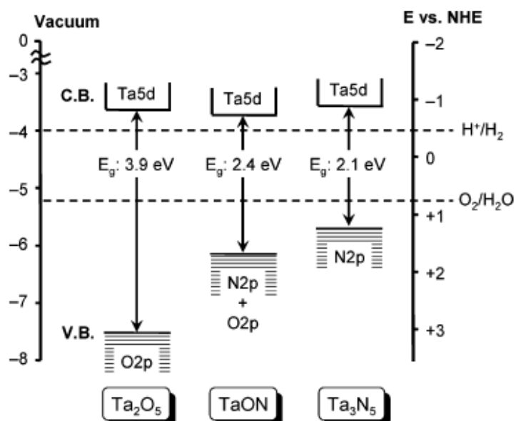
Fig. 1.8. Band structures of Ta 2 O 5 , TaON and Ta 3 N 5
