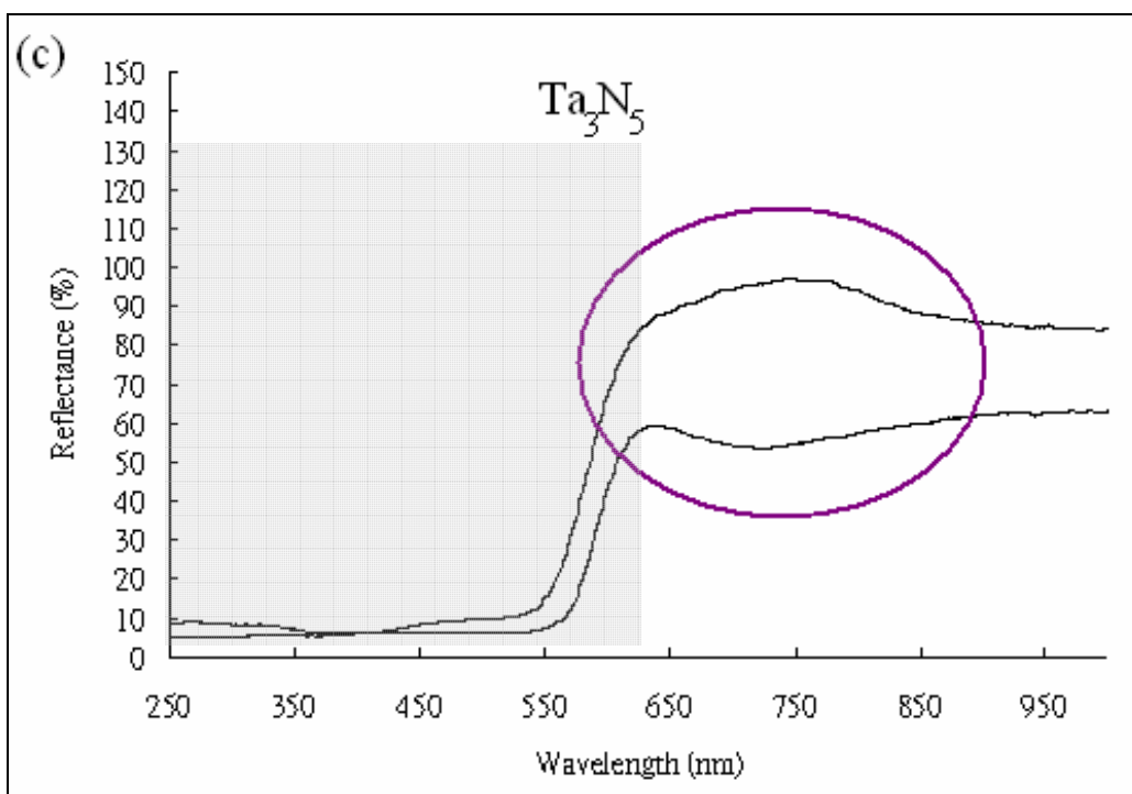
Fig. 2.10 Reflectance of a) Ta 2 O 5 ; b) TaON and c) Ta 3 N 5
