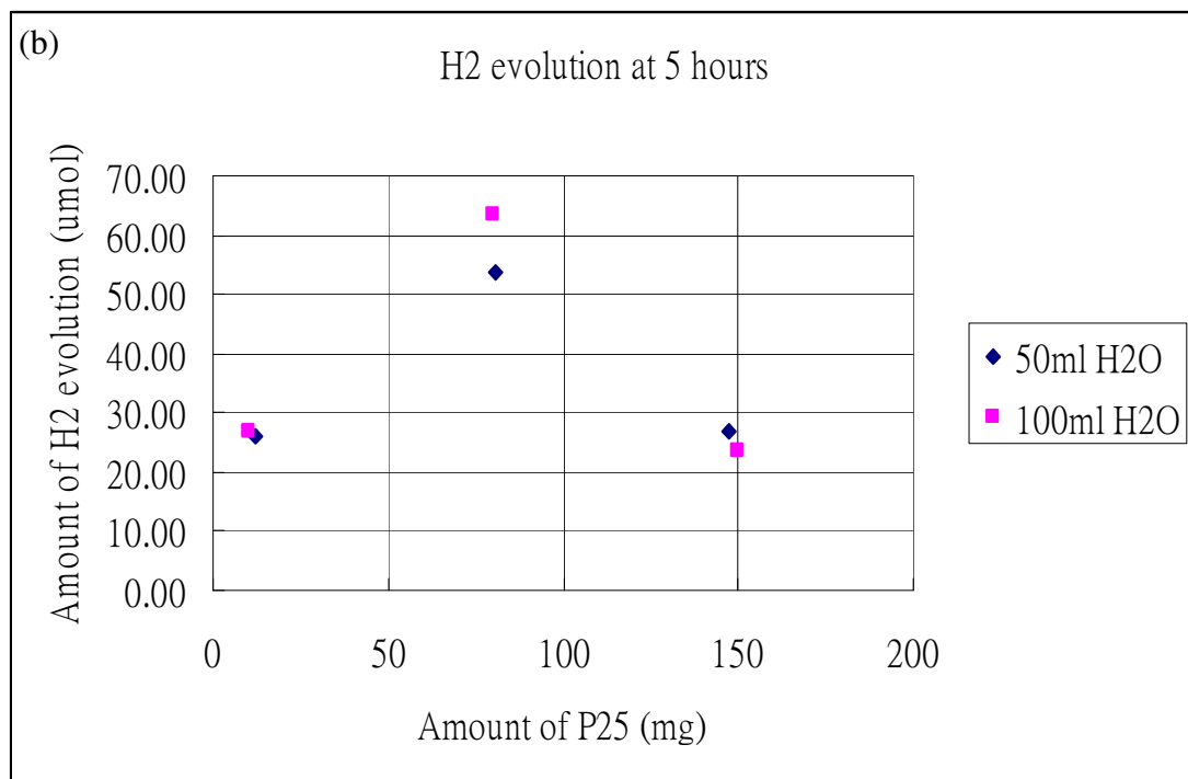
Fig. 3.6 Comparison of 50ml and 100ml H 2 O added to the catalytic cell with 10ml MeOH at 40 °C. a) The amount of H 2 production of the P25 catalytic system; b) amount of H 2 evolution after 5 hours photolysis of P25.
