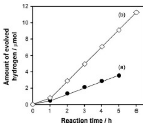
Fig. 1.10 H_2 evolution of (a) reference- Ta_3N_5 and (b) nanoparticle- Ta_3N_5 with the presence of methanol and Pt co-catalyst loaded. [23]
