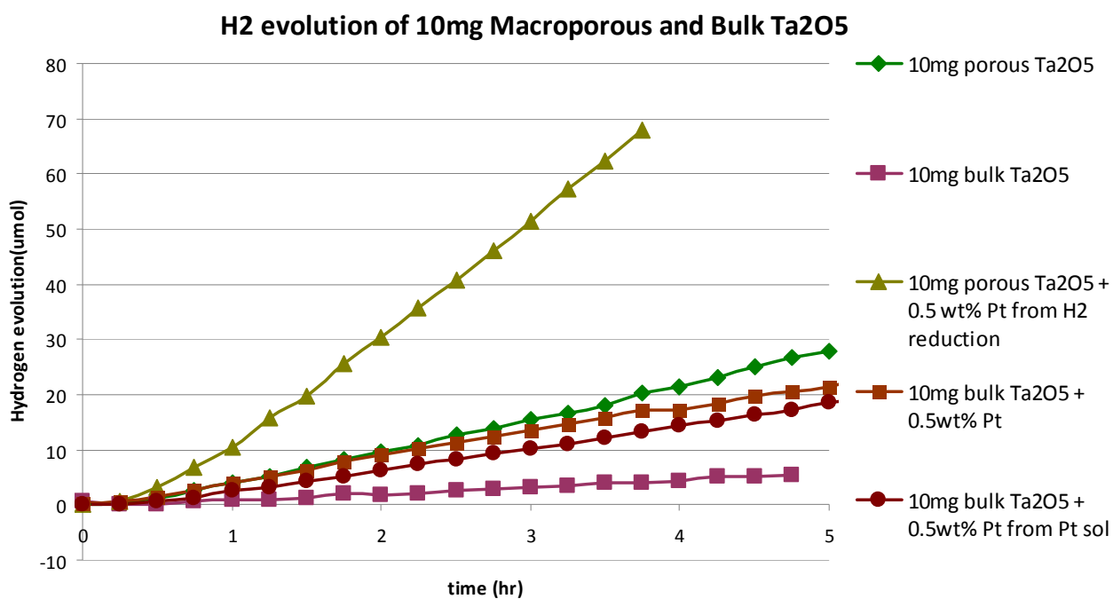
Fig. 2.12 Hydrogen evolution of bulk and macroporous Ta_2O_5 with/without presence of 0.5wt% Pt co-catalyst illuminated using Uv-Vis from a 300 W Xe lamp.
