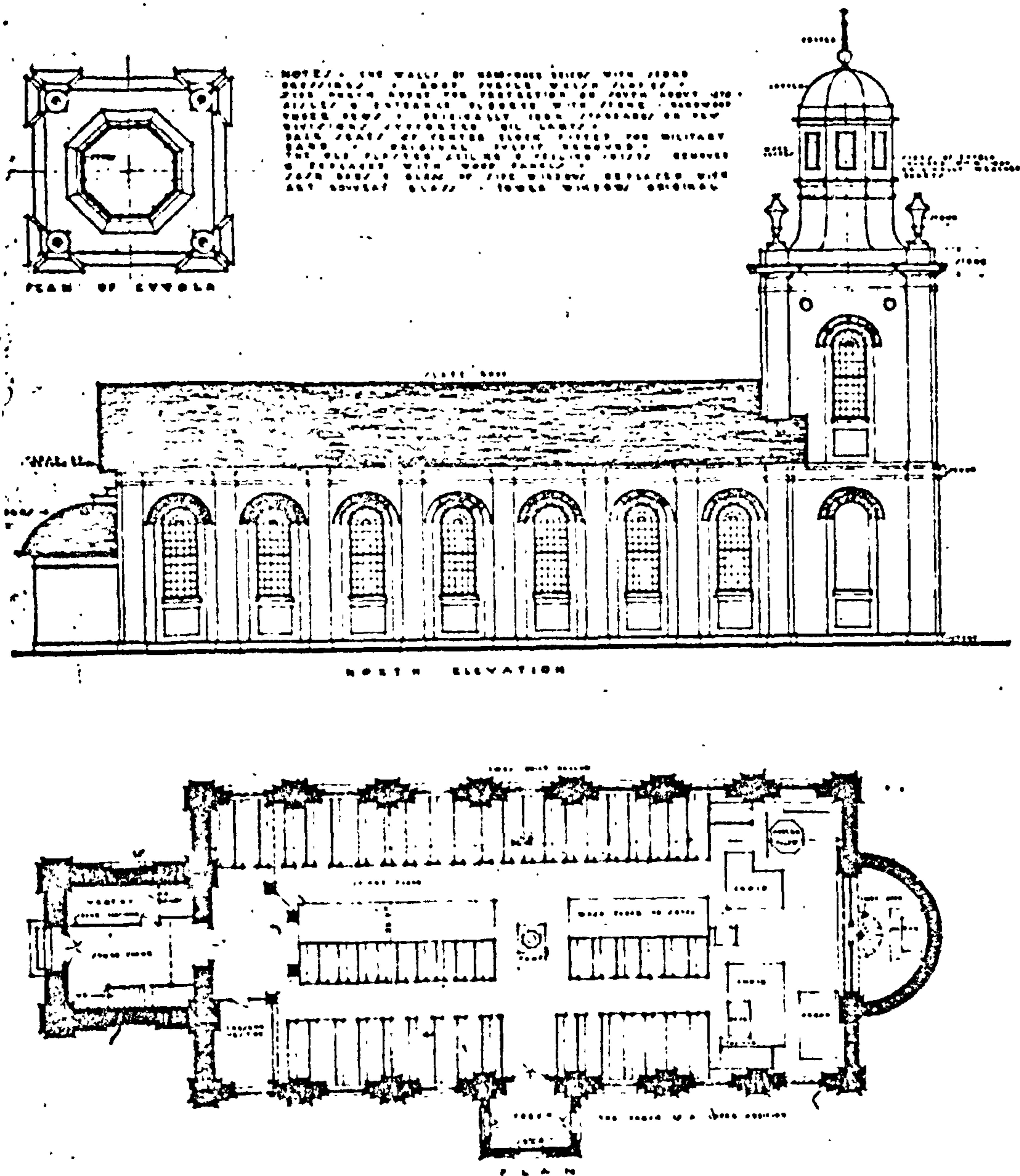
Fig. 5. St. Matthew's Windsor, by Francis Greenway: drawn by W. Hardy Wilson.
