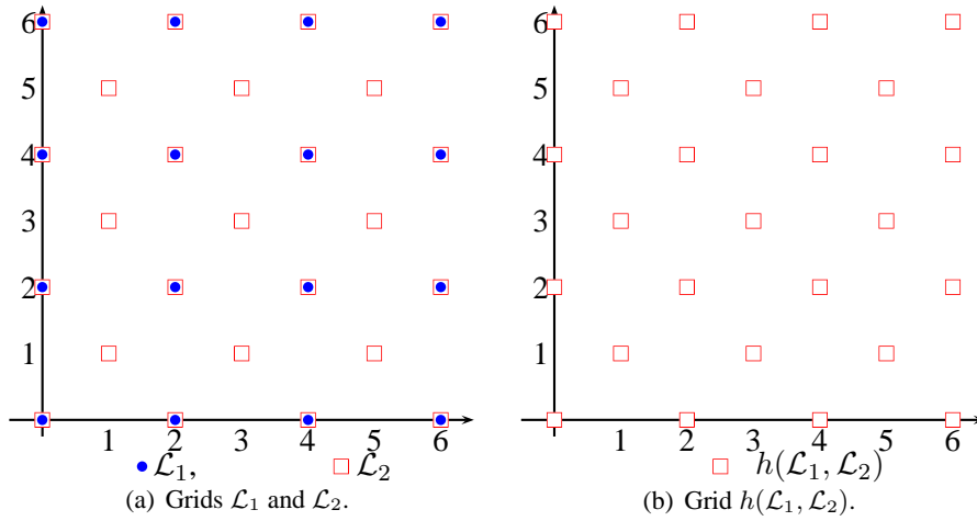
Figure 5.3: Grid Widening.
