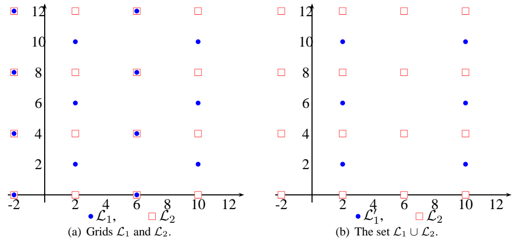
Figure 4.4: The union of two grids.
