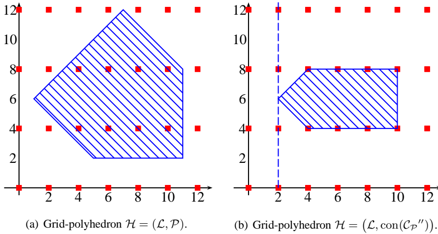
Figure 7.9: Proposition 7.12 does not hold for grid-octagons.
