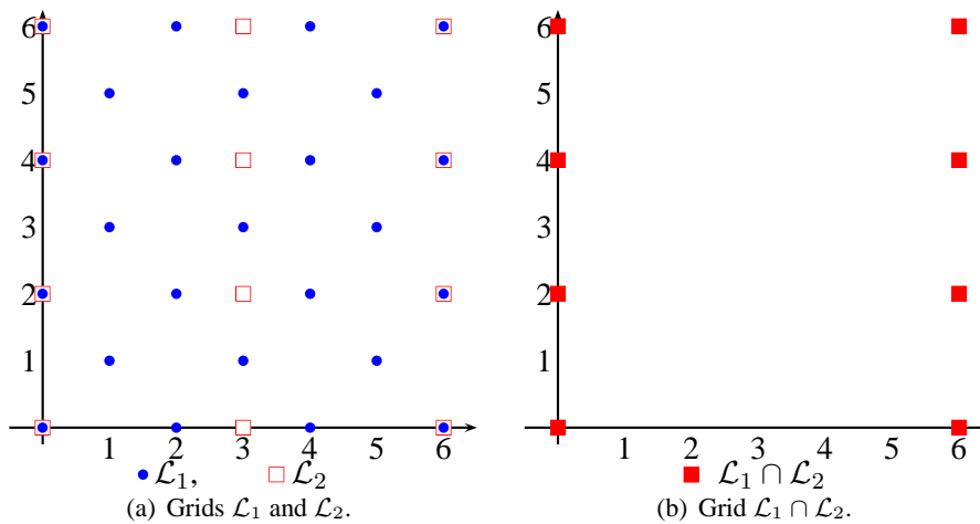
Figure 4.3: Grid intersection.
