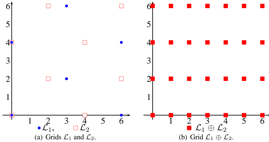
Figure 4.5: Grid join.
