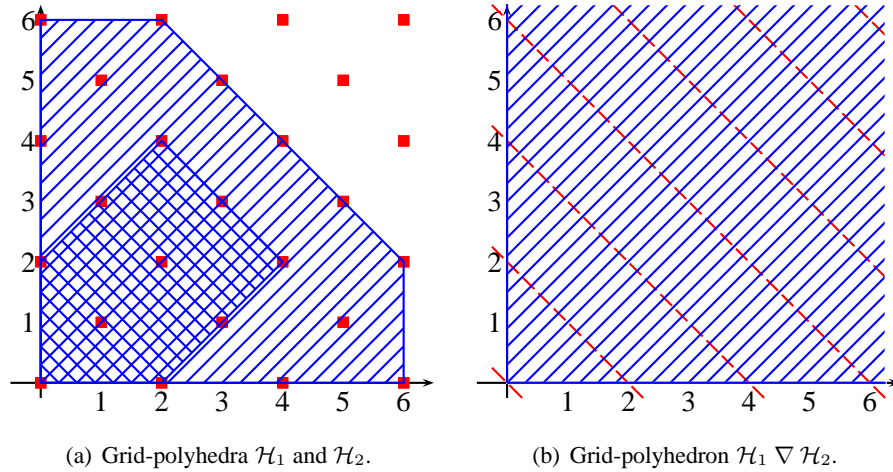
Figure 6.19: Grid-Polyhedron Widening.
