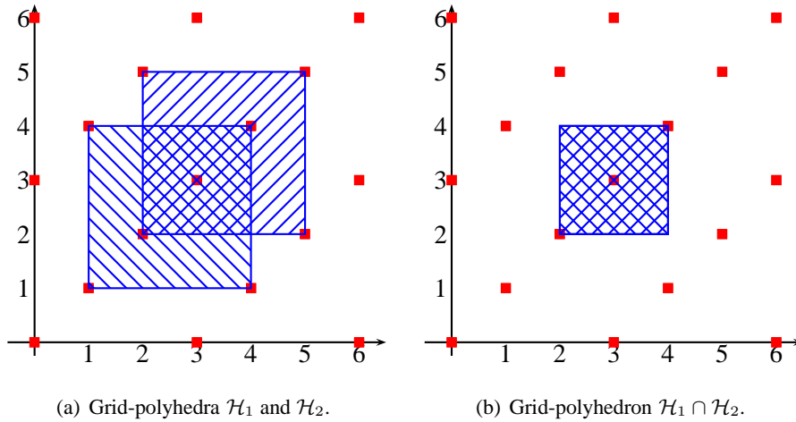
Figure 6.11: Grid-Polyhedron intersection.
