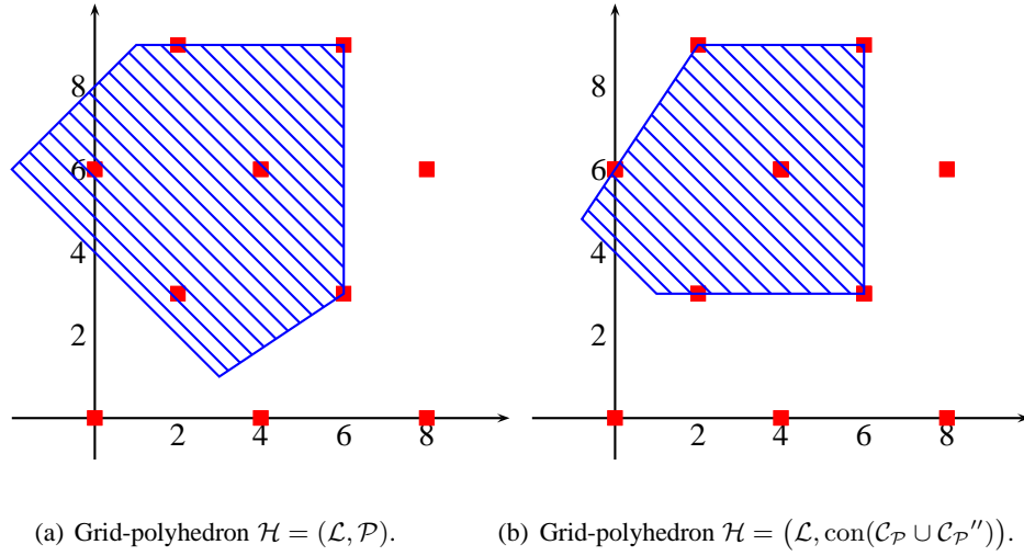
Figure 6.21: Adding constraints to a grid-polyhedron.
