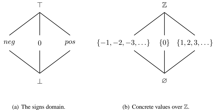
Figure 1.1: The abstract domain of signs represented as a lattice.
