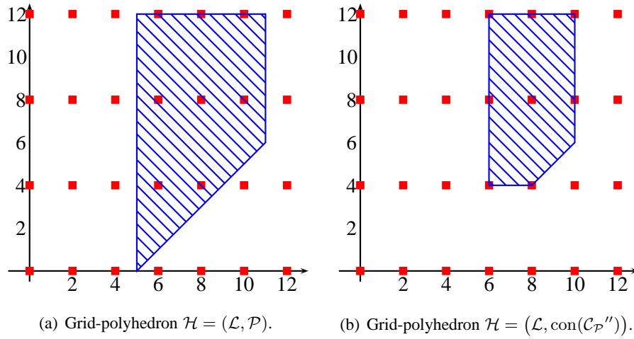
Figure 7.6: Proposition 7.12 requires the condition that \mathcal{C}_{\mathcal{P}} is a closed constraint system.
