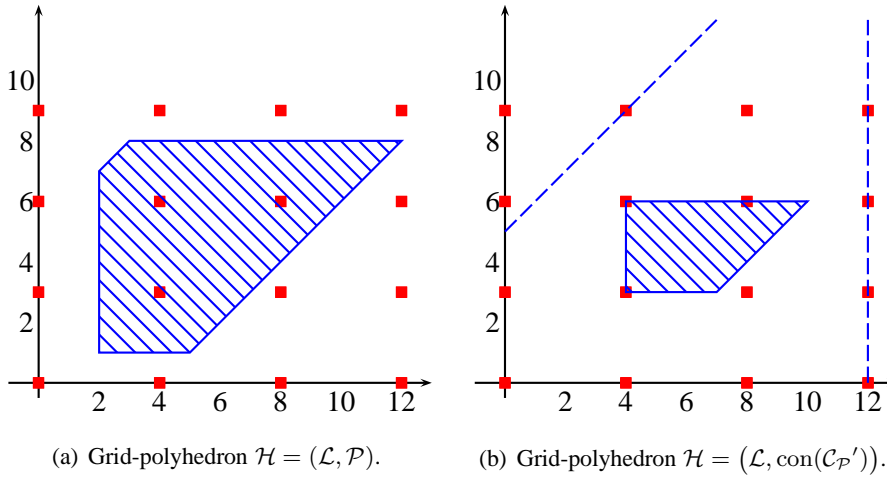
Figure 7.2: Producing a weakly tight grid-bds.
