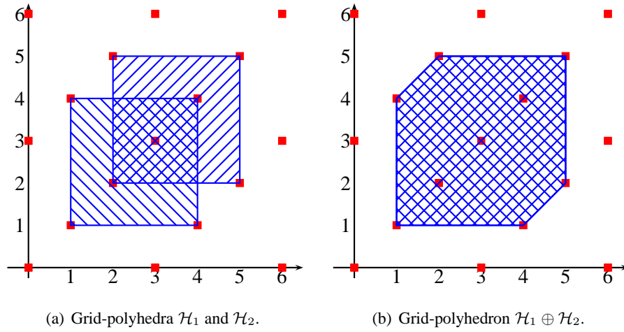
Figure 6.12: Grid-Polyhedron join.
