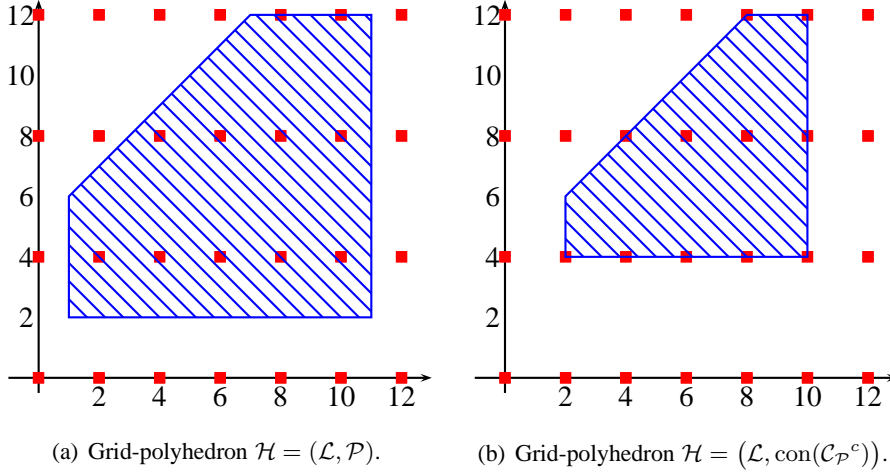
Figure 7.5: Producing a tight product grid-bds.
