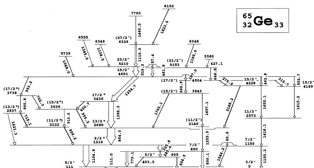
Figure 6.14: Energy level scheme of ^{65}\text{Ge} reproduced from Reference [63].
