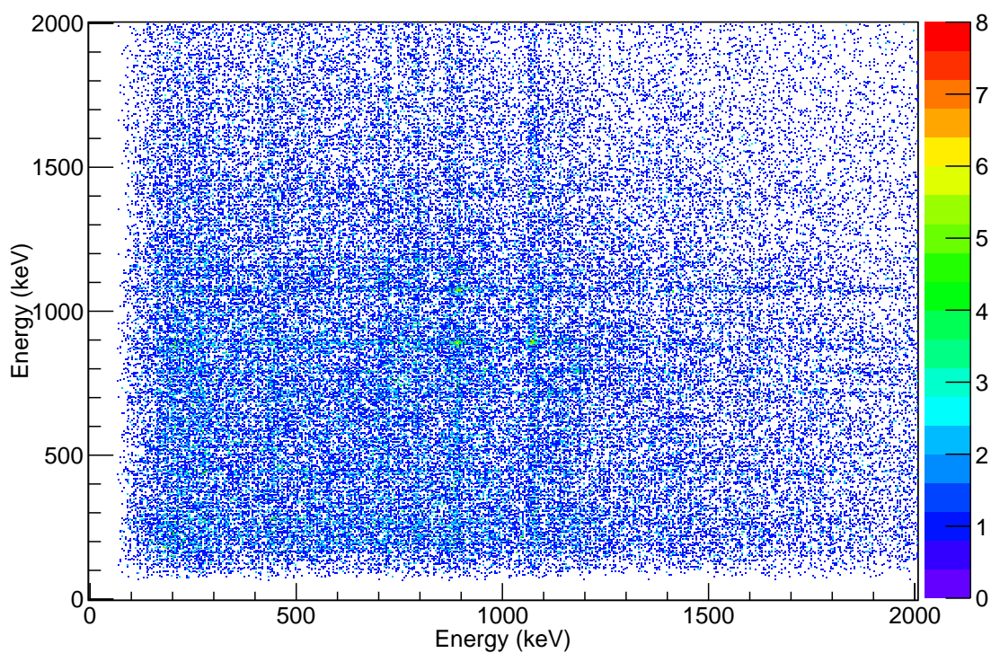
(b) A gamma gamma coincidence matrix for ^{63}\text{Ga} produced in one neutron knockout from ^{64}\text{Ga} .
