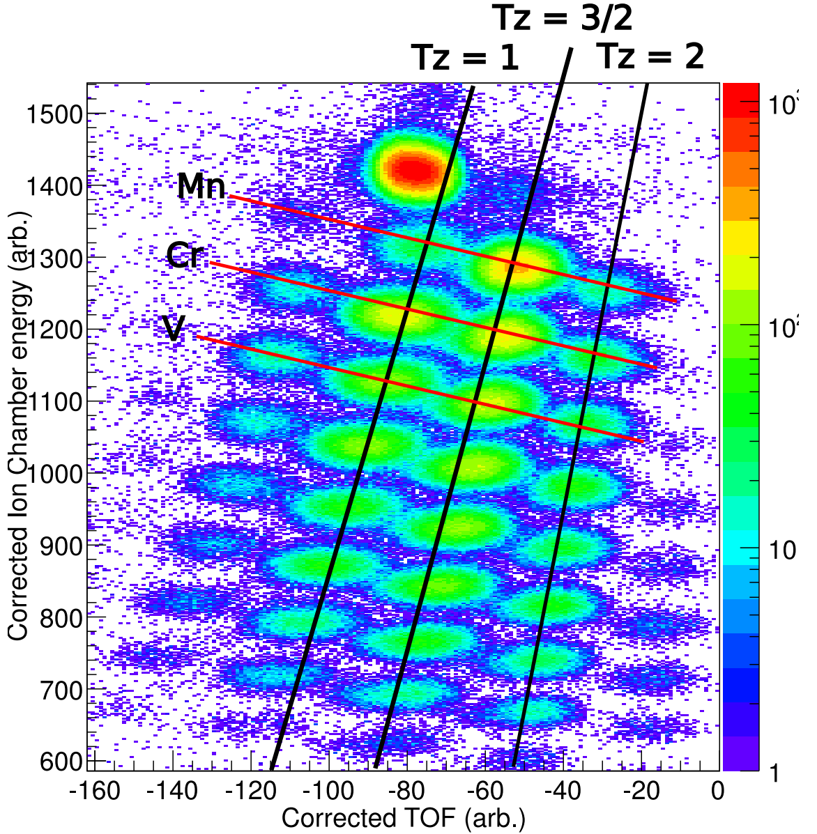
Figure 5.2: Particle identification after fragmentation of ^{54}\text{Fe} in the S800. The spectrum was created by selecting the ^{54}\text{Fe} data from plots such as Figure 5.1. See text for details.
