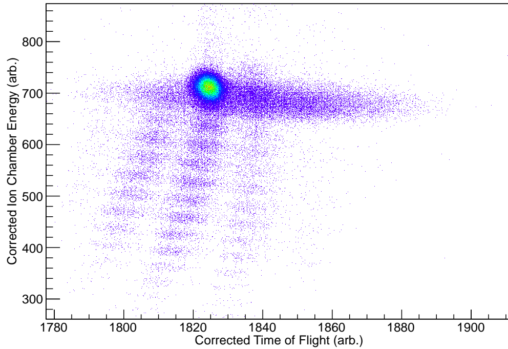
Figure D.2: S800 PID plot gated on the gate shown in Figure D.1.
