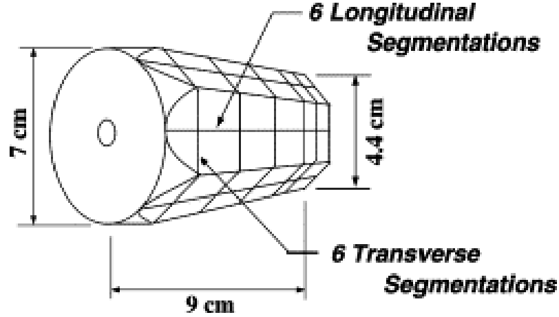
Figure 4.2: A diagram showing the size and segmentation of the GRETINA crystals, taken from [51]. There are six axial and six radial segments. Including the anode, 37 signals are read from each crystal.
