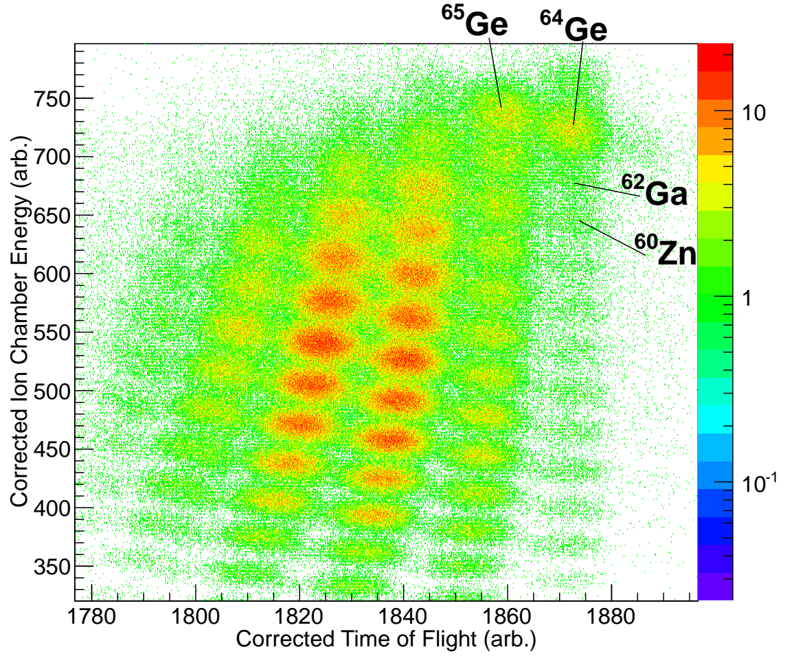
Figure 6.4: S800 PID plot produced by gated on a ^{65}\text{Ge} incoming beam from the A1900. This plot represents around 1-2% of the total accumulated data.
