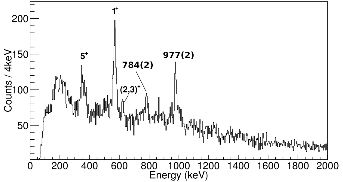
(a) Gamma ray spectrum from ^{62}\text{Ga} populated via two-neutron knockout from ^{64}\text{Ga} . The labelled 1^+ state has a measured energy of 570(2) keV and the labelled (2,3)^+ state has a measured energy of 623.7(10) keV. This spectrum was created by gating on ^{64}\text{Ga} data from the A1900 and ^{62}\text{Ga} data from the S800. A time cut has been applied such as that in Figure 6.6a and a FoM cut of 0.8 has been applied.
