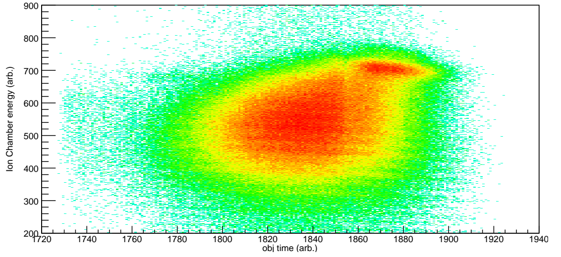
(a) Particle Identification in the S800 before the corrections detailed in Equations 6.1 and 6.2 have been applied, see text for details. This plot represents around 1-2% of the total accumulated data.
