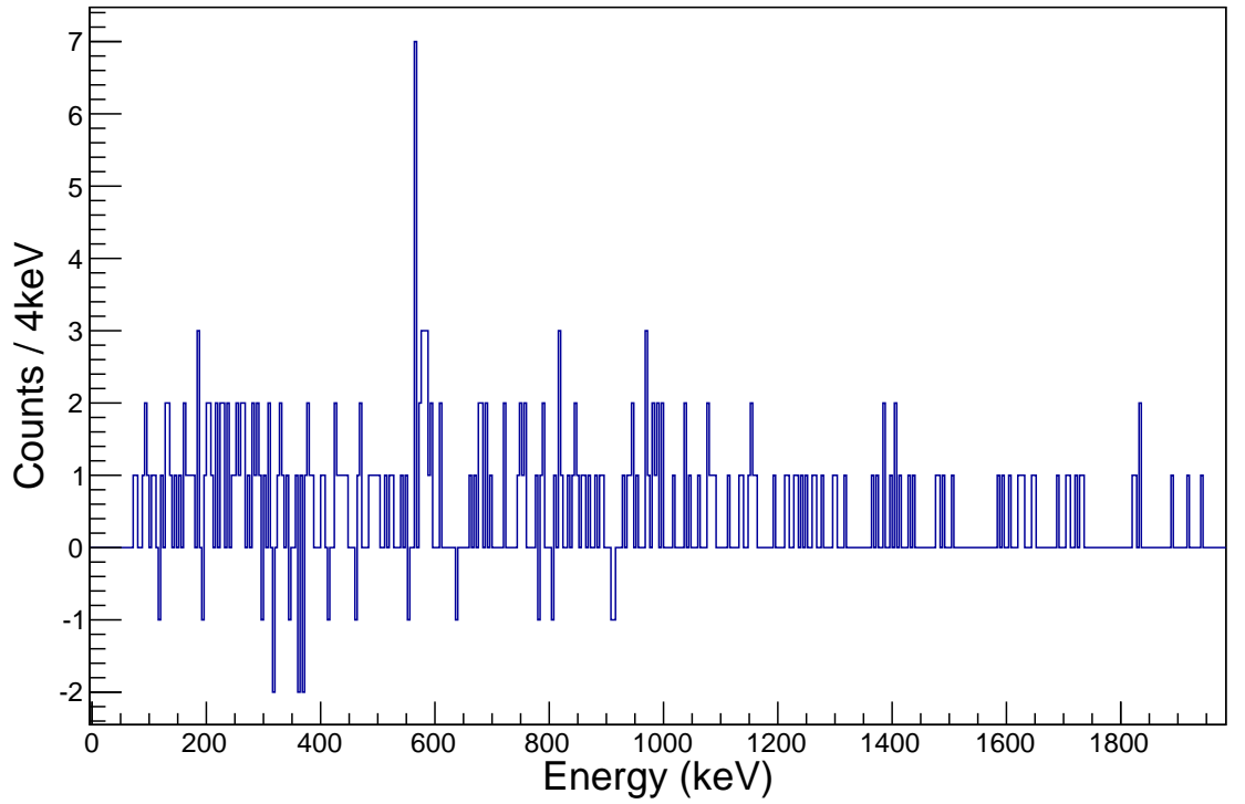
(b) A gamma gamma coincidence spectrum produced by projecting Figure 6.12 around the 784 keV peak and performing a local background subtraction above and below the peak.
