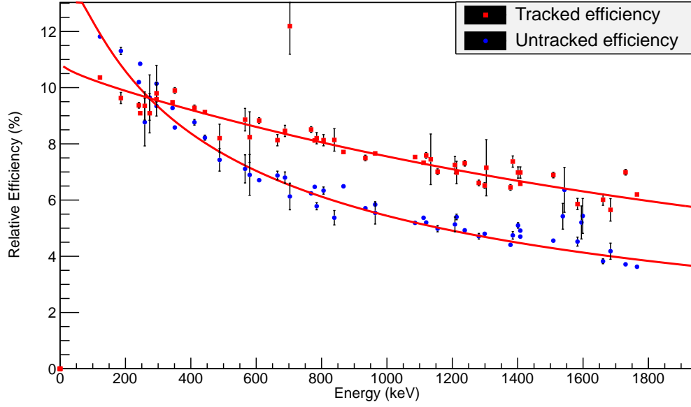
Figure 4.8: Efficiency curves for GREYINA calculated from a ^{152}\text{Eu} spectrum taken with the source at the centre of GREYINA. Mode 1 (red) is in red and Mode 2 in (blue).
