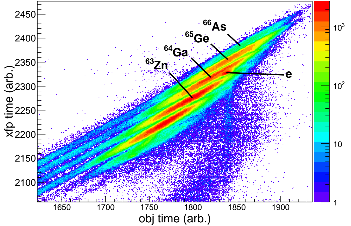
Figure 6.1: Particle identification of incoming beams; the time from the xjp and obj scintillator events, relative to the E1 scintillator are plotted against each other. This plot represents around 1-2% of the total accumulated data.
