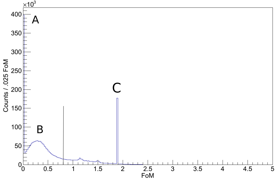
Figure 4.6: The FoM for fully tracked data taken with a ^{152}\text{Eu} source. The first bin, labelled A, mostly corresponds to events with only one interaction point, hence a FoM of 0. The hump around B is the majority of the good data, these have non-zero FoM due to the position resolution of GRETINA. The large peak labelled C corresponds to photoelectric events that happen too deep into the crystal and are most likely scatter (see step 6 above). The line at 0.8 is the cut applied to the FoM, those with a lower FoM are deemed to be good events.
