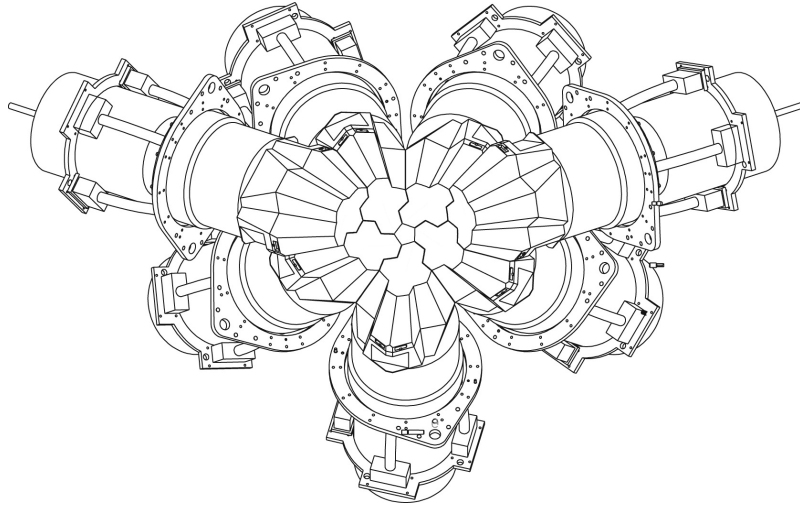
Figure 4.3: Schematic diagram showing a possible GRETINA configuration taken from [14].
