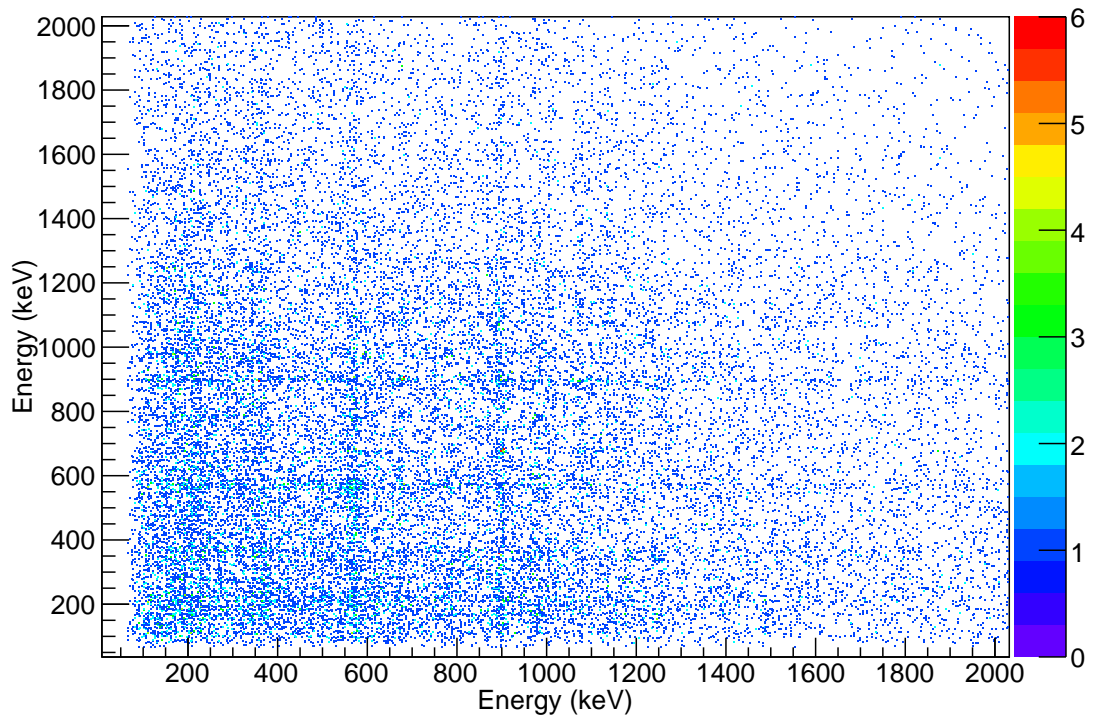
Figure 6.12: Gamma Gamma matrix for ^{62}\text{Ga} populated in 1p2n removal from ^{65}\text{Ge} . This spectrum was created by gating on ^{65}\text{Ge} data from the A1900 and ^{62}\text{Ga} data from the S800. A time cut has been applied such as that in Figure 6.6a and a FoM cut of 0.8 has been applied. The X and Y axis both show gamma ray energies for coincident events. The Z axis denotes the number of coincident events in units of coincidences per 4 keV per 4 keV. This matrix was constructed the same gates as those used to create the gamma ray spectrum in Figure 6.11a
