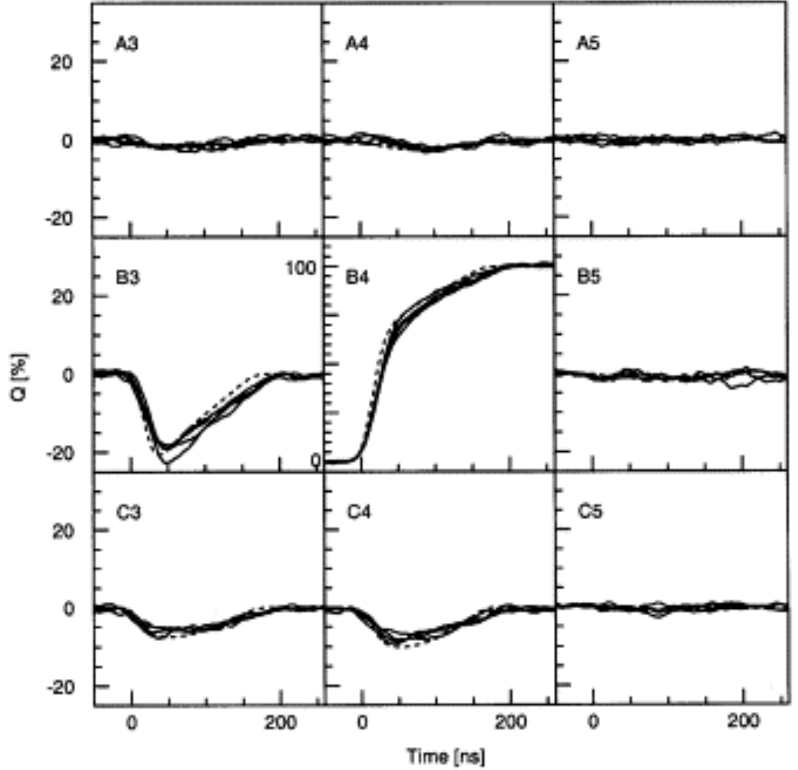
Figure 4.4: An example of signals collected from a GRETINA crystal using a collimated source. Each panel is the signal read from a different cathode, letters represent radial segments and numbers axial. The interactions are assumed close to segment B4 where most of the signal is collected and 4.5 mm away from segment C4 and 1.5 mm away from segment B3. The dashed lines show calculated signals, these signals have been corrected for cross talk effects [53].
