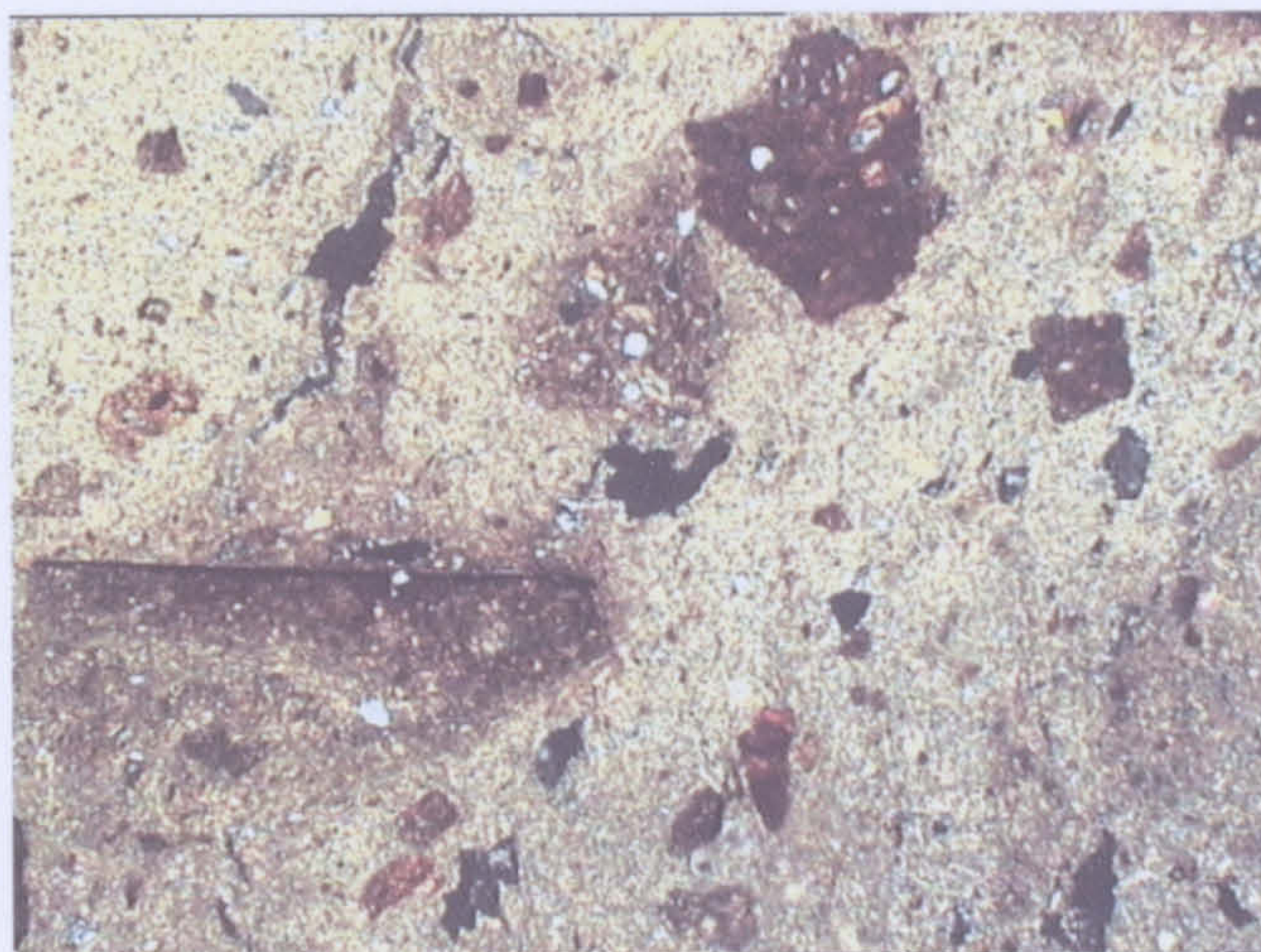
a (DIM 97/71) Field of view: 2.44 mm Fabric 32 Impressed, Dimini
