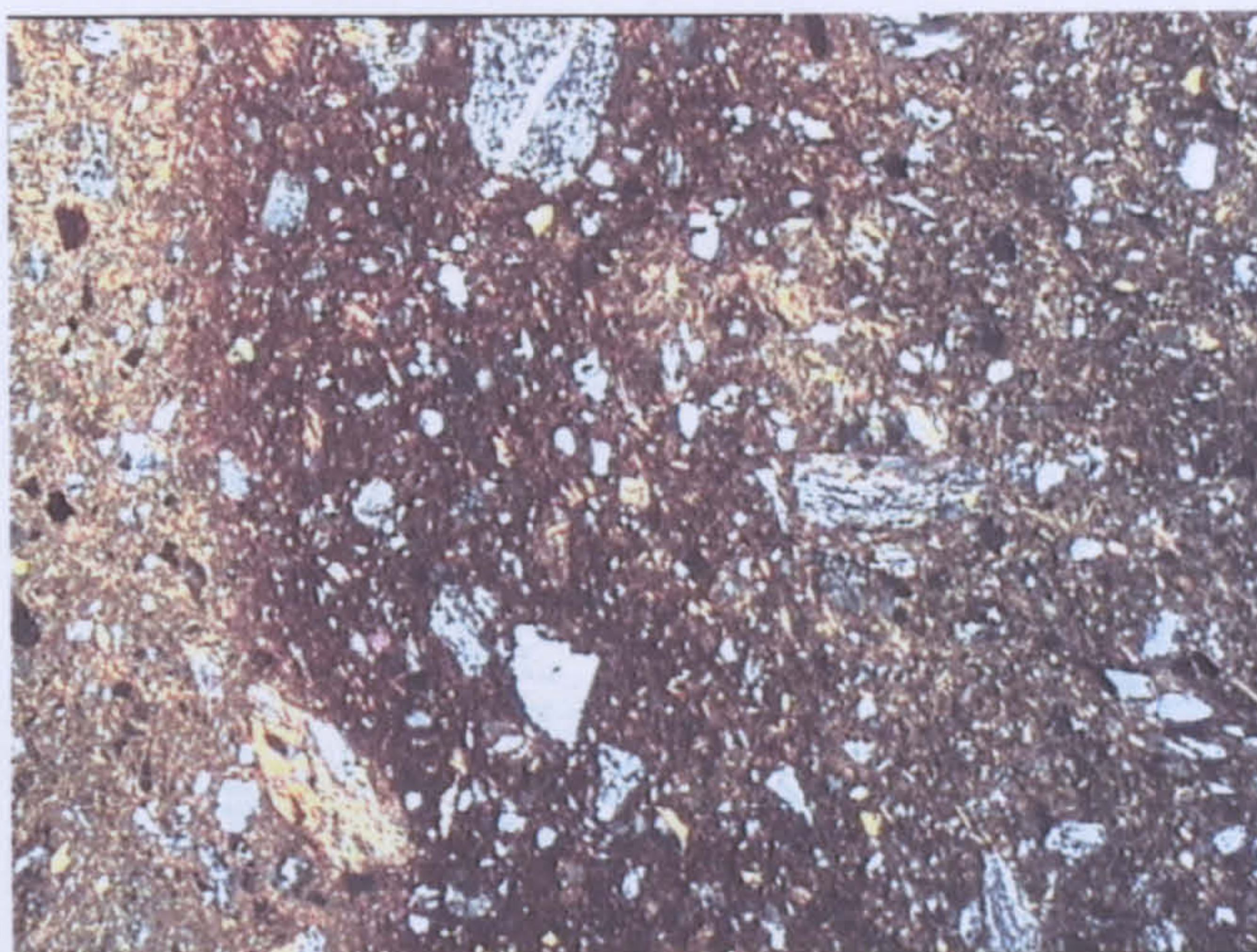
b (DIM 97/48) Field of view: 3.90 mm Fabric 7 Polychrome, Dimini
