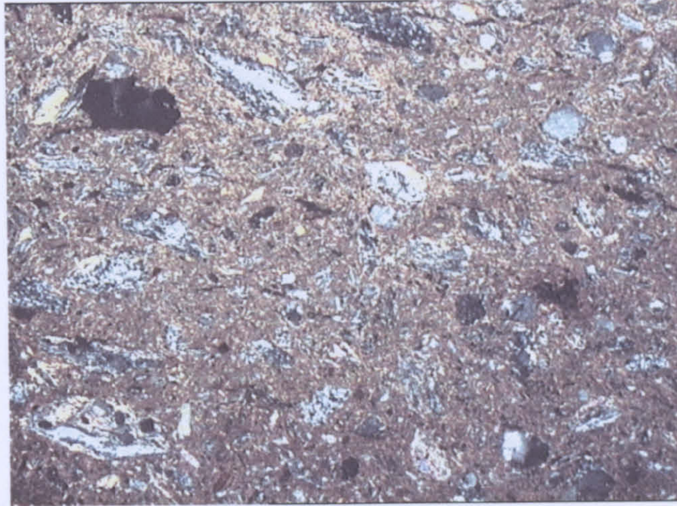
a (DIM 97/58) Field of view: 3.90 mm Fabric 10 Black Burnished, Dimini
