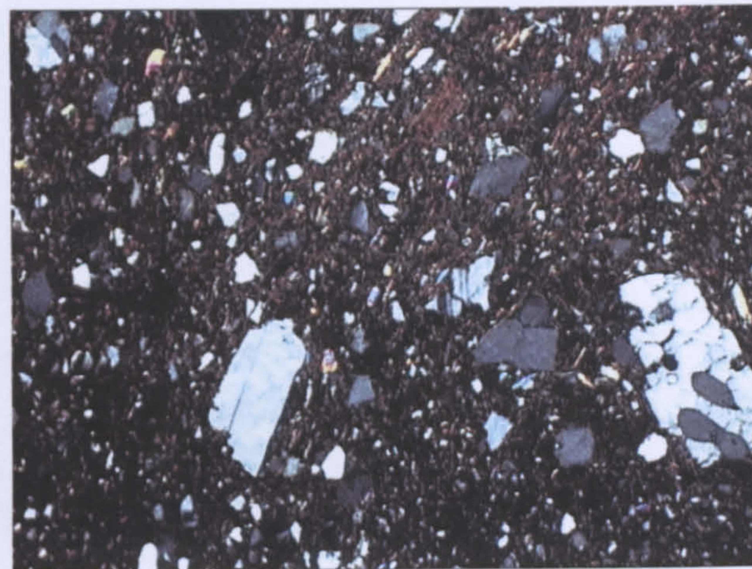
b (MAK 97/53) Field of view: 2.44 mm Fabric 19 Brown-on-Red, Makrygialos
