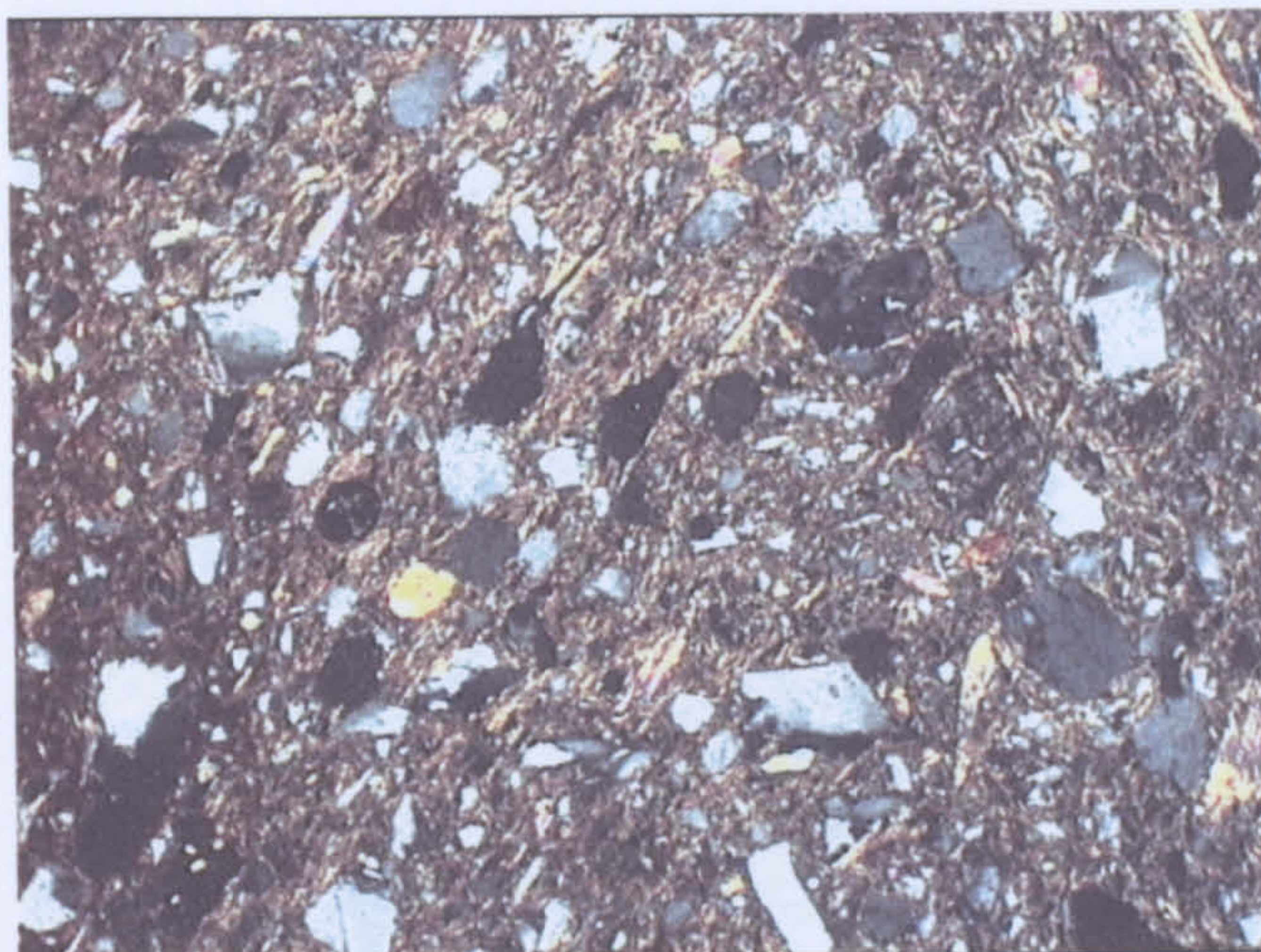
a (MAK 96/18) Field of view: 2.44 mm Fabric 13 Incised I, Makrygialos
