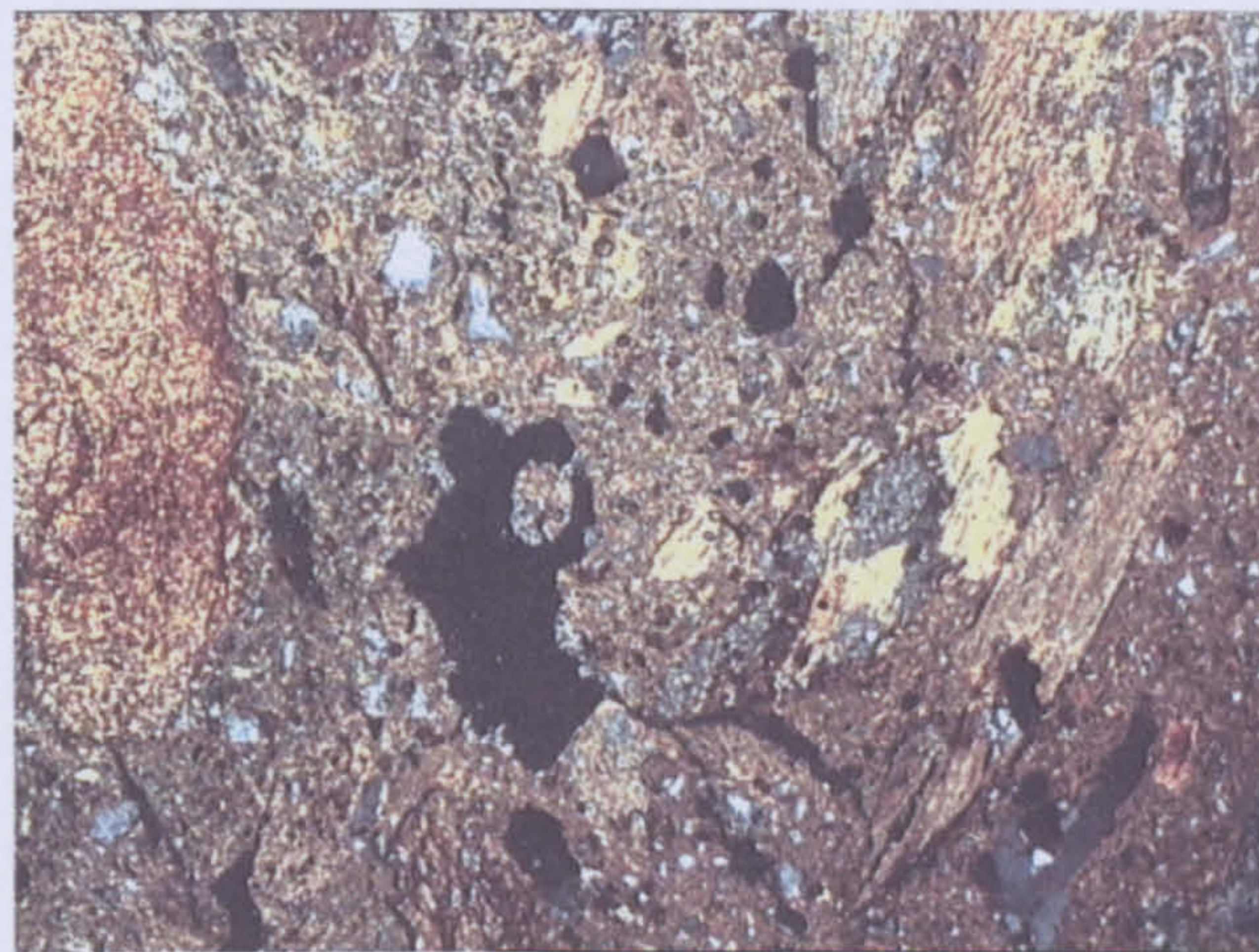
c (MAK 96/112) Field of view: 3.90 mm Fabric 39 Uncecorated, Makrygialos
