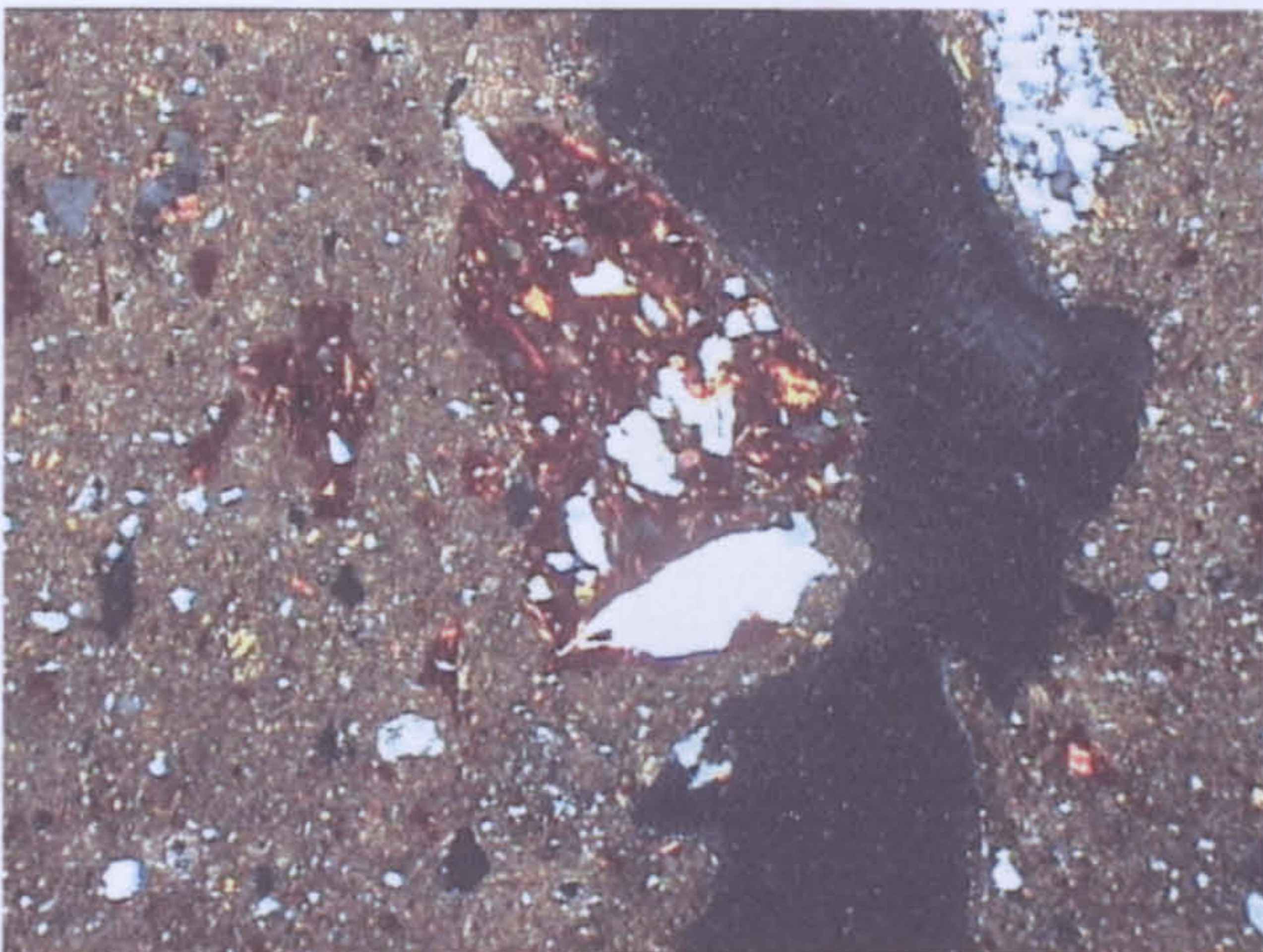
c (MAK 96/108) Field of view: 2.44 mm Fabric 2 Brown-on-Cream I, Makrygialos
