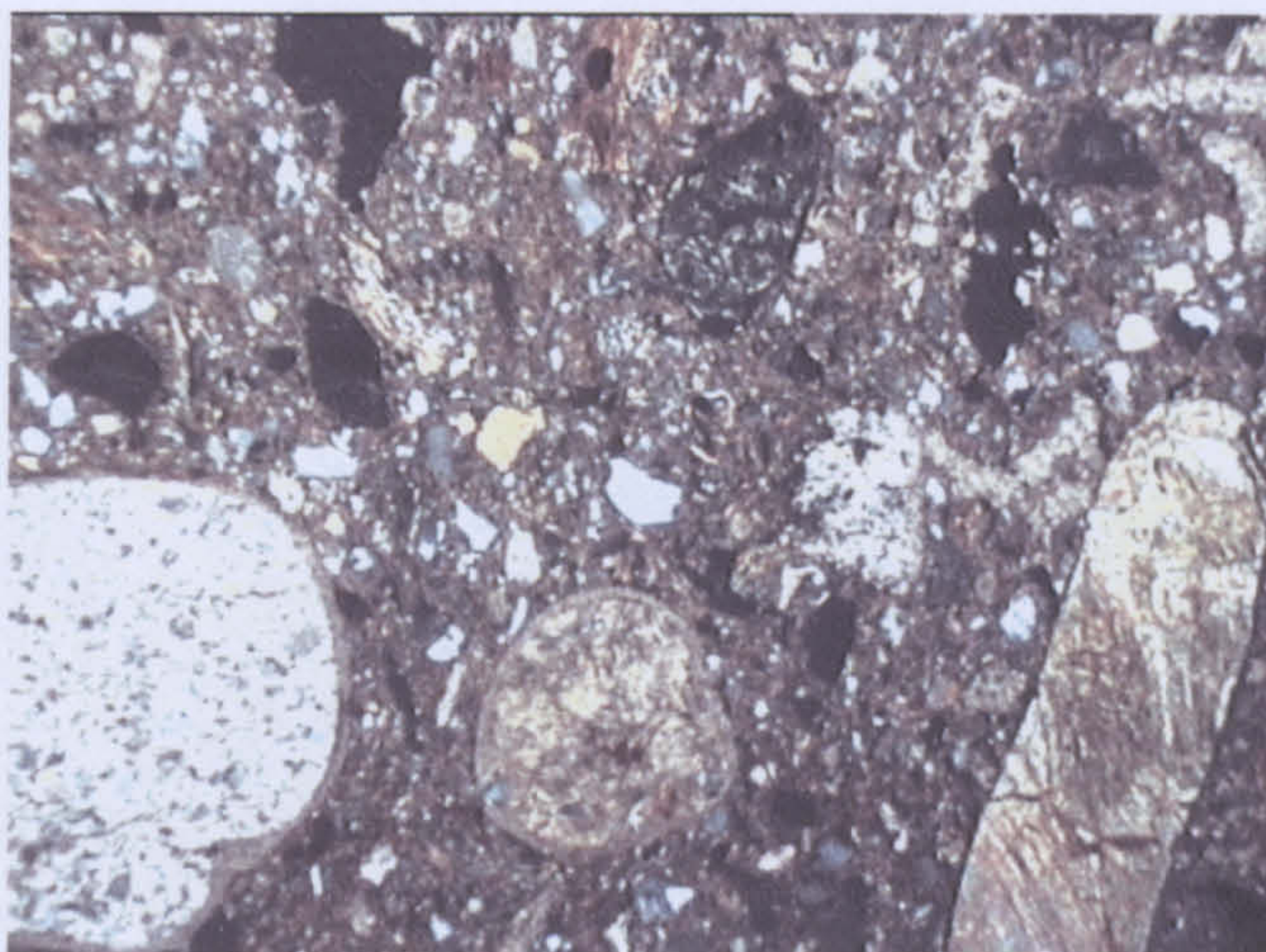
a (MAK 96/105) Field of view: 3.90 mm Fabric 38 Brown Burnished, Makrygialos
