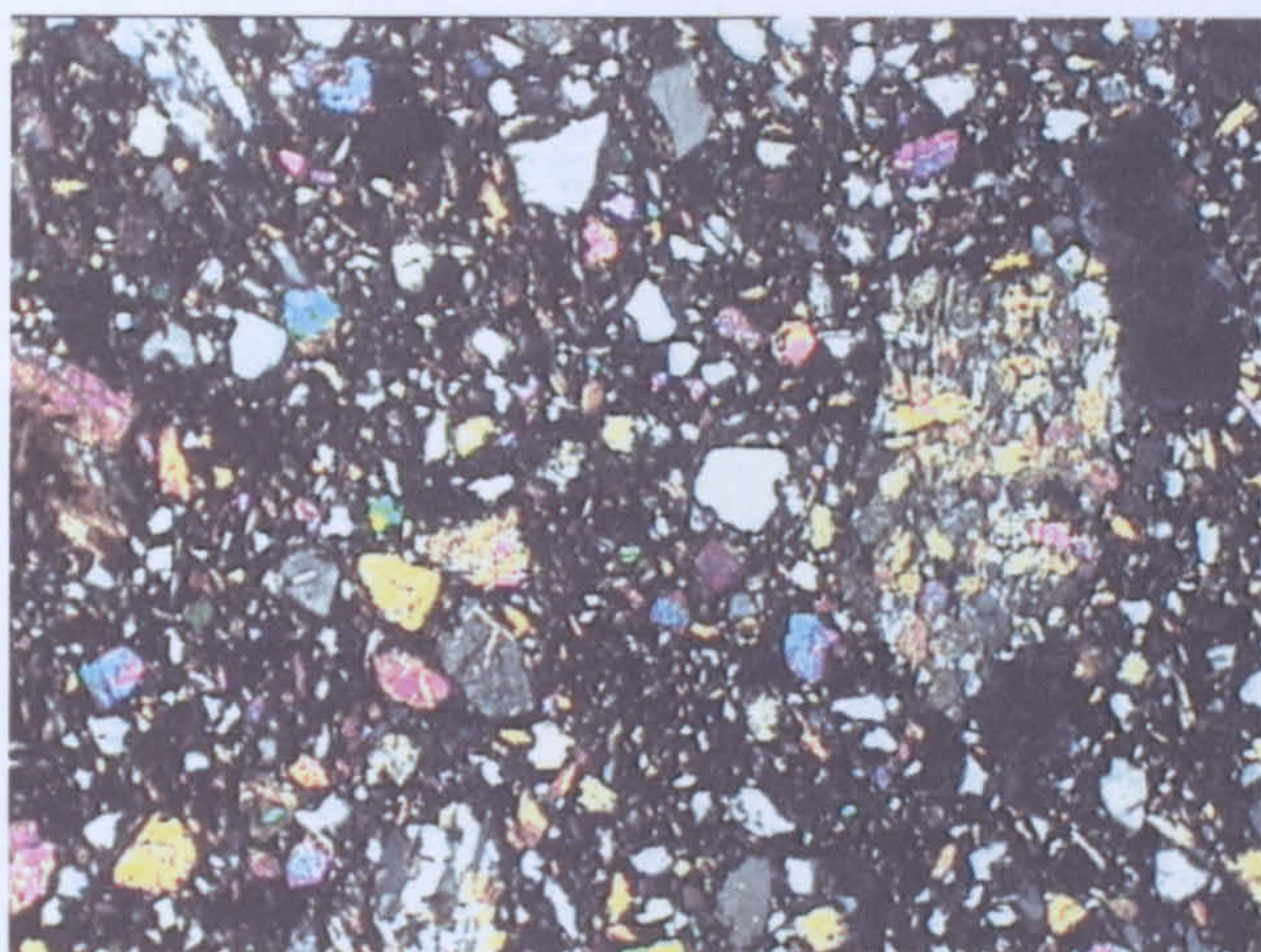
a (MAK 97/52) Field of view: 2.44 mm Fabric 12 Incised I, Makrygialos
