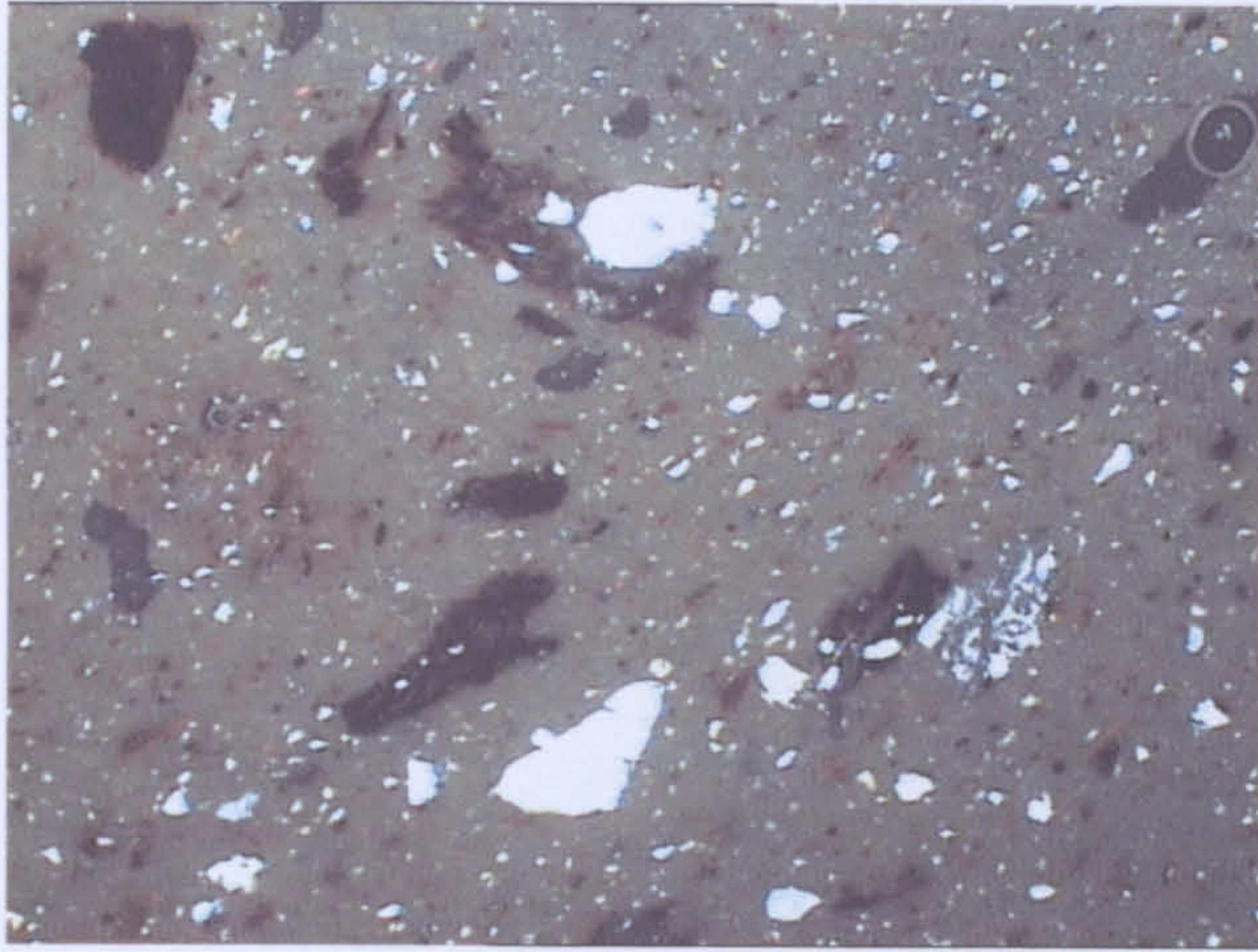
a (MAK 96/45) Field of view: 2.44 mm Fabric 1 Brown-on-Buff I, Makrygialos
