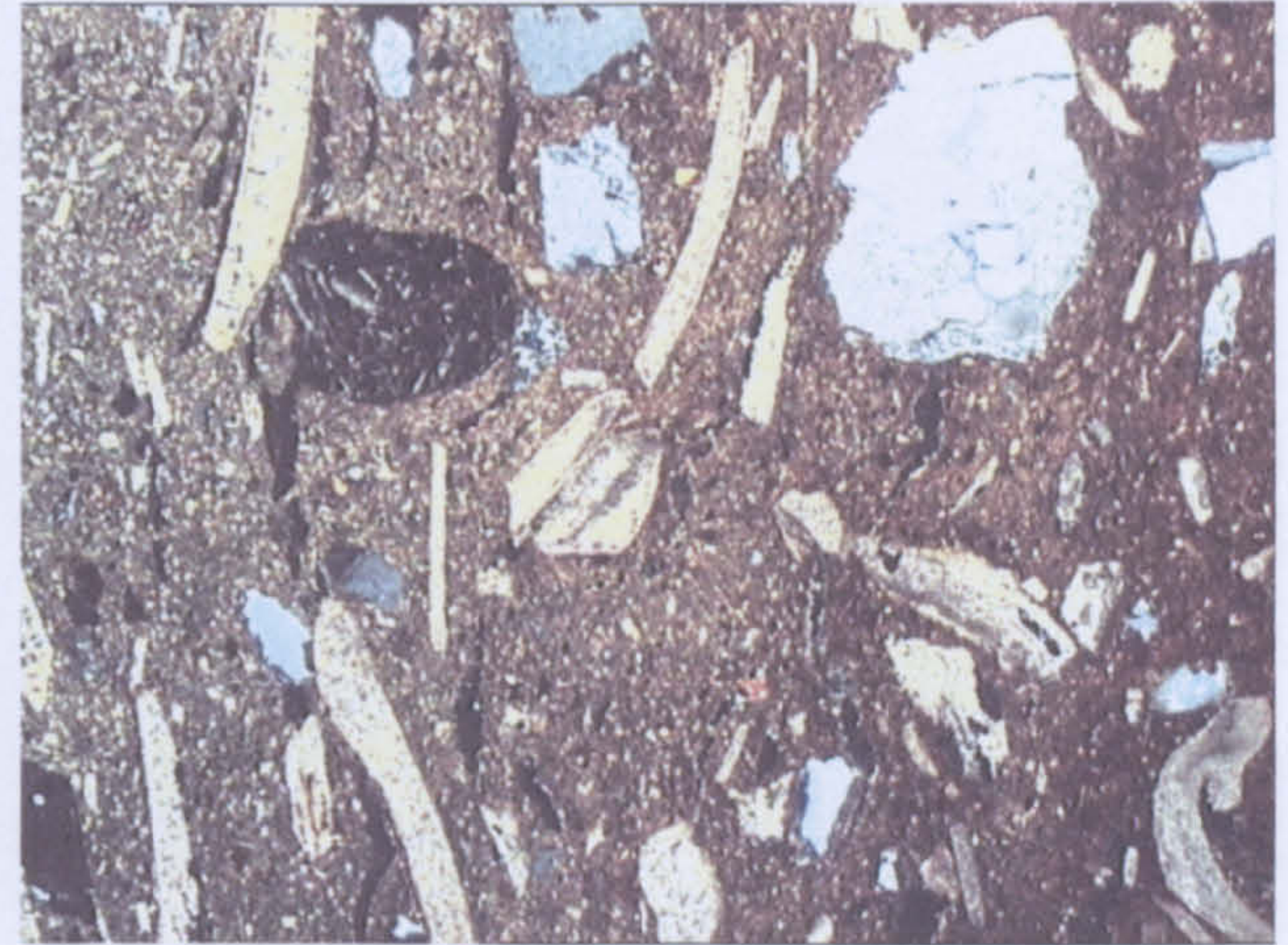
b (MAK 96/217) Field of view: 3.90 mm Fabric 24 Brown Burnished, Makrygialos
