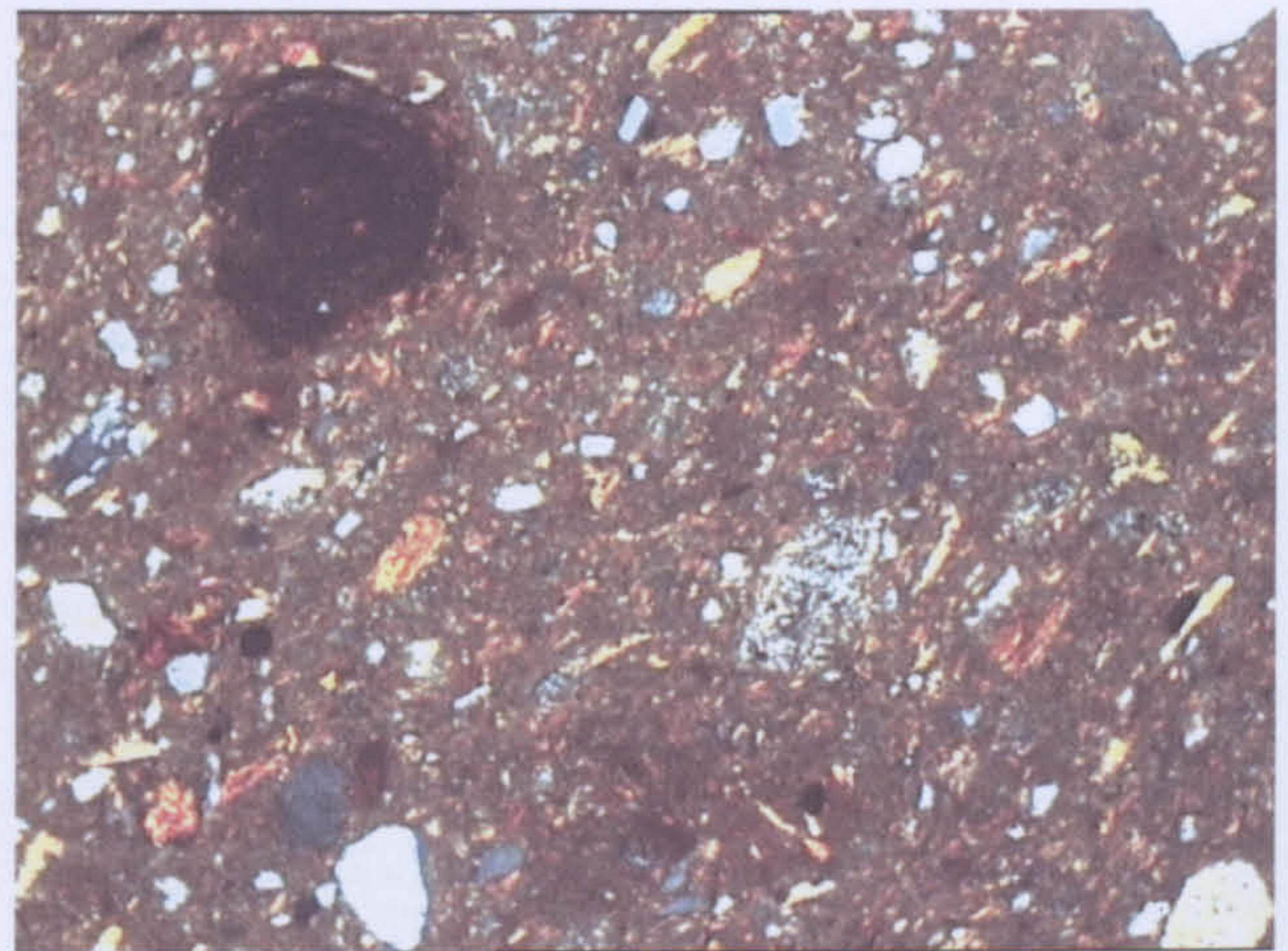
d (GIAN 97/1) Field of view: 0.99 mm Fabric 1 Brown-on-Cream, Giannitsa
