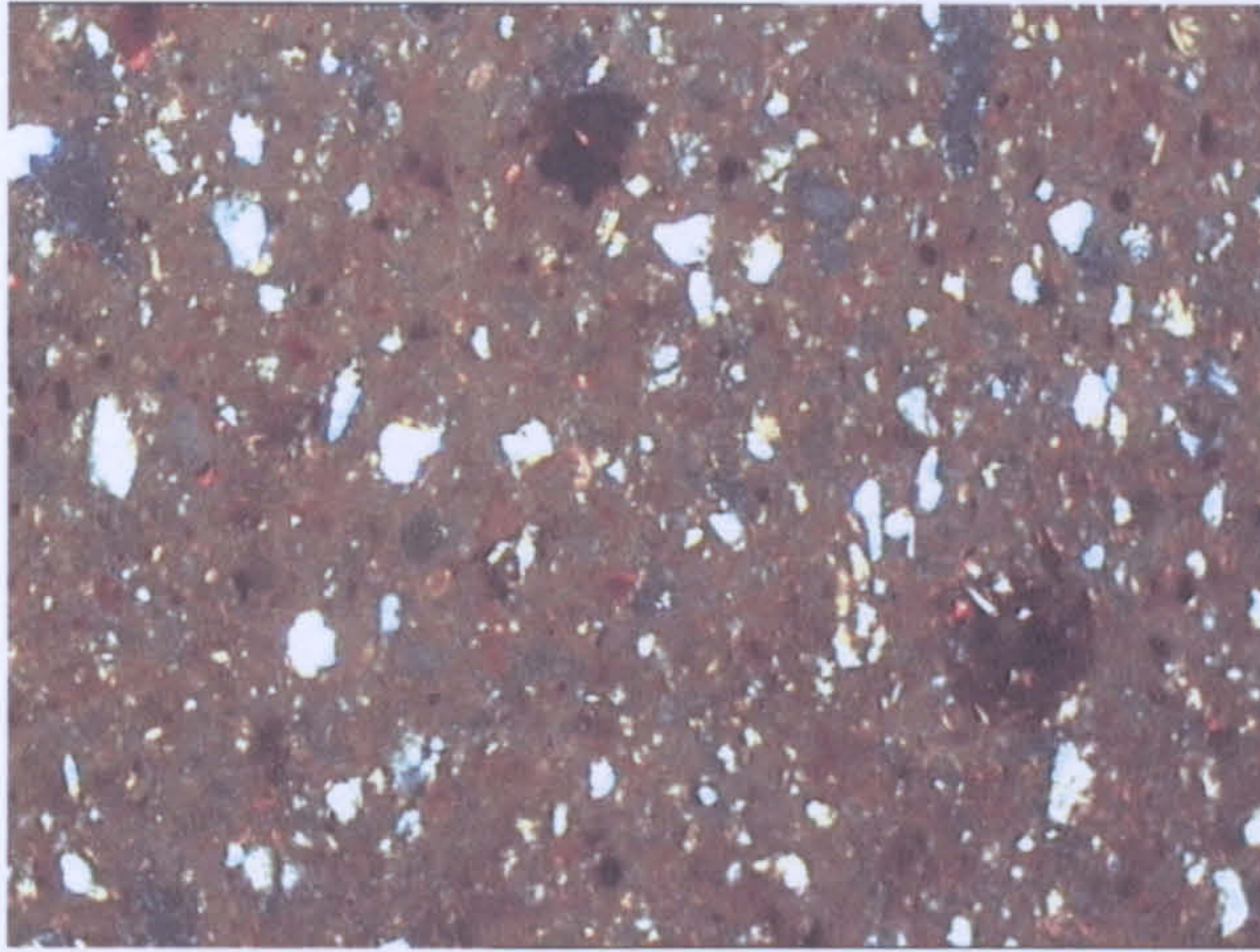
a (MAK 96/34) Field of view: 0.99 mm Fabric 1 Brown-on-Cream I, Makrygialos
