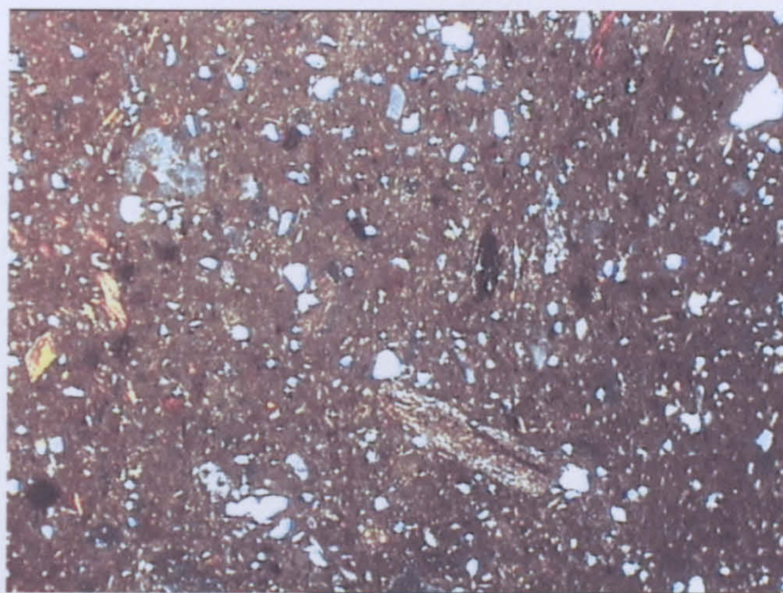
b (MAK 96/41) Field of view: 2.44 mm Fabric 1 Brown-on-Cream I, Makrygialos
