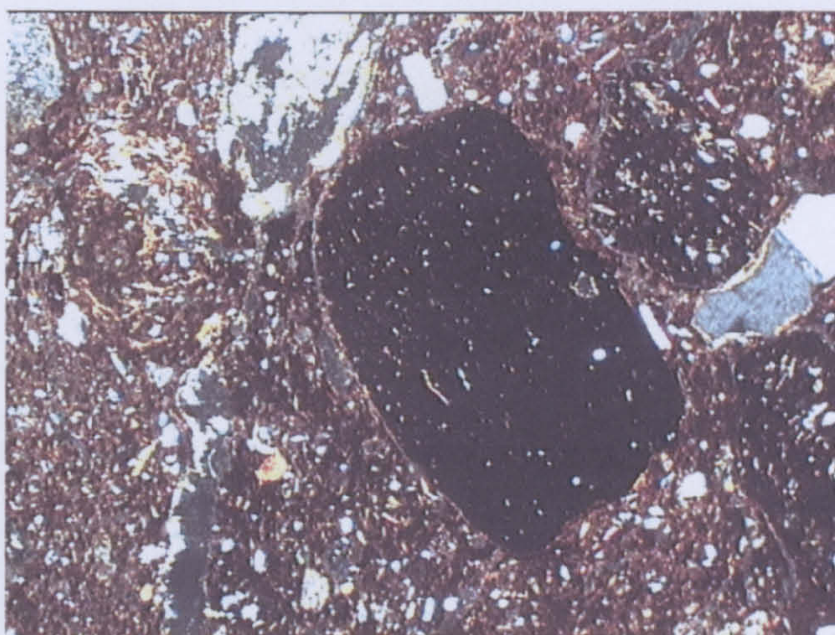
b (MAK 96/75) Field of view: 2.44 mm Fabric 40 Red Burnished, Makrygialos
