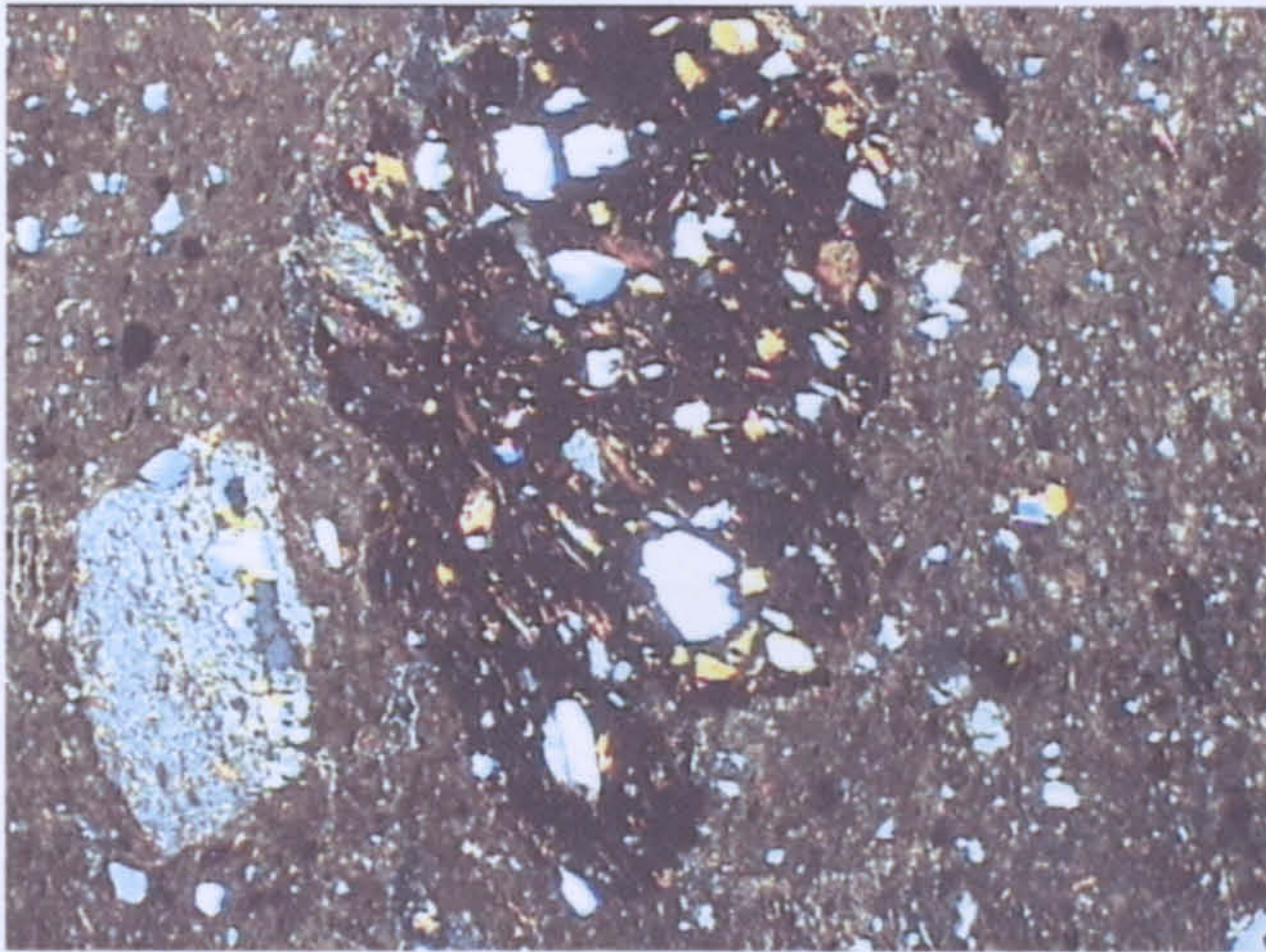
a (MAK 96/108) Field of view: 2.44 mm Fabric 2 Brown-on-Cream I, Makrygialos
