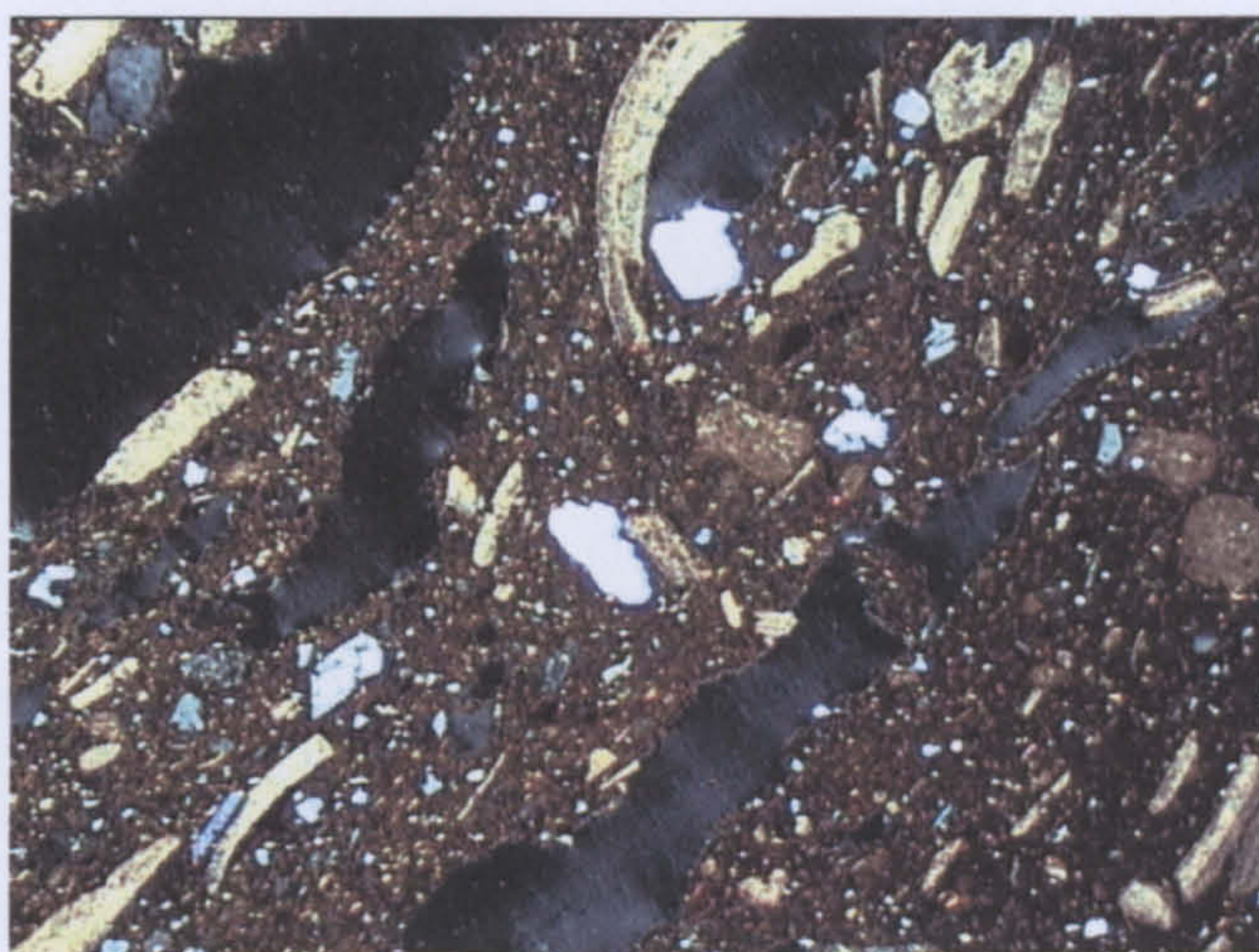
b (MAK 97/73) Field of view: 3.90 mm Fabric 24 Undecorated, Makrygialos
