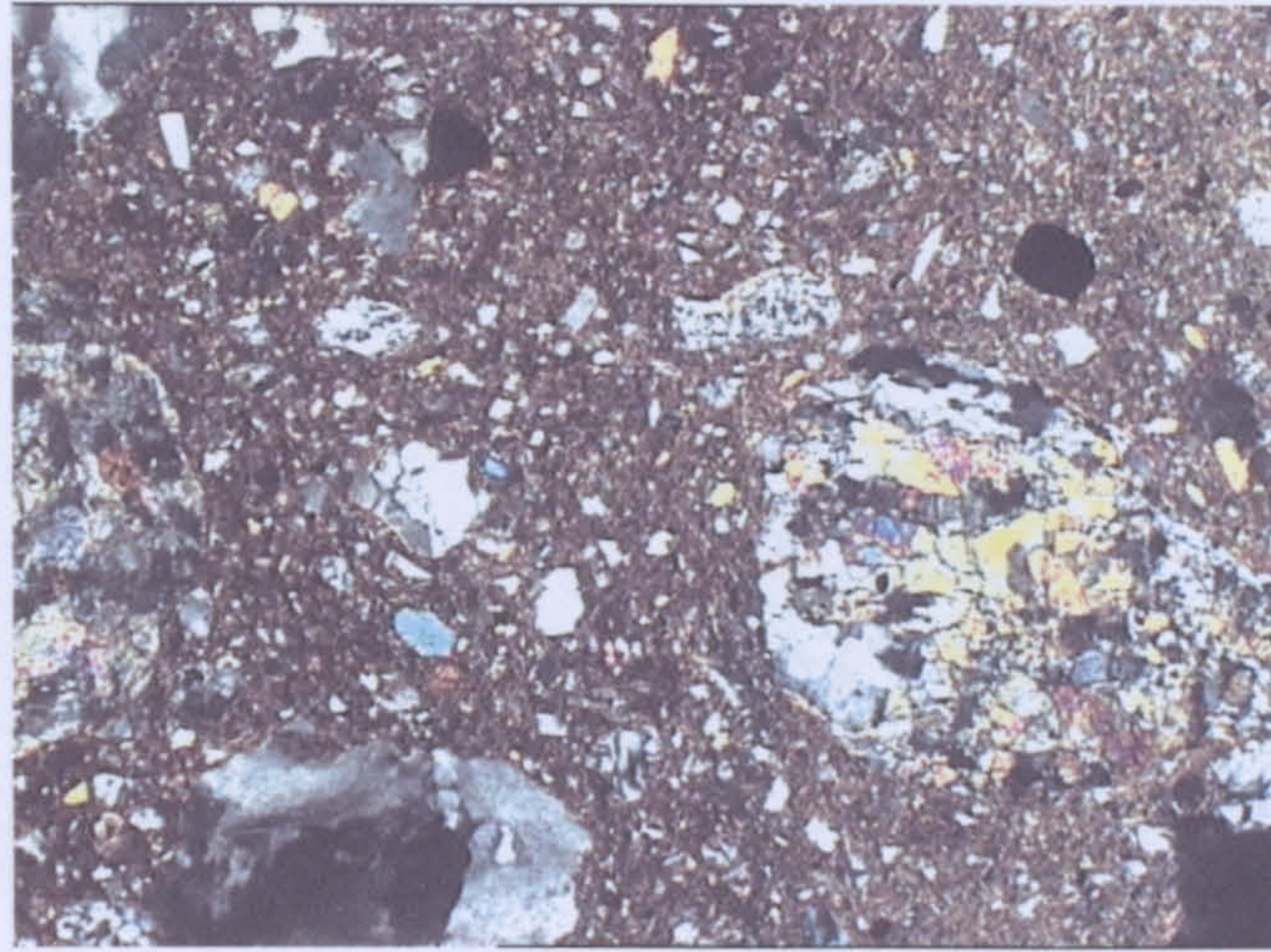
a (DIM 97/40) Field of view: 2.44 mm Fabric 11 Black-on-Red, Dimini
