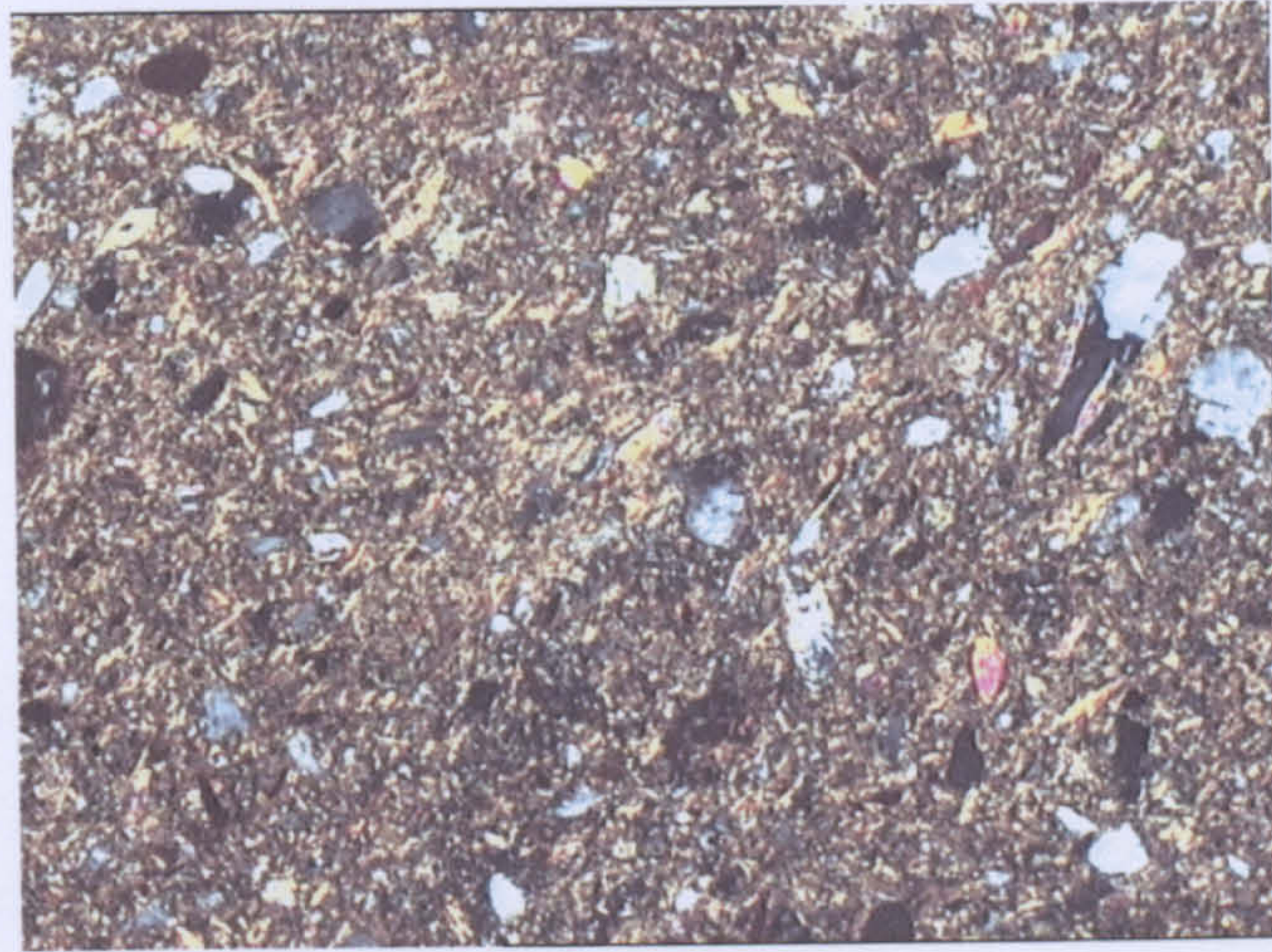
b (GIAN 97/9) Field of view: 0.99 mm Fabric 5 Brown-on-Cream, Giannitsa
