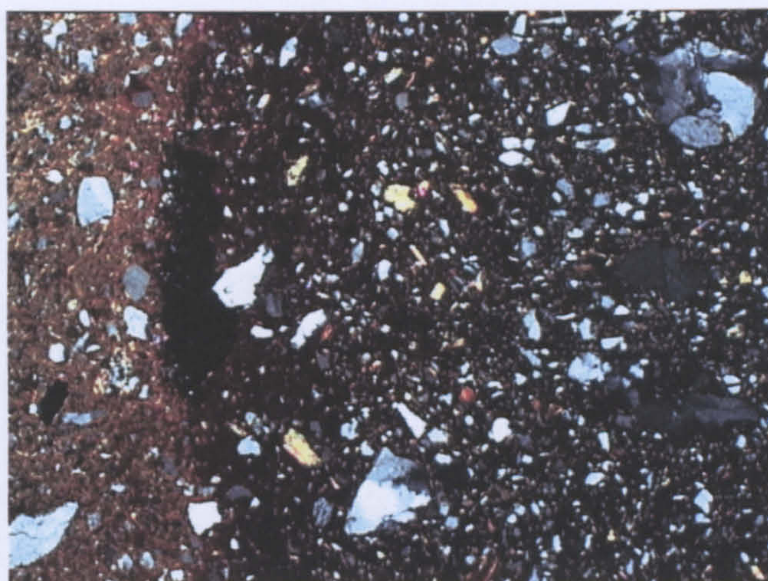
a (MAK 96/26) Field of view: 2.44 mm Fabric 16 Black-on-Red, Makrygialos
