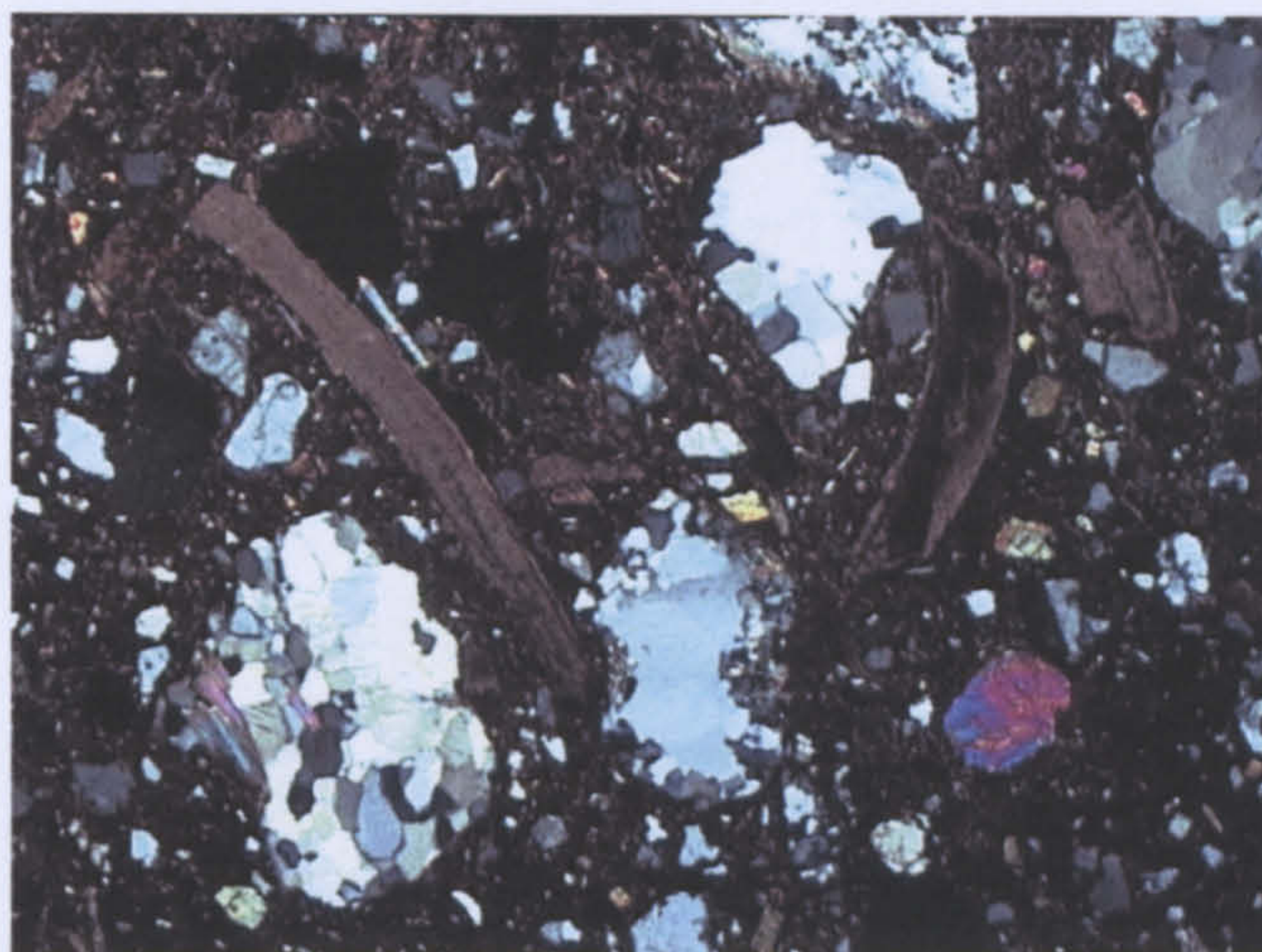
a (MAK 96/198) Field of view: 3.90 mm Fabric 27 Brown Burnished, Makrygialos
