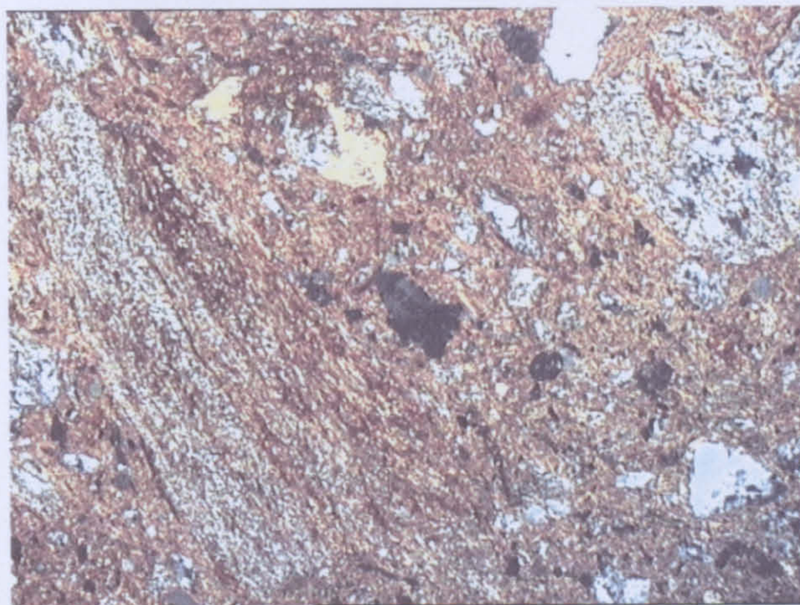
c (DIM 97/65) Field of view: 3.90 mm Fabric 8 Underdecorated, Dimini
