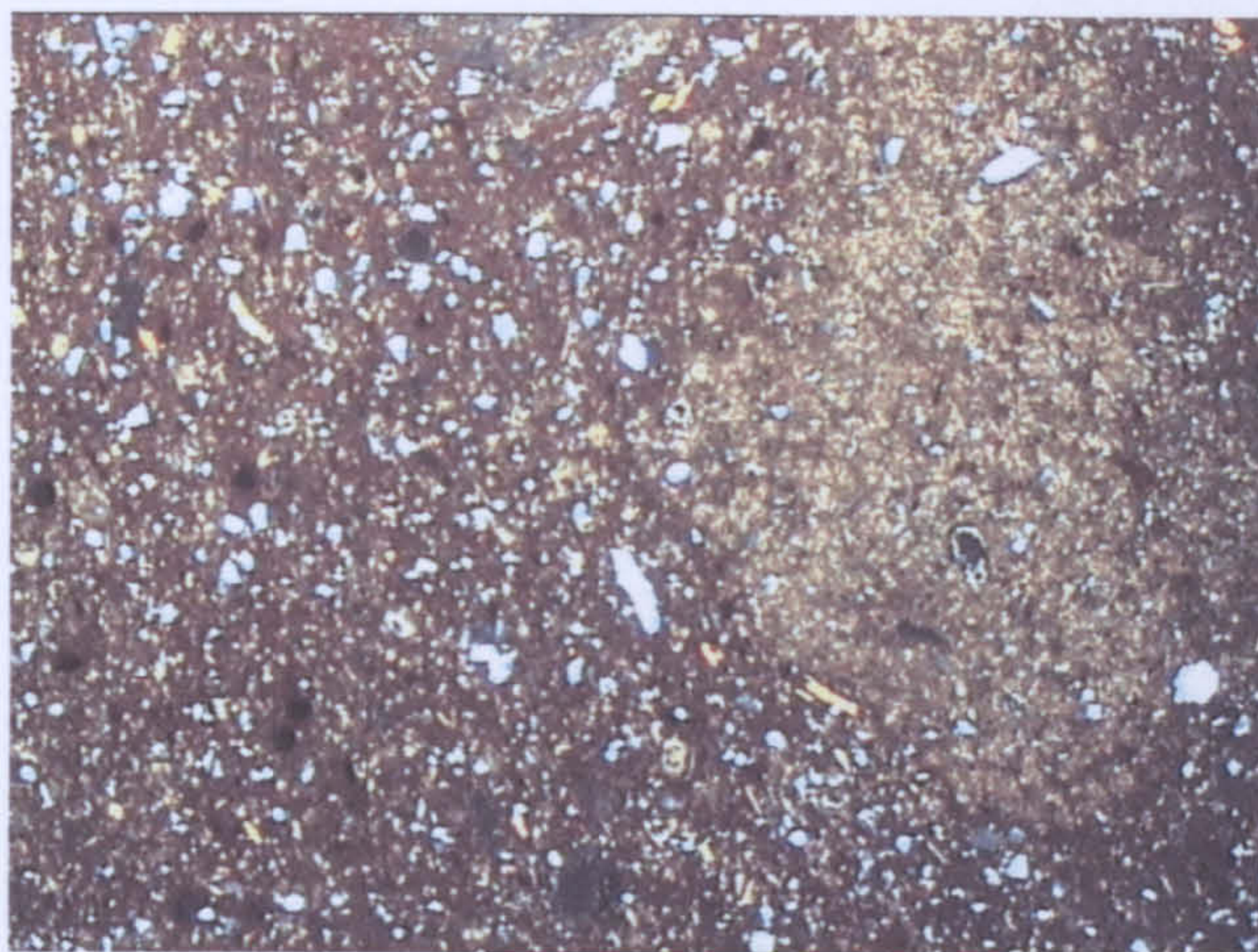
a (MAK 96/23) Field of view: 3.90 mm Fabric 1 Brown-on-Cream I, Makrygialos
