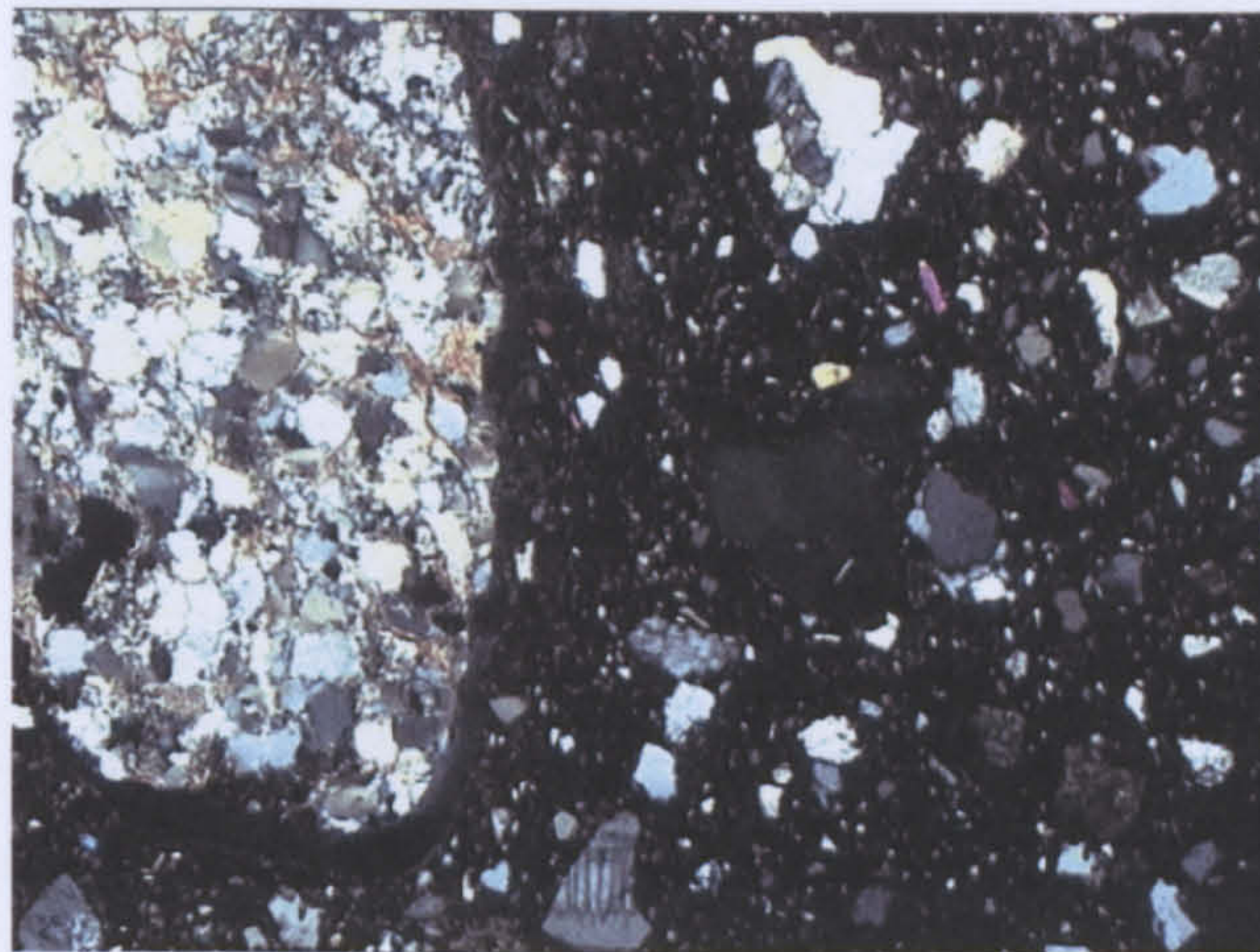
c (MAK 96/209) Field of view: 2.44 mm Fabric 18 Brown Burnished, Makrygialos
