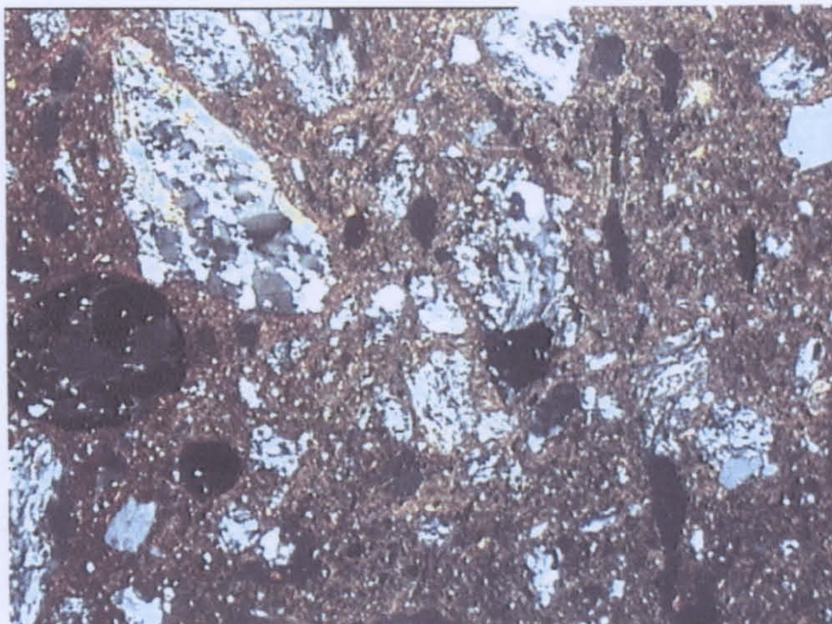
a (DIM 97/44) Field of view: 3.90 mm Fabric 7 Polychrome, Dimini
