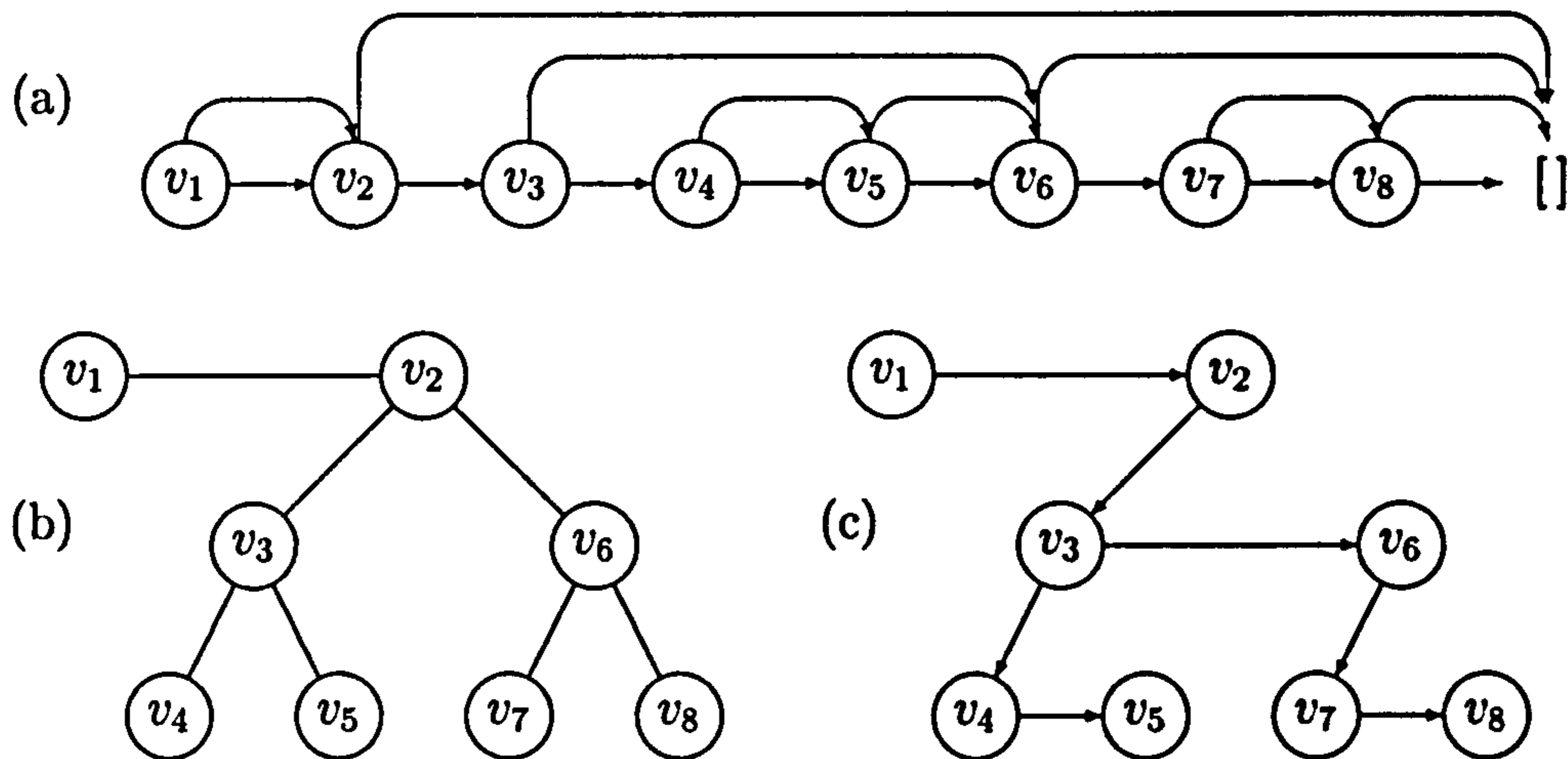
Figure 2.11: A list [v_1, \dots, v_8] represented (a) by Myers' random-access list, (b) by Okasaki's random-access list, and (c) by Myers' list with redundant pointers removed. Note the similarity between (b) and (c).
