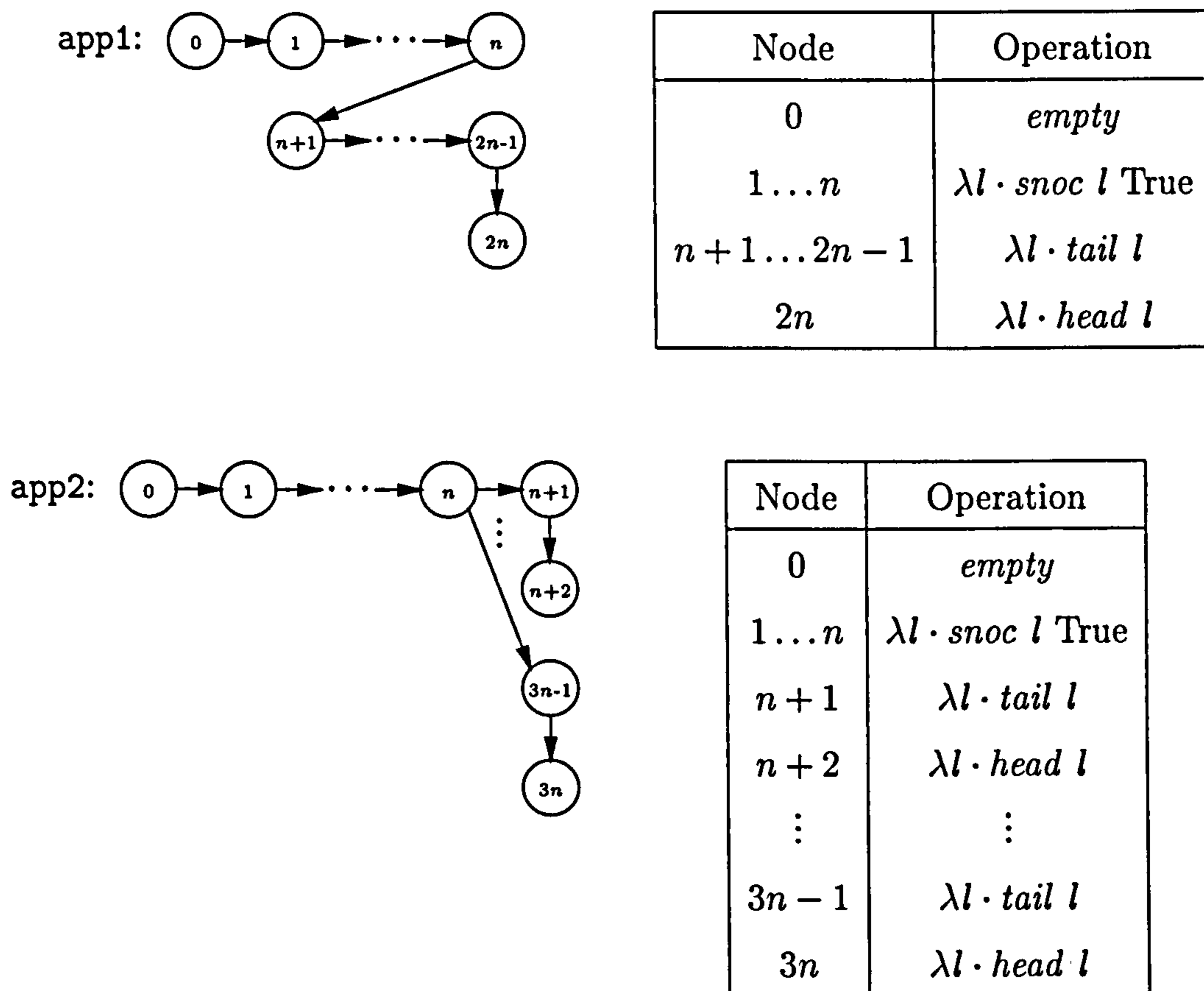
Figure 3.2: Graphs showing how the queue ADT is used by the different applications given in Figure 3.1. Note that node n of app2 corresponds to the value n\text{Snocs} shared by n applications of tail .
