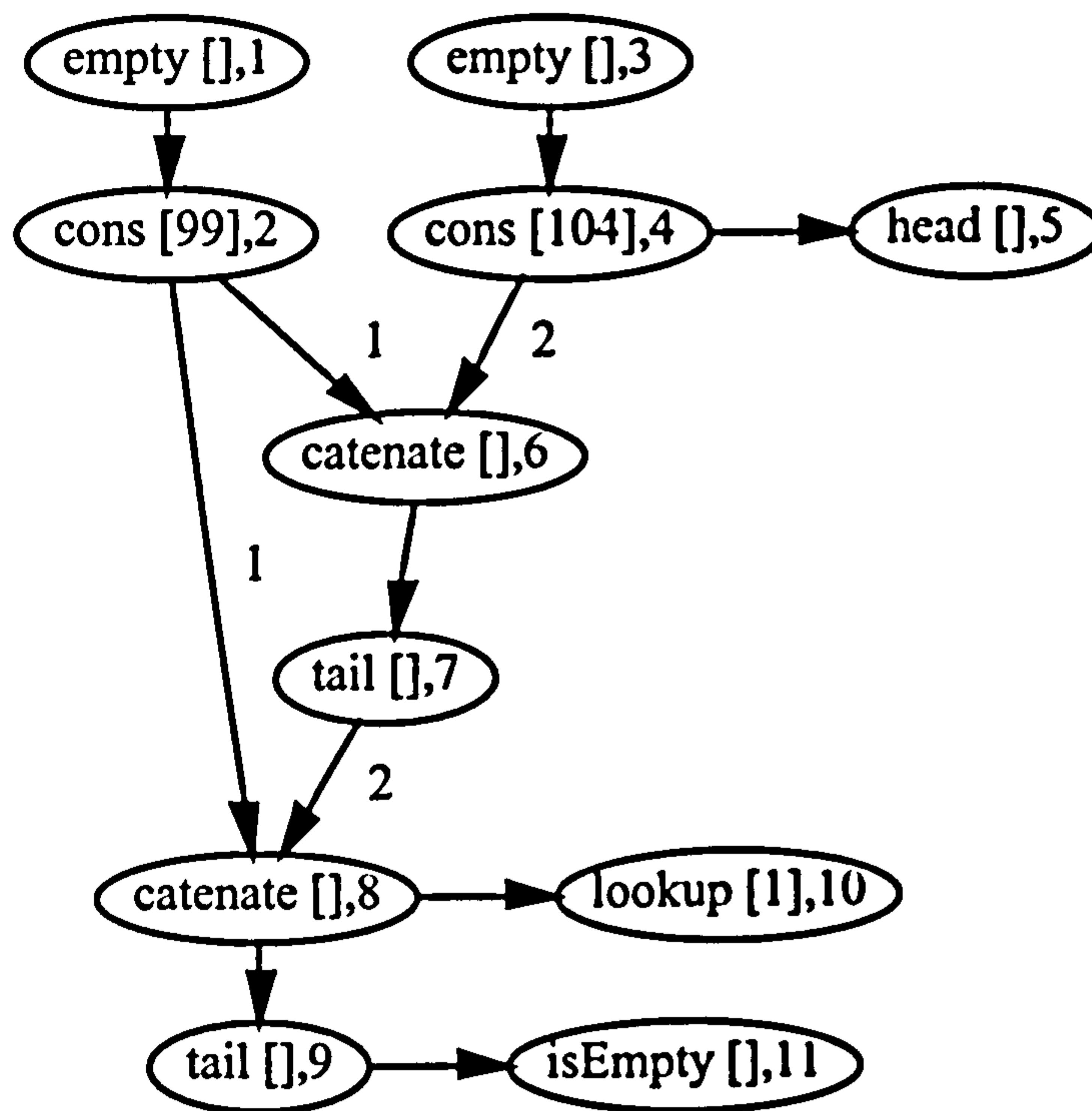
Figure 6.4: Output from the GraphViz package viewing the DAG of Figure 3.4 (the orientation, the spacing and the font size were altered so the output could fit on this page). The functions \eta , \sigma , and \tau —see Definition 3.6—are indicated on the graph. Each node is labelled with the partial application given by \eta (the name of an operation and a list of non-version arguments), and the node's position in the order of evaluation, given by \sigma . The arc labels given by \tau are placed next to the relevant arcs.
