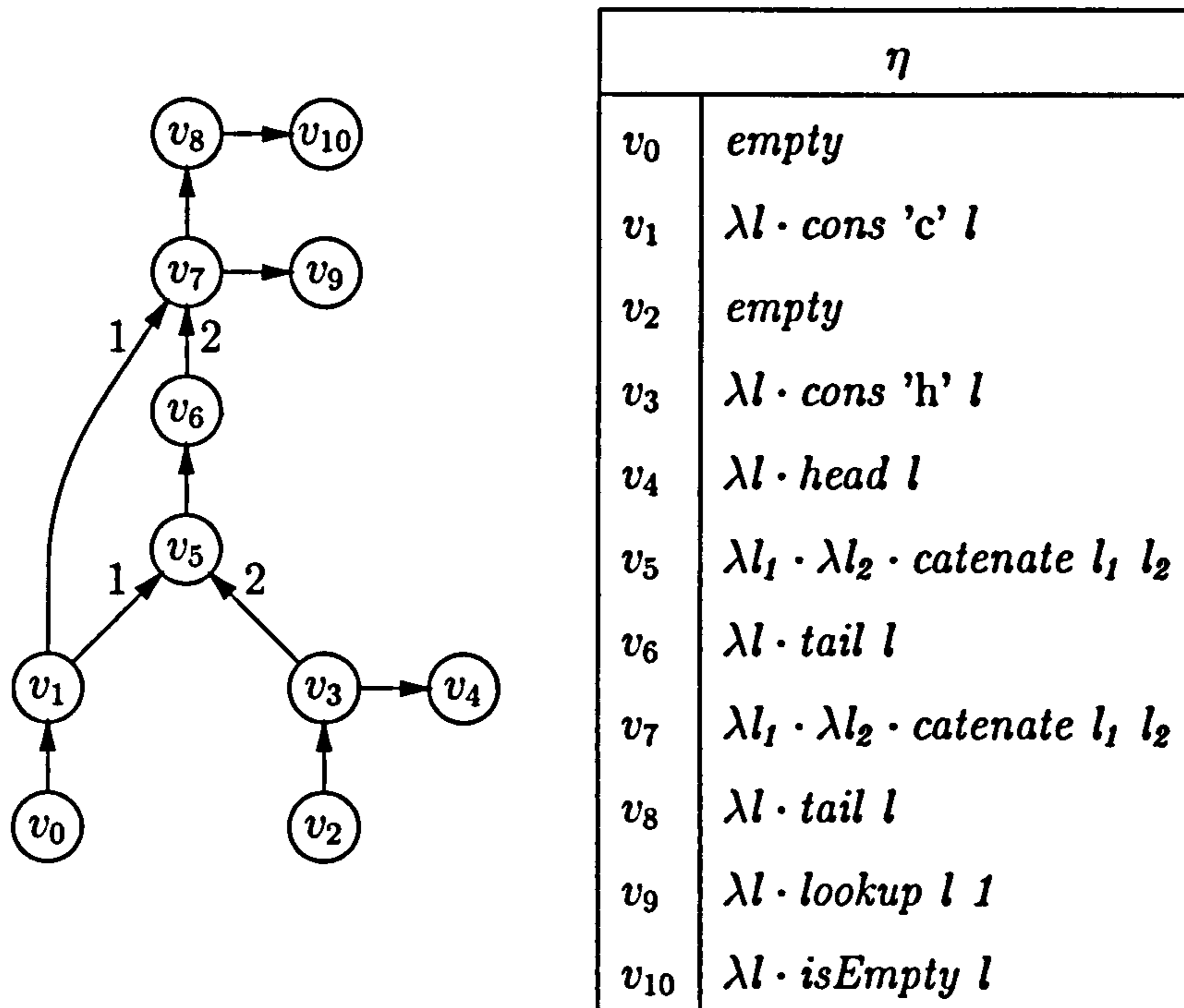
Figure 3.4: A DUG for the list ADT \mathcal{A}_{List} (see Figure 3.3).
