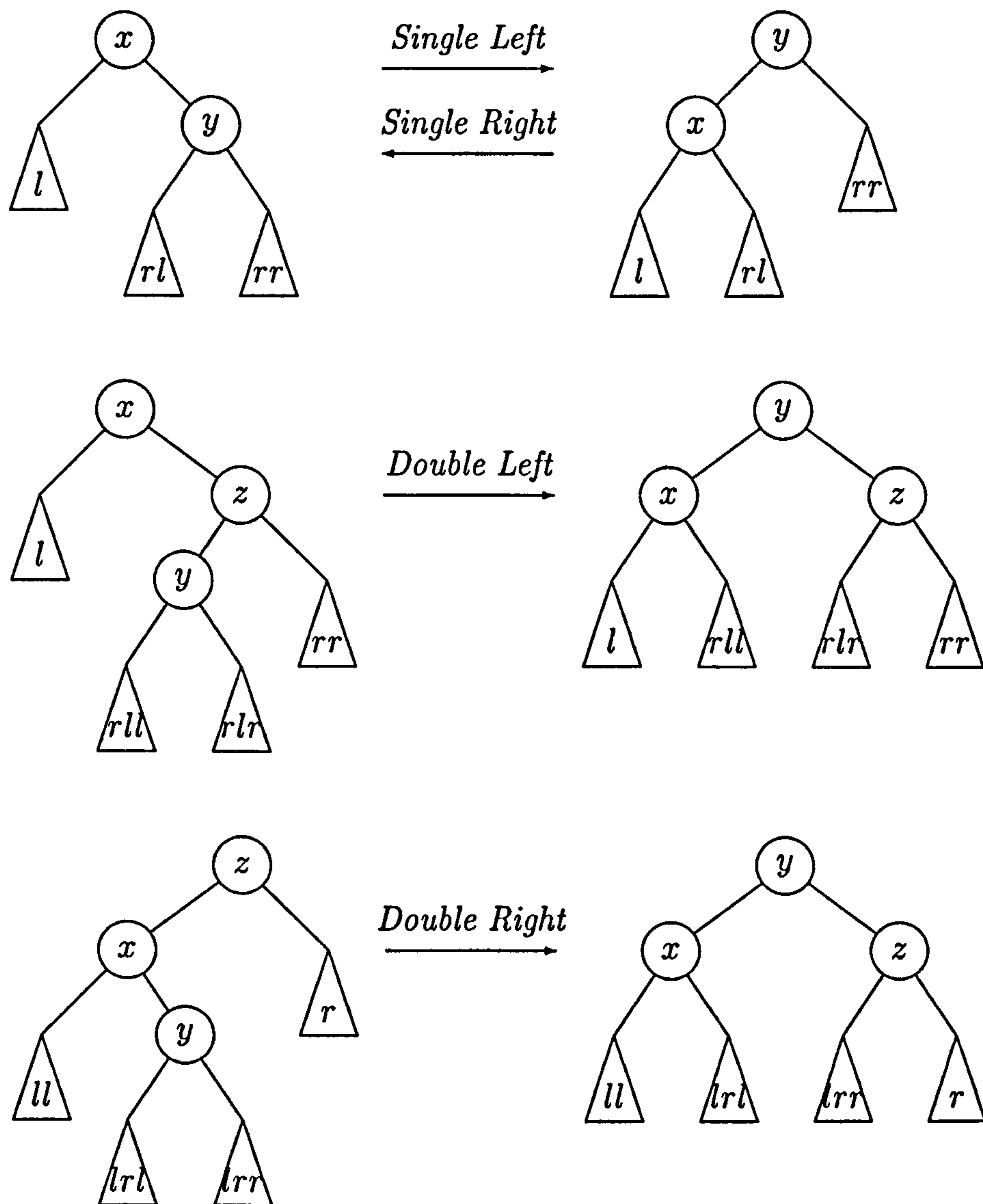
Figure 2.4: Rotations of a binary tree.
