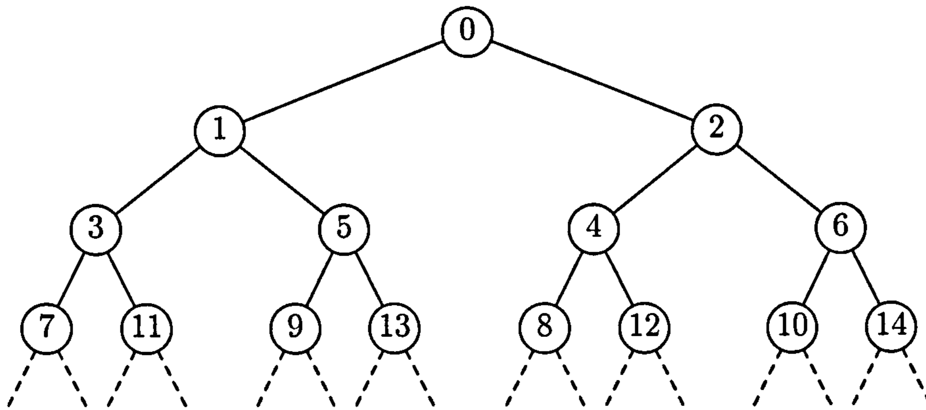
Figure 2.7: The infinite Braun tree.
