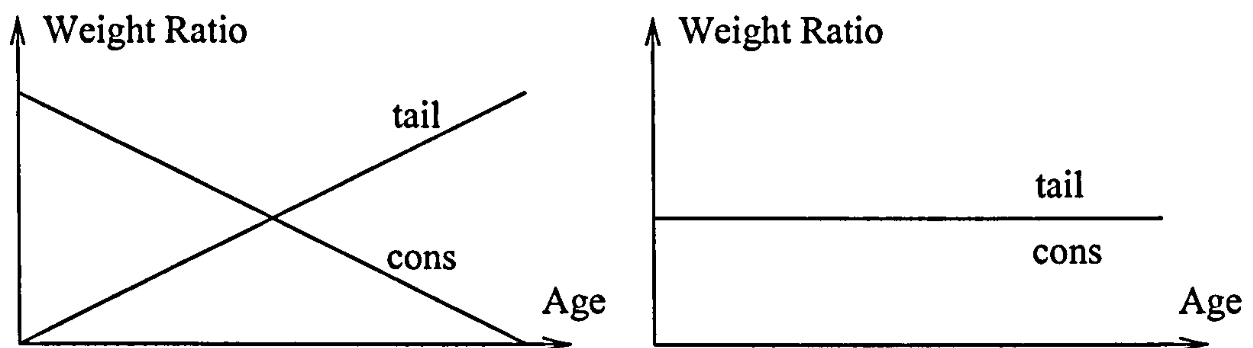
Figure 5.3: Two linear functions giving weight ratios for lists. Each produce an equal number of applications of cons and tail , but the left one produces applications on larger lists.
