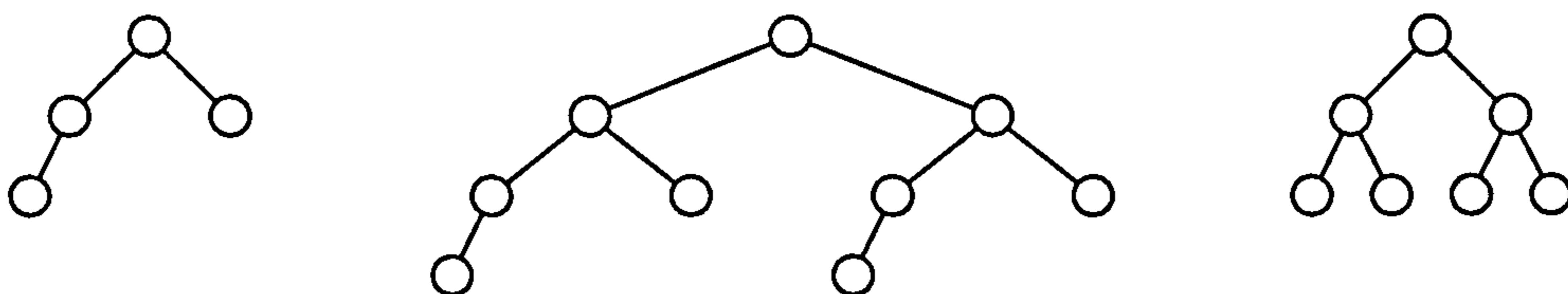
Figure 2.8: The Braun trees of size four, nine and seven.
