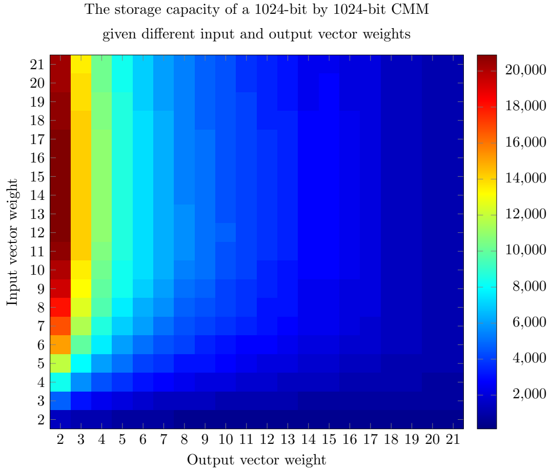
Figure 3.7: Heat map showing how the capacity of a CMM changes as the input and output vector weights are independently varied. The capacity is considered as the point at which the number of associated vector pairs cannot be increased without the recall success rate falling below 99%. All vector lengths are 1024-bits; the input and output vector weights are independently varied between 2 and 21.
