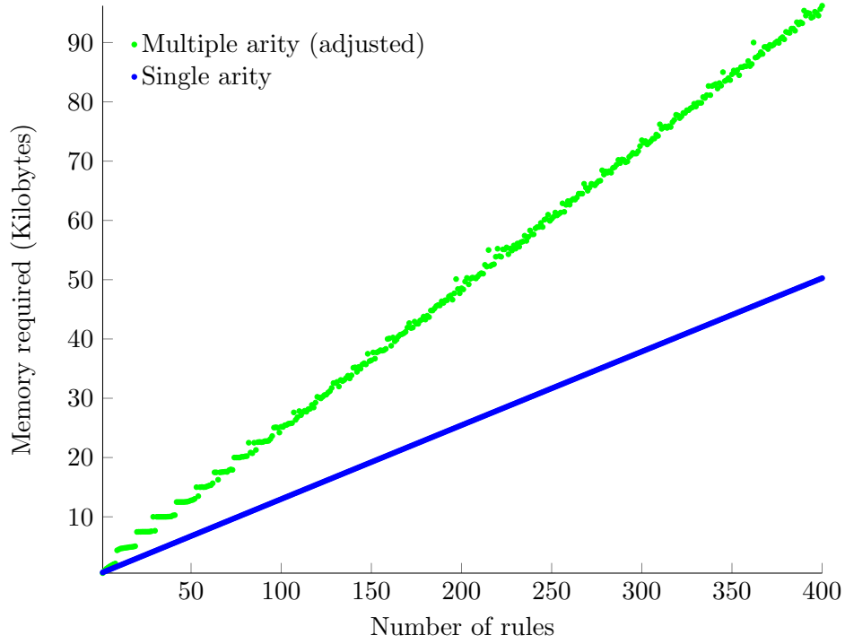
Single and multiple arity ARCA performance with maximum branching factor 2
