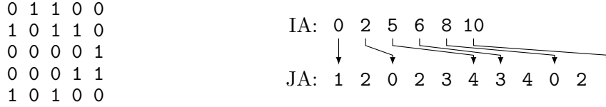
Figure 3.2: An example binary matrix represented non-sparately (on the left) and using the binary Yale format (on the right). In the binary Yale format the first array (IA) stores indexes into the second array (JA) to denote the beginning of each matrix row. JA then stores the column indices of bits set to one.
