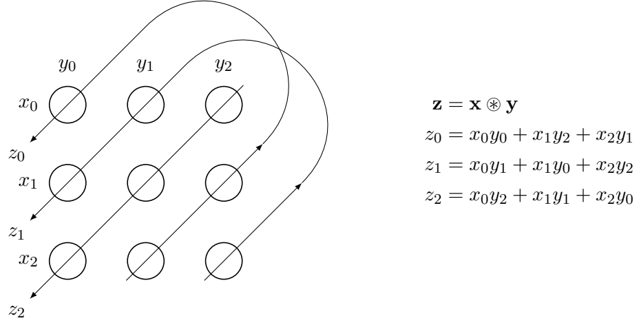
Figure 2.7: Circular convolution with vectors of length 3 ( n = 3 ) [85]. Each of the circles is an element of the outer product of \mathbf{x} and \mathbf{y} . Each of the elements of the final circular convolution are sums along the diagonal lines.
