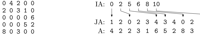
Figure 3.1: An example matrix represented non-sparately (on the left) and using the Yale format (on the right). In the Yale format the first array (IA) stores indexes into the other arrays to denote the beginning of each matrix row. The second array (JA) stores the column indices of non-zero elements. Finally, the main array (A) stores the values of each of the non-zero elements.
