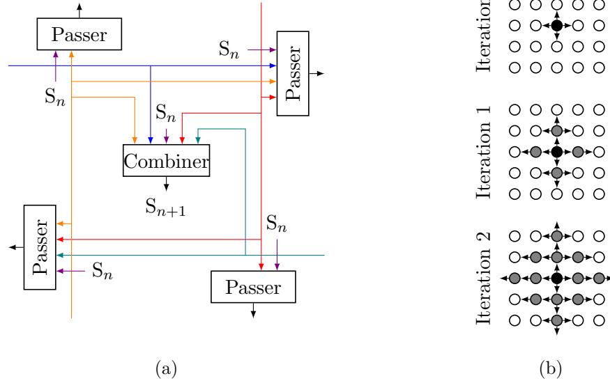
Figure 5.2: (a) The “Corner Turning 2” CANN module configuration, where S_n is the cell state (the output of the combiner module) after the n^{\text{th}} iteration and (b) information flow of this configuration over two iterations [16].
