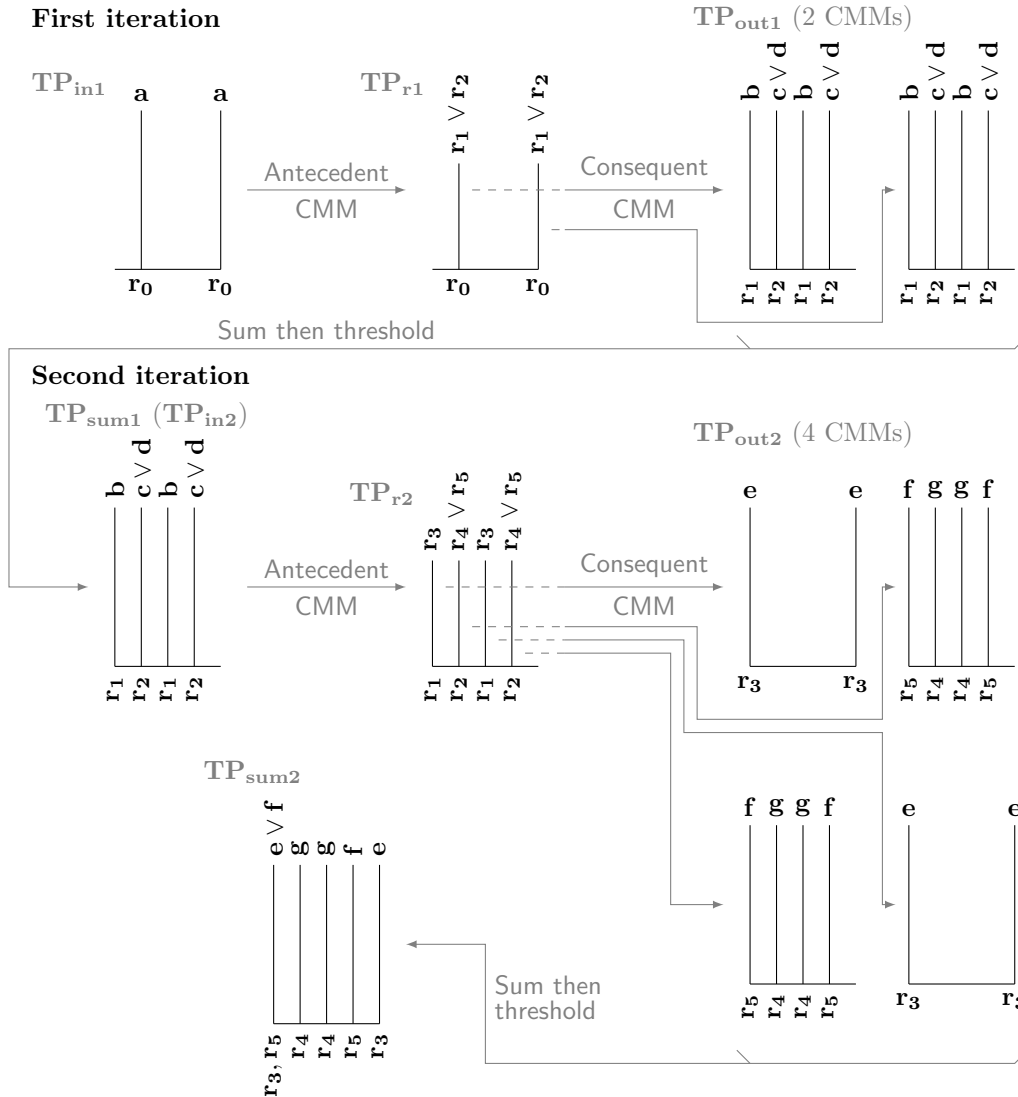
Figure 4.4: A visualisation of two iterations of the rule chaining process within ARCA. The process is initialised by creating a tensor product, \mathbf{TP}_{in1} , binding the input tokens (in this case a ) to a rule vector ( r_0 ). Each column of this tensor product is then recalled in turn from the antecedent CMM, to form a new tensor product, \mathbf{TP}_{r1} , containing the rules which have fired. Each column of \mathbf{TP}_{r1} can then be recalled in turn from the consequent CMM, resulting in a number of output tensor products ( \mathbf{TP}_{out1} —one tensor product for every non-zero column of \mathbf{TP}_{r1} ). These output tensor products can be summed to form a non-binary CMM, before a threshold is applied using a value equal to the weight of a rule vector and resulting in \mathbf{TP}_{sum1} . The second iteration continues in the same fashion, using \mathbf{TP}_{sum1} as the new input tensor product.
