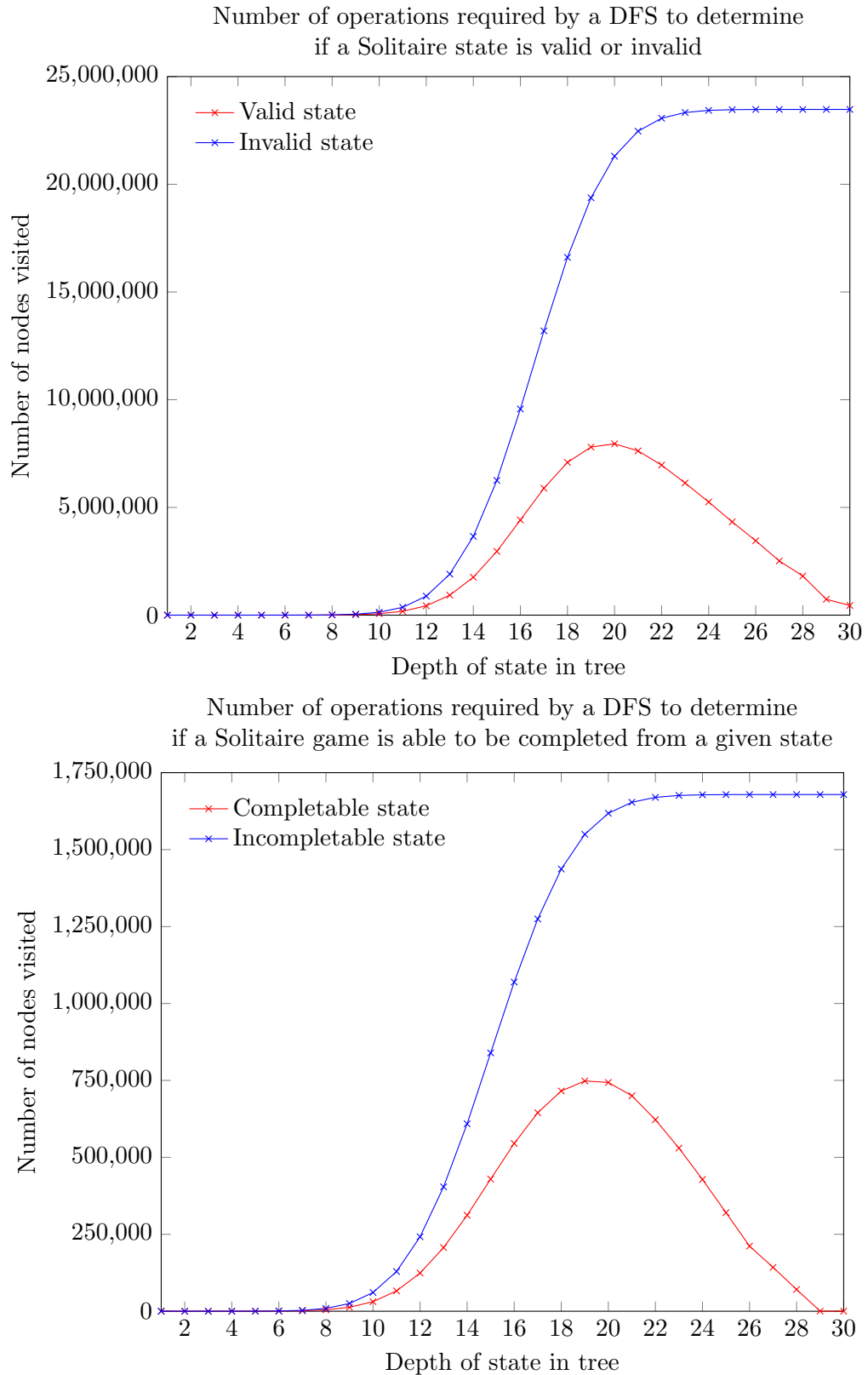
Figure 4.24: Plots showing the number of operations required by a DFS, compared to the single operation ARCA requires. For each depth of tree the plots show the average number of nodes which must be inspected to find a valid/completable state, as well as the number of nodes which must be inspected to determine that a state is invalid/incompletionable.
